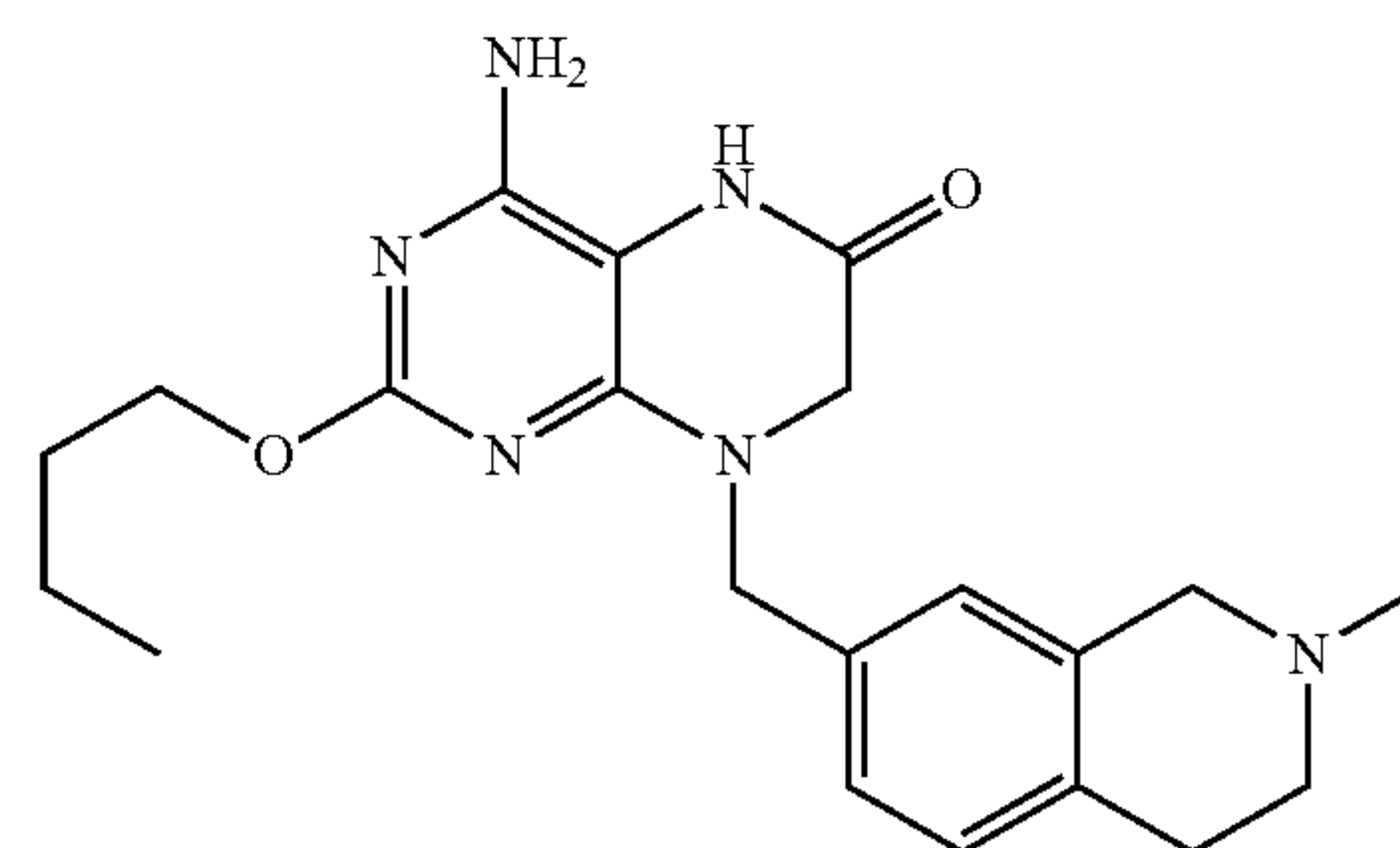
Example 52
