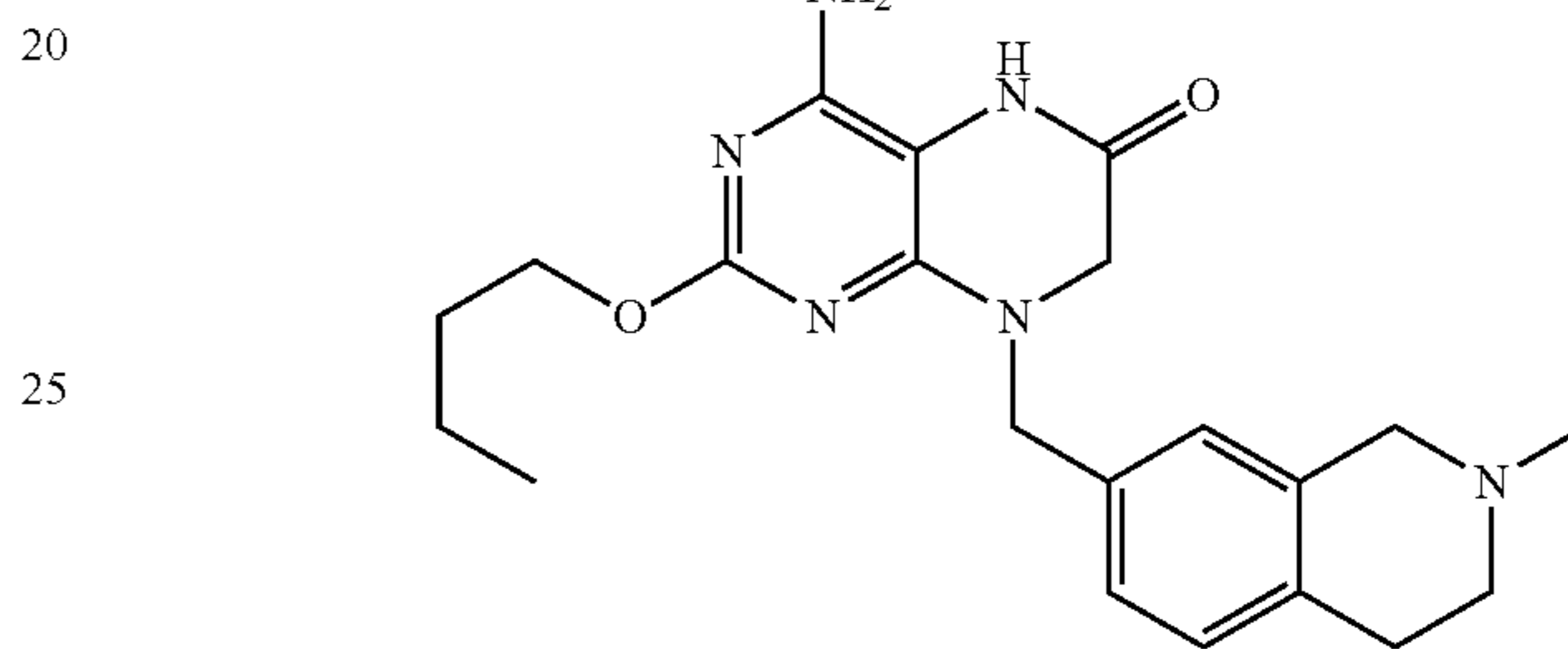
Example 52
