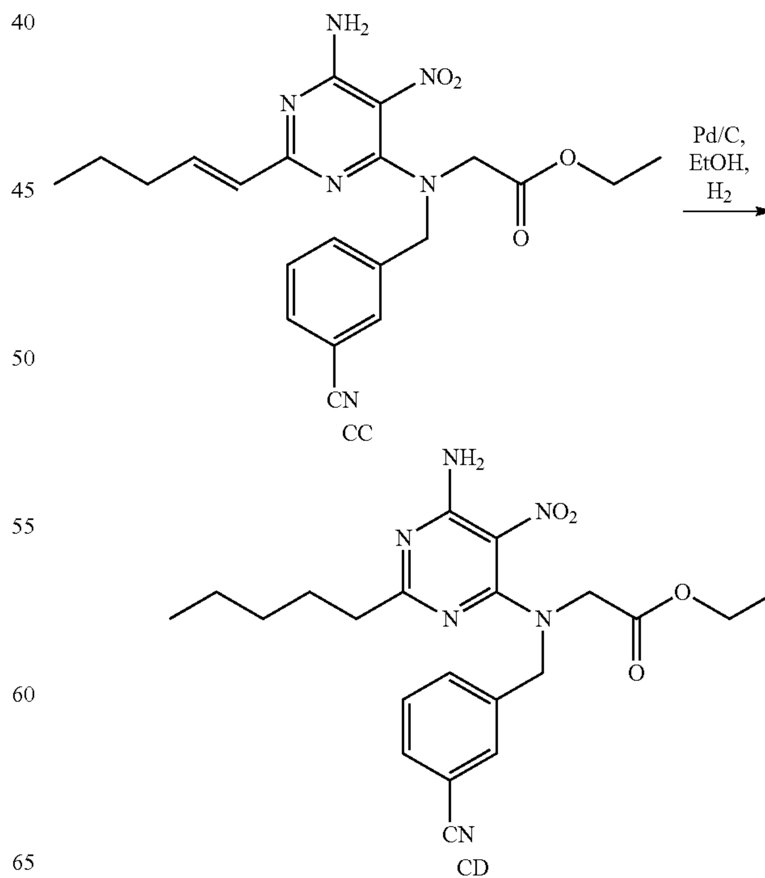
Scheme 51
