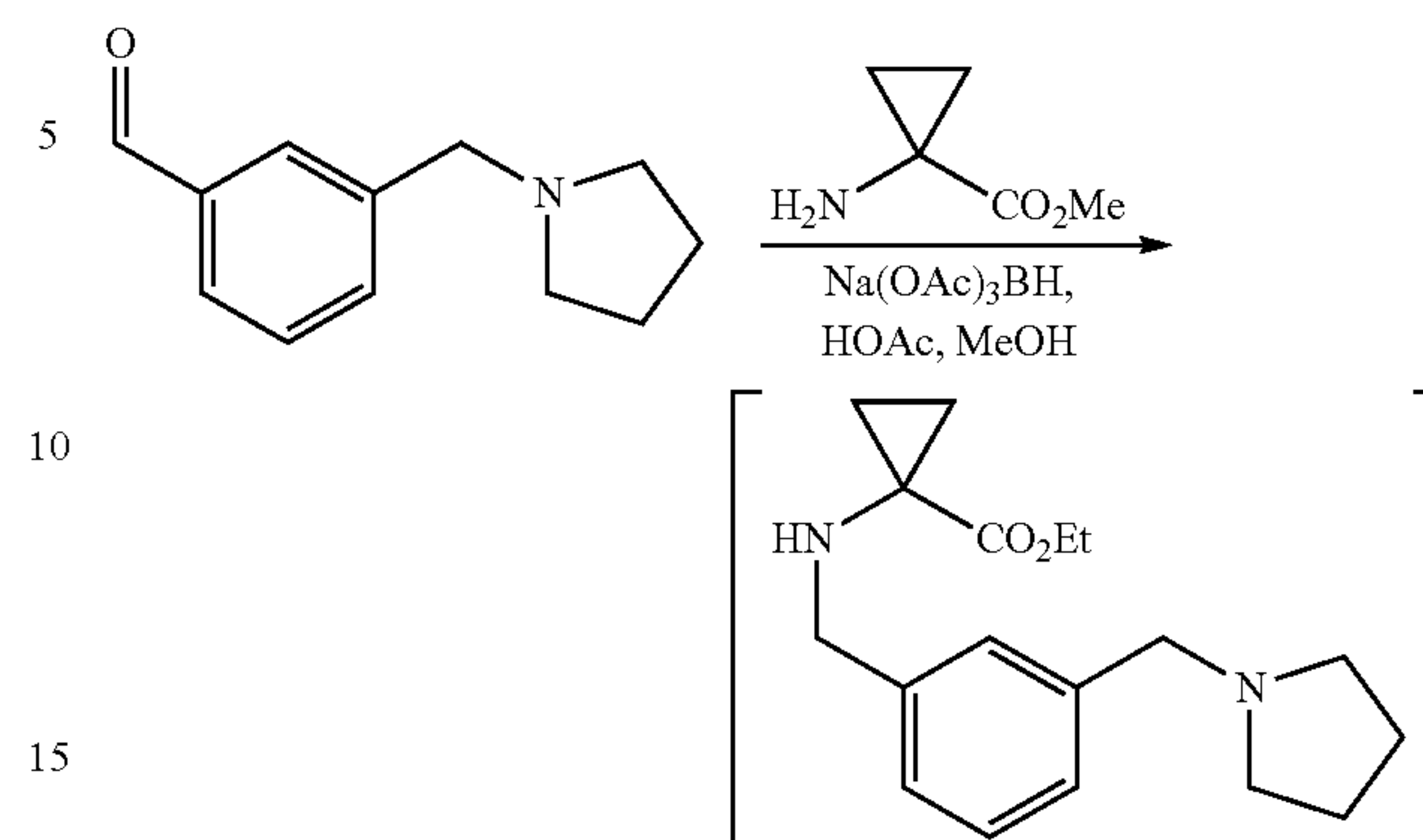
Scheme 12
