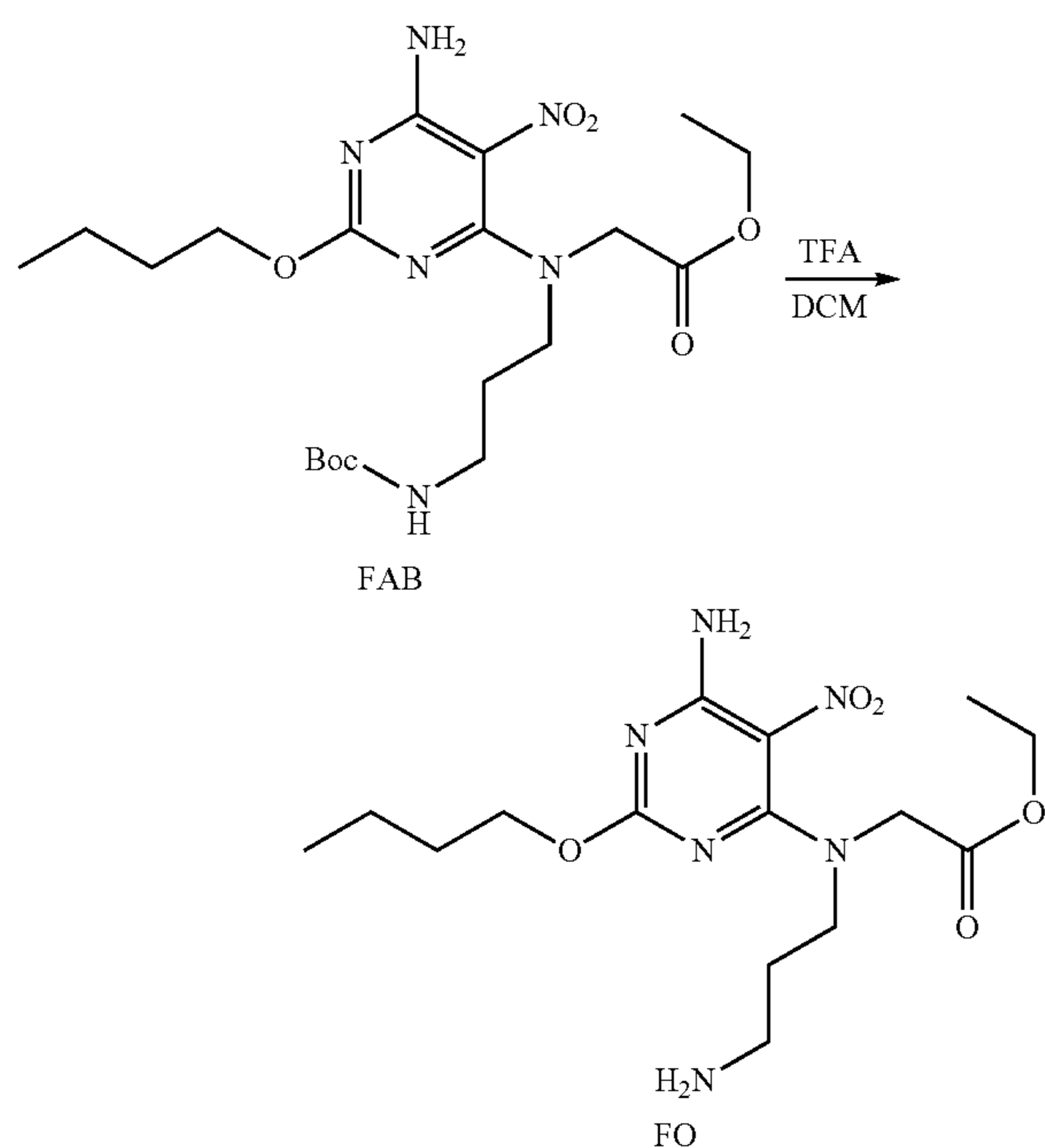
Scheme 105:
