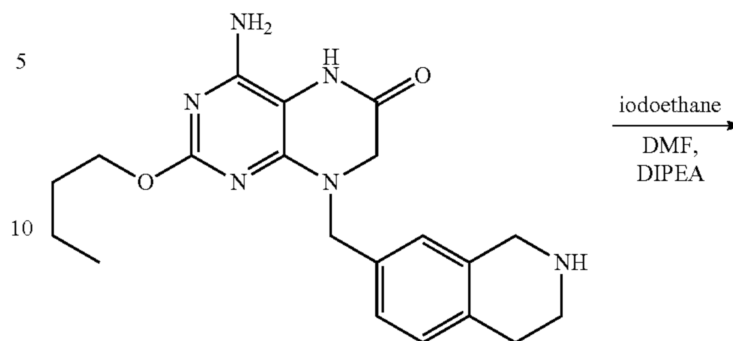
Example 51
