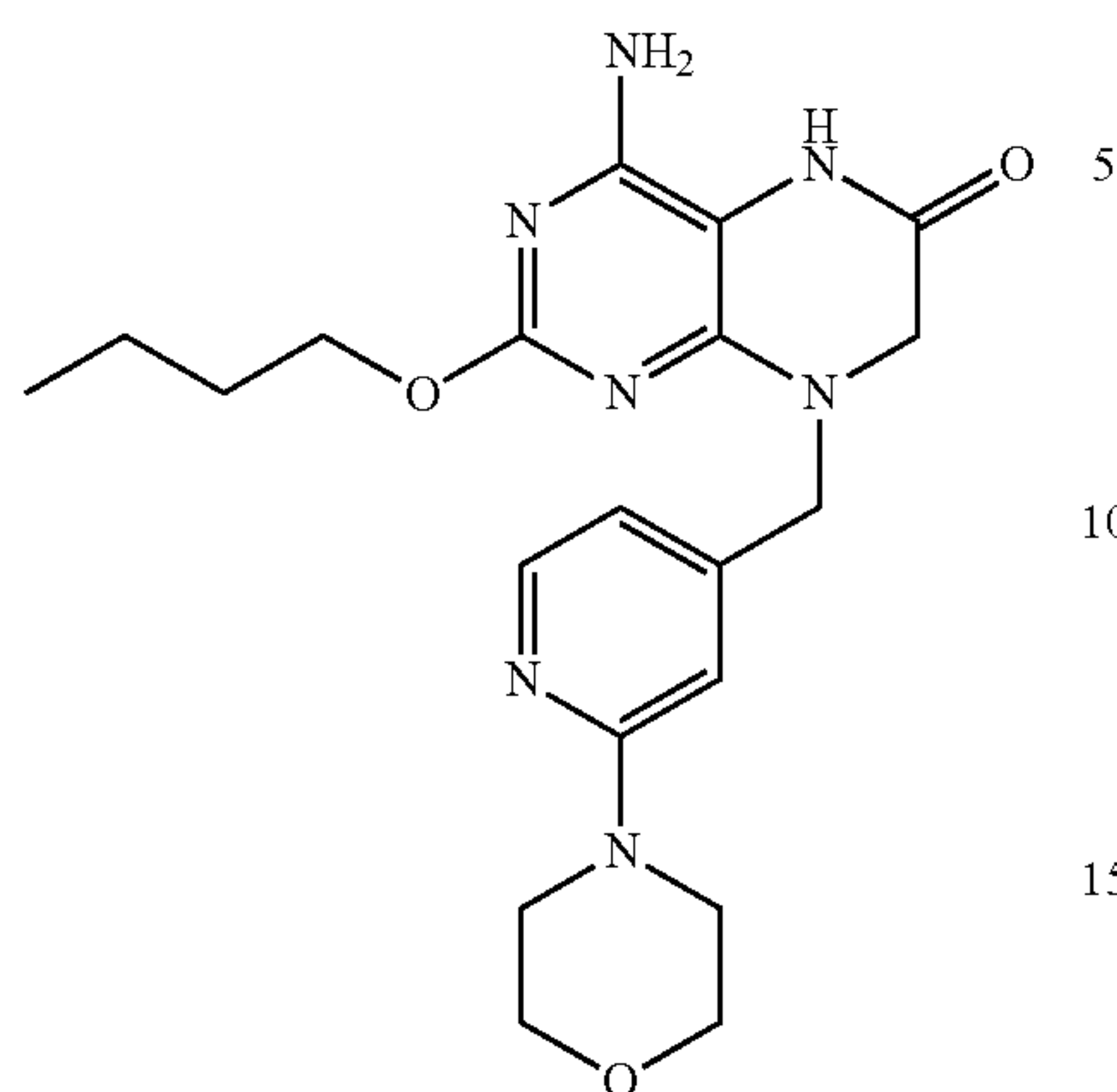
Example 66
