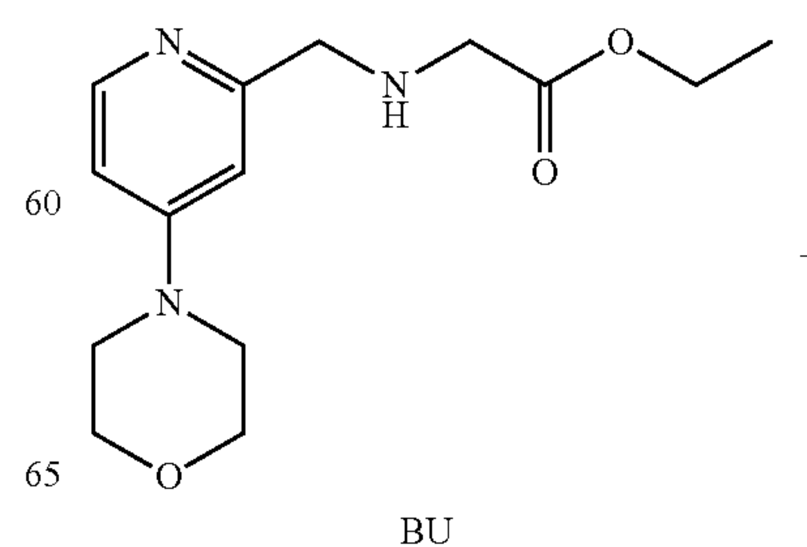
Scheme 43
