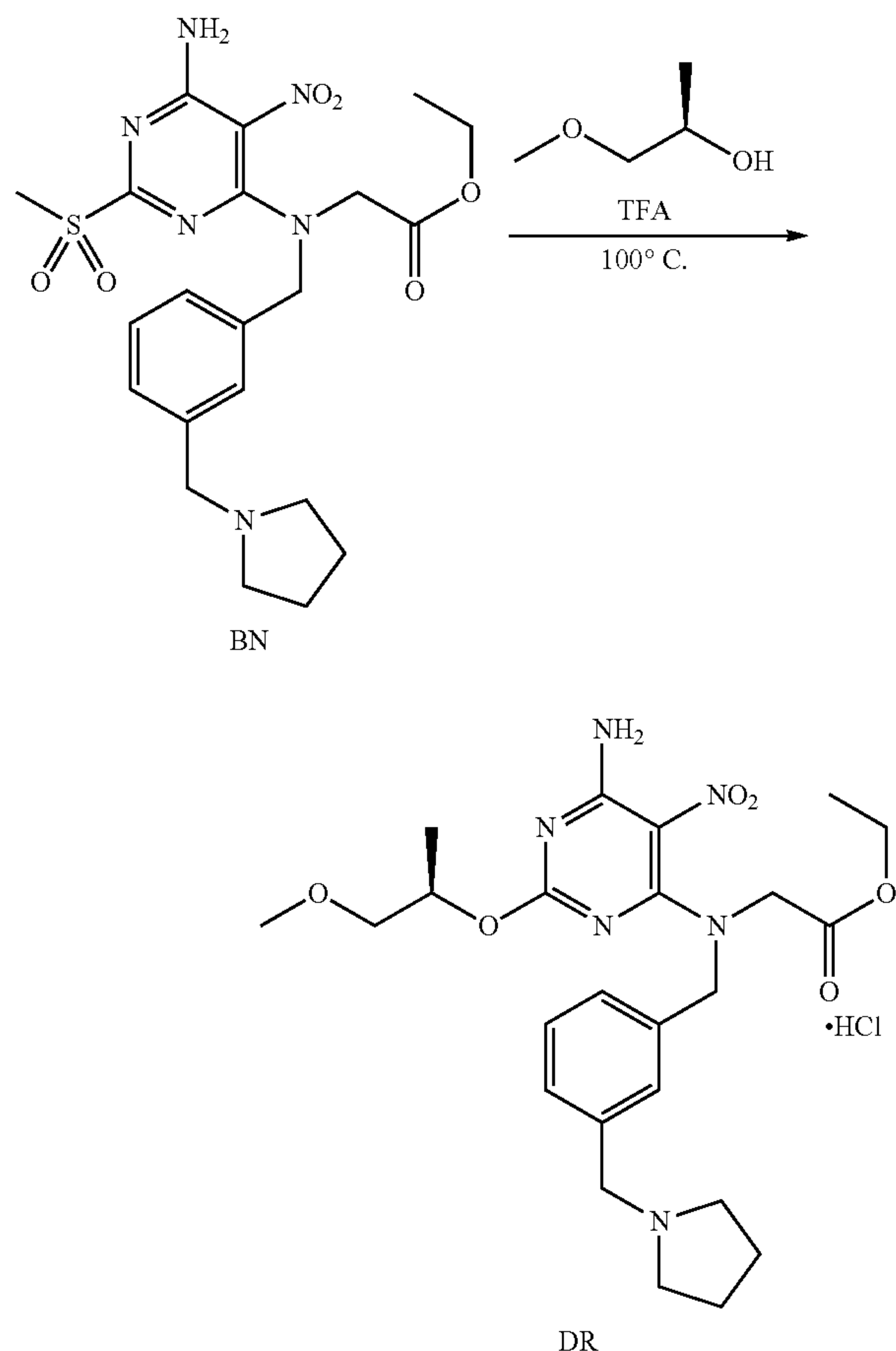
Scheme 85
