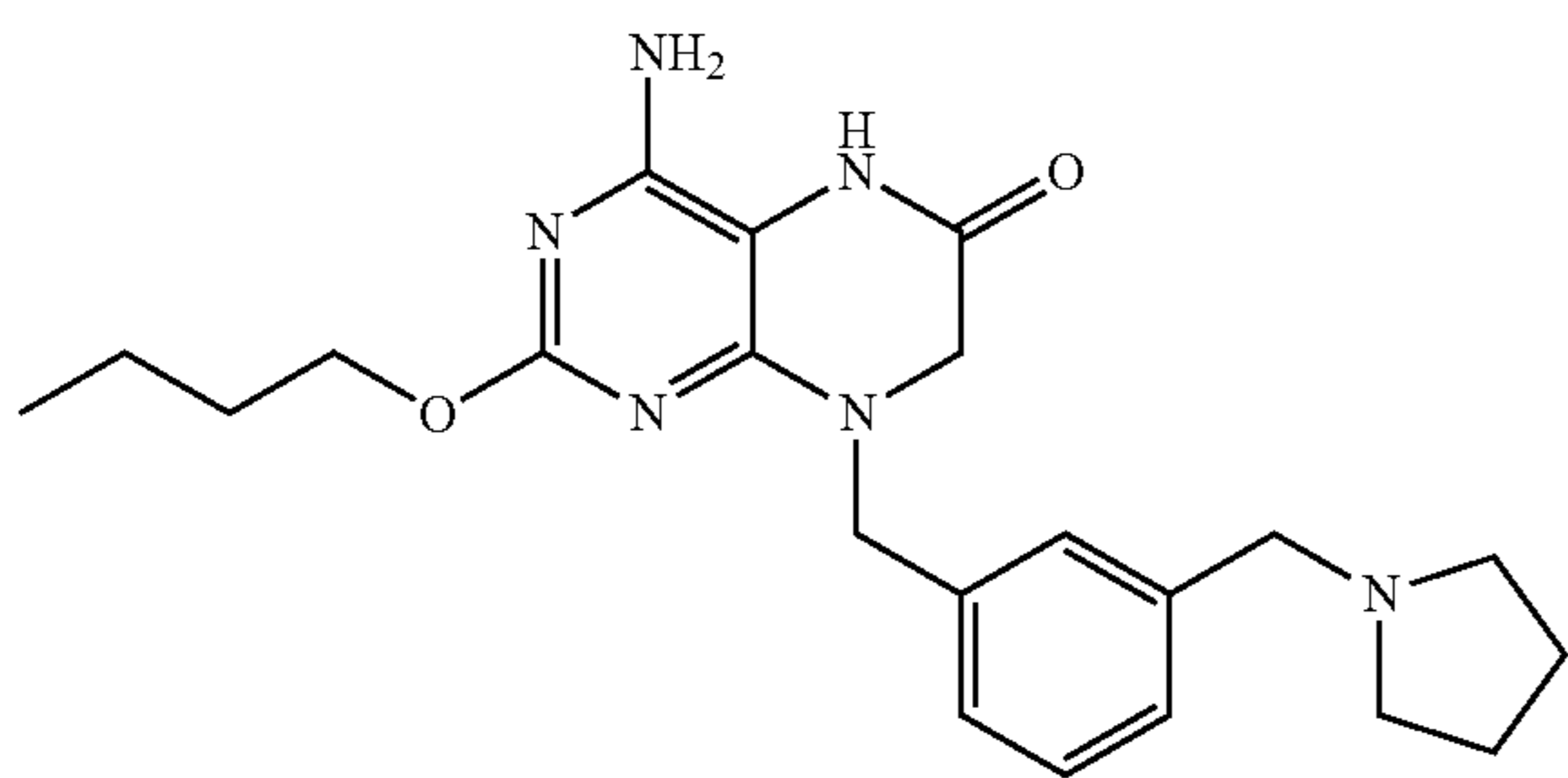
4-amino-2-n-butoxy-8-[3'-(pyrrolidin-1''-ylmethyl)-benzyl]-5,6,7,8-tetrahydropyrido[2,1-b]imidazole-6-one
