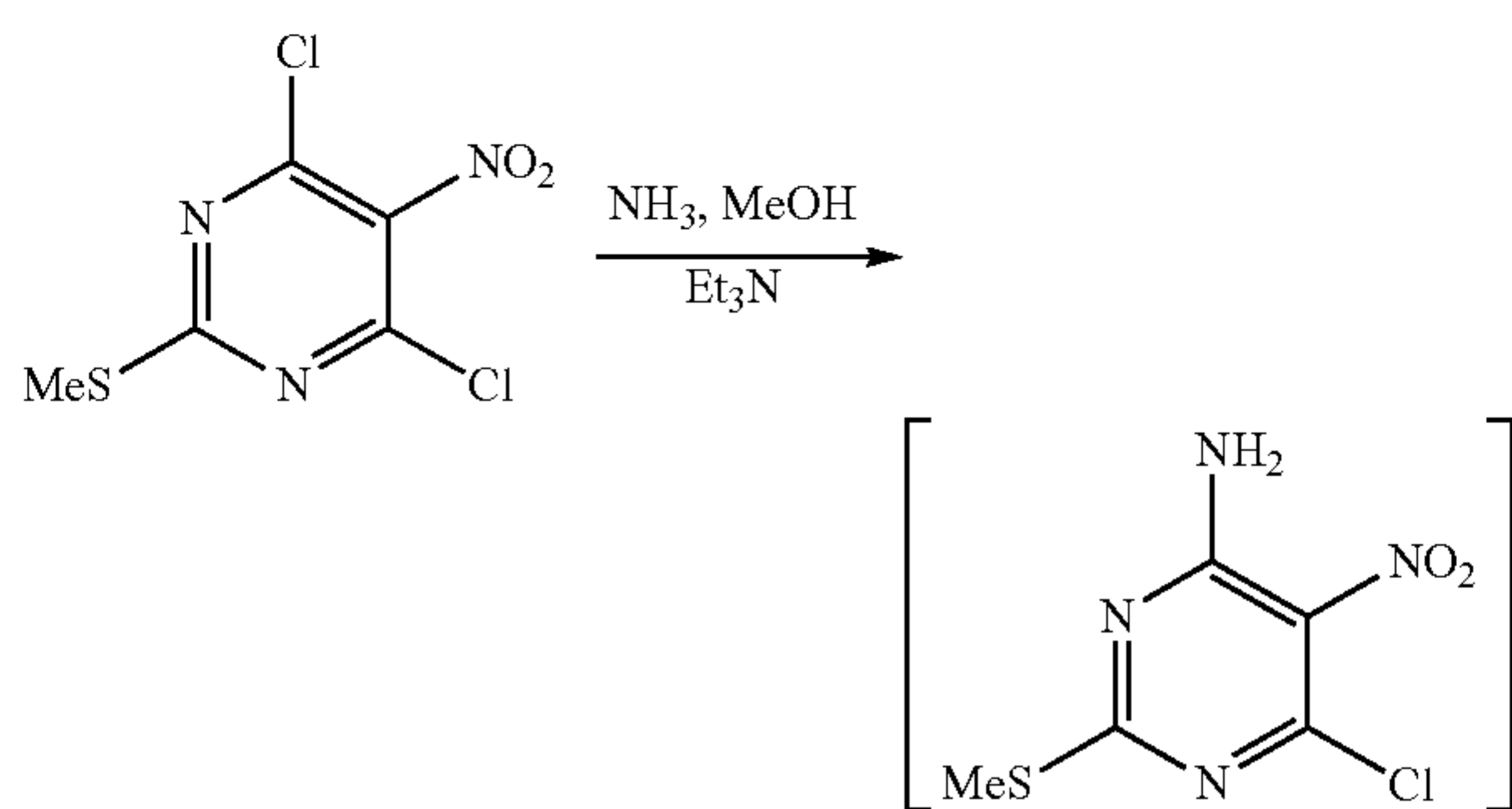
Scheme 18
