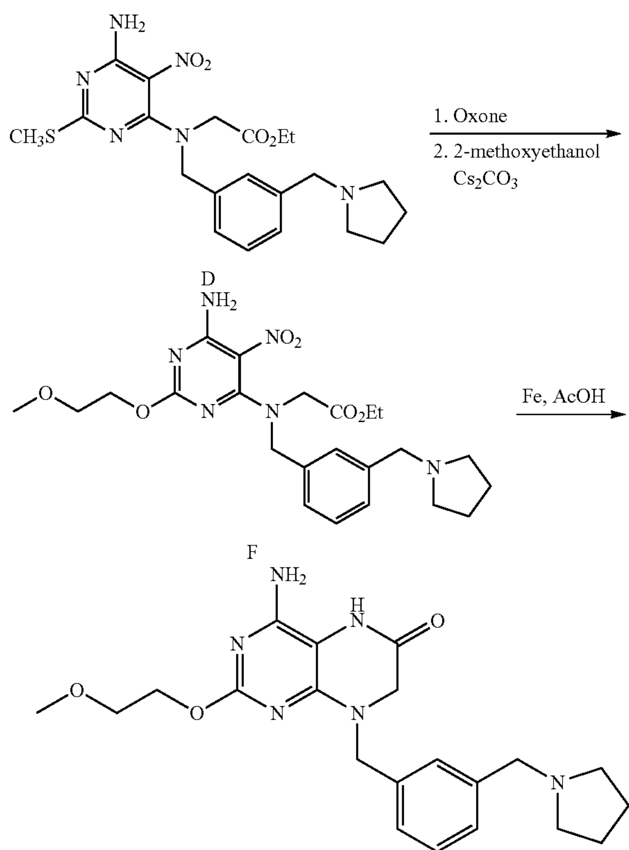
Example 2
