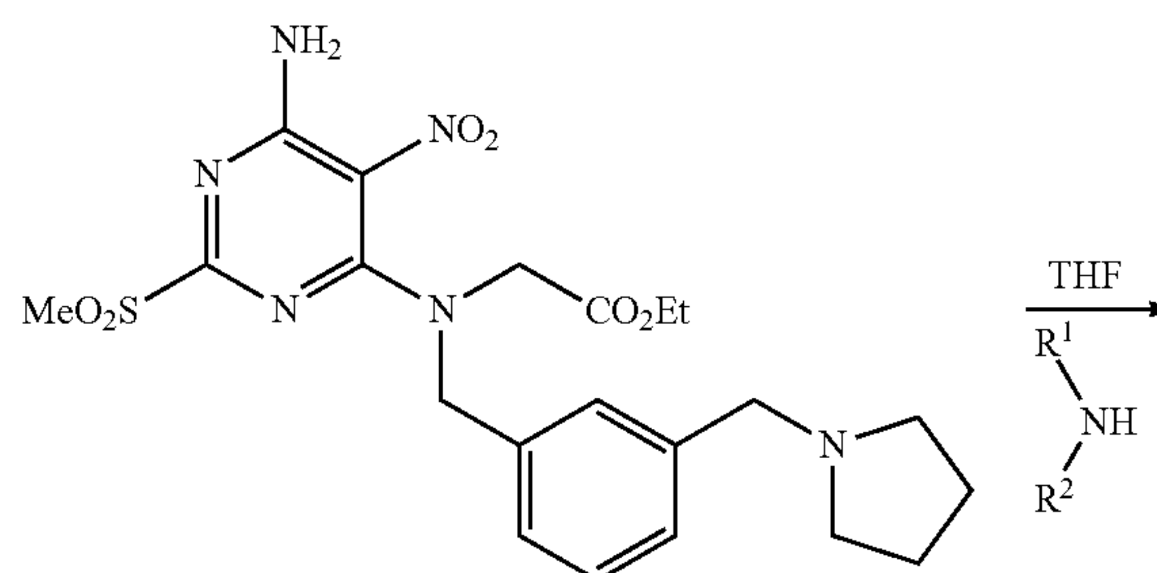
Scheme 16
