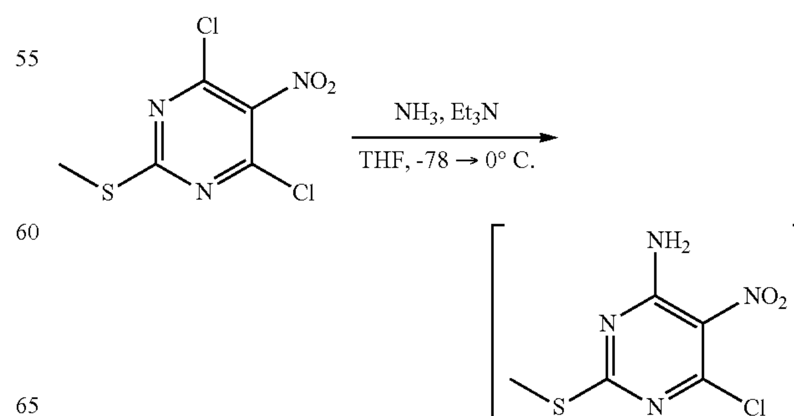
Scheme 34
