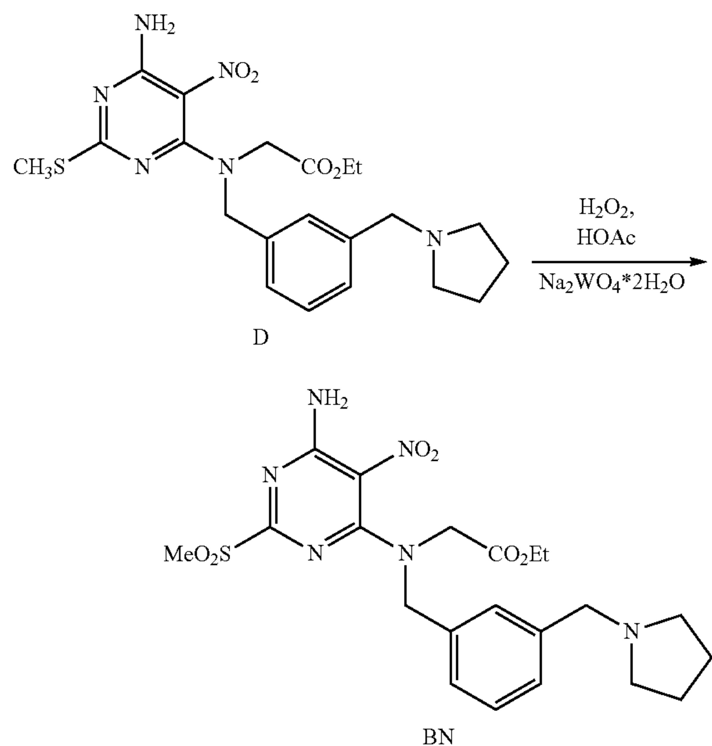
Scheme 32
