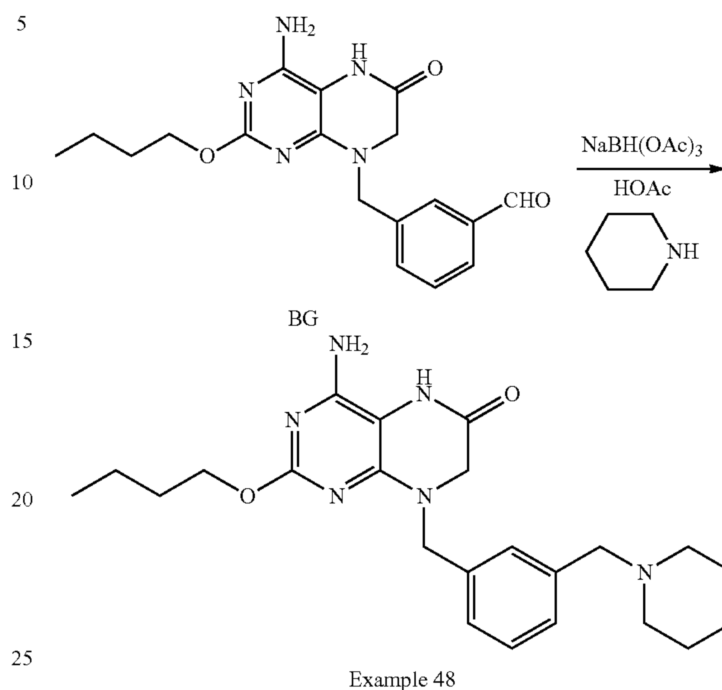
Scheme 26
