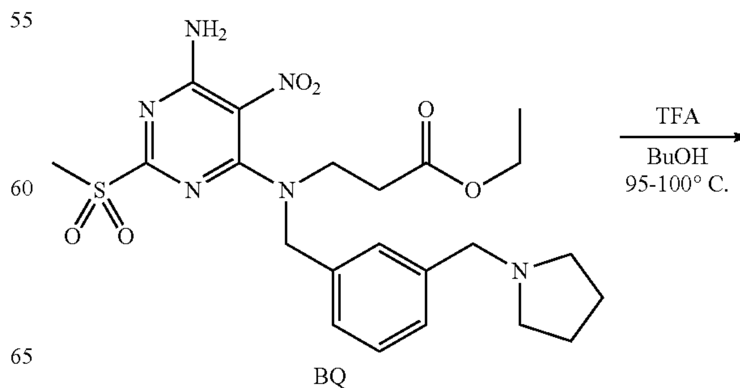
Scheme 37
