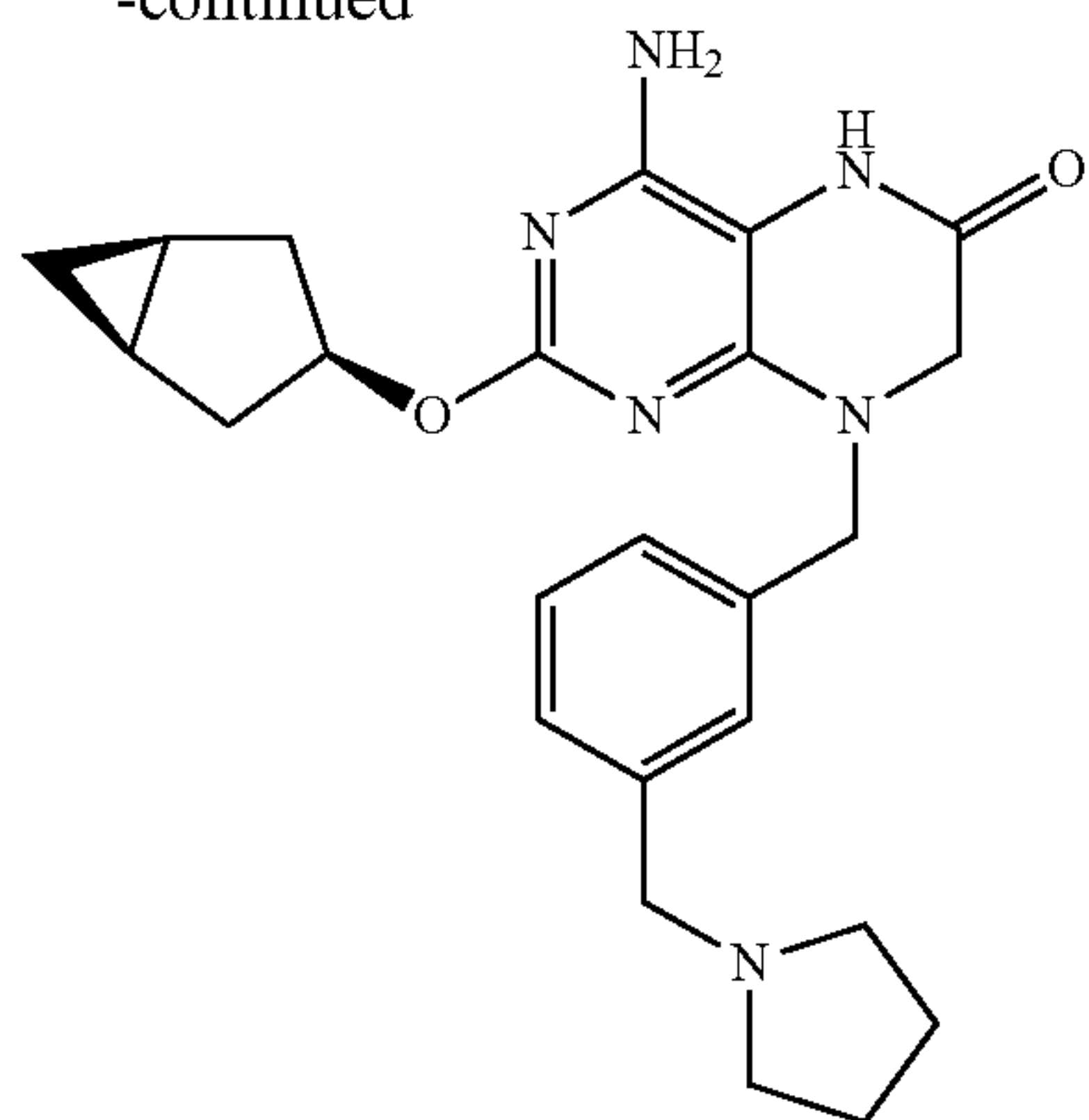
Example 68
