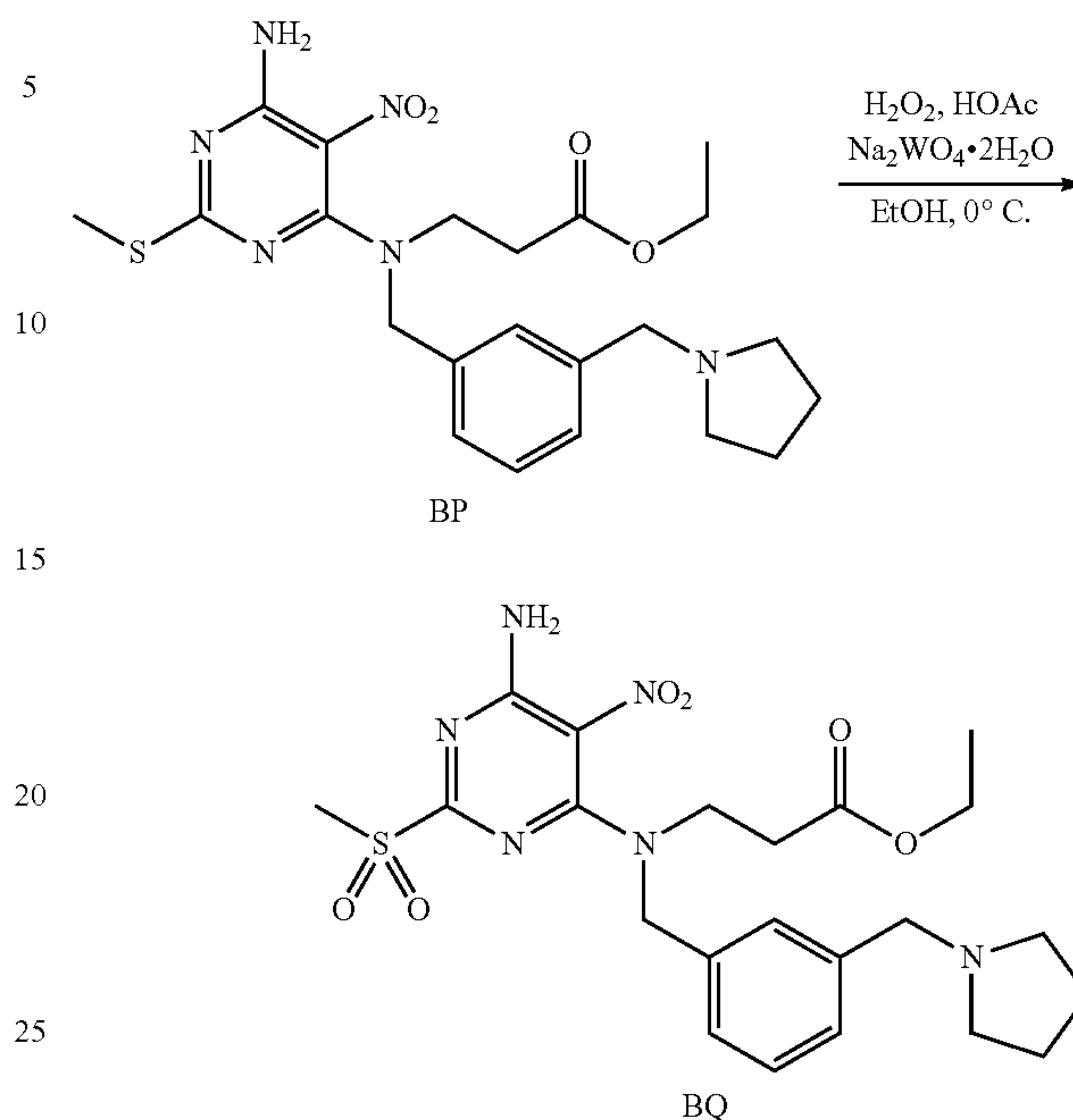
Scheme 36
