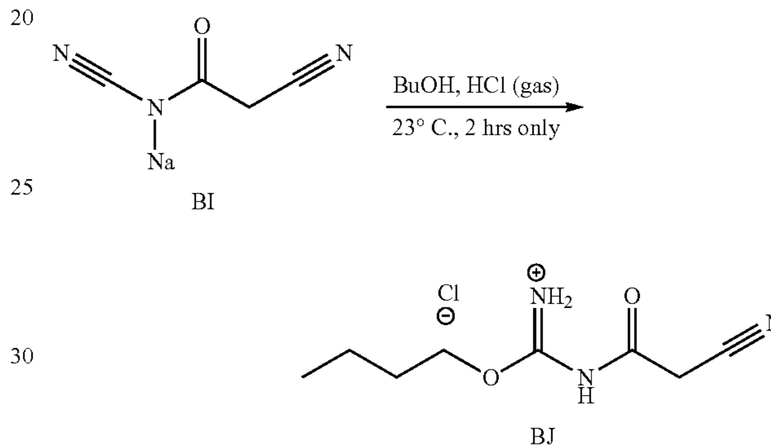
4-amino-2-n-butoxy-8-[3'-(pyrrolidin-1'-ylmethyl)-benzyl]-5,6,7,8-tetrahydropyrido-6-one
