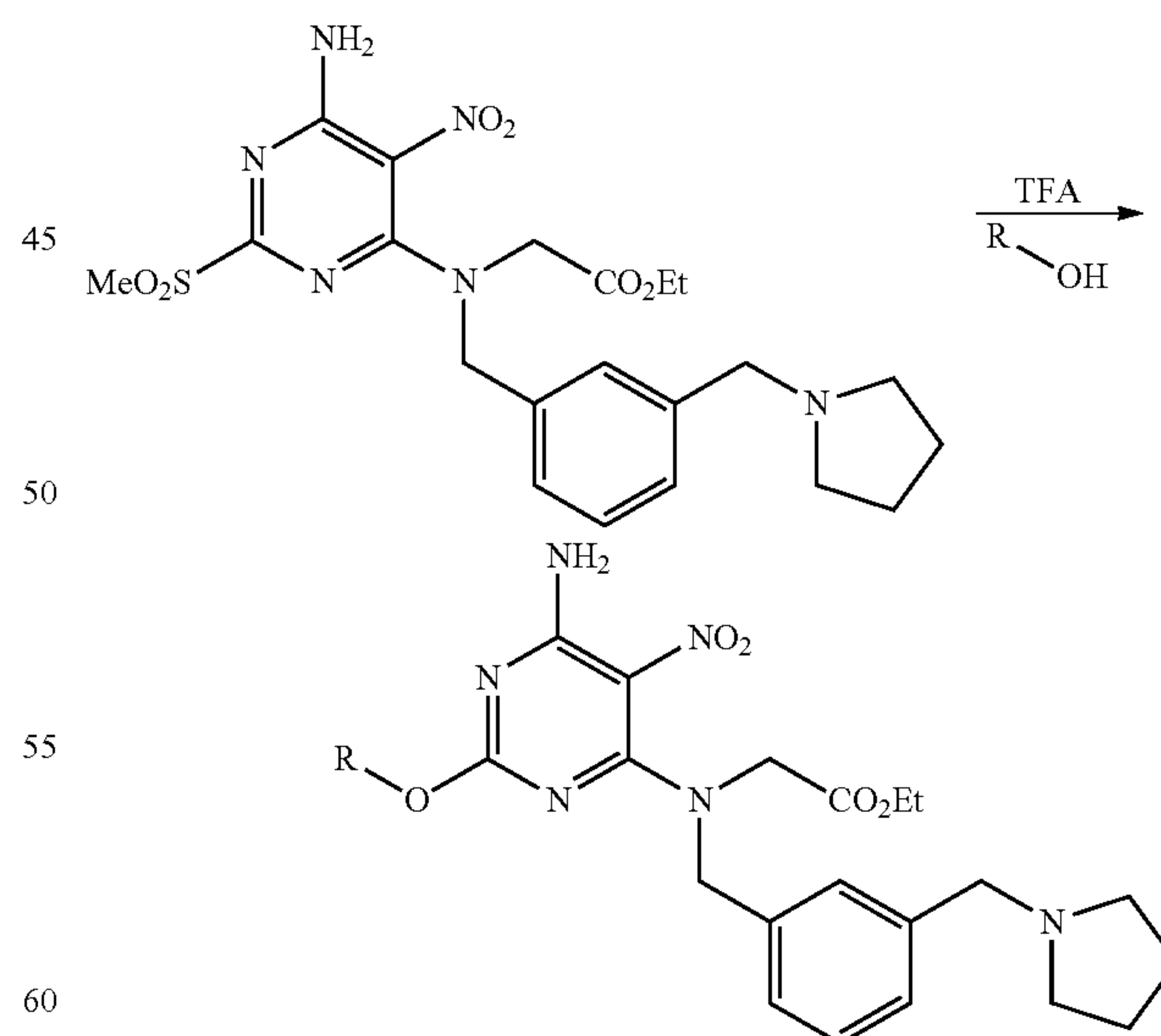
Scheme 13
