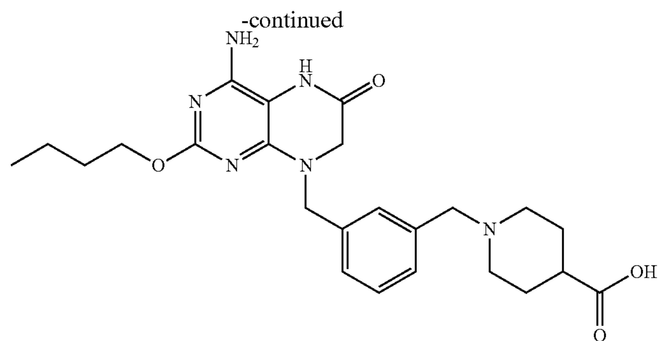
Example 75
