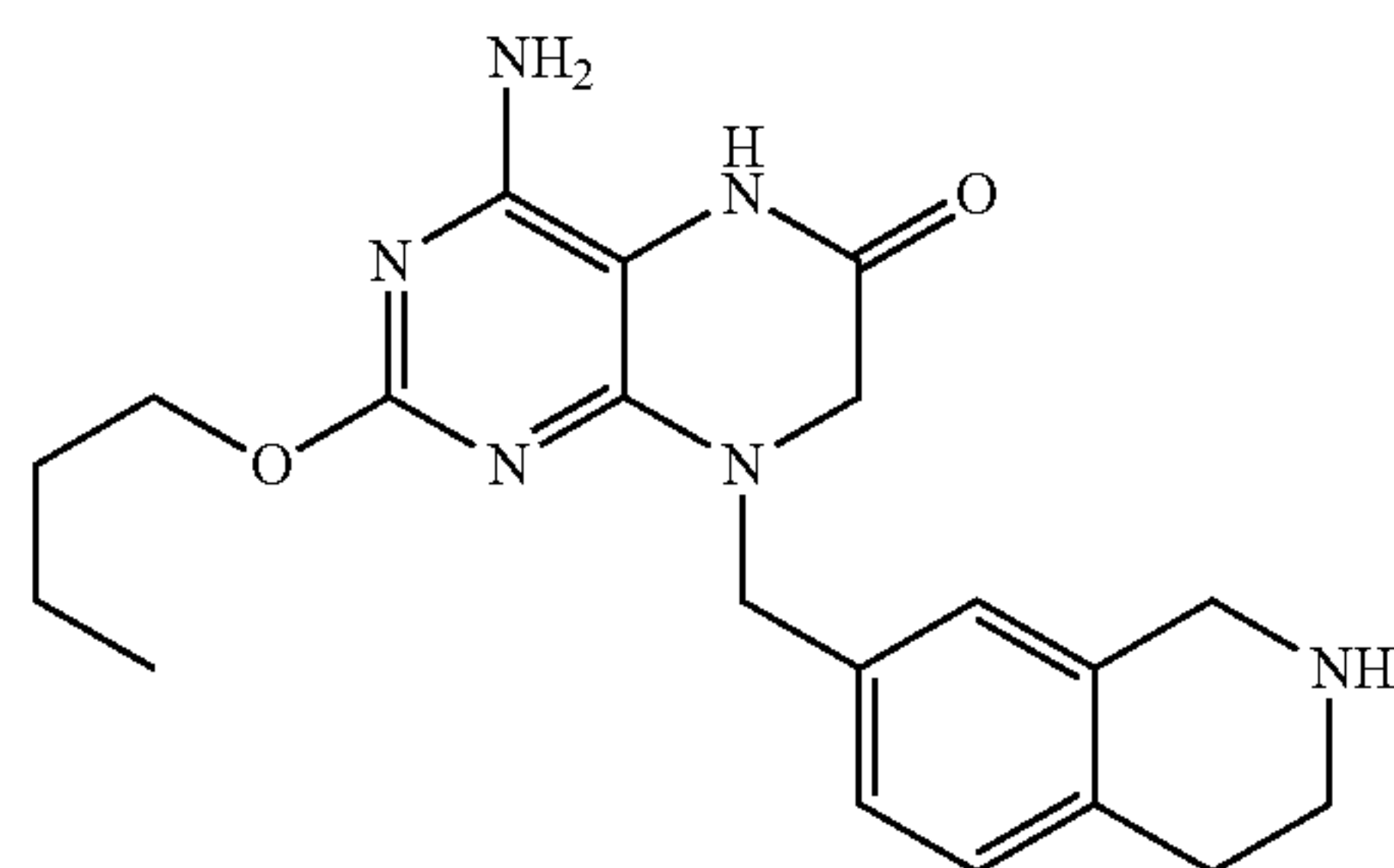
Example 51
