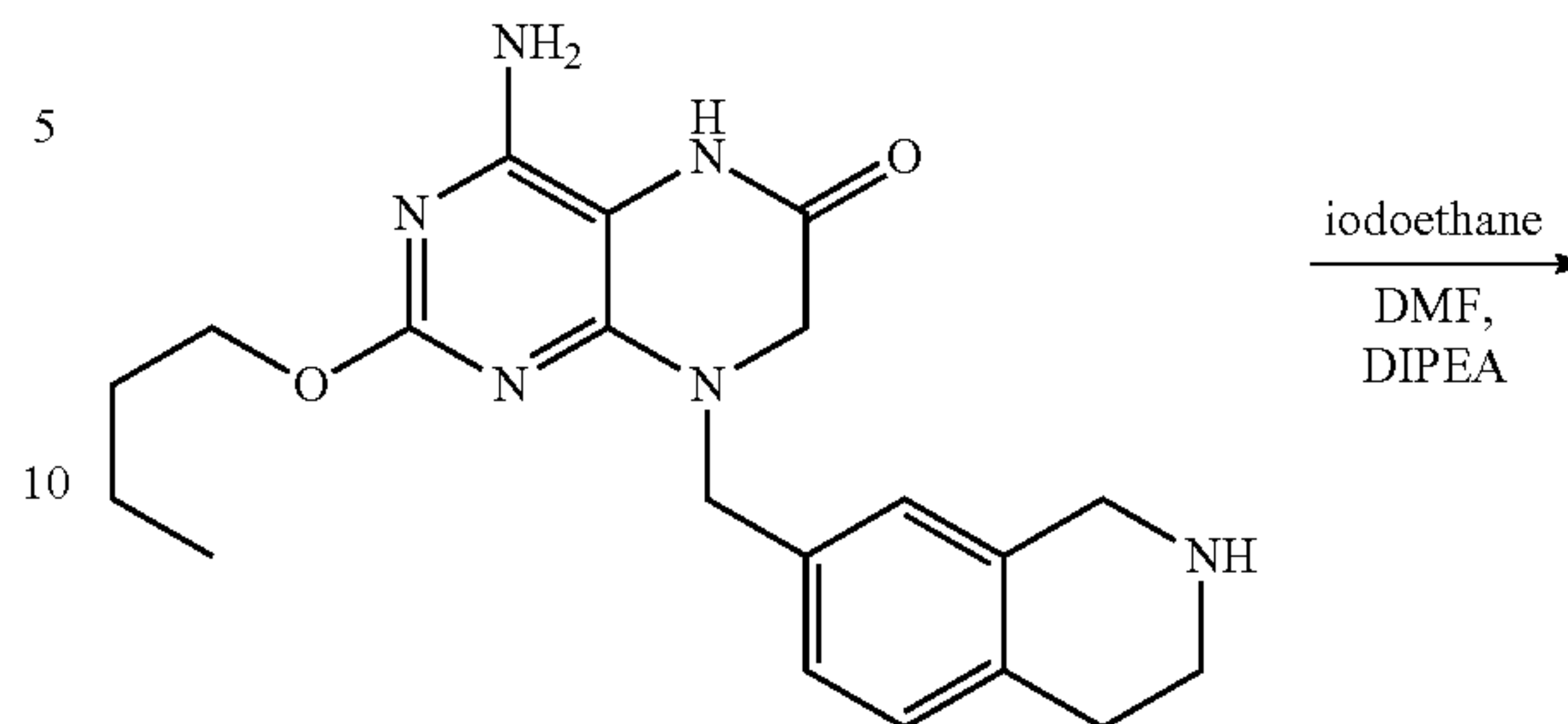
Example 51
