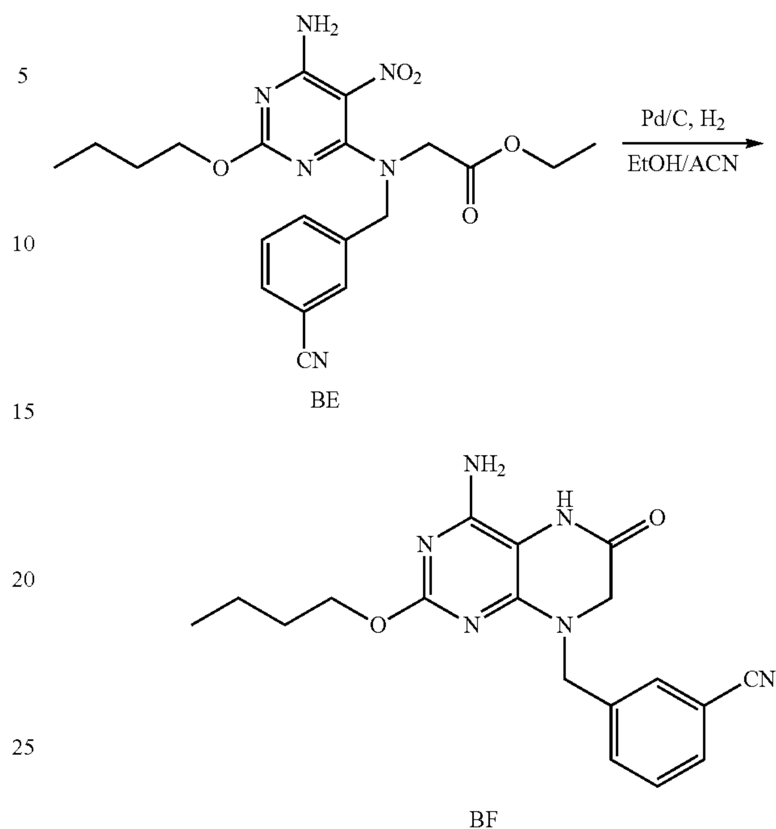
Scheme 23
