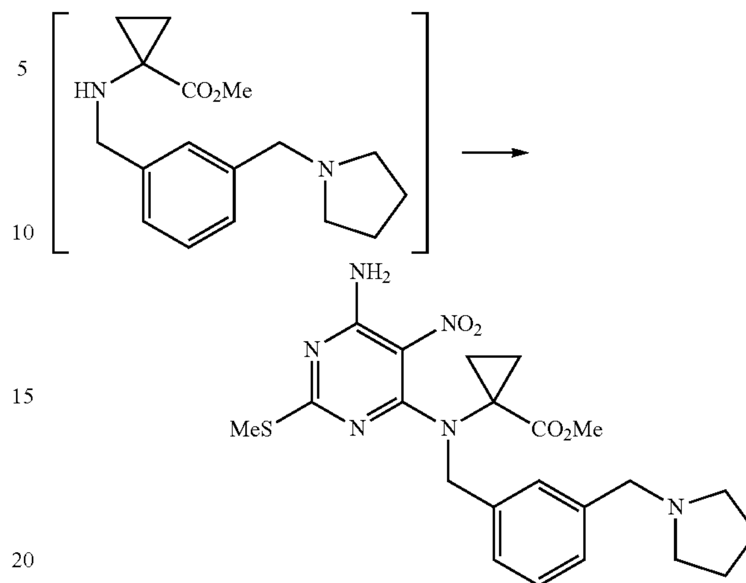
Scheme 19
