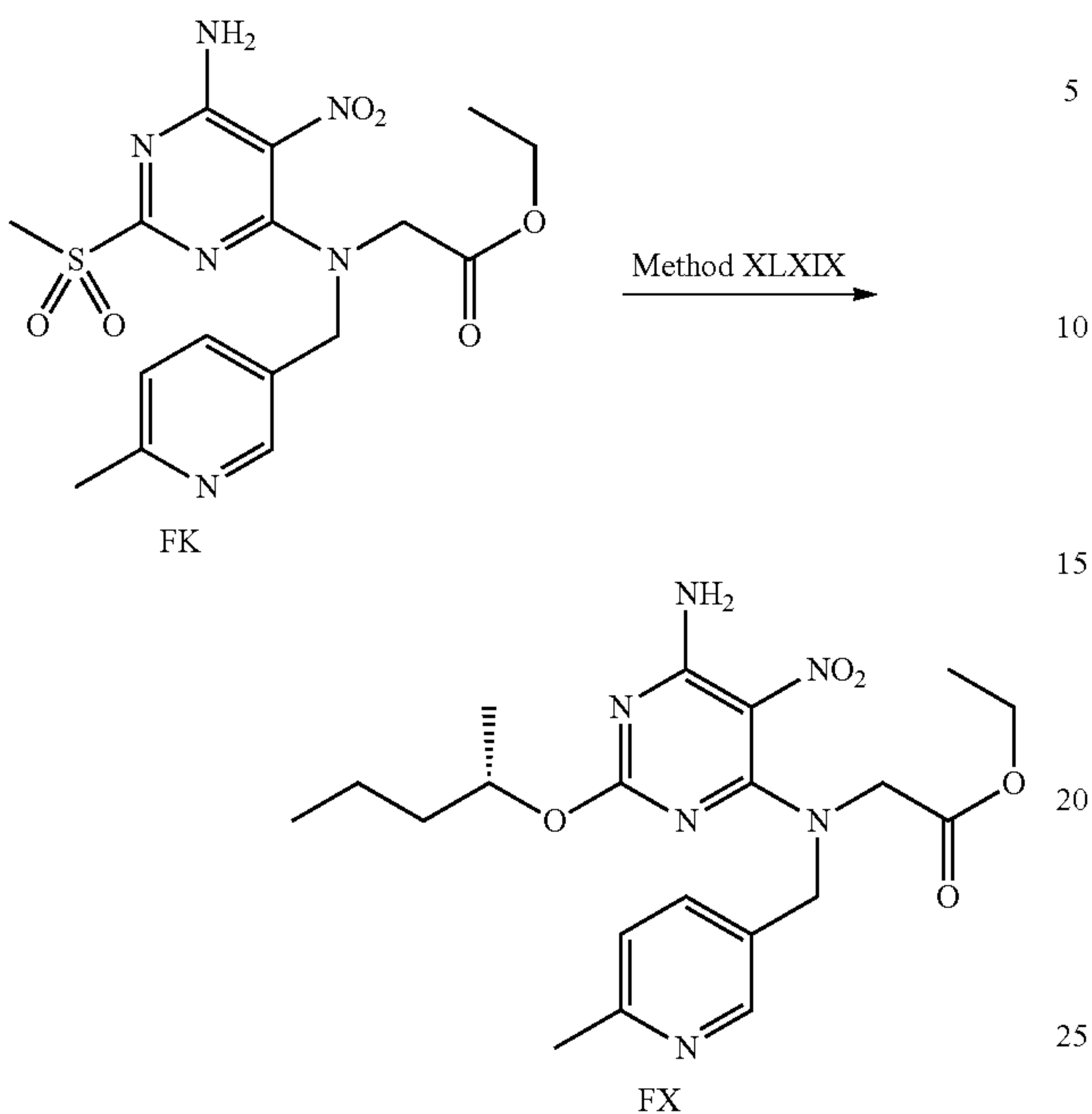
Scheme 116: Prepared Via Method XLXIX
