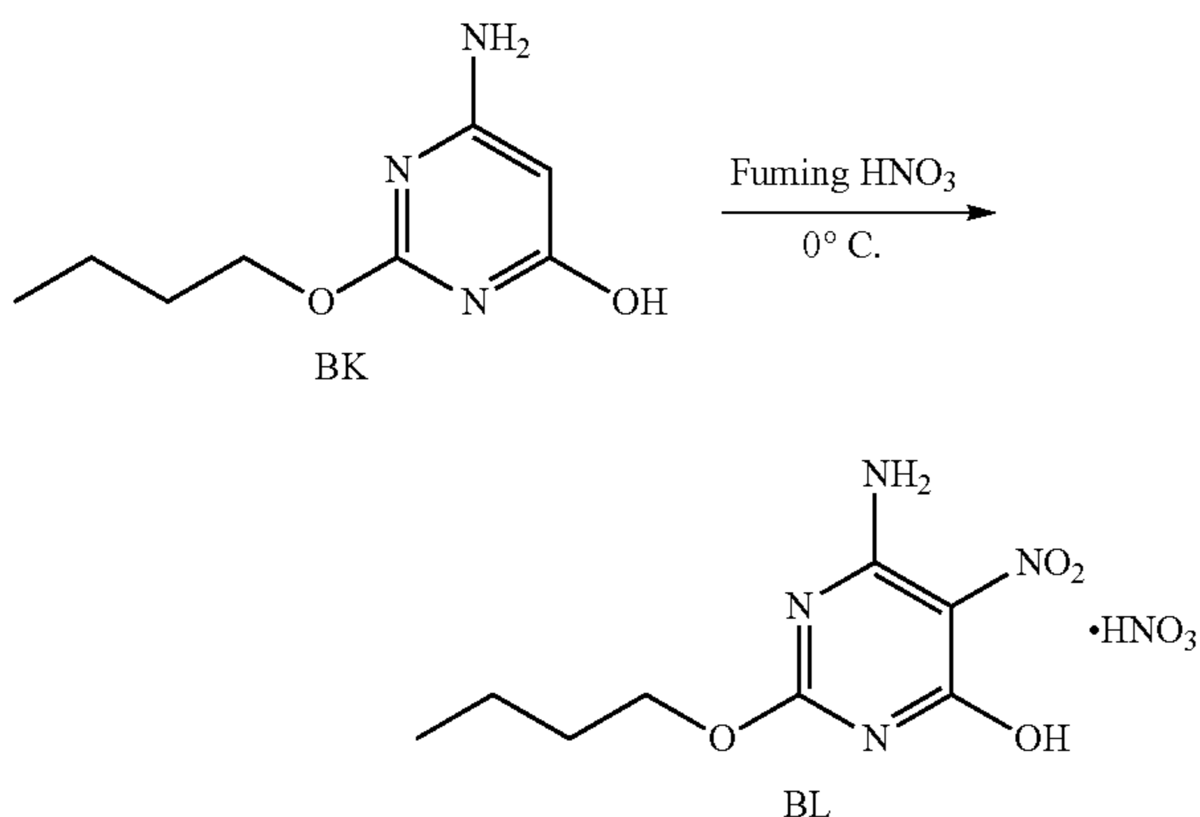
Scheme 30
