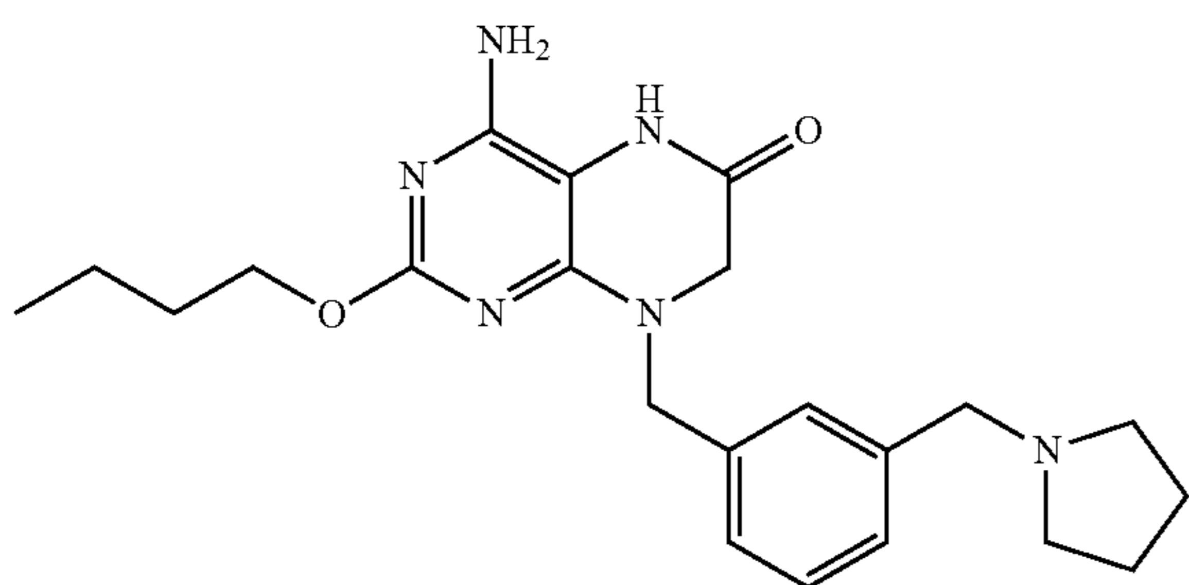
4-amino-2-n-butoxy-8-[3'-(pyrrolidin-1'-ylmethyl)-benzyl]-5,6,7,8-tetrahydropyrido-6-one
