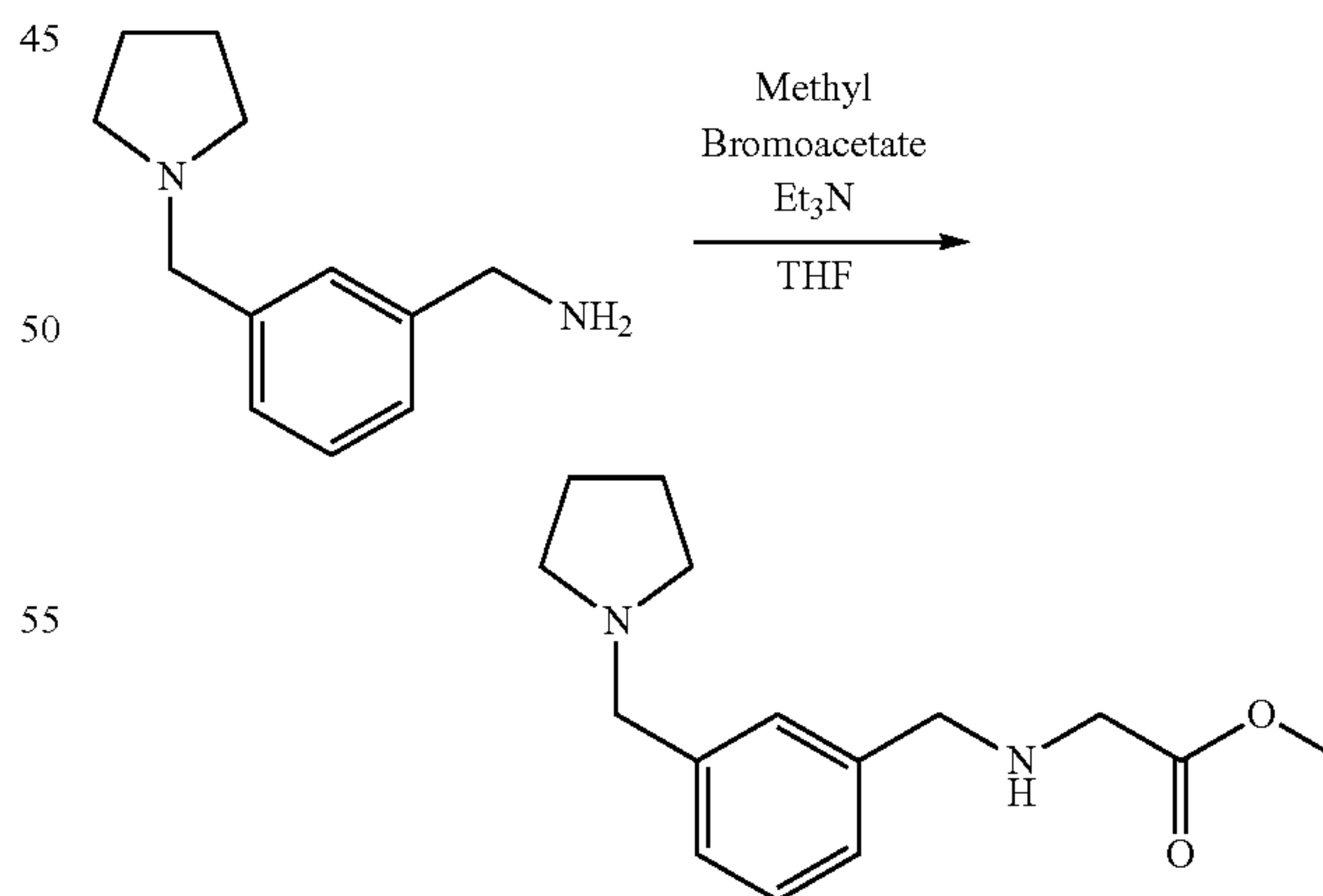
Scheme 20
