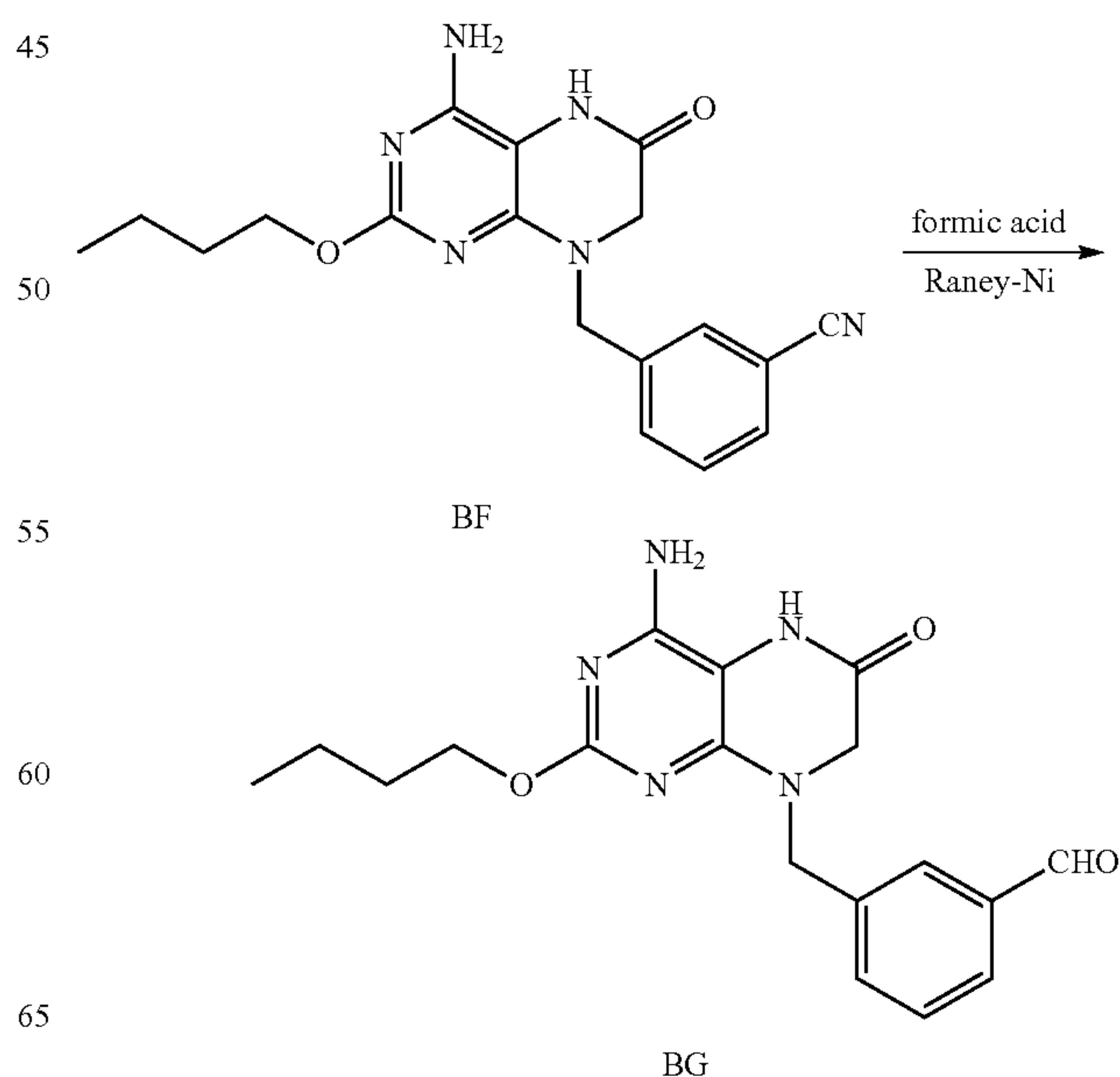
Scheme 24
