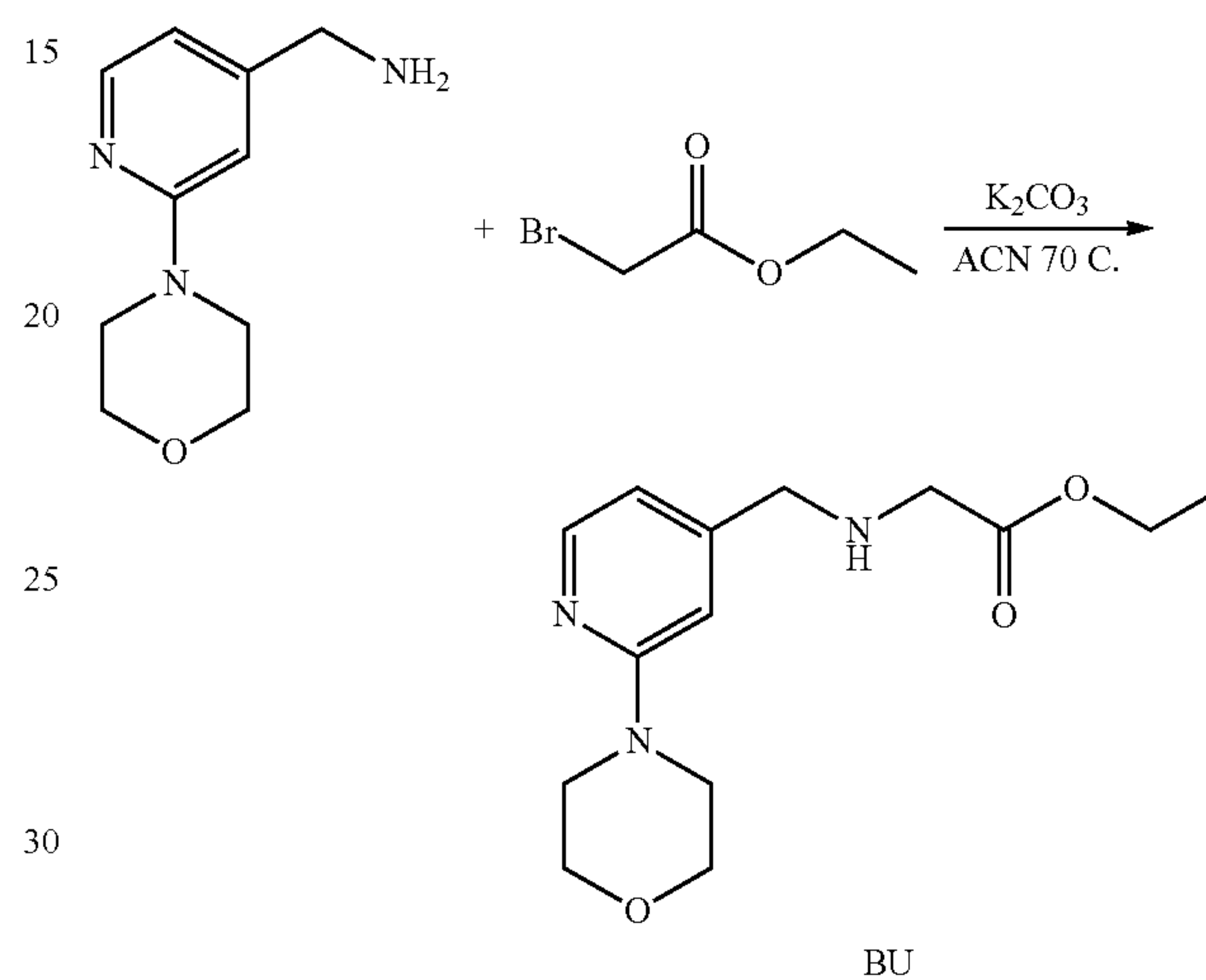
Scheme 42
