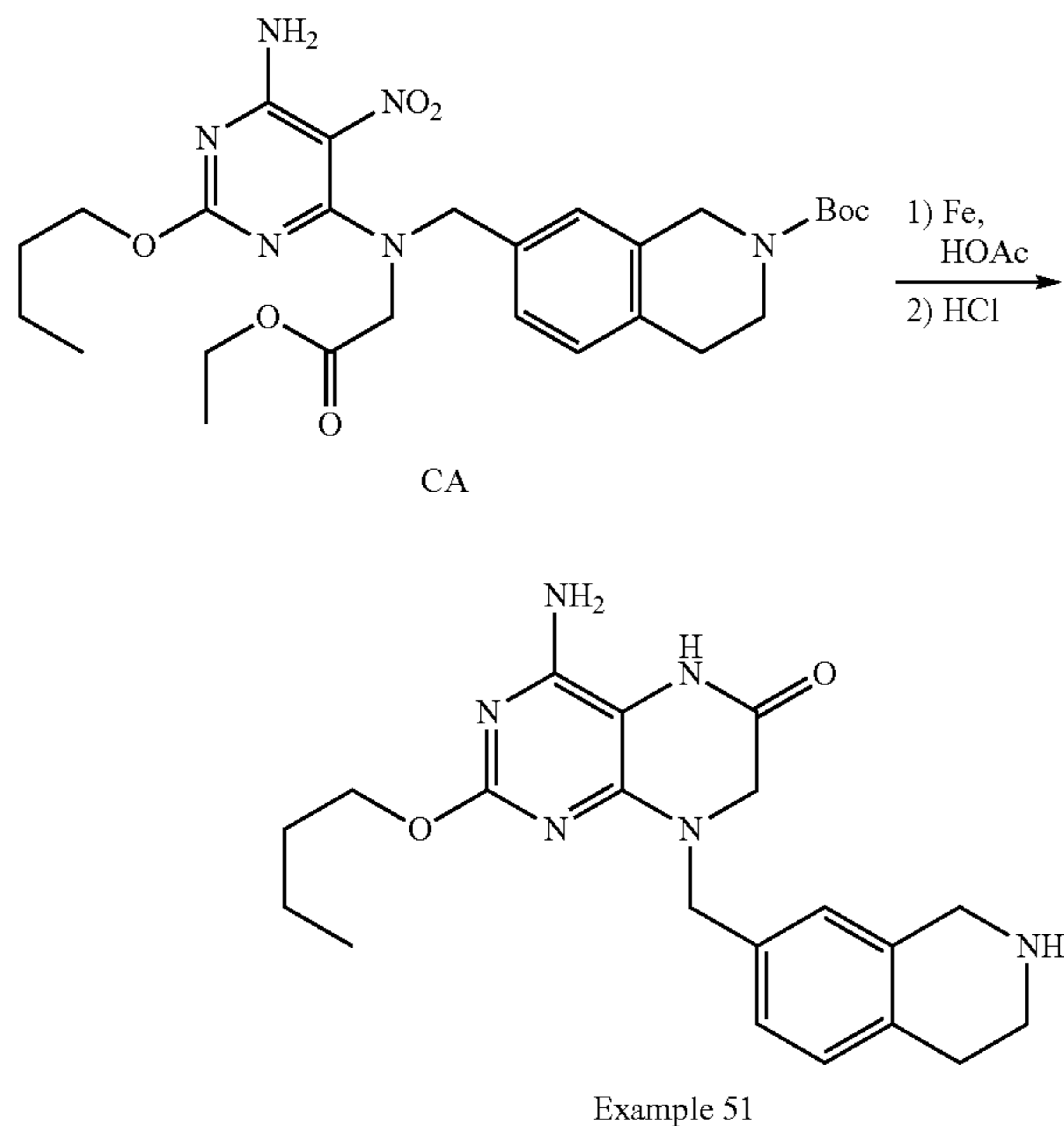
Scheme 47: Example 51
