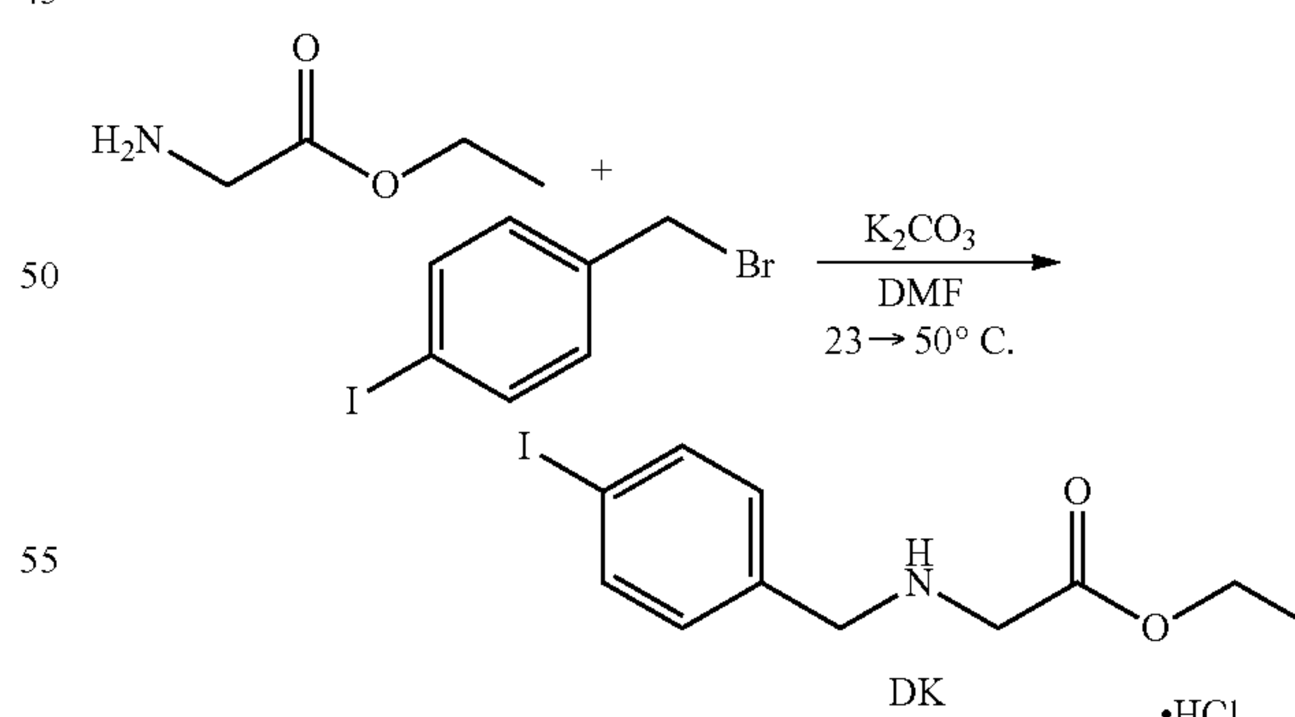
Scheme 77
