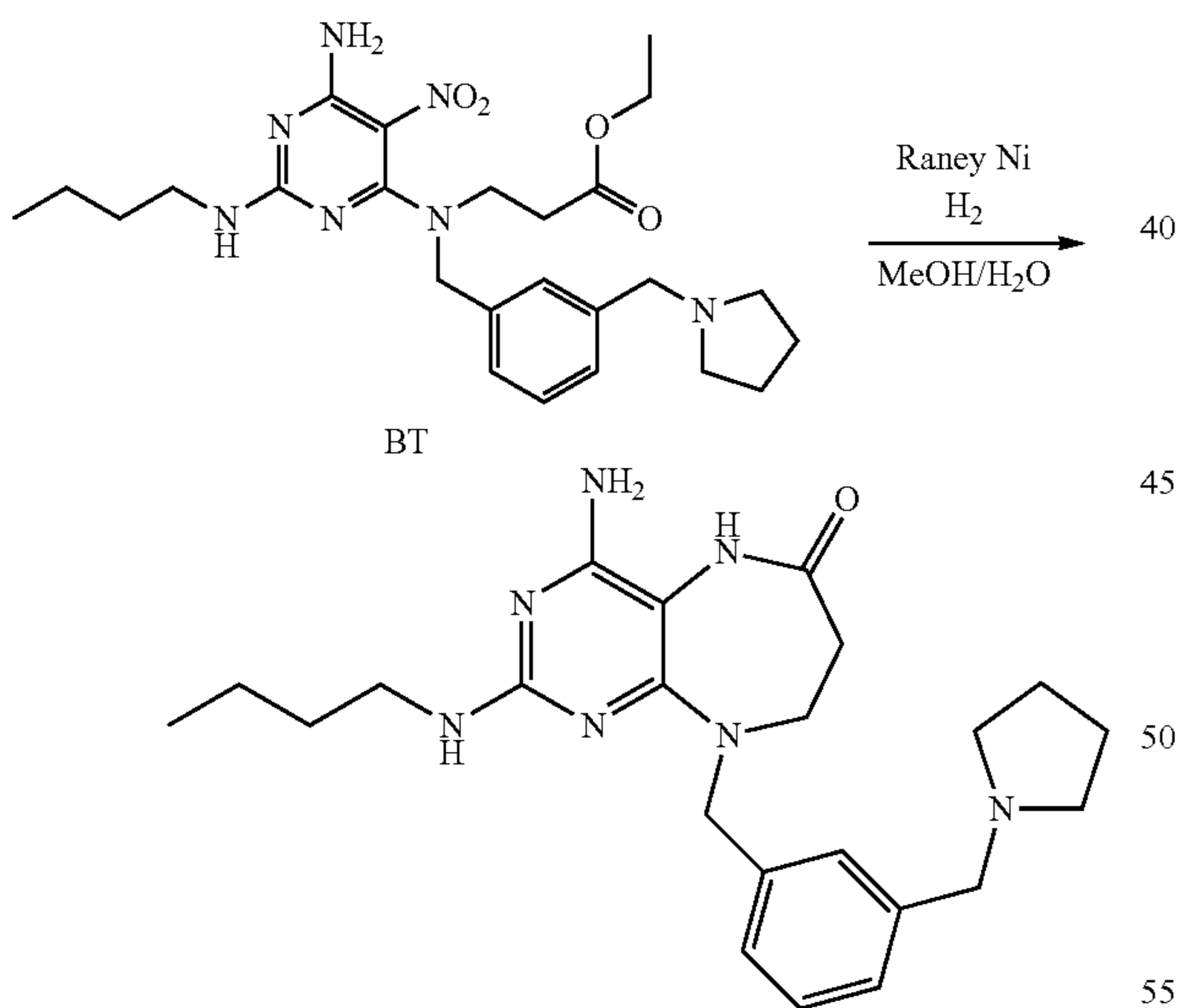
Example 76
