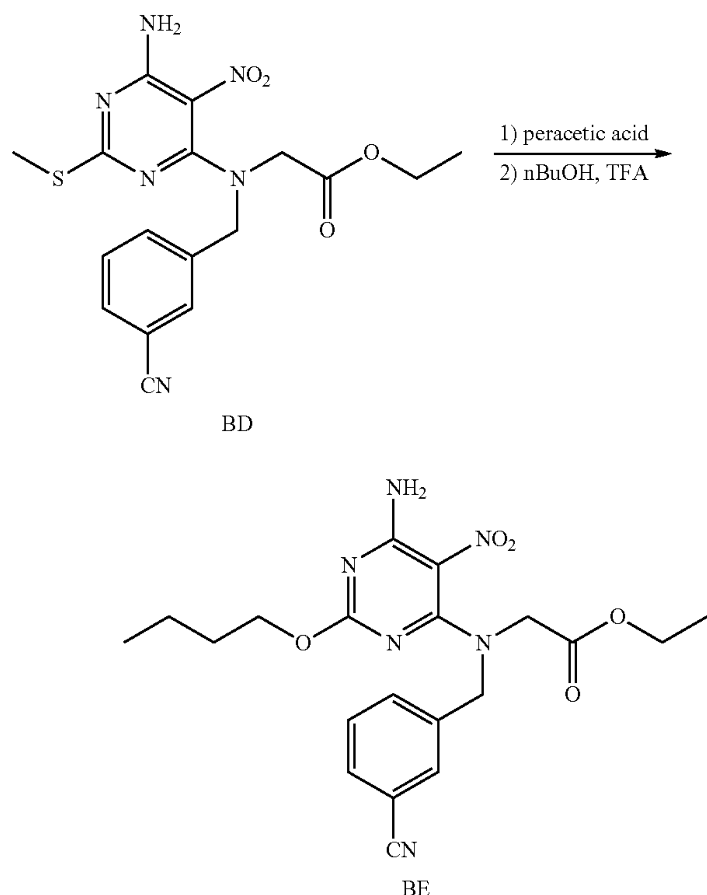
Scheme 22
