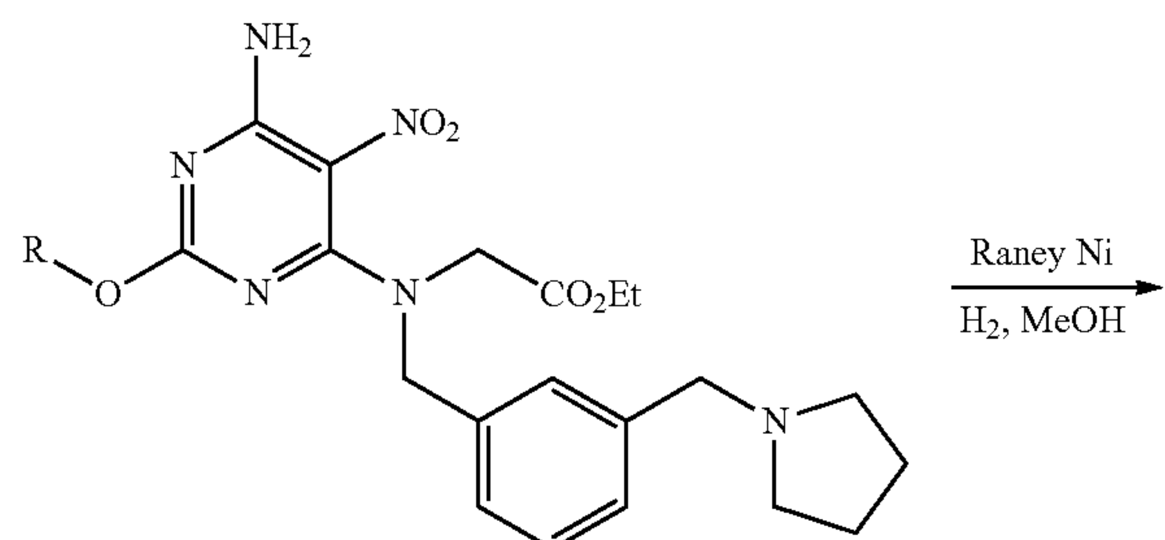
Scheme 15
