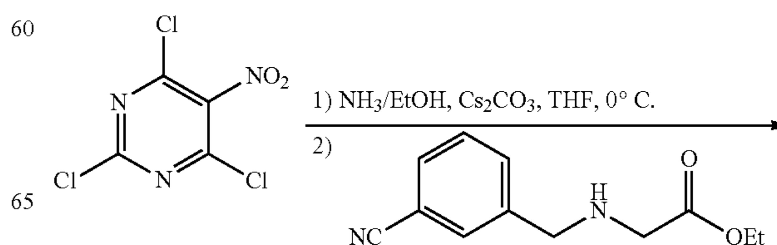
Scheme 49
