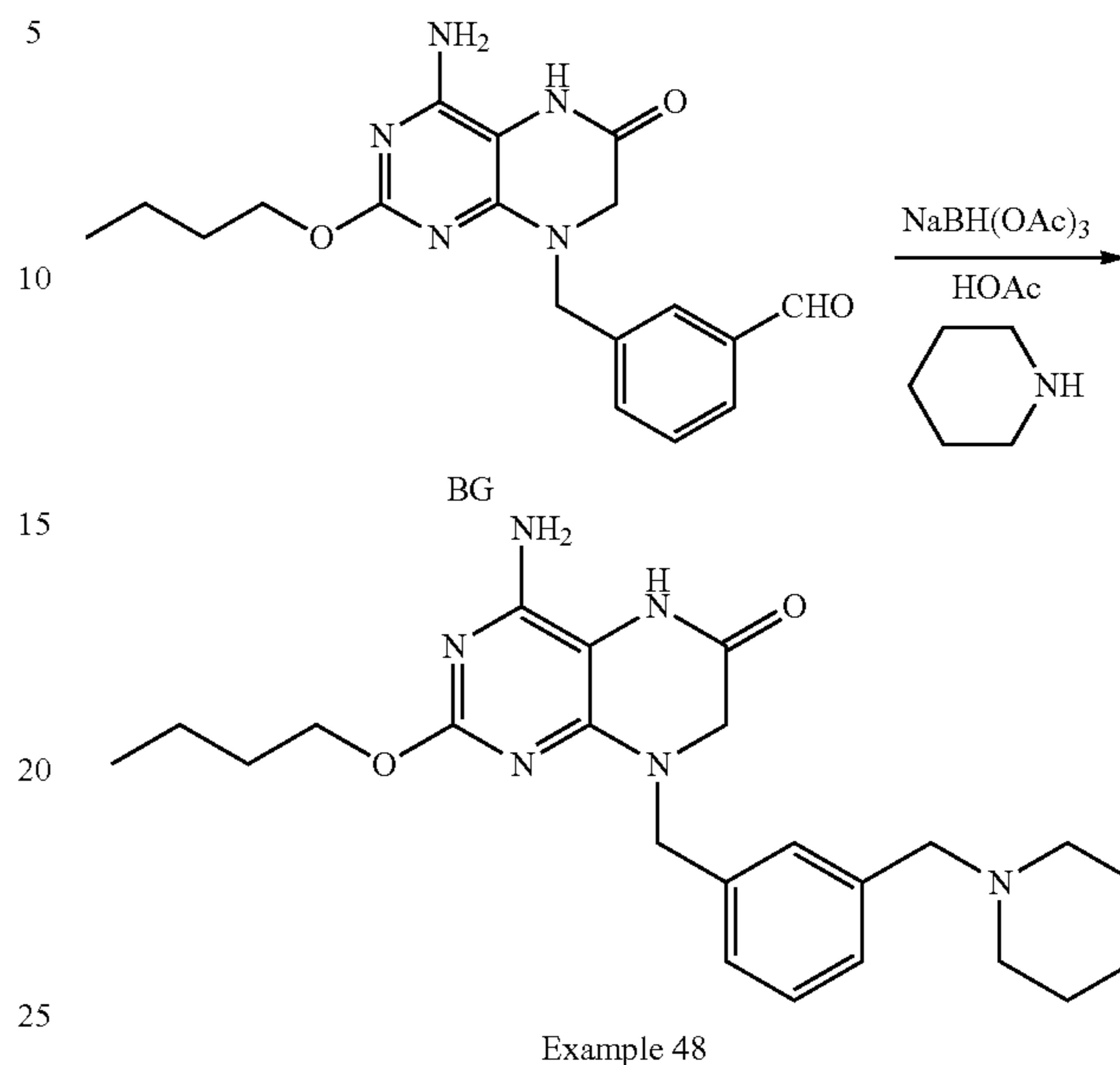
Scheme 26
