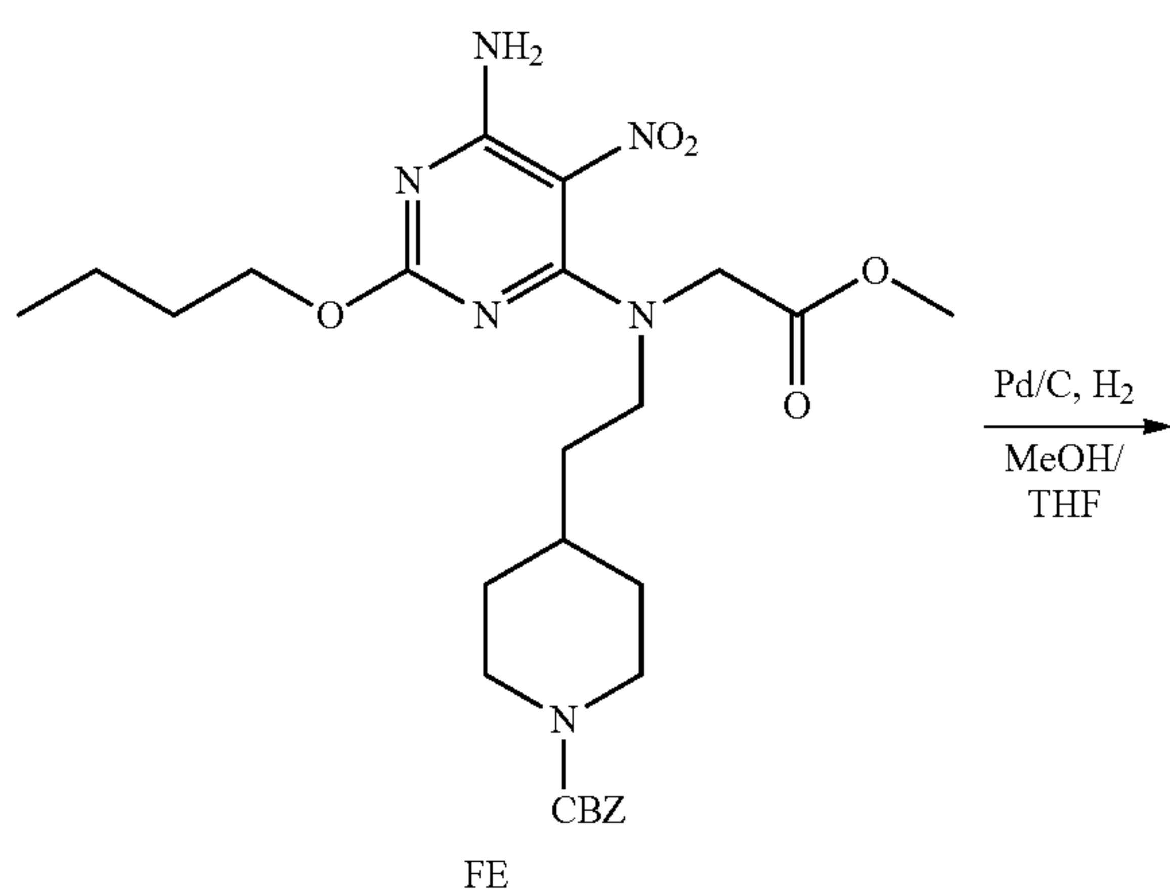
Scheme 94
