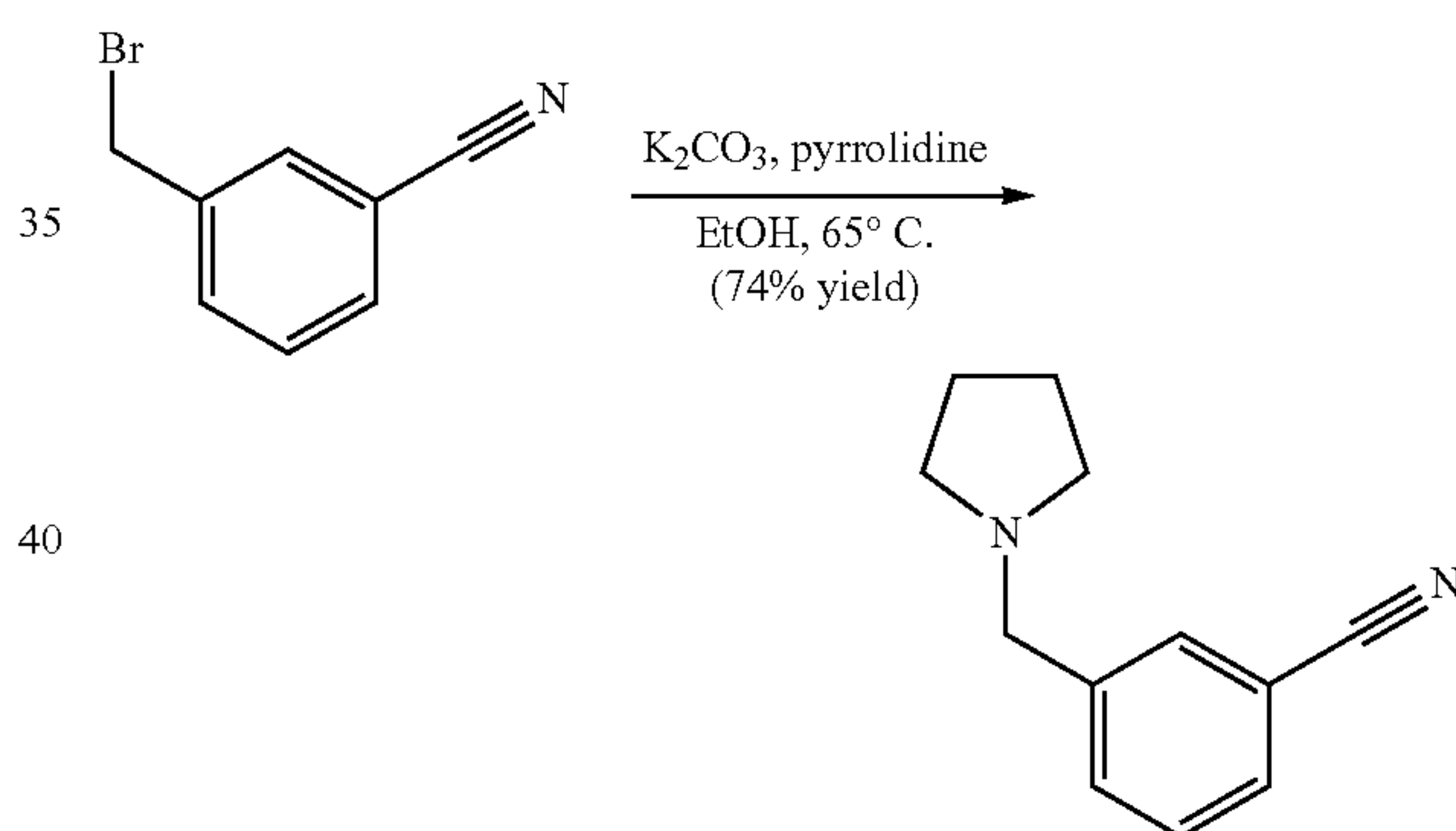
Scheme 3
