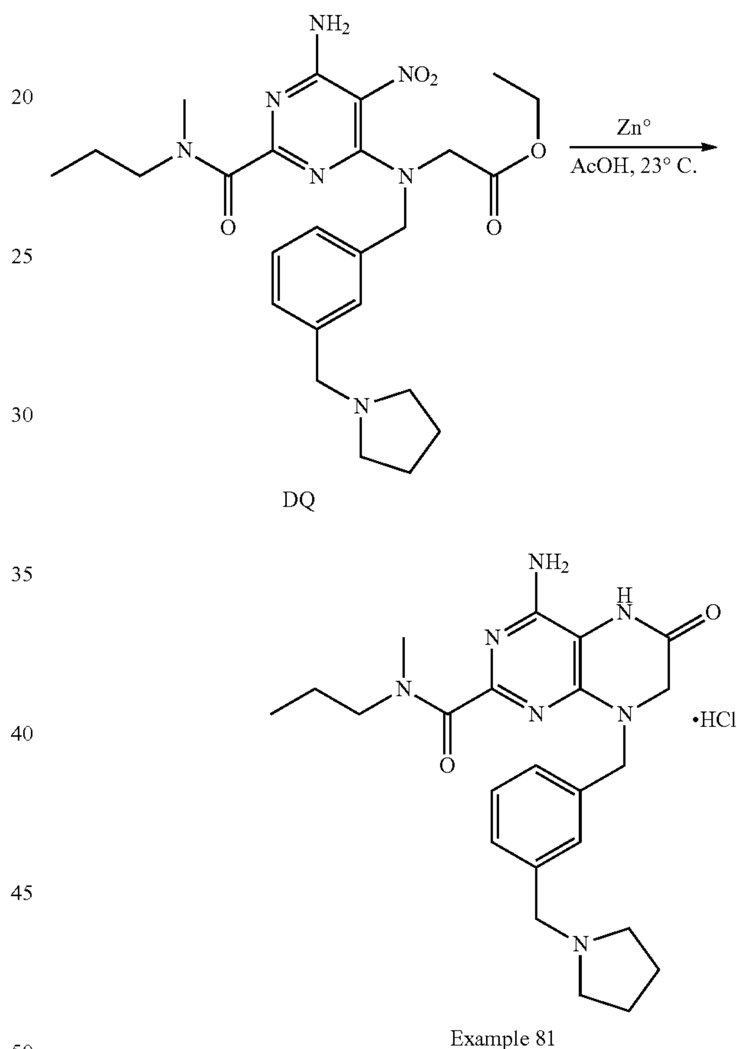
Scheme 84: Example 81
