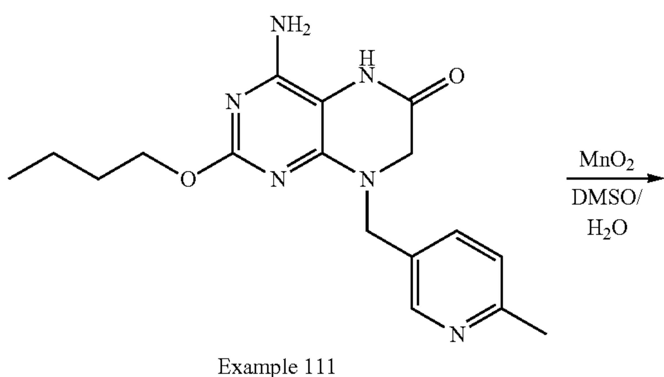
Scheme 111
