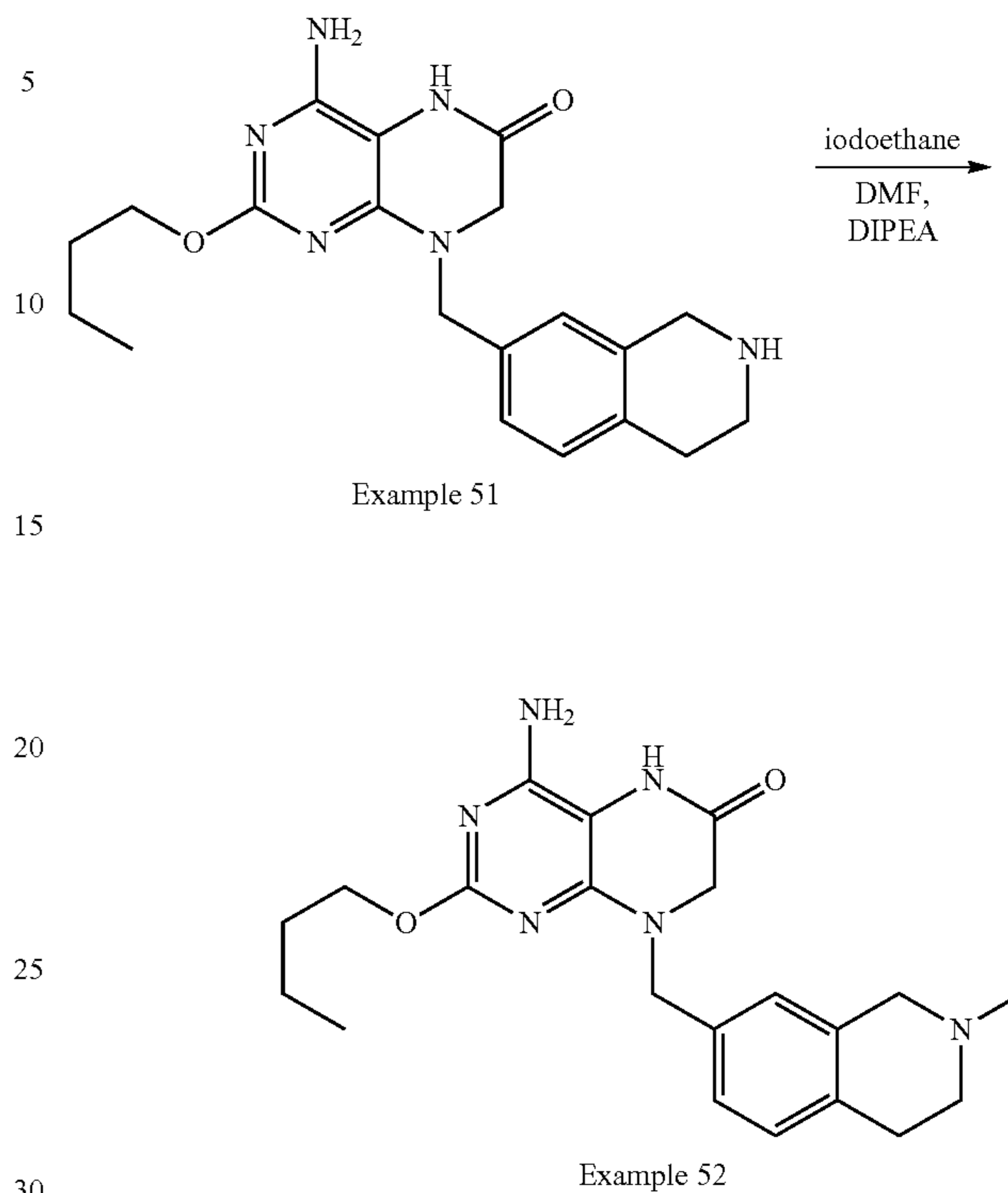
Scheme 48: Example 52
