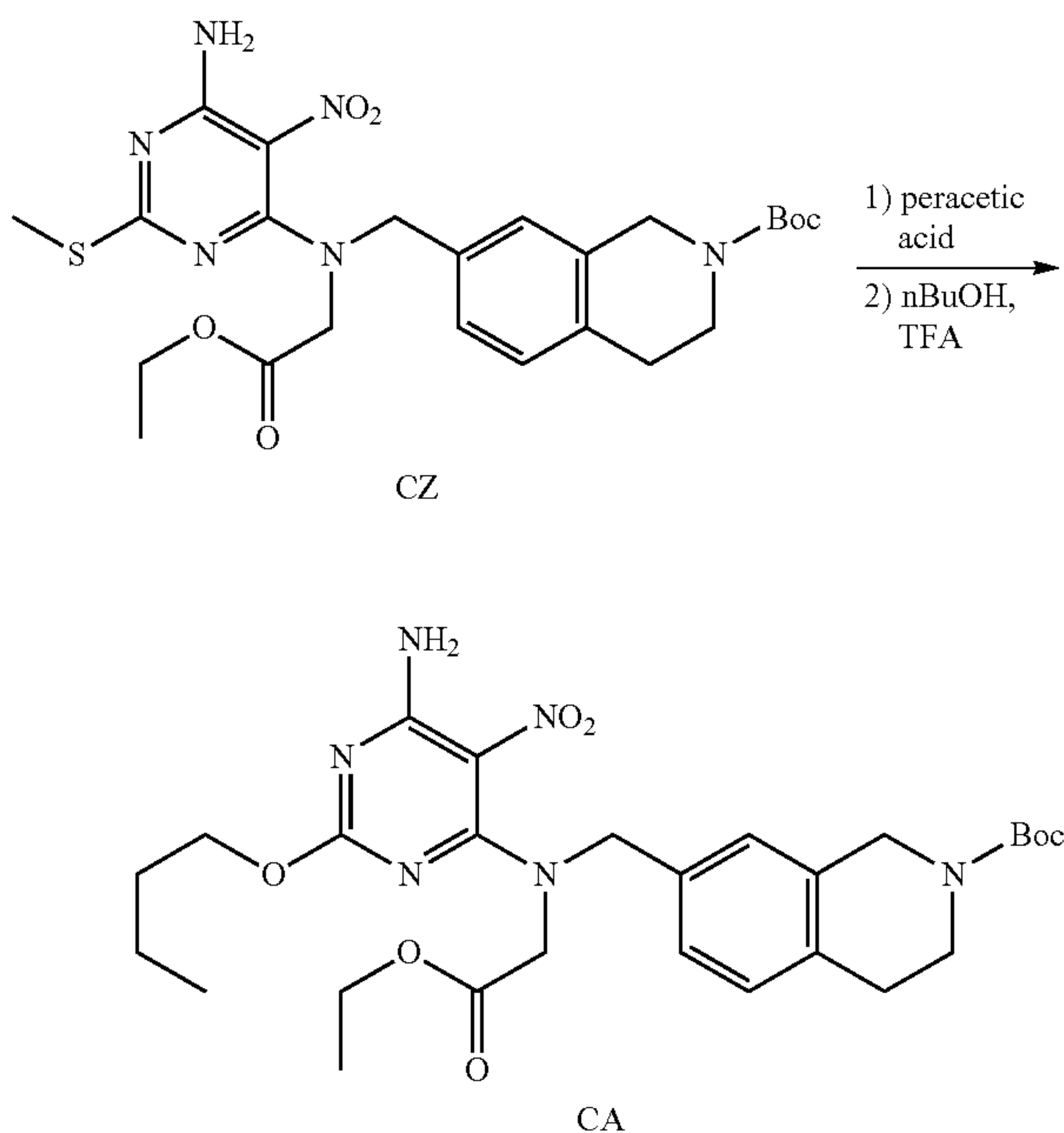
Scheme 60: Compound CA Prepared Via Method XVIII:
