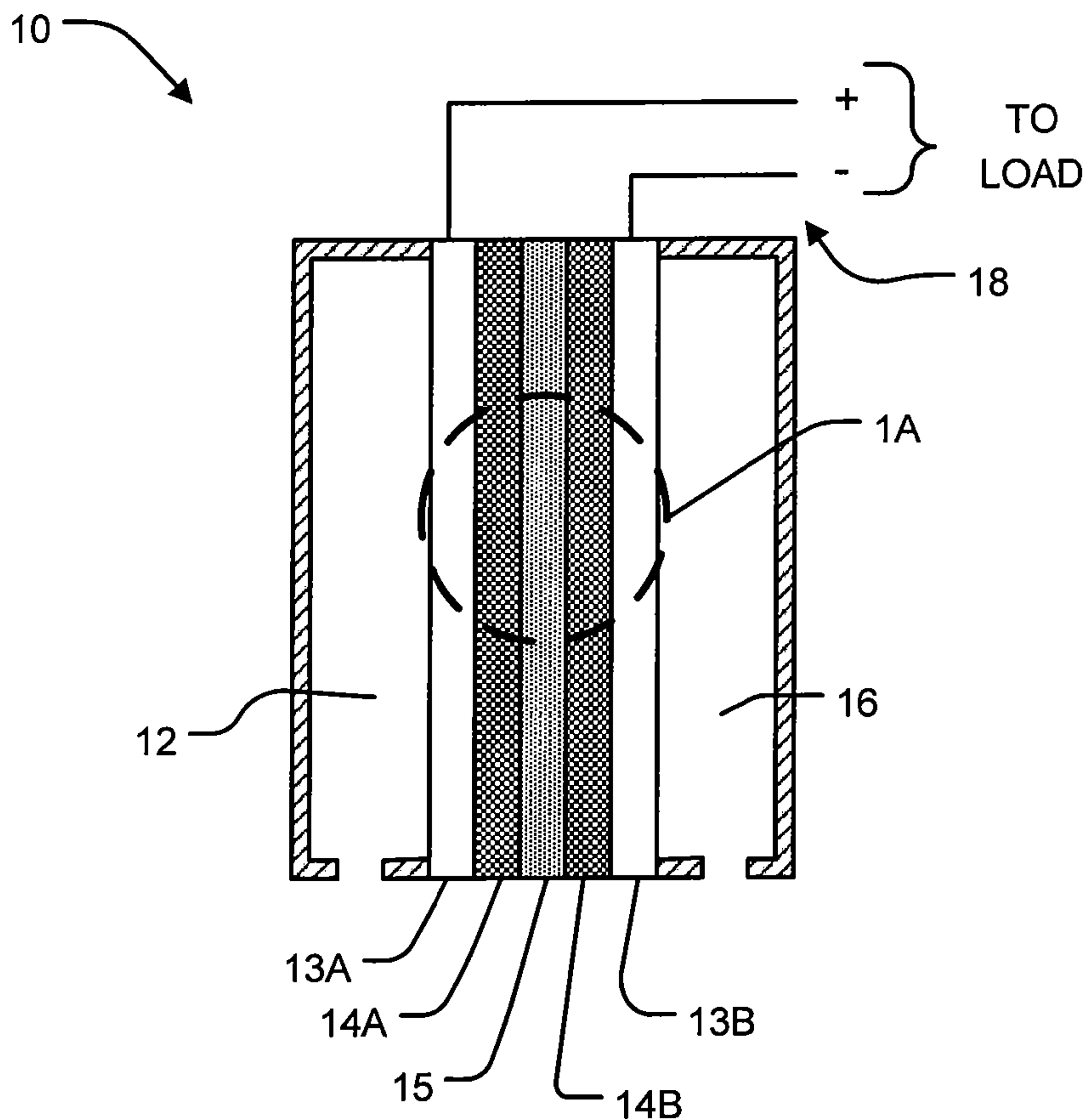
FIGURE 1 (Prior Art)
