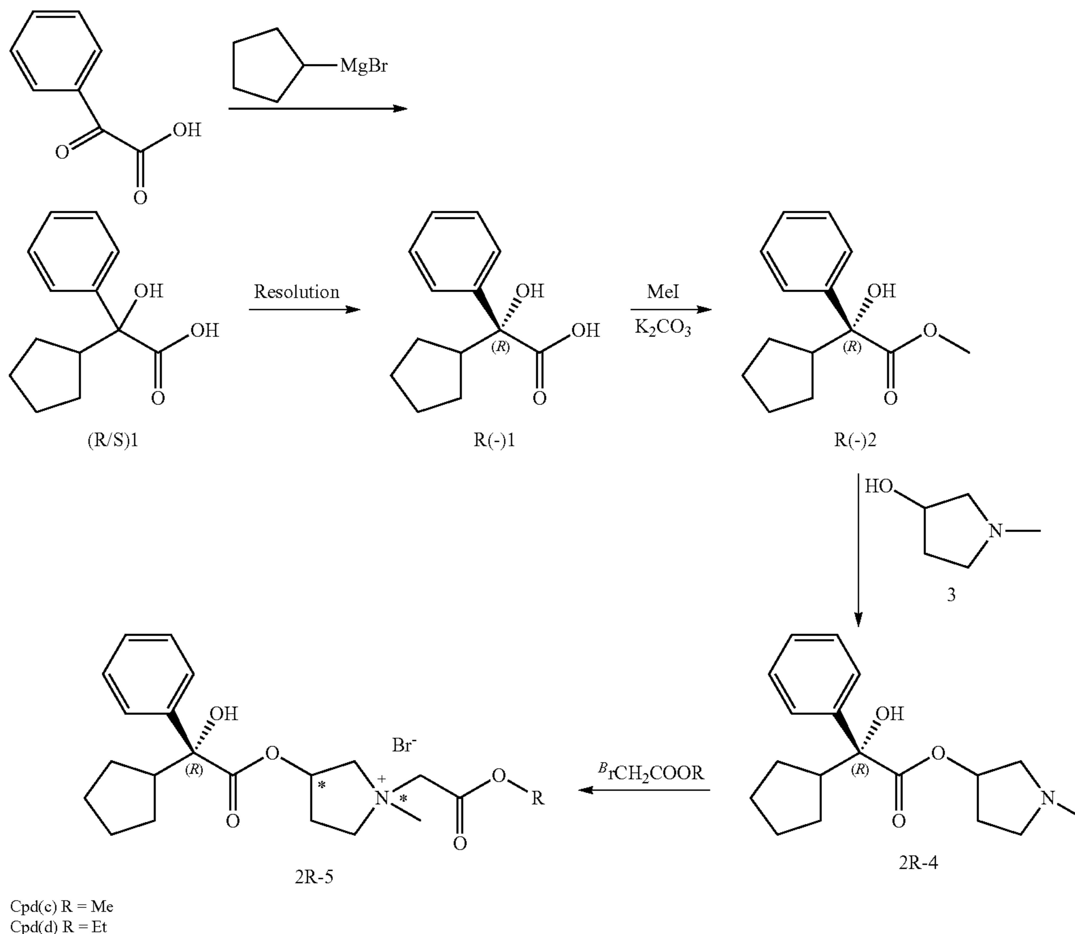
Scheme 1
