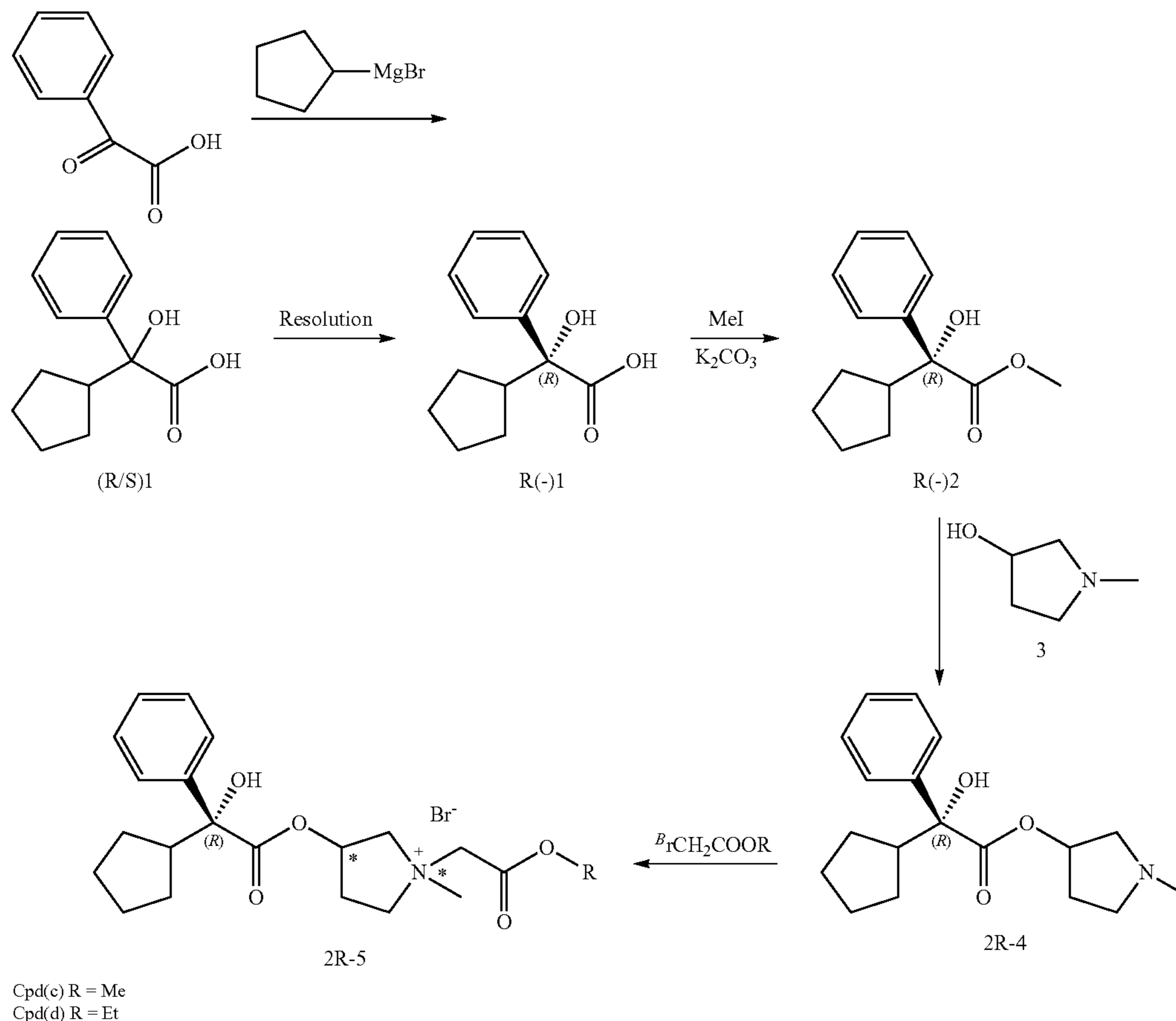
Scheme 1
