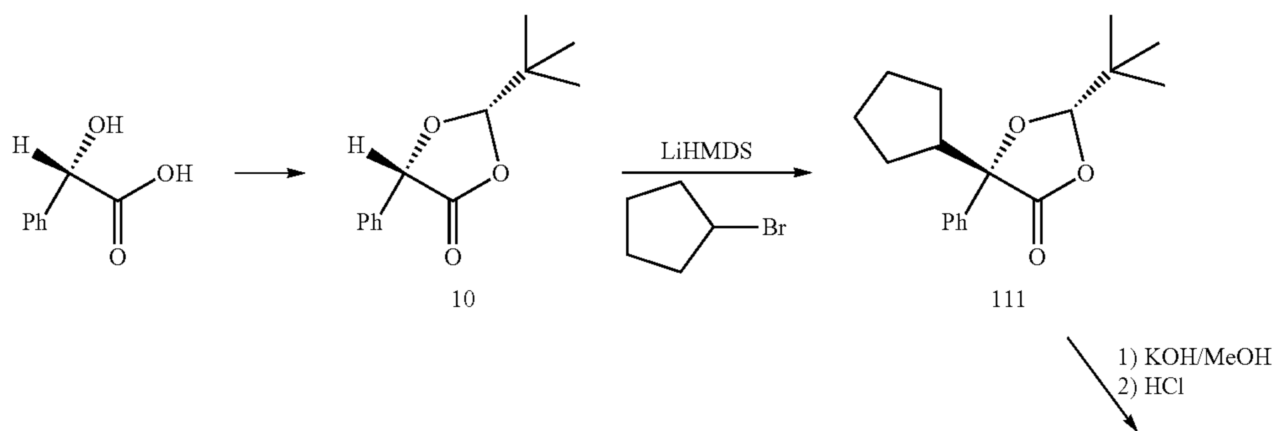
Scheme 3
