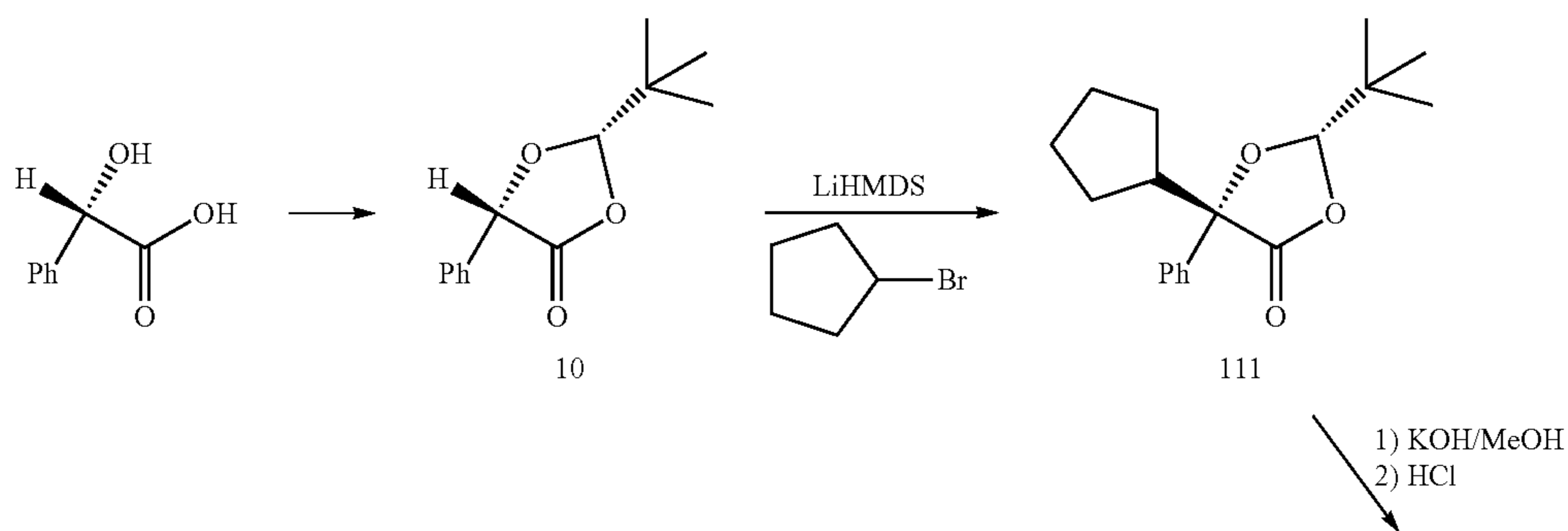
Scheme 3
