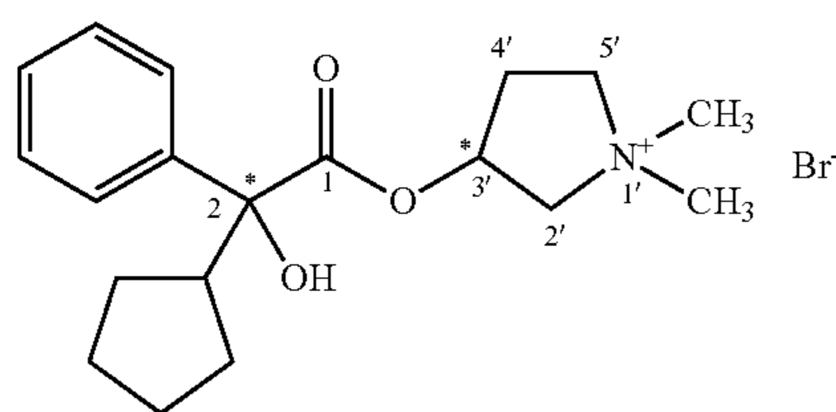
Glycopyrrolate
