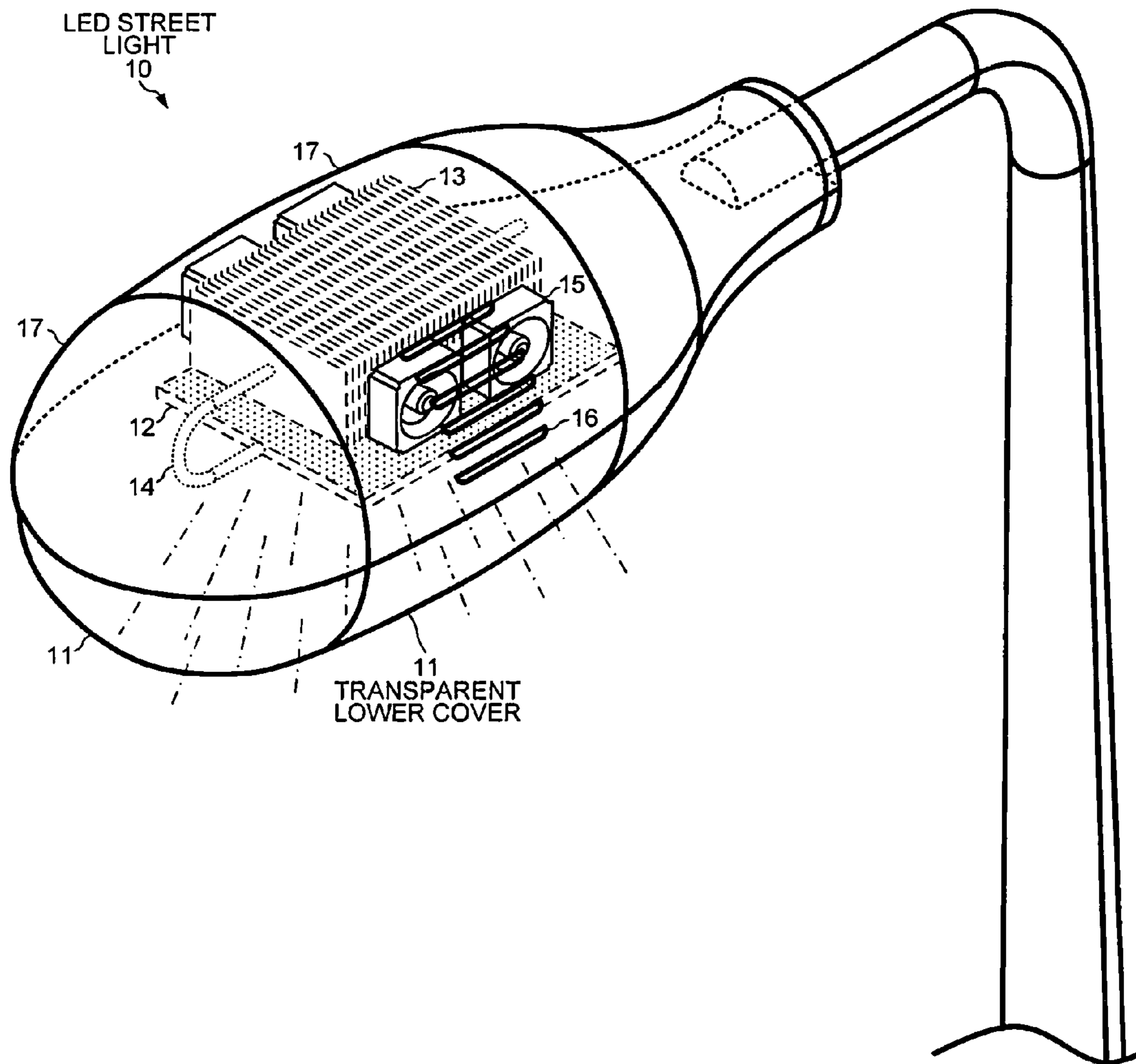
FIG. 1 (PRIOR ART)
