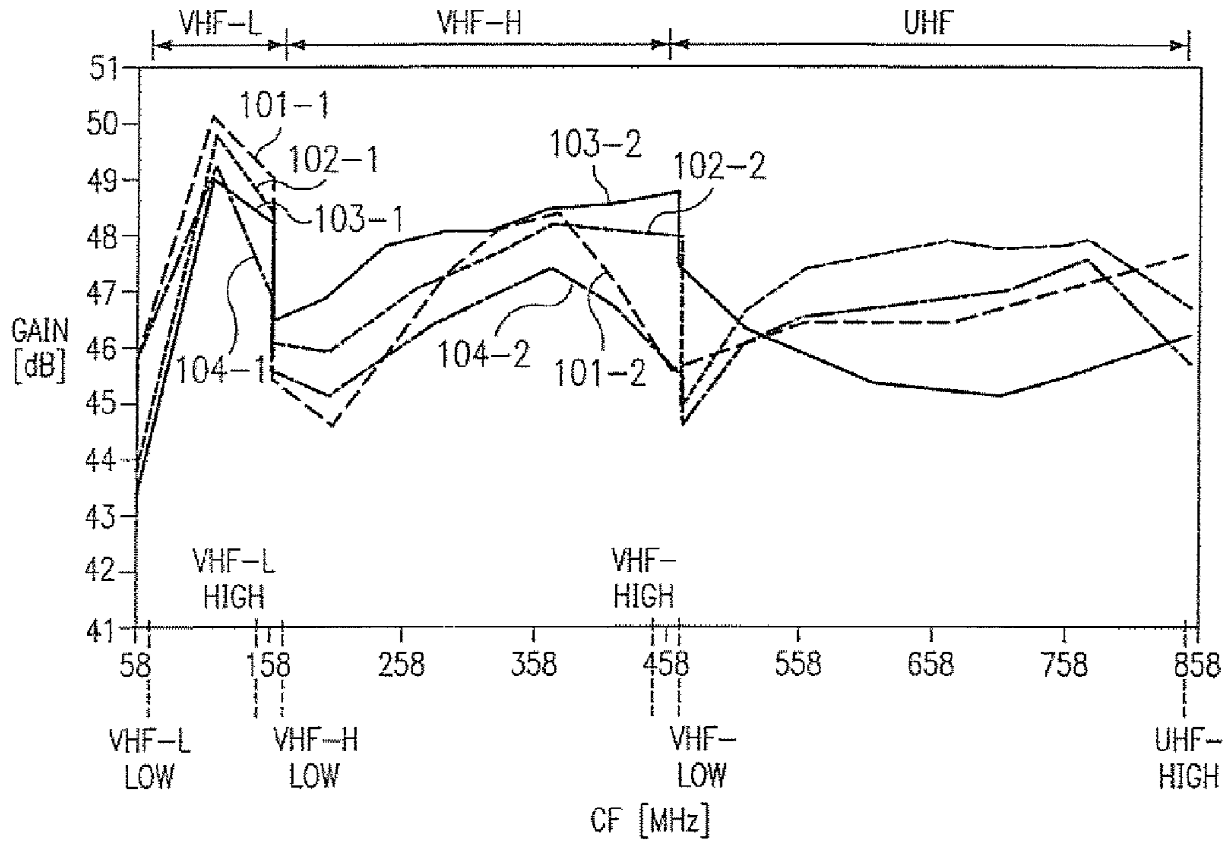
FIG. 1 (PRIOR ART)
