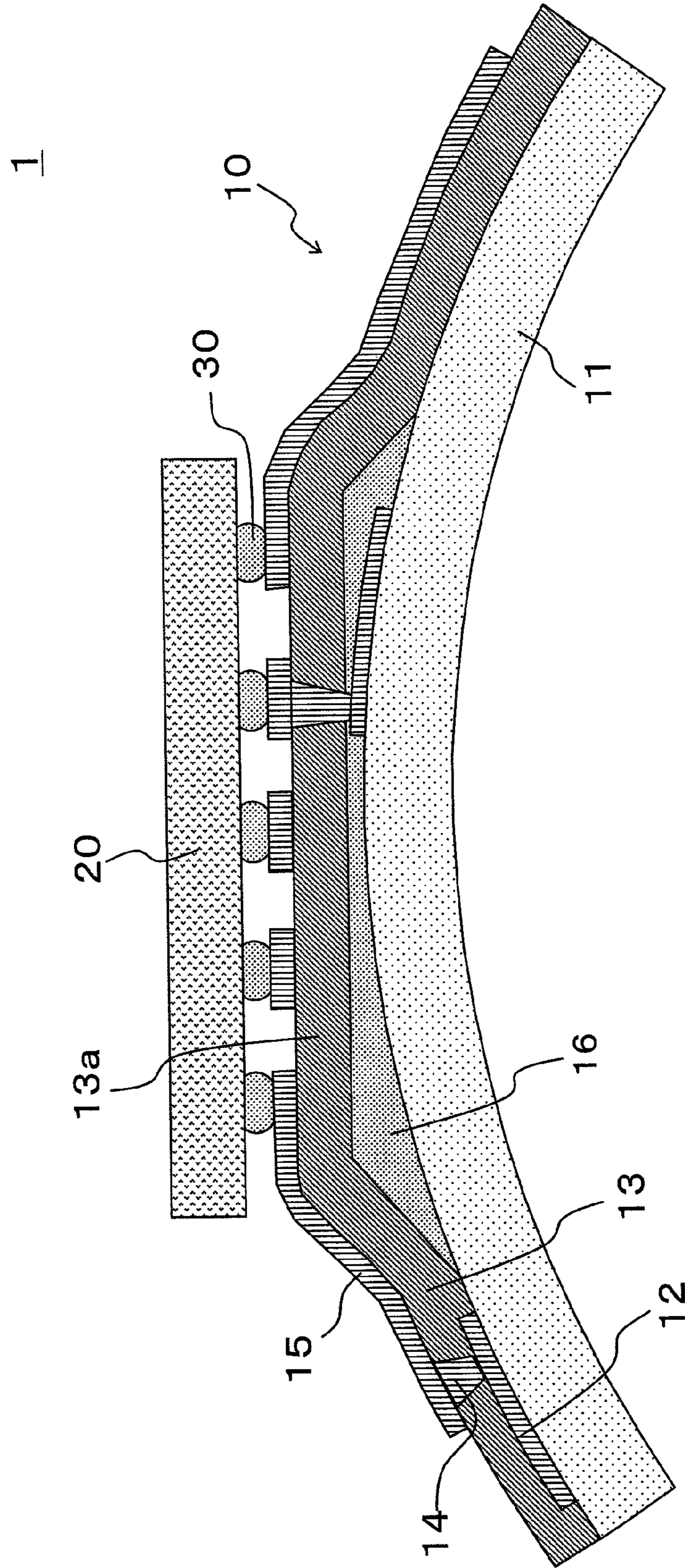
FIG.11 (FOURTH EXEMPLARY EMBODIMENT)
