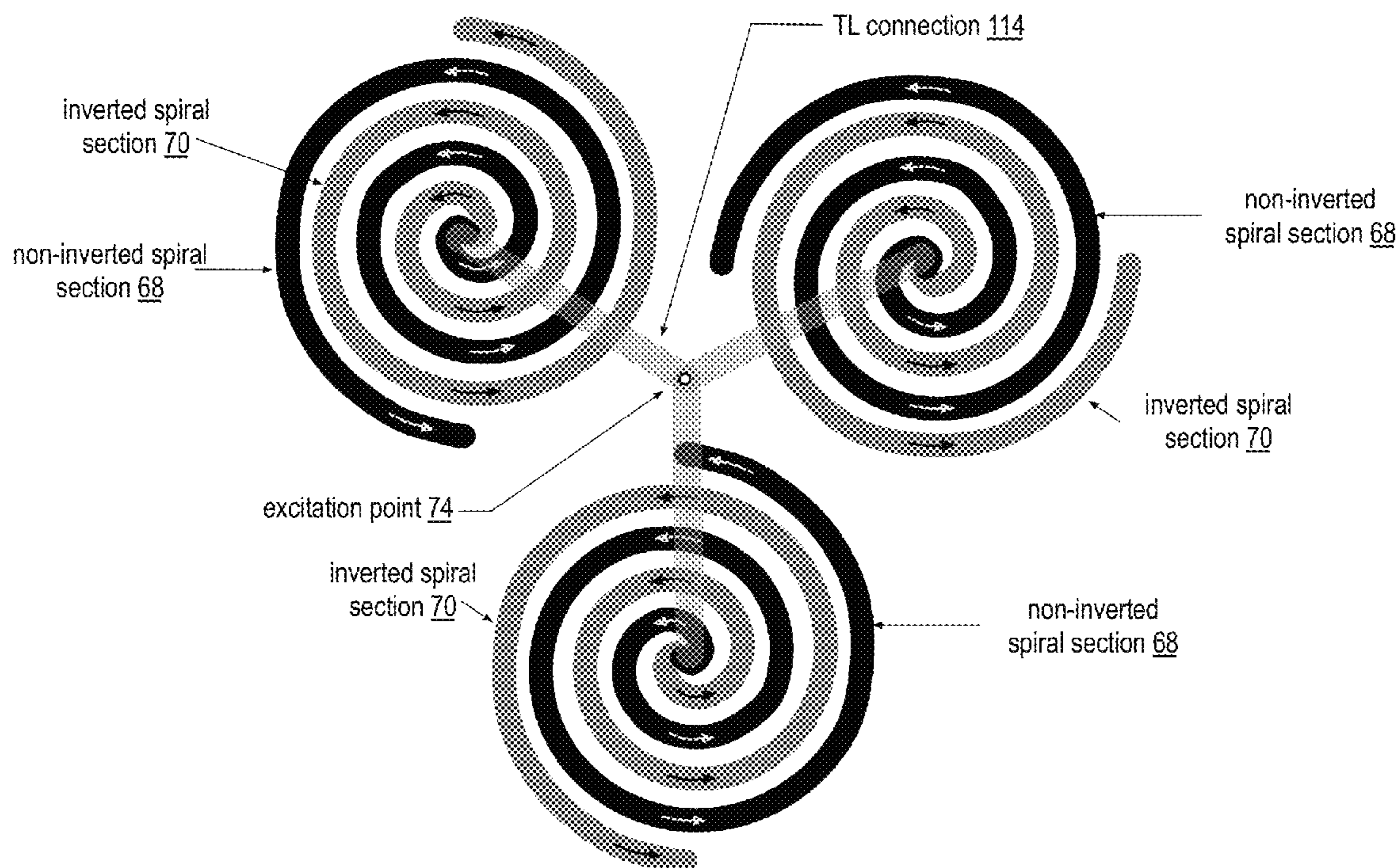
multiple two-arm spiral antenna 112
