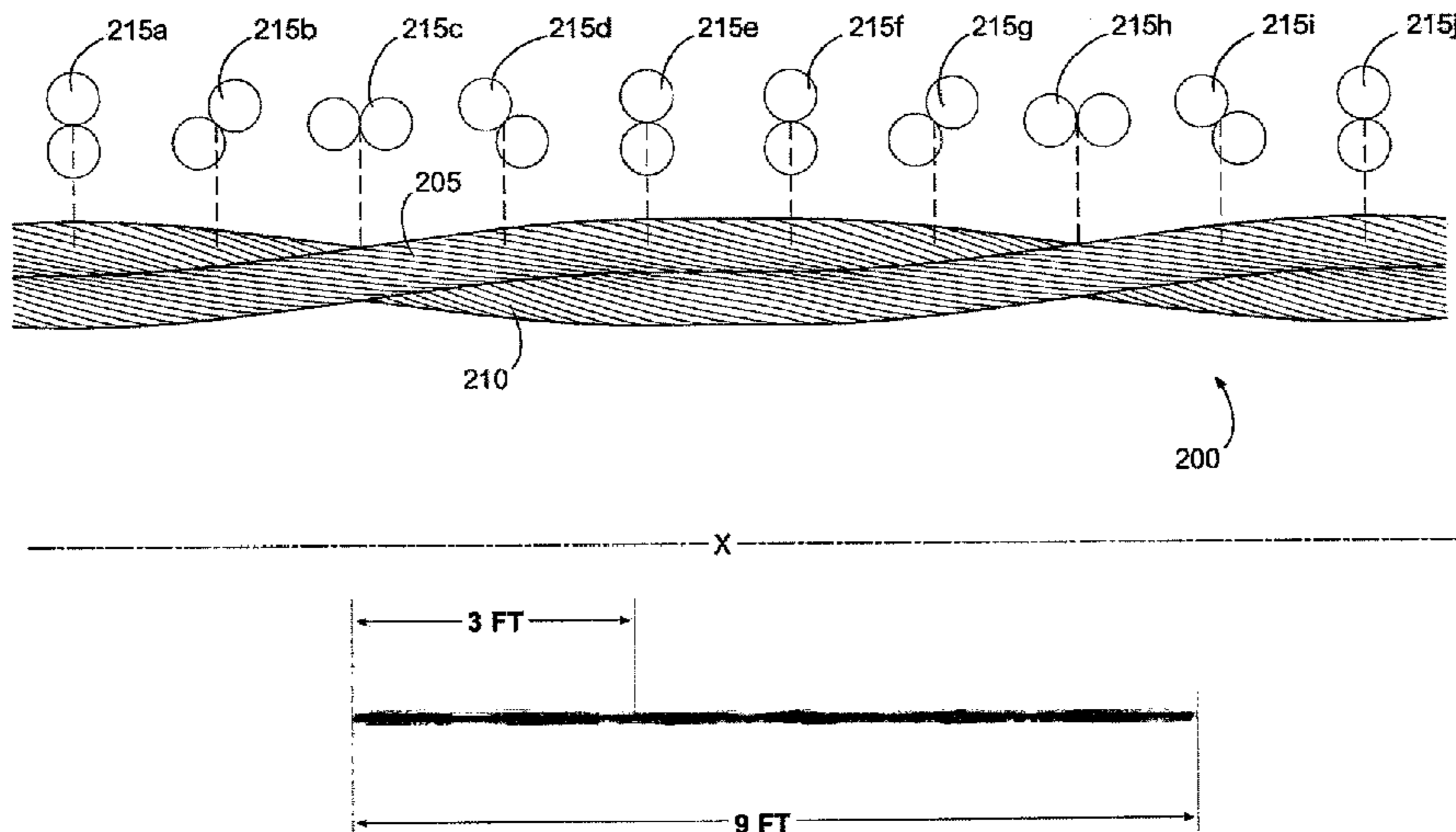
3 FT LAY CABLE
