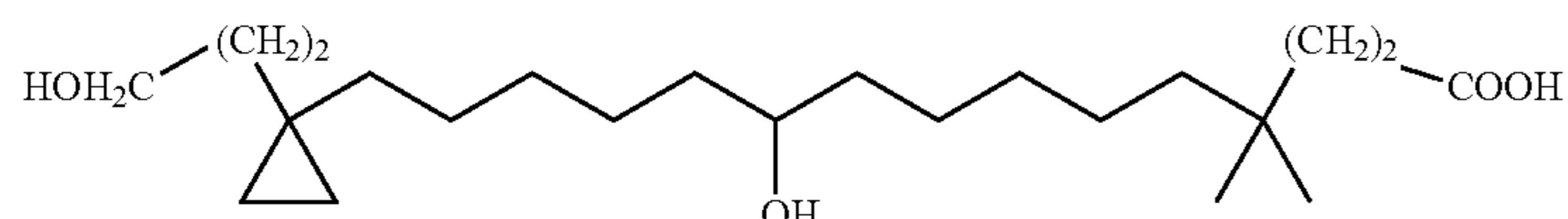
4,4-Dimethyl-10-hydroxy-15-[1-(3-hydroxy-propyl)-cyclopropyl]-pentadecanoic acid
