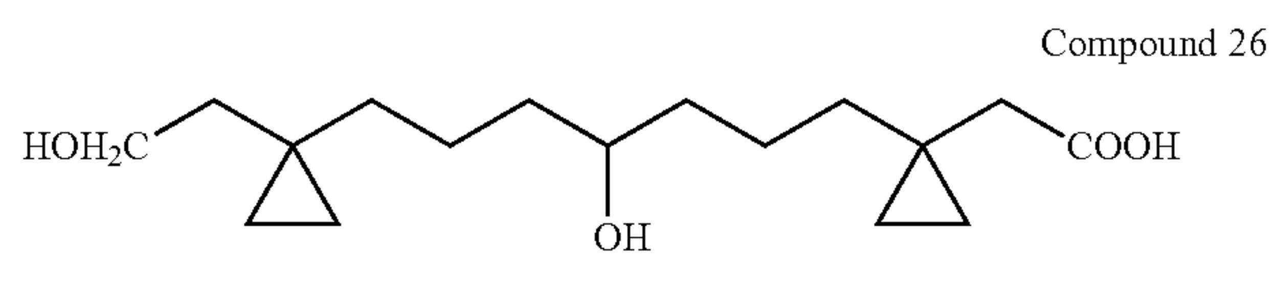
(1-{4-Hydroxy-7-[1-(2-hydroxy-ethyl)-cyclopropyl]-heptyl}-cyclopropyl)-acetic acid
