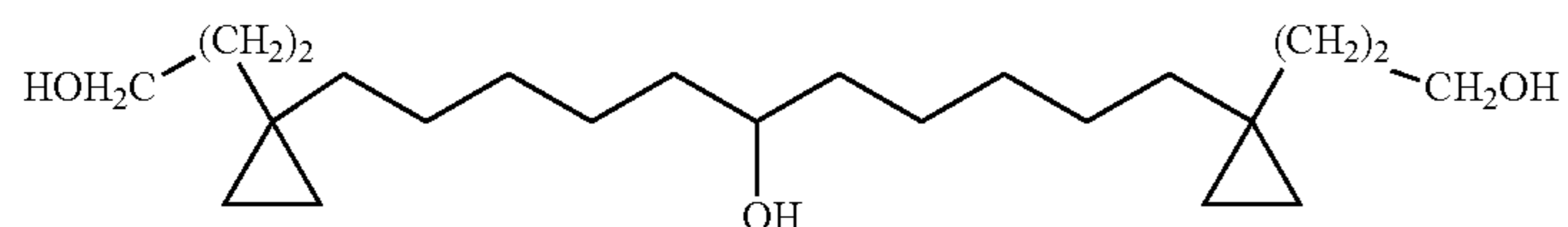
1,11-Bis-[1-(3-hydroxy-propyl)-cyclopropyl]-undecan-6-ol
