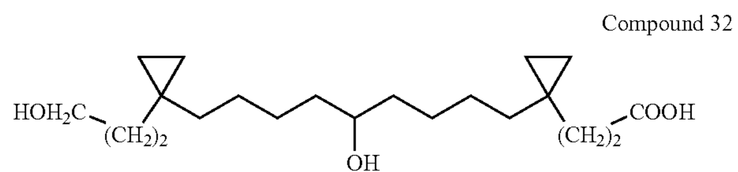
3-(1-{5-Hydroxy-9-[1-(3-hydroxy-propyl)-cyclopropyl]-nonyl}-cyclopropyl)-propionic acid
