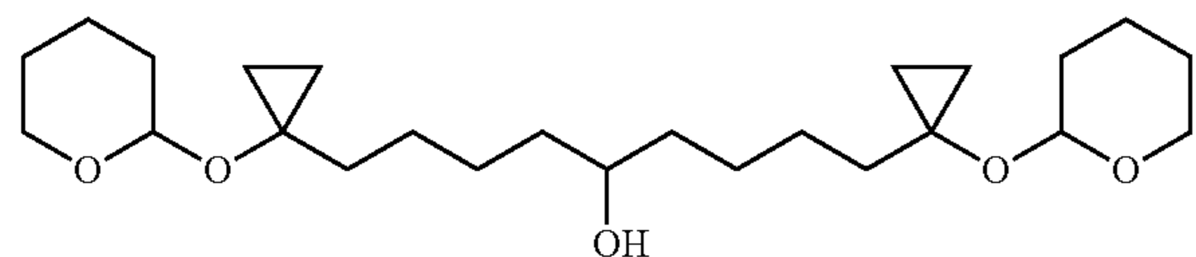
1,9-Bis-[1-(tetrahydro-pyran-2-yloxy)-cyclopropyl]-nonan-5-ol
