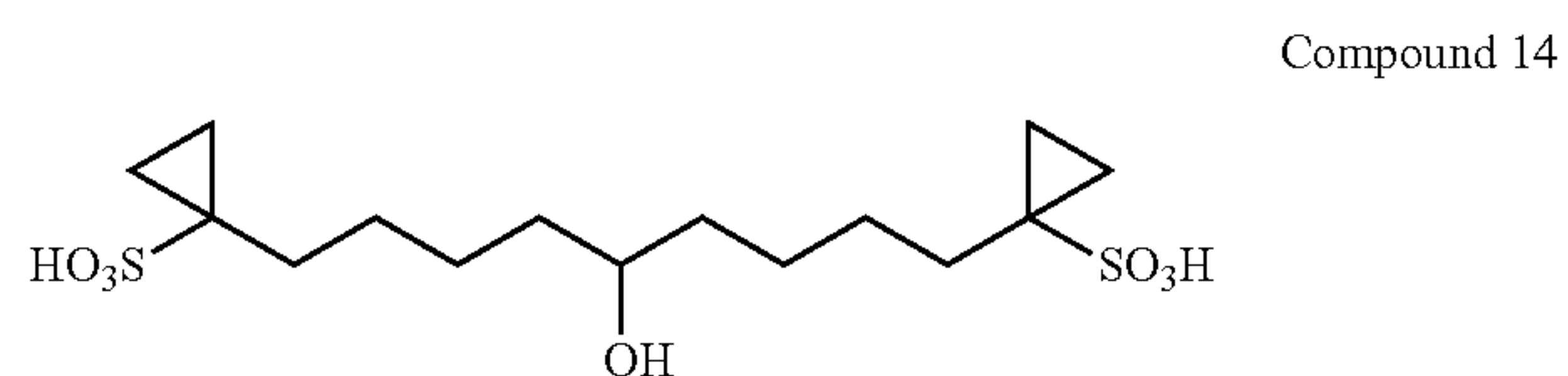
1,9-Bis-(1-sulfonyloxy-cyclopropyl)-nonan-5-ol
