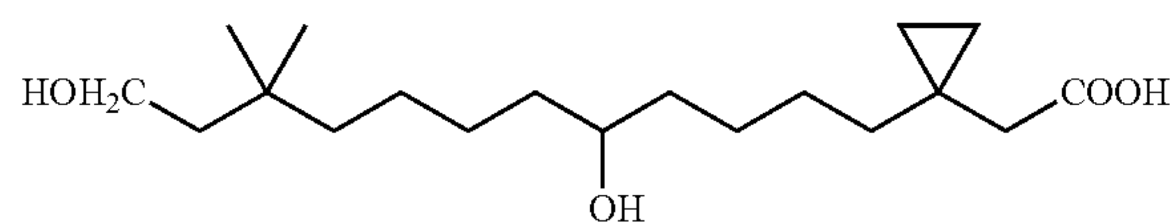
[1-(5,12-Dihydroxy-10,10-dimethyl-dodecyl)-cyclopropyl]-acetic acid
