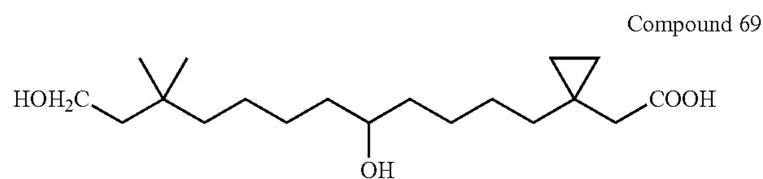
[1-(5,12-Dihydroxy-10,10-dimethyl-dodecyl)-cyclopropyl]-acetic acid
