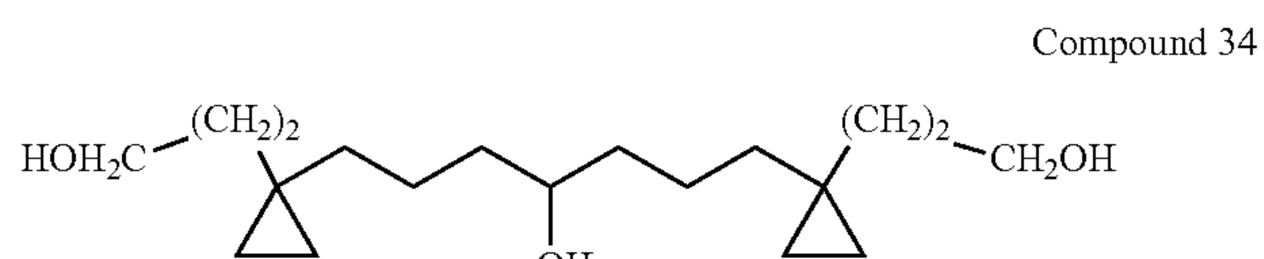
1,7-Bis-[1-(3-hydroxy-propyl)-cyclopropyl]-heptan-4-ol
