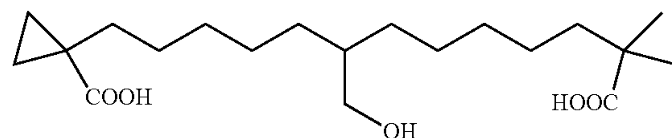
1-(12-Carboxy-6-hydroxymethyl-12-methyl-tridecyl)-cyclopropanecarboxylic acid
