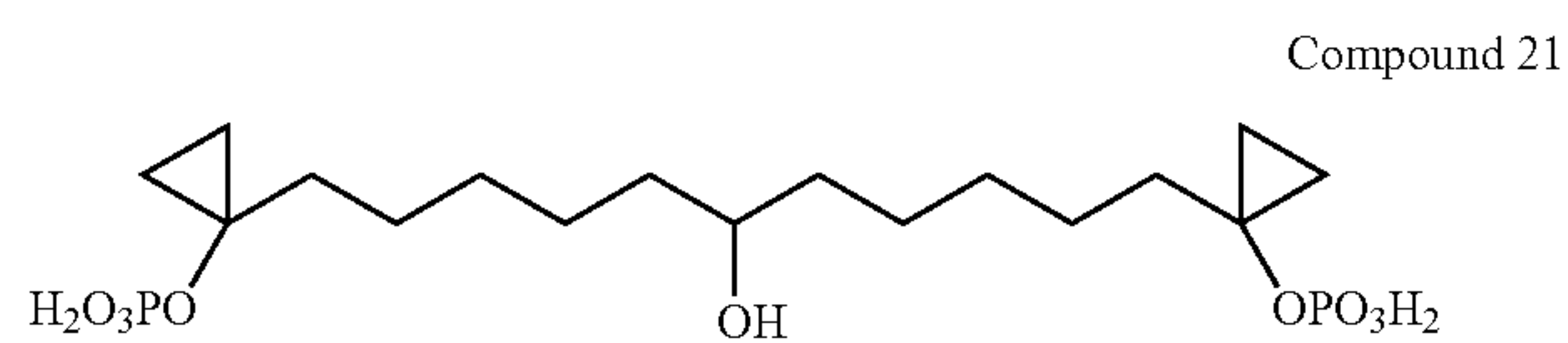
1,9-Bis-(1-phosphonoxy-cyclopropyl)-nonan-5-ol
