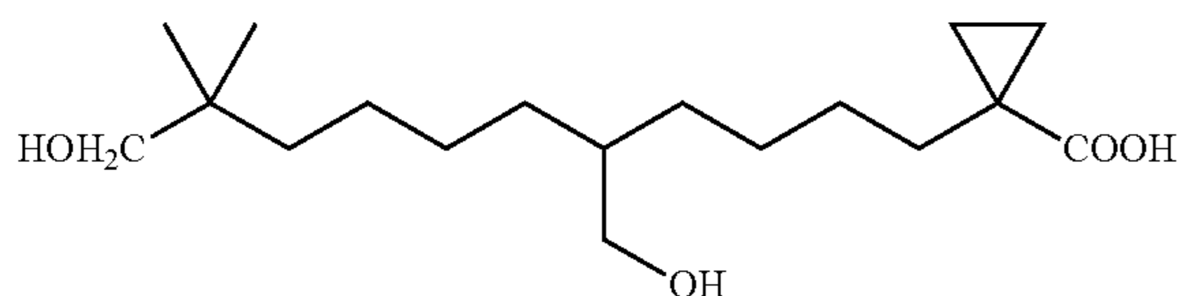
1-(11-Hydroxy-5-hydroxymethyl-10,10-dimethyl-undecyl)-cyclopropanecarboxylic acid
