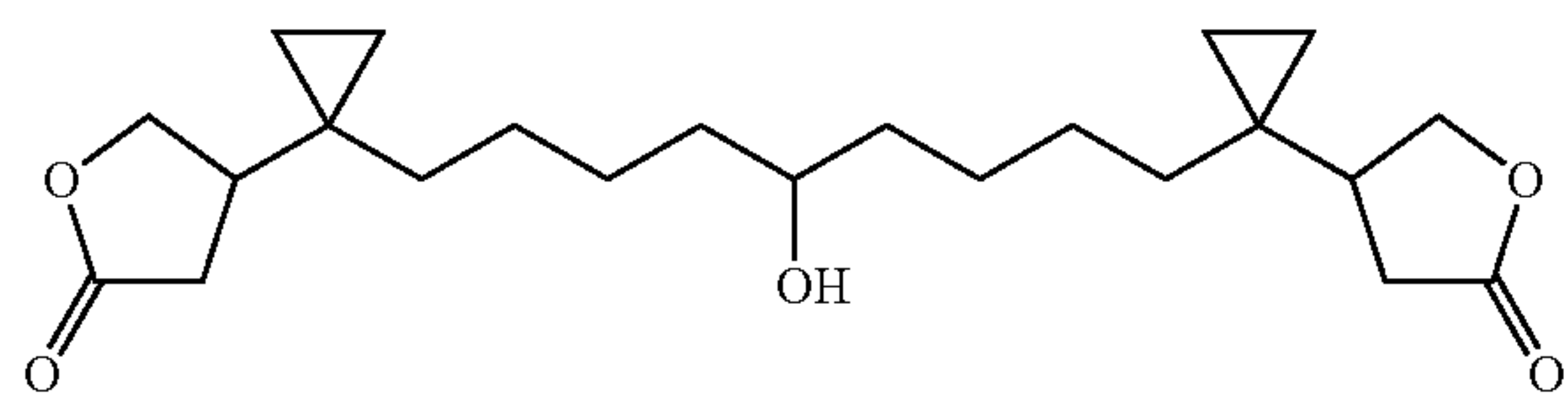
1,9-Bis-[1-(2-oxo-tetrahydrofuran-4-yl)-cyclopropyl]-nonan-5-ol
