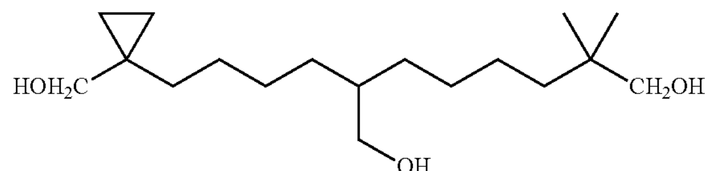
7-[4-(1-Hydroxymethyl-cyclopropyl)-butyl] 2,2-dimethyl-octane-1,8-diol
