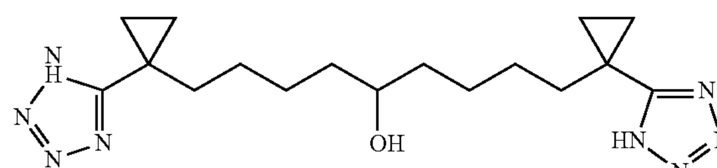
1,9-Bis-[I-(1H-tetrazol-5-yl)-cyclopropyl]-nonan-5-ol
