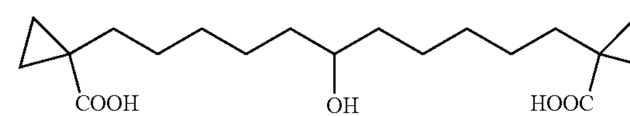
1-(12-Carboxy-6-hydroxy-12-methyl-tridecyl)-cyclopropanecarboxylic acid
