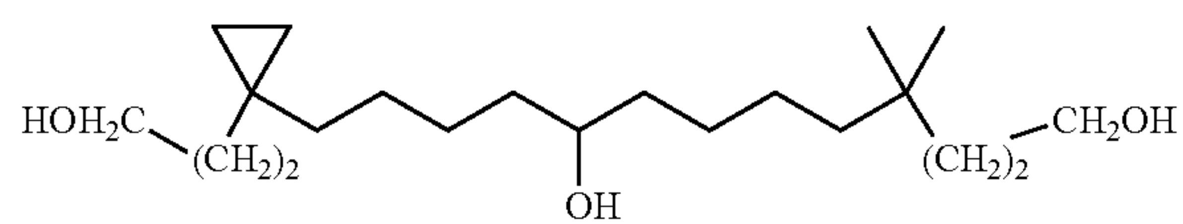
13-[1-(3-Hydroxy-propyl)-cyclopropyl]-4,4-dimethyl-tridecane-1,9-diol
