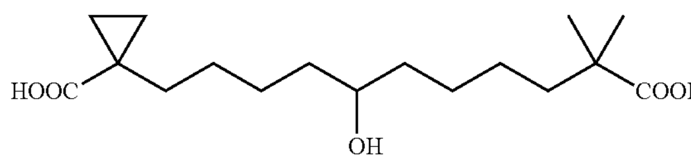
1-(10-Carboxy-5-hydroxy-10-methyl-undecyl)-cyclopropanecarboxylic acid
