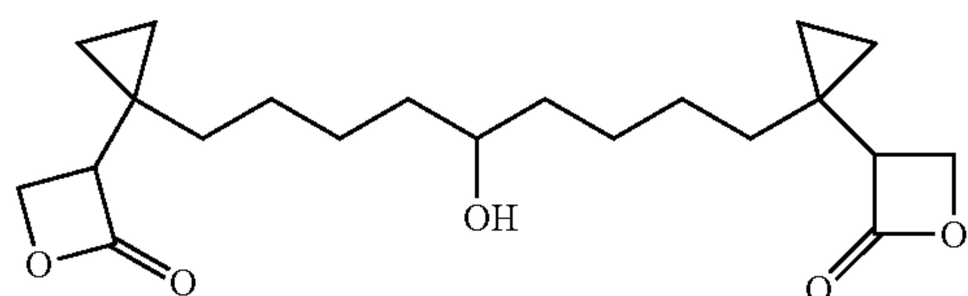
1,9-Bis-[1-(2-oxo-oxoethan-3-yl)-cyclopropyl]-nonan-5-ol
