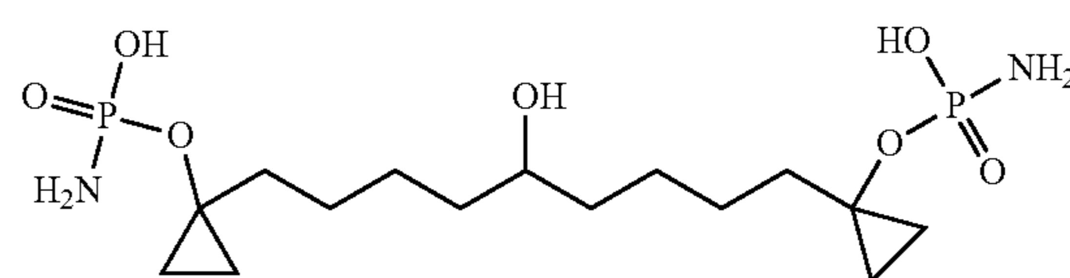
1,7-Bis-(1-phosponamido-cyclopropyl)-5-hydroxy-nonane
