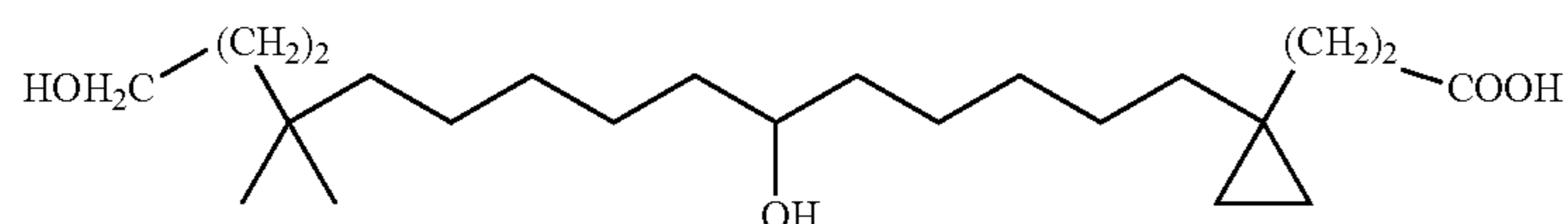
3-[1-(6,15-Dihydroxy-12,12-dimethyl-pentadecyl)-cyclopropyl]-propionic acid
