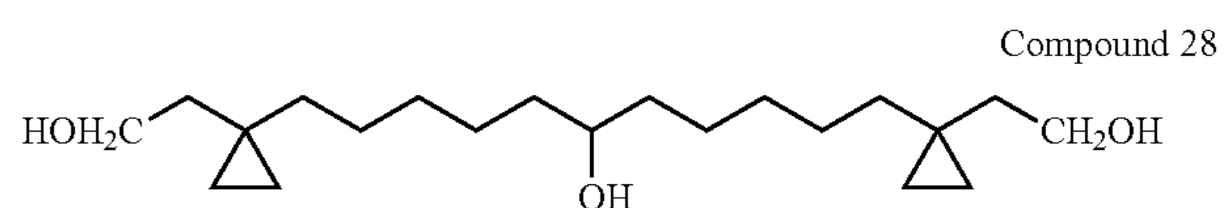
1,11-Bis-[1,2-hydroxy-ethyl]-cyclopropyl]-undecan-6-ol
