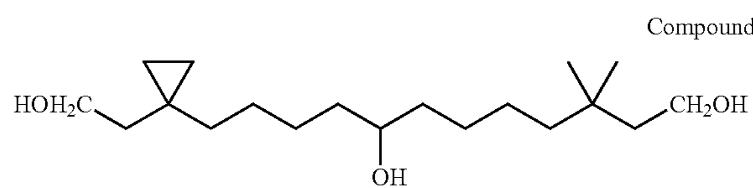
12-[1-(2-Hydroxy-ethyl)-cyclopropyl]-3,3-dimethyl-dodecane-1,8-diol
