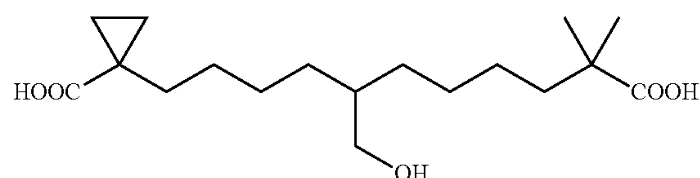
1-(1,0-Carboxy-5-hydroxymethyl-10-methyl-undecyl)-cyclopropanecarboxylic acid
