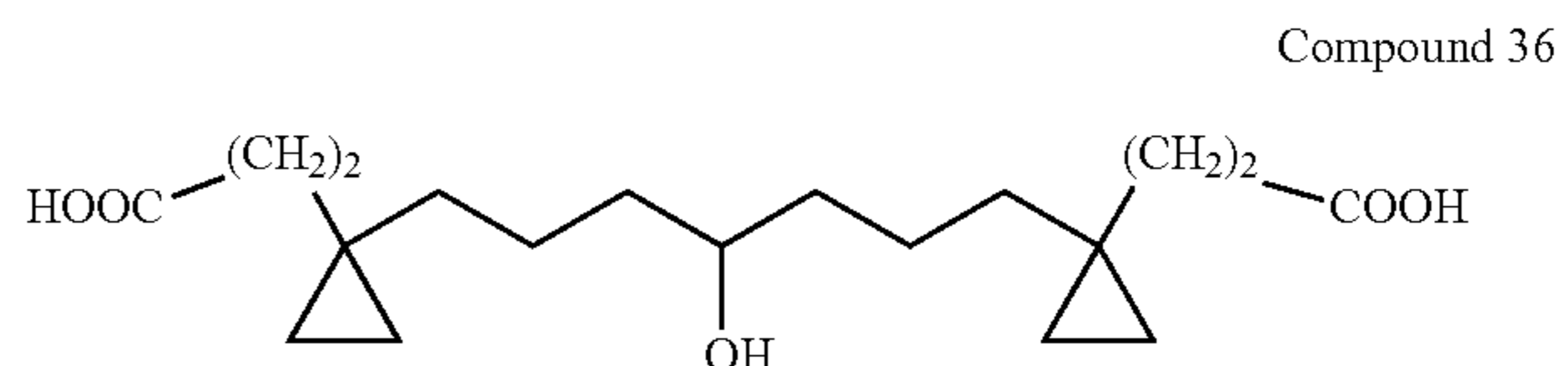
3-(1-{7-[1-(2-Carboxy-ethyl)-cyclopropyl]-4-hydroxy-heptyl}-cyclopropyl)-propionic acid
