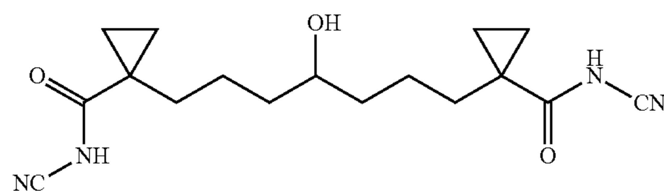
1,7-Bis-(1-dicyanimido-cyclopropyl)-4-hydroxy-heptane
