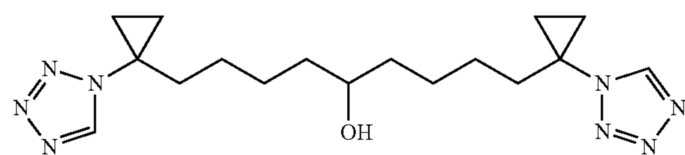
1,9-Bis-(1-tetrazol-1-yl-cyclopropyl)-nonan-5-ol
