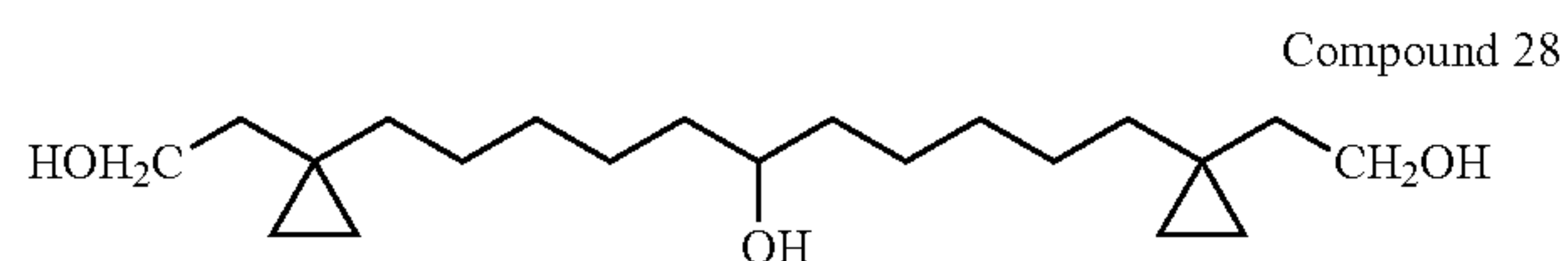
1,11-Bis-[1,2-hydroxy-ethyl)-cyclopropyl]-undecan-6-ol
