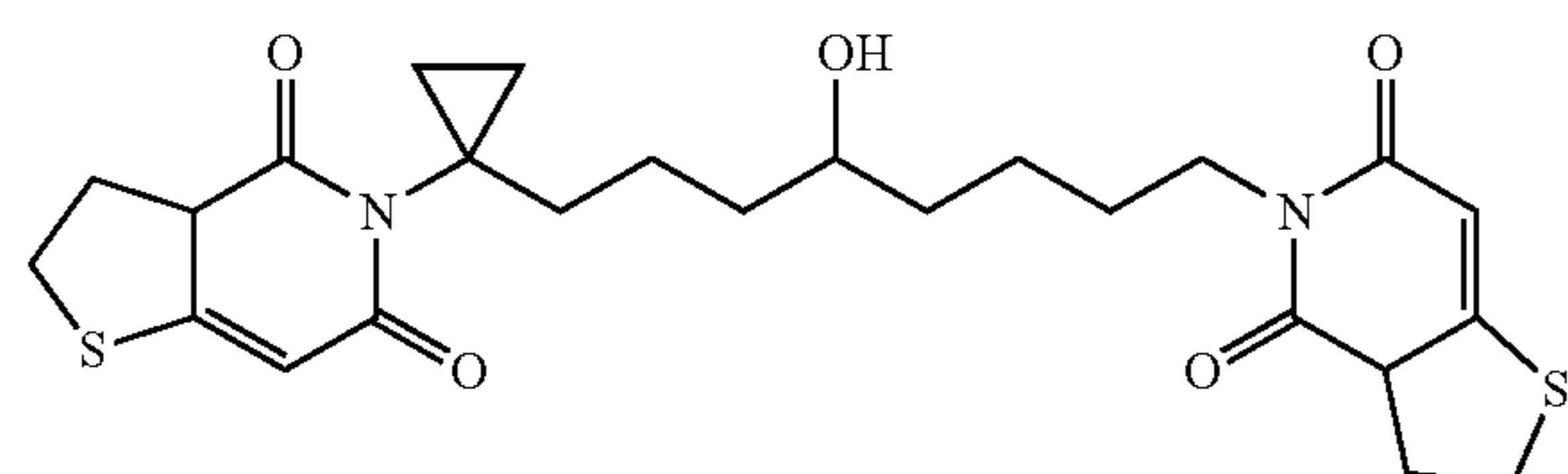
1,7-Bis-(4,6-dioxo-2,3,3a,6-tetrahydro-4H-thieno[3,2-c]pyridin-5-yl)-1-(cyclopropyl)-6-hydroxy-heptane
