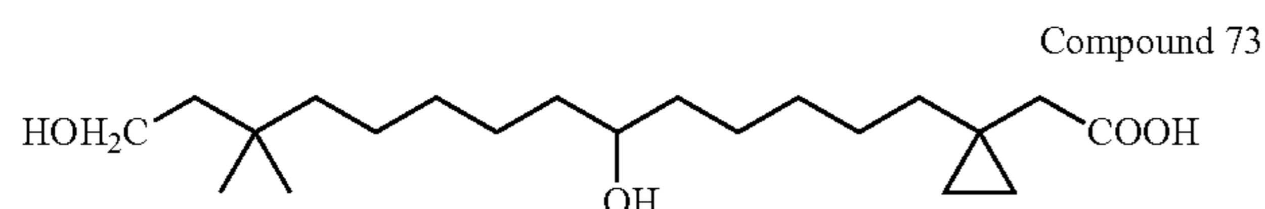
[1-(6,14-Dihydroxy-12,12-dimethyl-tetradecyl)-cyclopropyl]-acetic acid
