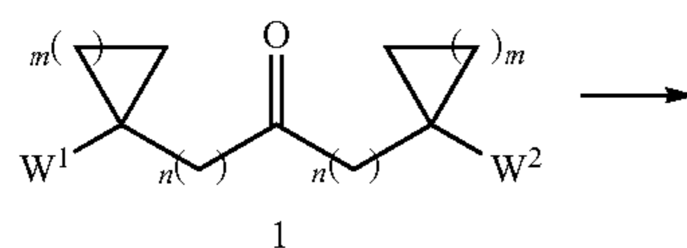
Scheme 1: Synthesis of compounds of formula 2 and 4
