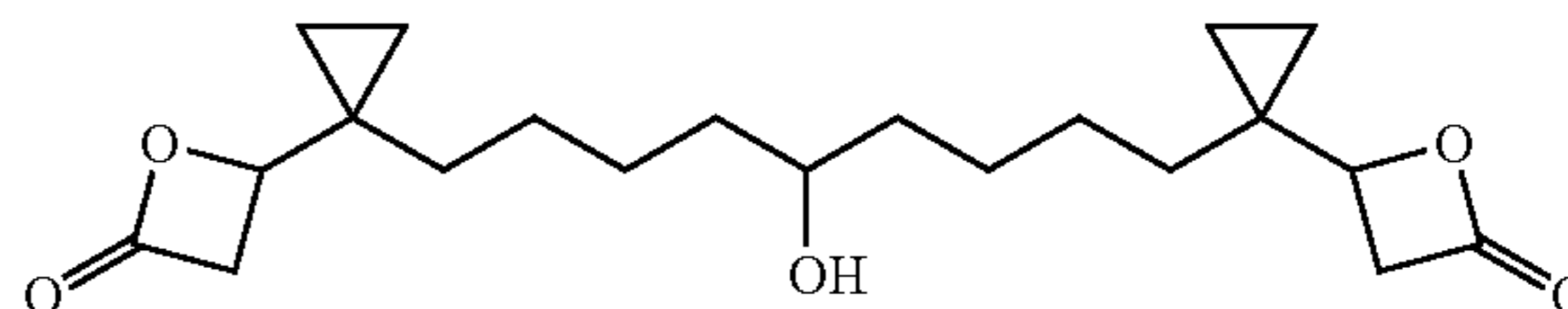
1,9-Bis-[1-(2-oxo-oxoethan-3-yl)-cyclopropyl]-nonan-5-ol
