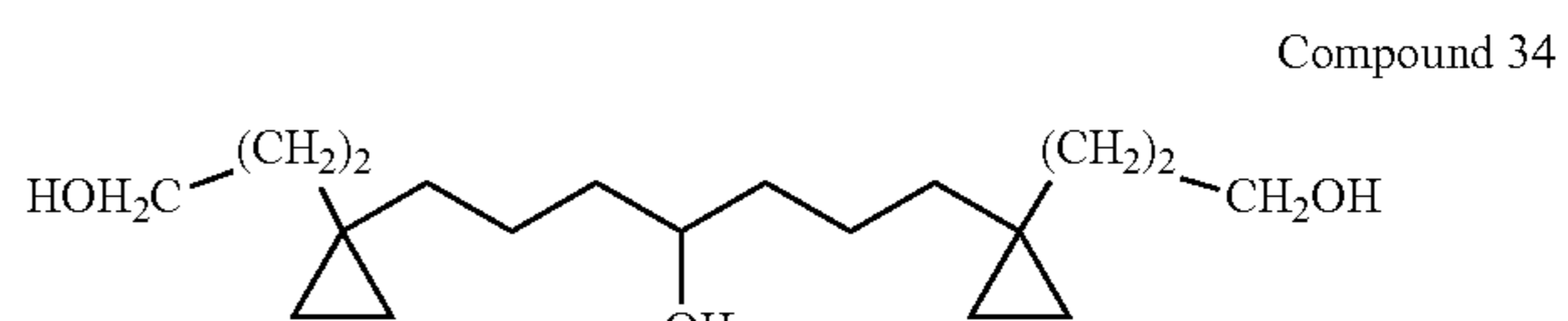
3-(1-{5-Hydroxy-9-[1-(3-hydroxy-propyl)-cyclopropyl]-nonyl}-cyclopropyl)-propionic acid
