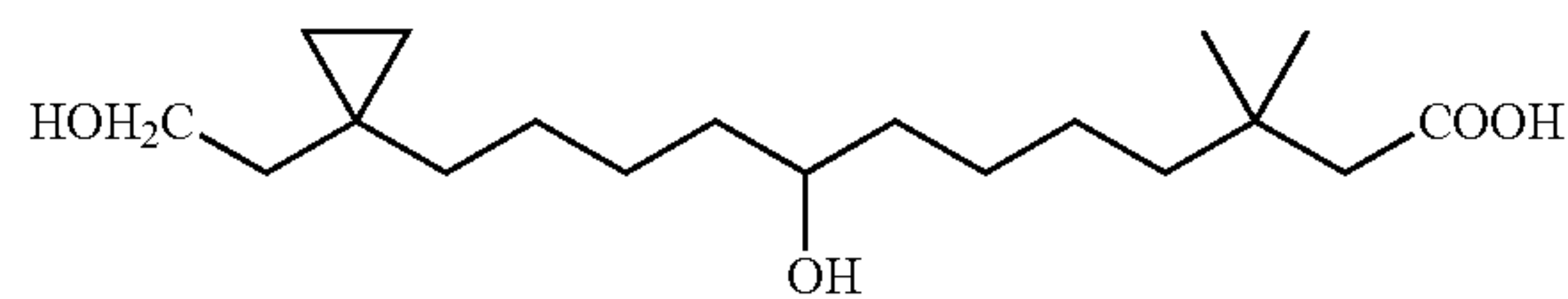
8-Hydroxy-12-[1-(2-hydroxy-ethyl)-cyclopropyl]-3,3-dimethyl-dodecanoic acid
