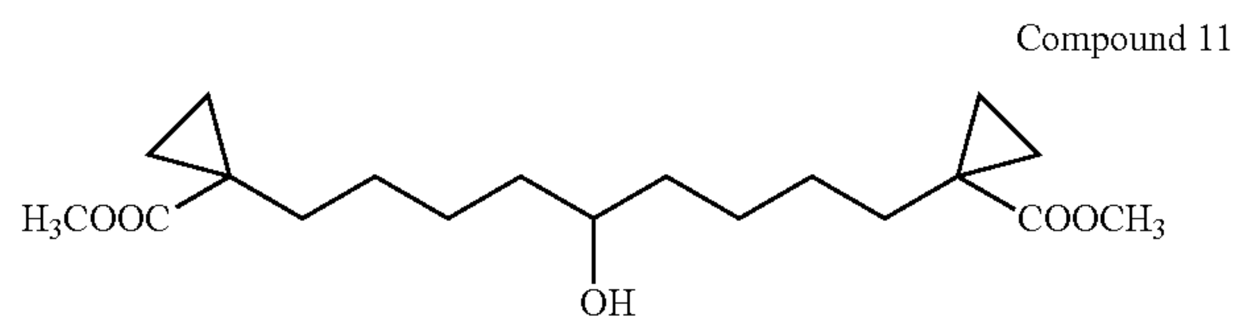
1,9-Bis-(1-carbomethoxy-cyclopropyl)-nonan-5-ol
