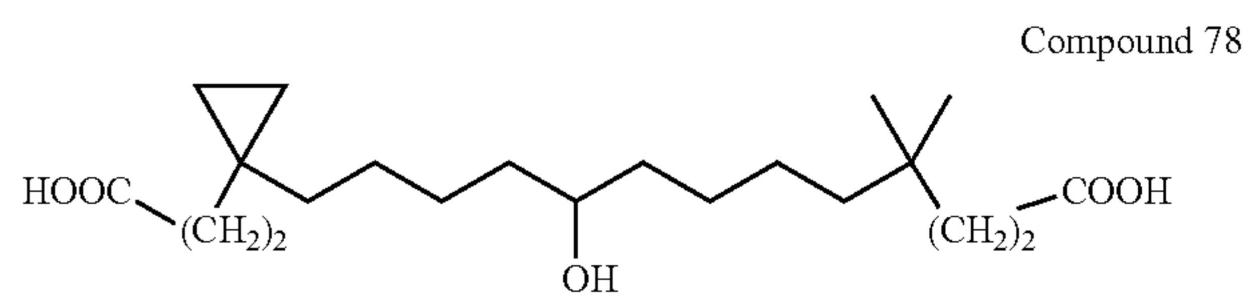
13-[1-(2-Carboxyethyl)-cyclopropyl]-9-hydroxy-4,4-dimethyl-tridecanoic acid
