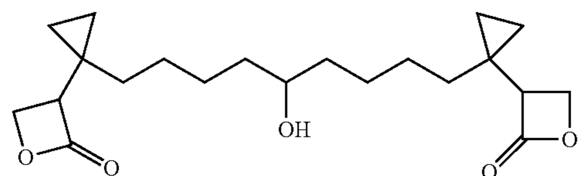
1,9-Bis-[1-(2-oxo-oxoethan-3-yl)-cyclopropyl]-nonan-5-ol
