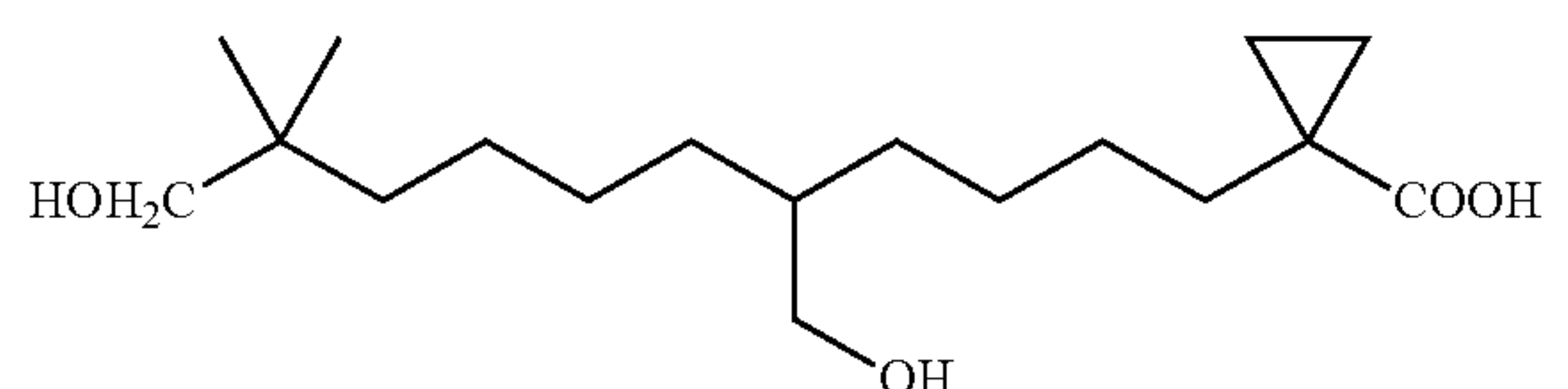
1-(11-Hydroxy-5-hydroxymethyl-10,10-dimethyl-undecyl)-cyclopropanecarboxylic acid
