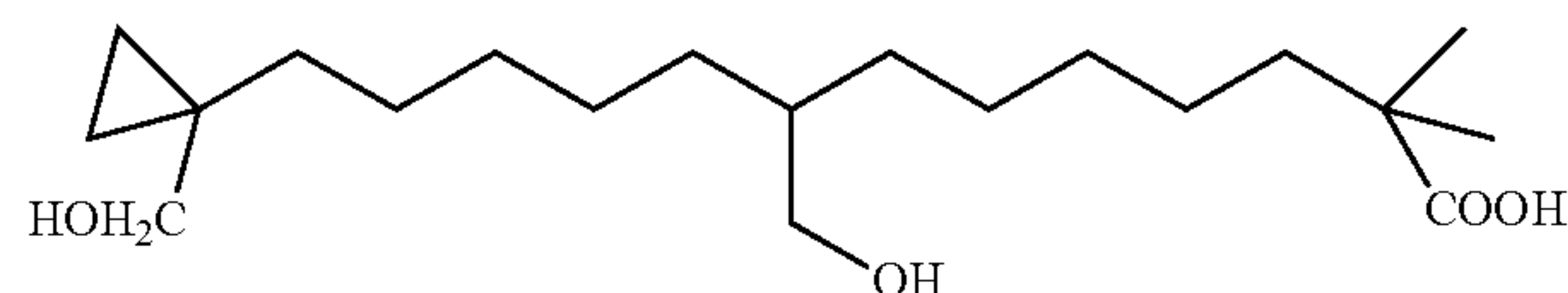
8-Hydroxymethyl-13-(1-hydroxymethyl-cyclopropyl)-2,2-dimethyl-tridecanoic acid
