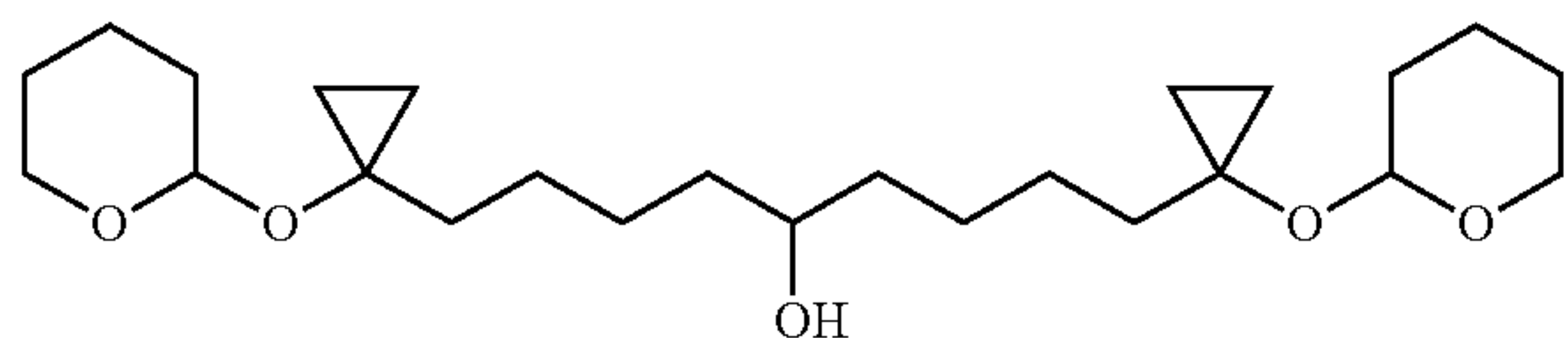
1,9-Bis-[1-(tetrahydro-pyran-2-yloxy)-cyclopropyl]-nonan-5-ol
