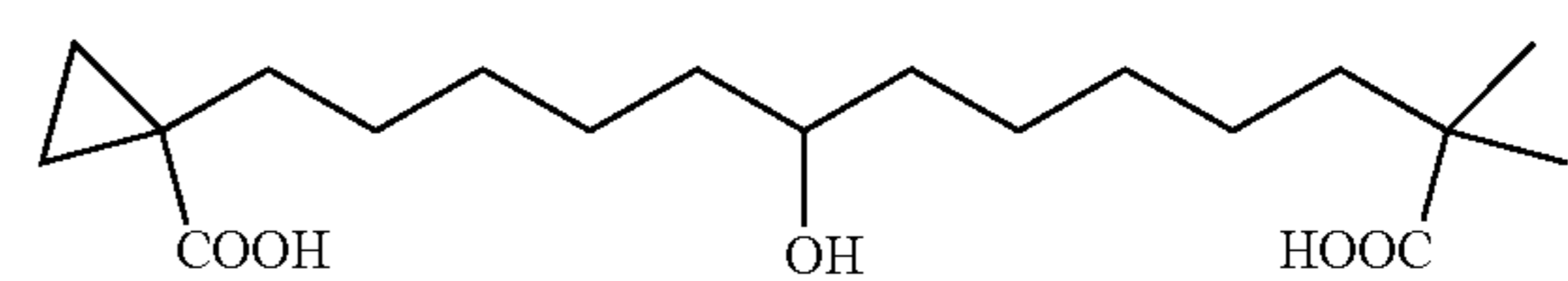
1-(12-Carboxy-6-hydroxy-12-methyl-tridecyl)-cyclopropanecarboxylic acid
