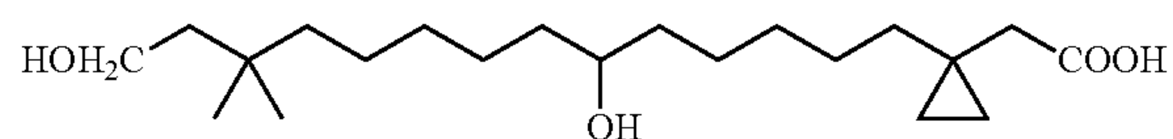
[1-(6,14-Dihydroxy-12,12-dimethyl-tetradecyl)-cyclopropyl]-acetic acid
