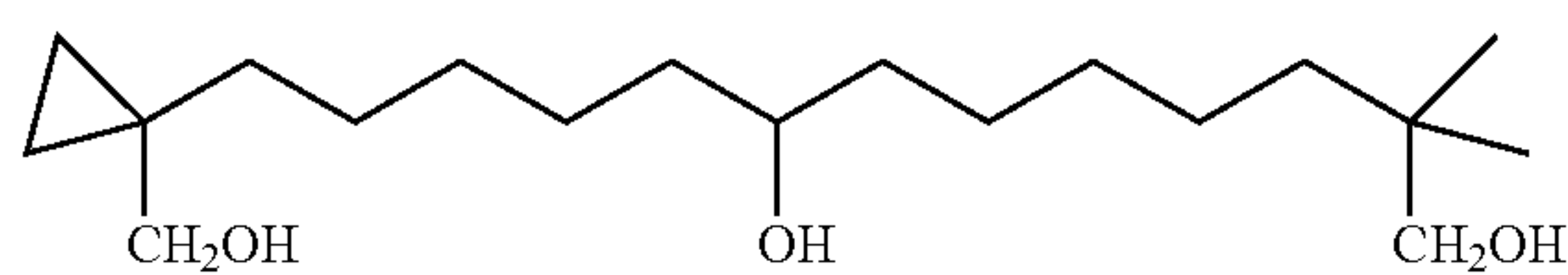
13-(1-Hydroxymethyl-cyclopropyl)-2,2-dimethyl-tridecane-1,8-diol
