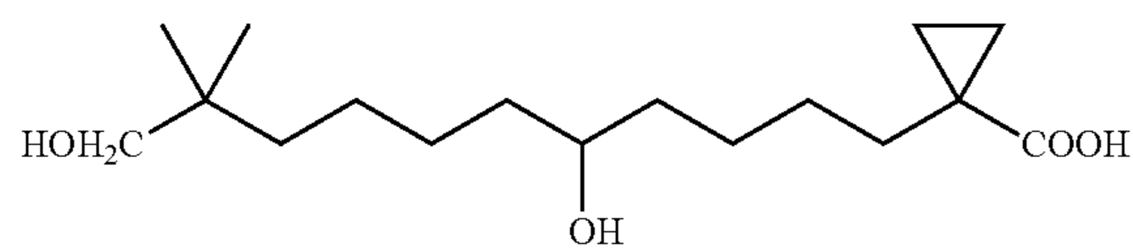
1-(5,11-Dihydroxy-10,10-dimethyl-undecyl)-cyclopropanecarboxylic acid
