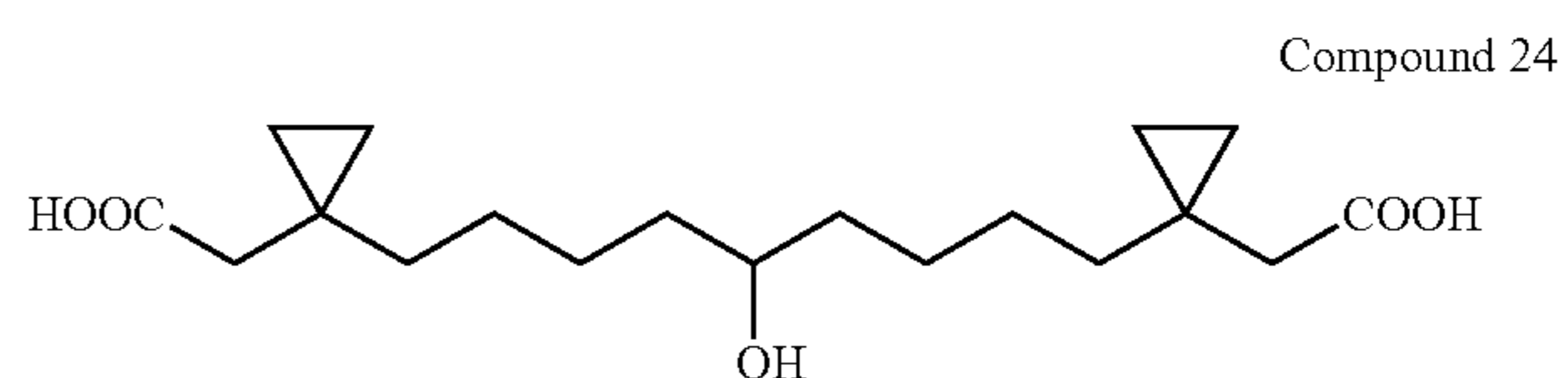
{1-[9-Carboxymethyl-cyclopropyl]-5-hydroxy-nonyl}-cyclopropyl}-acetic acid
