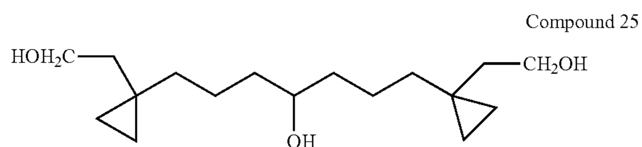
1,7-Bis-[1-(2-hydroxy-ethyl)-cyclopropyl]-heptan-4-ol
