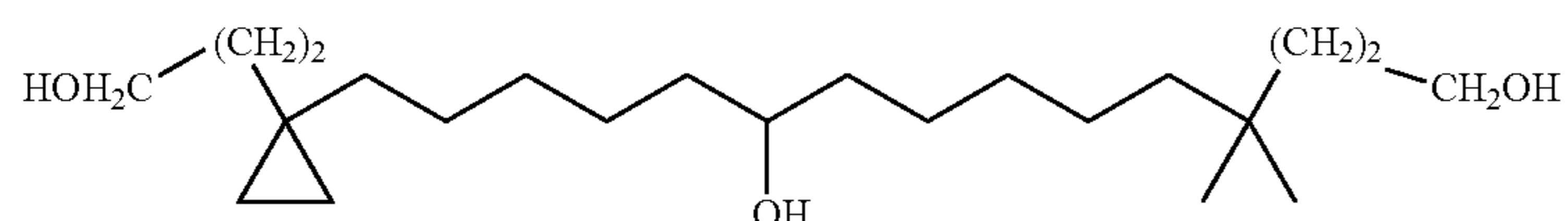
15-[1-(3-Hydroxy-propyl)-cyclopropyl]-4,4-dimethyl-pentadecane-1,10-diol
