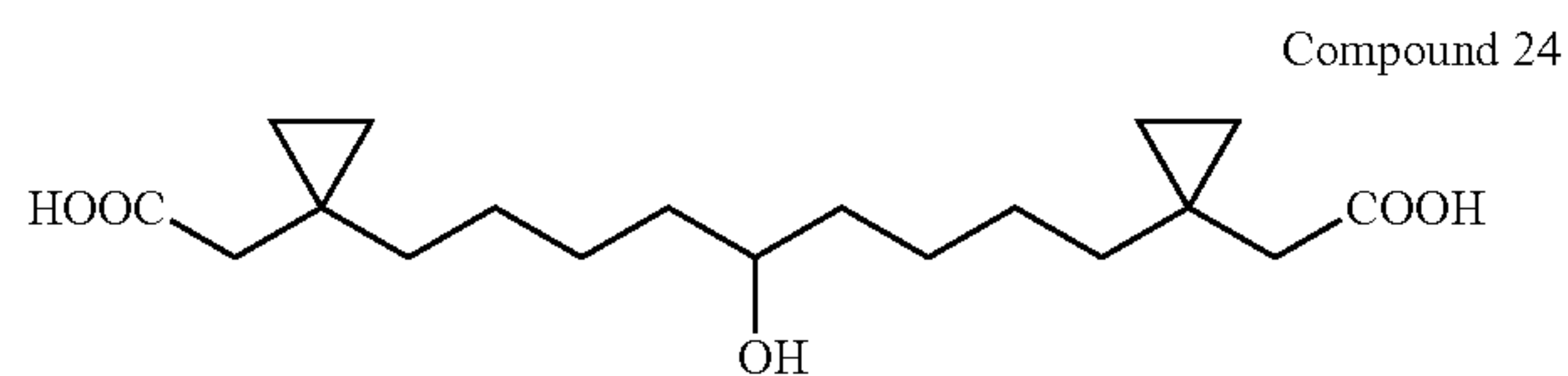
{1-[9-Carboxymethyl-cyclopropyl]-5-hydroxy-nonyl}-cyclopropyl}-acetic acid
