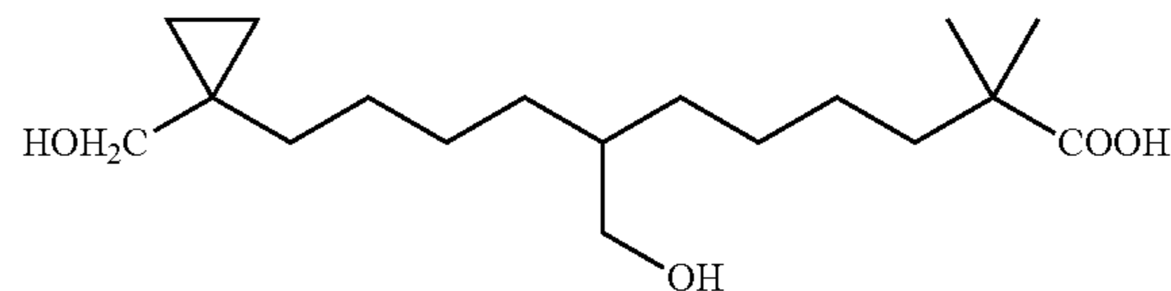
7-Hydroxymethyl-11-(1-hydroxymethyl-cyclopropyl)-2,2-dimethyl-undecanoic acid
