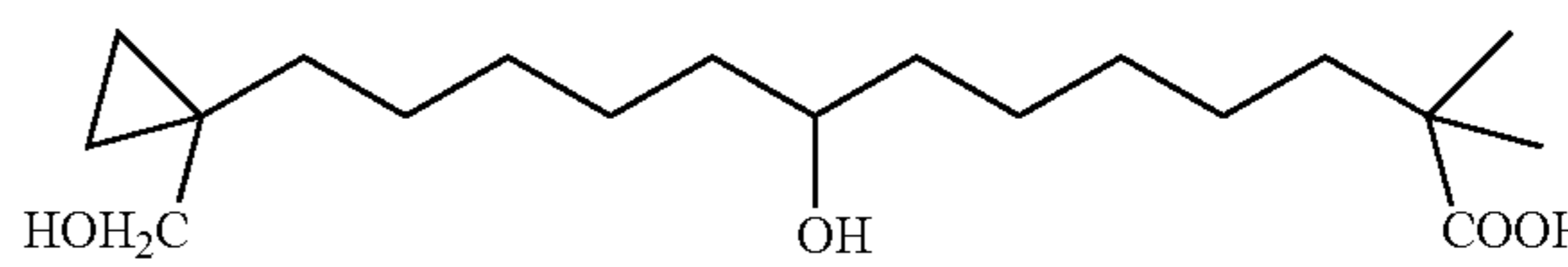
8-Hydroxy-13-(1-hydroxymethyl-cyclopropyl)-2,2-dimethyl-tridecanoic acid
