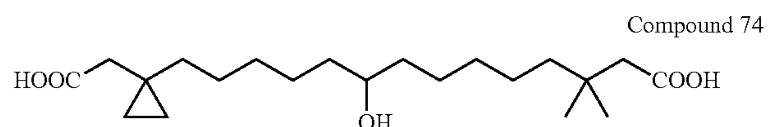
14-(1-Carboxymethyl-cyclopropyl)-9-hydroxy-3,3-dimethyl-tetradecanoic acid
