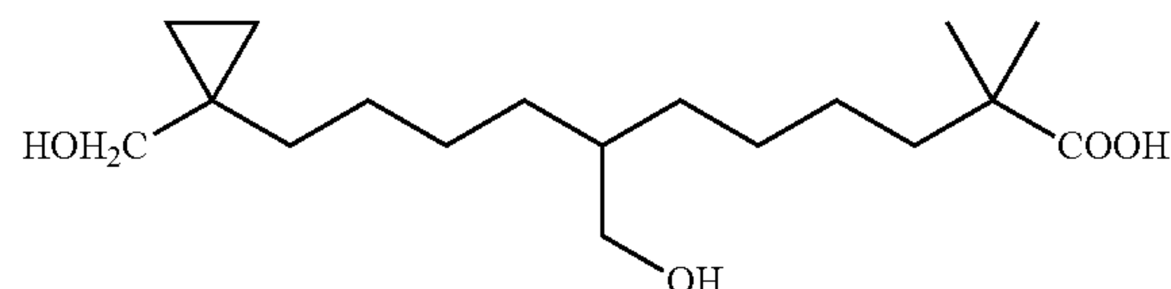
7-Hydroxymethyl-11-(1-hydroxymethyl-cyclopropyl)-2,2-dimethyl-undecanoic acid
