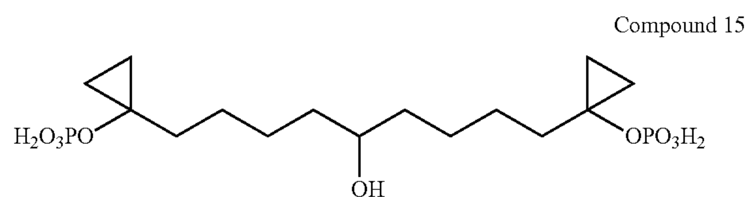
1,9-Bis-(1-phosphonoxy-cyclopropyl)-nonan-5-ol
