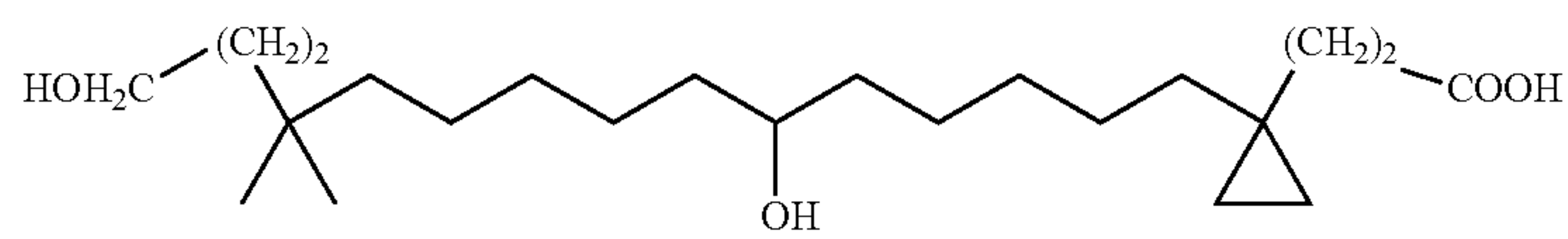
3-[1-(6,15-Dihydroxy-12,12-dimethyl-pentadecyl)-cyclopropyl]-propionic acid
