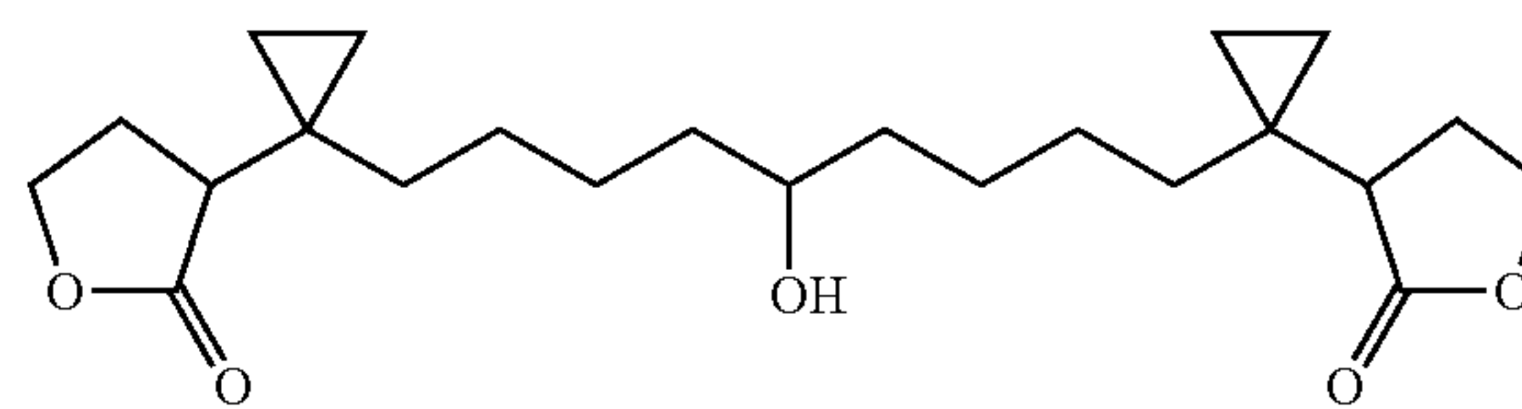
1,9-Bis-[1-(2-oxo-tetrahydrofuran-3-yl)-cyclopropyl]-nonan-5-ol
