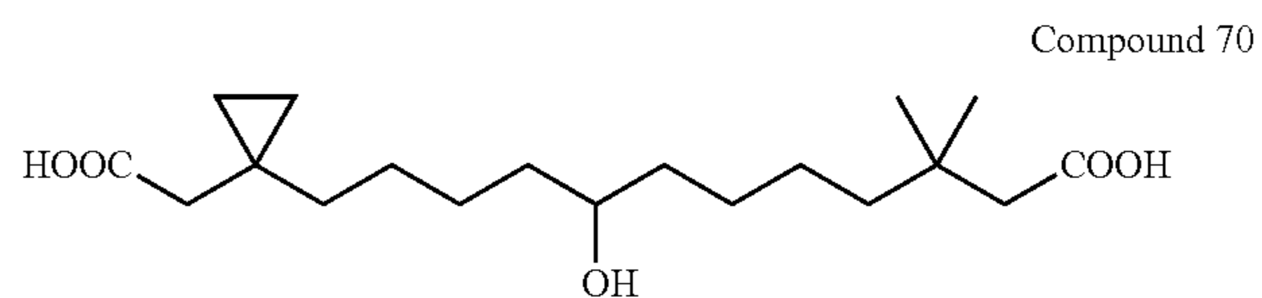
12-(1-Carboxymethyl-cyclopropyl)-8-hydroxy-3,3-dimethyl-dodecanoic acid
