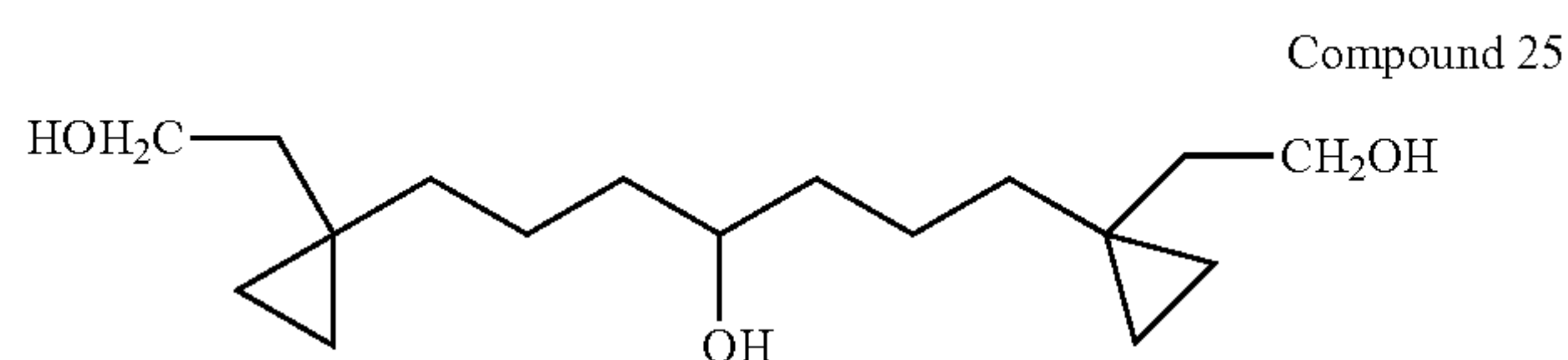
1,7-Bis-[1-(2-hydroxy-ethyl)-cyclopropyl]-heptan-4-ol
