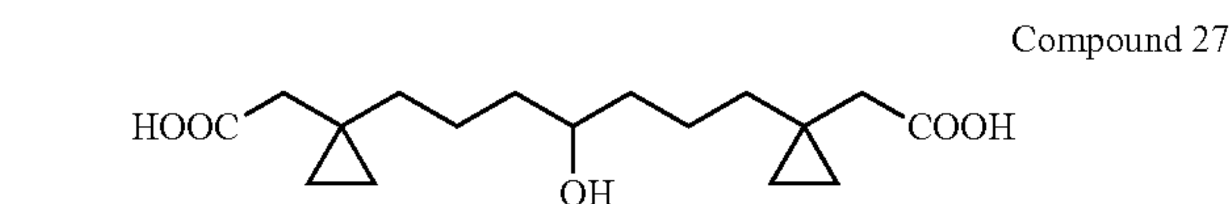
{1-[7-(1-Carboxymethyl-cyclopropyl)-4-hydroxy-heptyl]-cyclopropyl}-acetic acid
