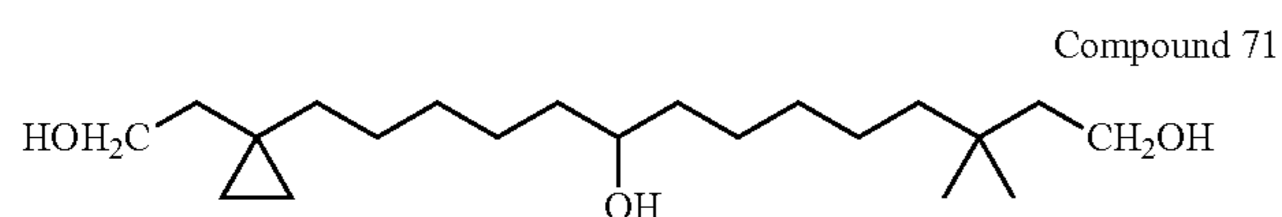
14-[1-(2-Hydroxy-ethyl)-cyclopropyl]-3,3-dimethyl-tetradecane-1,9-diol
