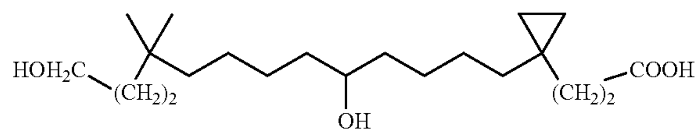
3-[1-(5,13-Dihydroxy-10,10-dimethyl-tridecyl)-cyclopropyl]-propionic acid
