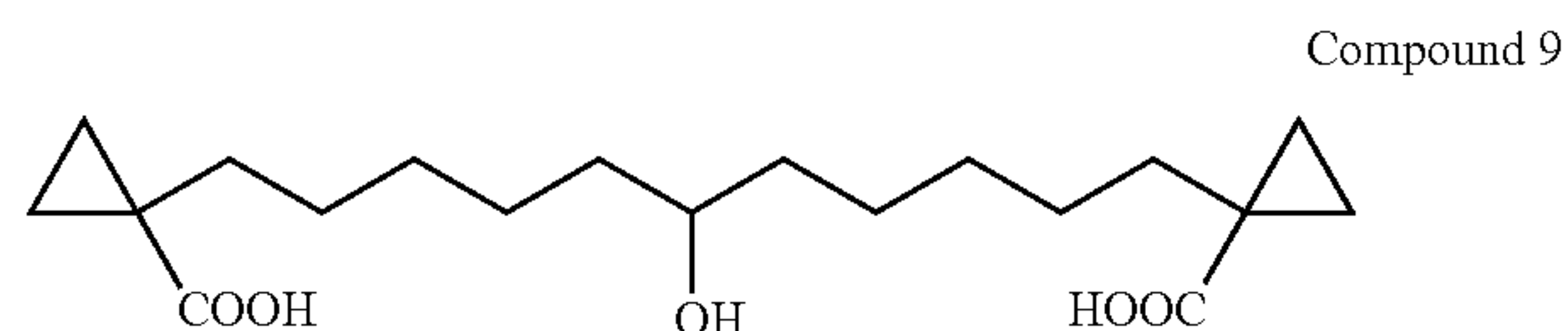
1,11-Bis-(1-carboxy-cyclopropyl)-undecan-6-ol
