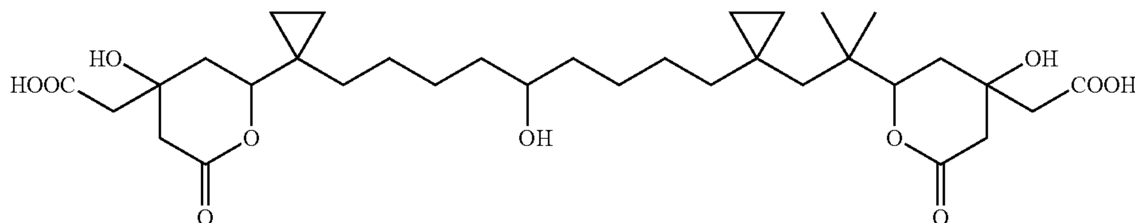
1,9-Bis {1-[9-(4-carboxymethyl-4-hydroxy-6-oxo-tetrahydro-pyran-2-yl)-(cyclopropyl)]}-5-hydroxy-nonane
