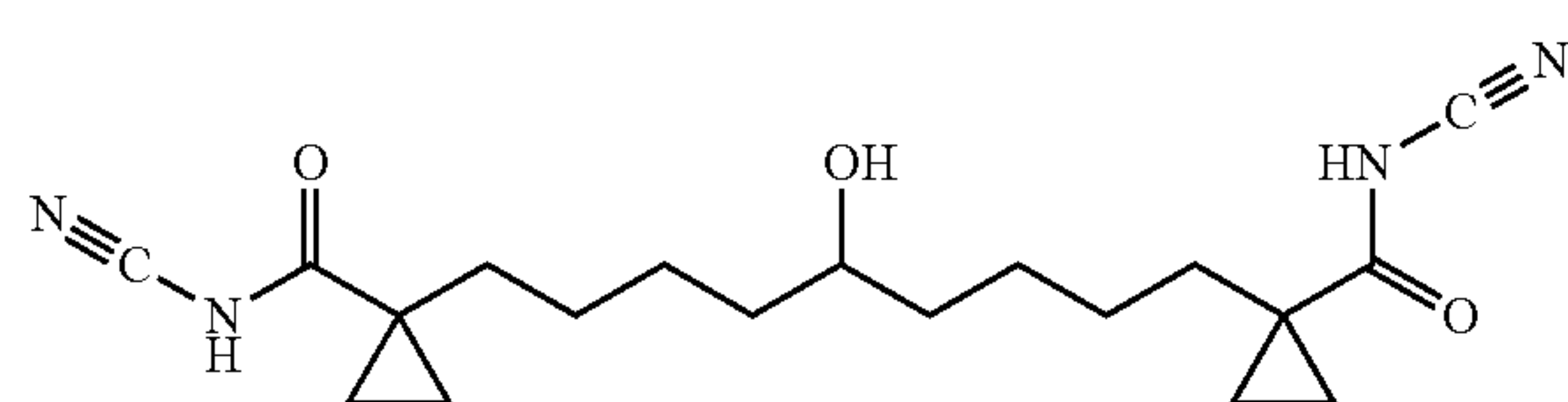
1,7-Bis-(1-dicyanimido-cyclopropyl)-5-hydroxy-nonane
