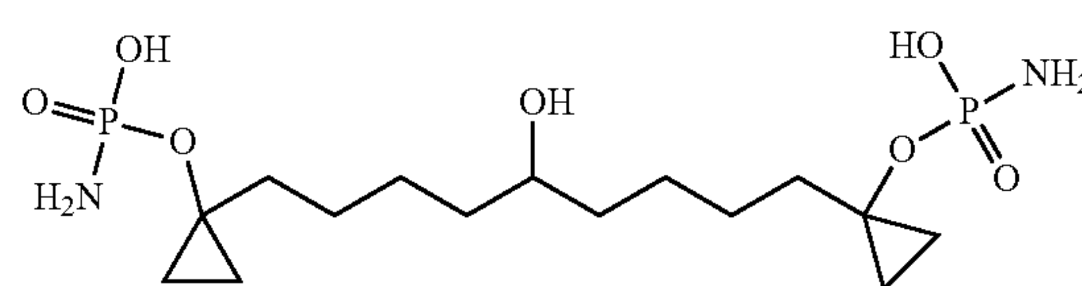
1,7-Bis-(1-phosponamido-cyclopropyl)-5-hydroxy-nonane
