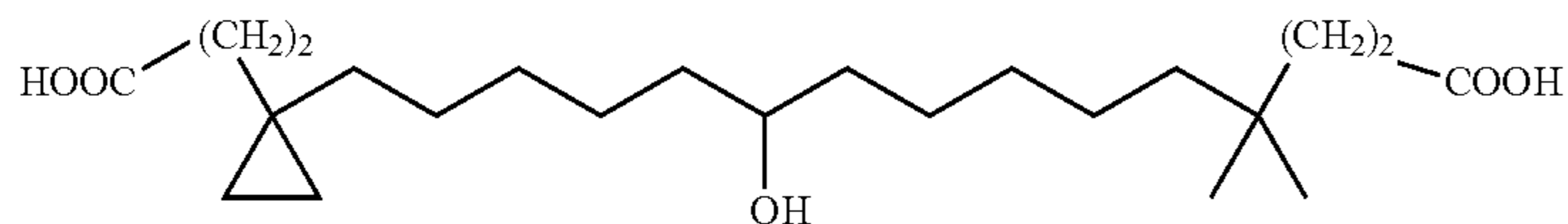
15-[1-(2-Carboxyethyl)-cyclopropyl]-10-hydroxy-4,4-dimethyl-tridecanoic acid
