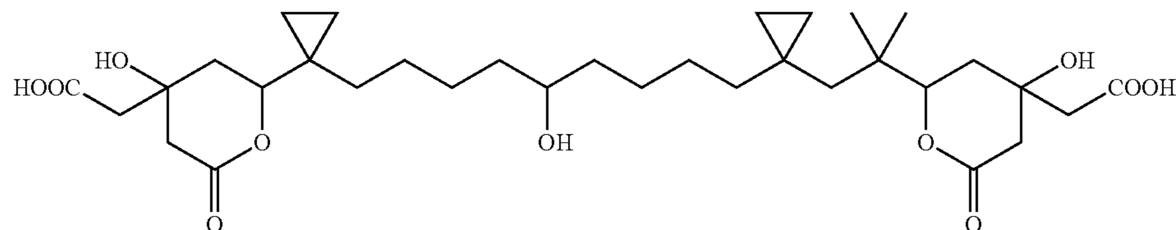
1,9-Bis {1-[9-(4-carboxymethyl-4-hydroxy-6-oxo-tetrahydro-pyran-2-yl)-(cyclopropyl)]}-5-hydroxy-nonane
