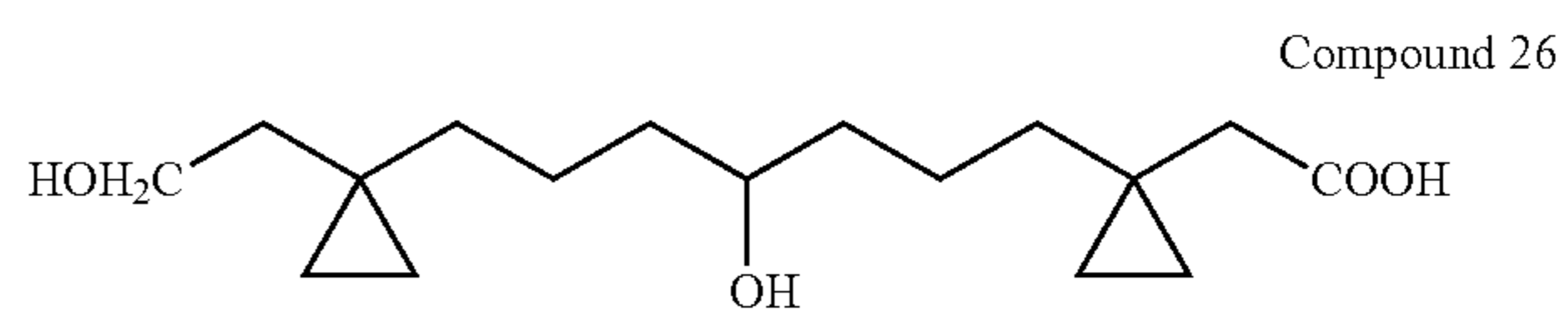
(1-{4-Hydroxy-7-[1-(2-hydroxy-ethyl)-cyclopropyl]-heptyl}-cyclopropyl)-acetic acid
