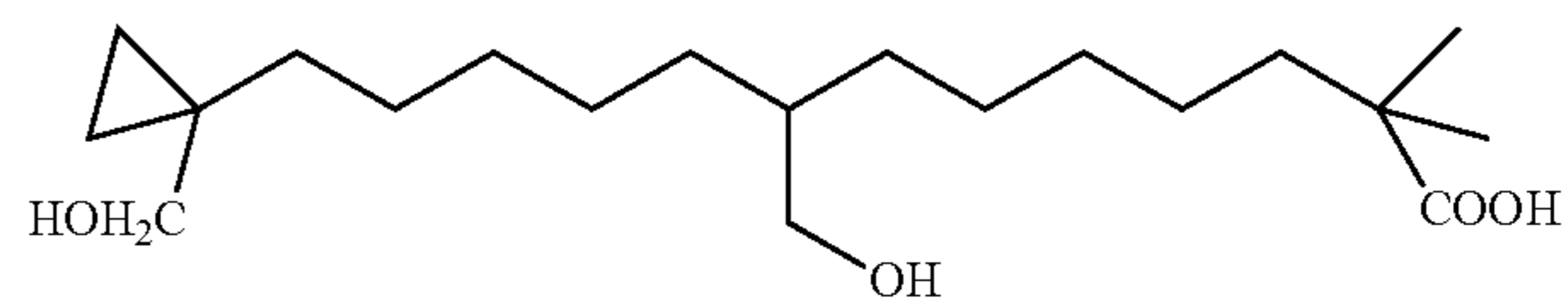
8-Hydroxymethyl-13-(1-hydroxymethyl-cyclopropyl)-2,2-dimethyl-tridecanoic acid
