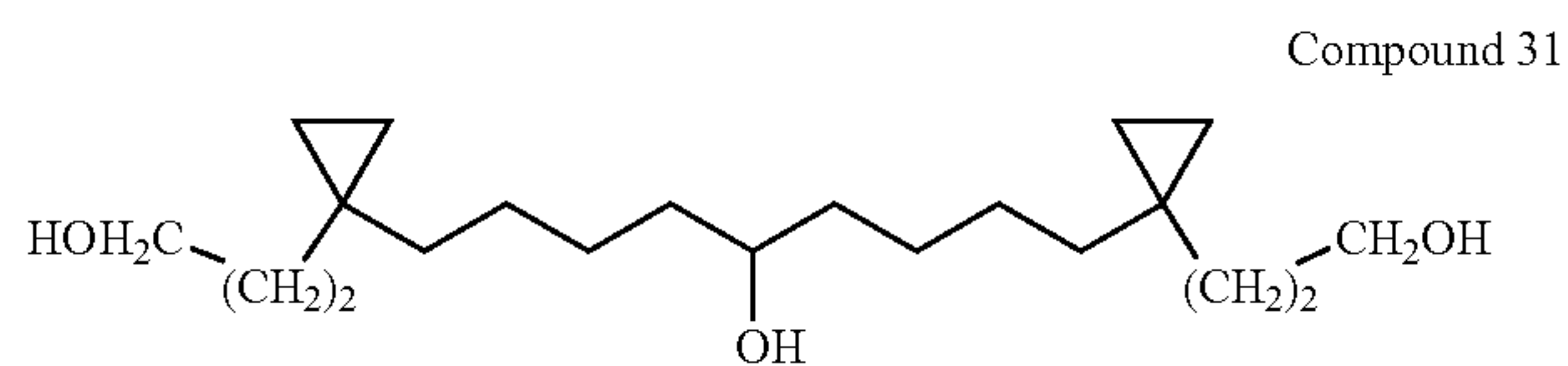
1,9-Bis-[1-(3-hydroxy-propyl)-cyclopropyl]-nonan-5-ol
