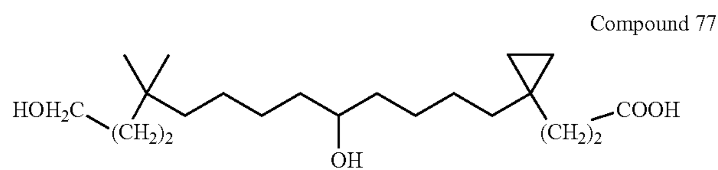
3-[1-(5,13-Dihydroxy-10,10-dimethyl-tridecyl)-cyclopropyl]-propionic acid
