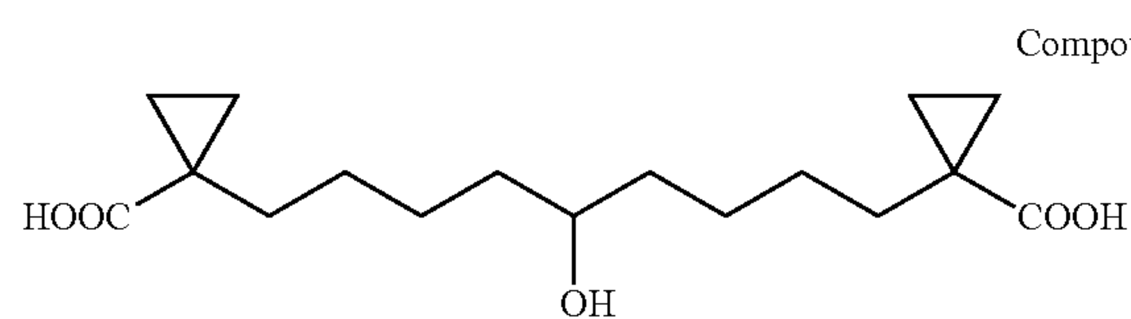
1,9-Bis-(1-carboxy-cyclopropyl)-nonan-5-ol
