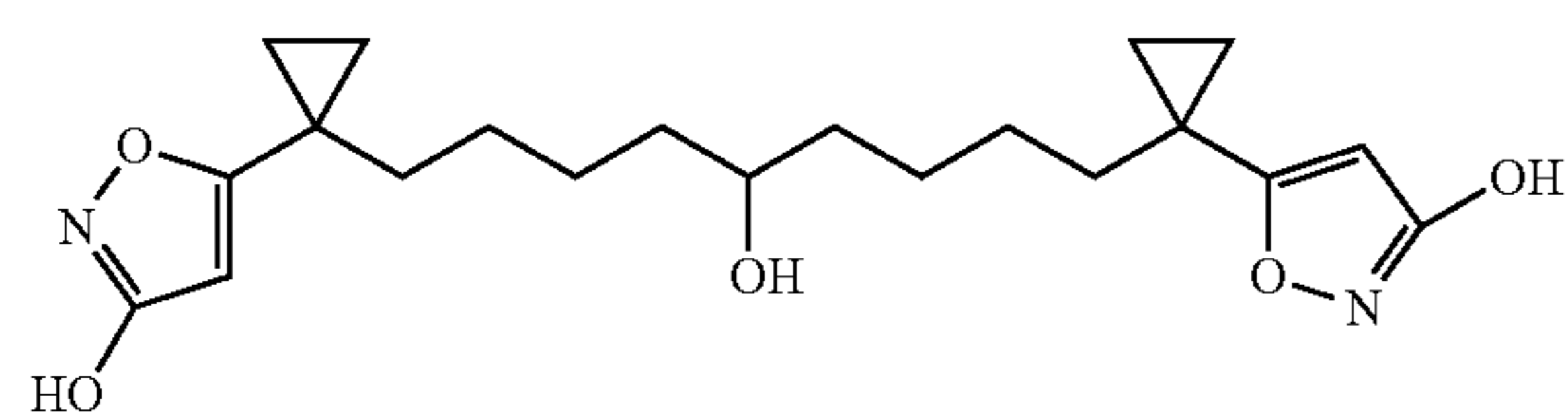
1,9-Bis-[1-(3-hydroxy-isoxazol-5-yl)-cyclopropyl]-nonan-5-ol
