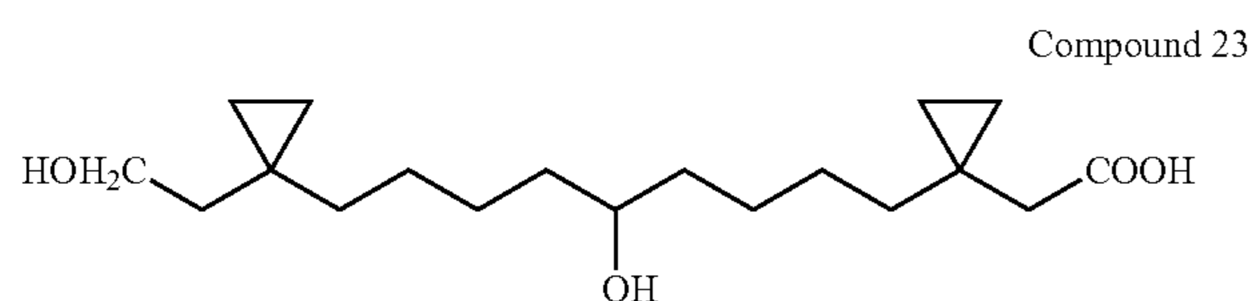
(1-{5-Hydroxy-9-[1-(2-hydroxy-ethyl)-cyclopropyl]-nonyl}-cyclopropyl)-acetic acid
