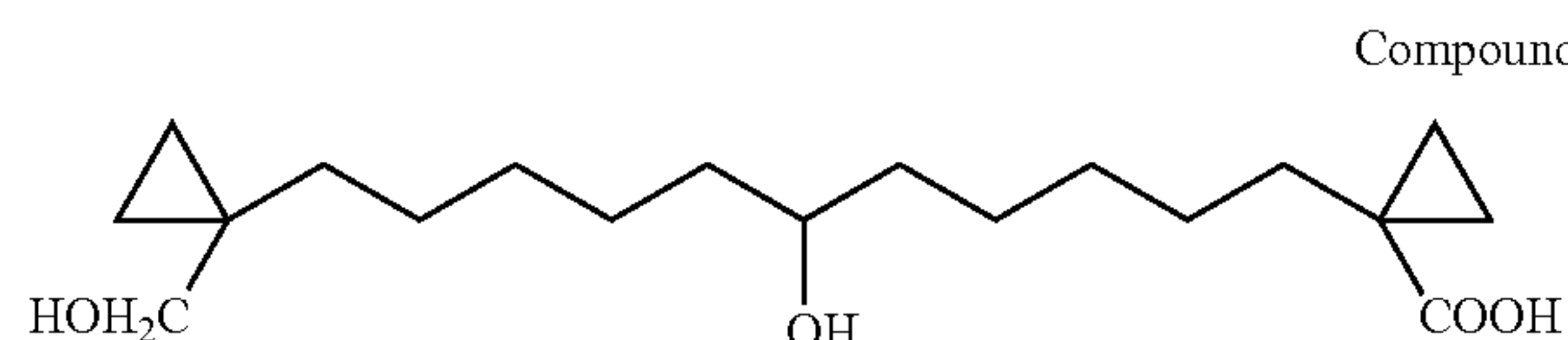
1-[6-Hydroxy-11-(1-hydroxymethyl-cyclopropyl)-undecyl]-cyclopropanecarboxylic acid
