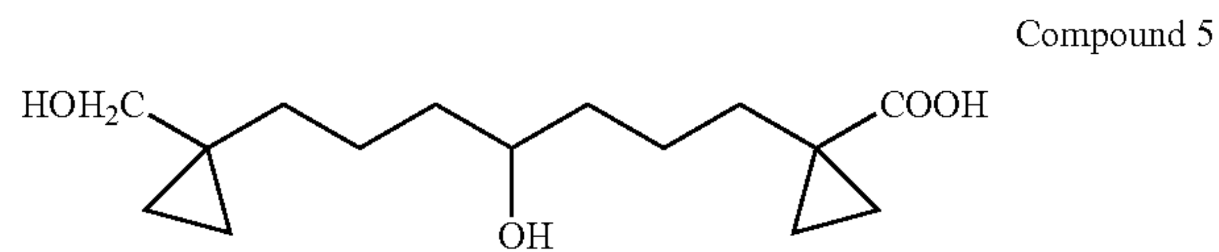
1-[4-Hydroxy-7-(1-hydroxymethyl-cyclopropyl)-heptyl]-cyclopropanecarboxylic acid
