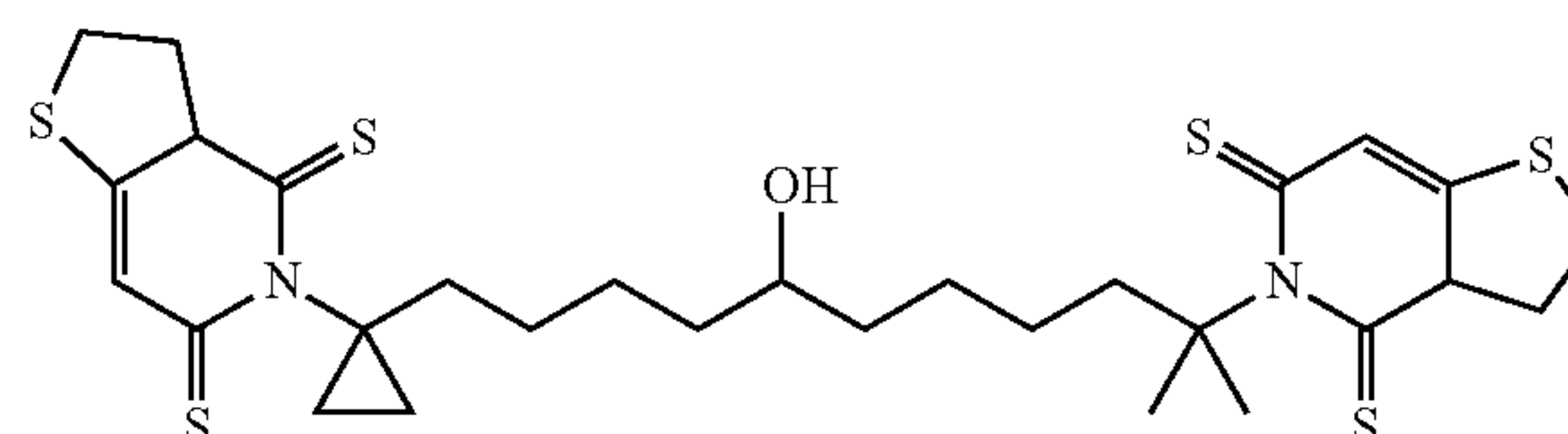
2,12-Bis-(4,6-dithio-2,3,3a,6-tetrahydro-4H-thieno[3,2-c]pyridin-5-yl)-2-methyl-12-(cyclopropyl)-7-hydroxy-dodecane
