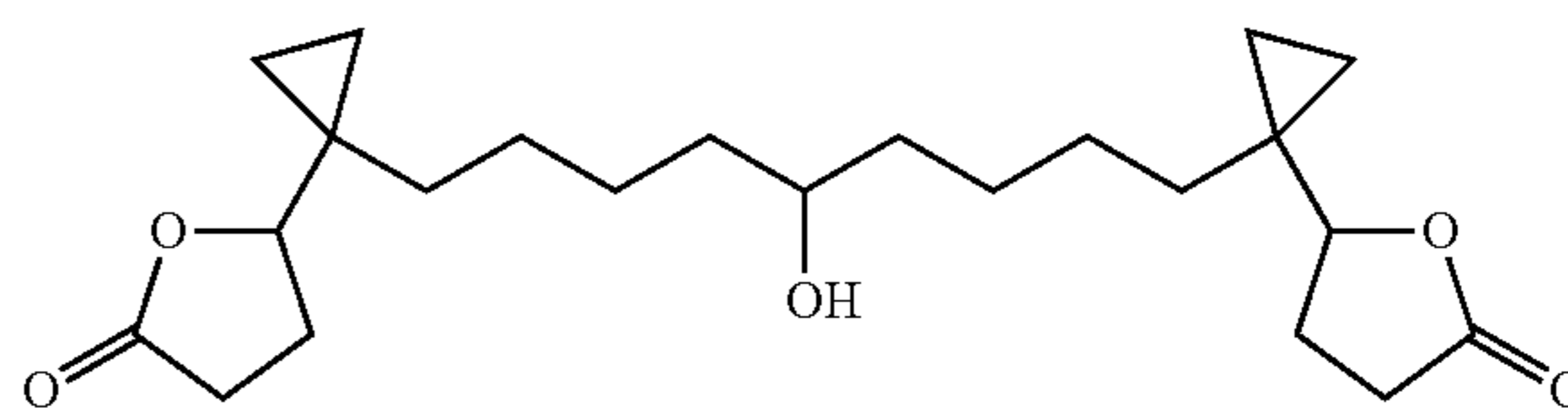
1,9-Bis-[1-(2-oxo-tetrahydrofuran-5-yl)-cyclopropyl]-nonan-5-ol
