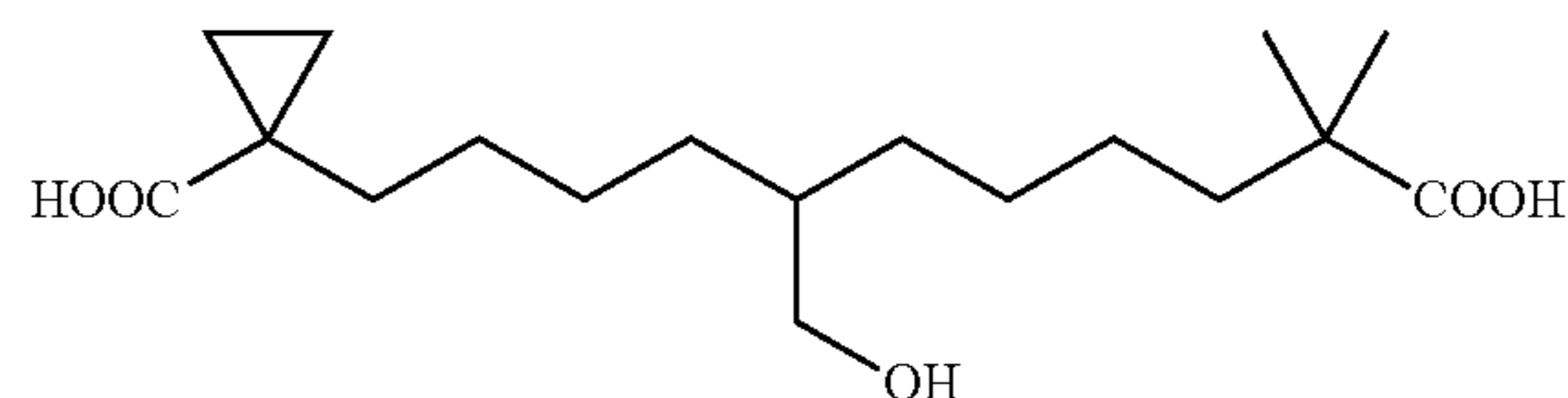
1-(1,0-Carboxy-5-hydroxymethyl-10-methyl-undecyl)-cyclopropanecarboxylic acid
