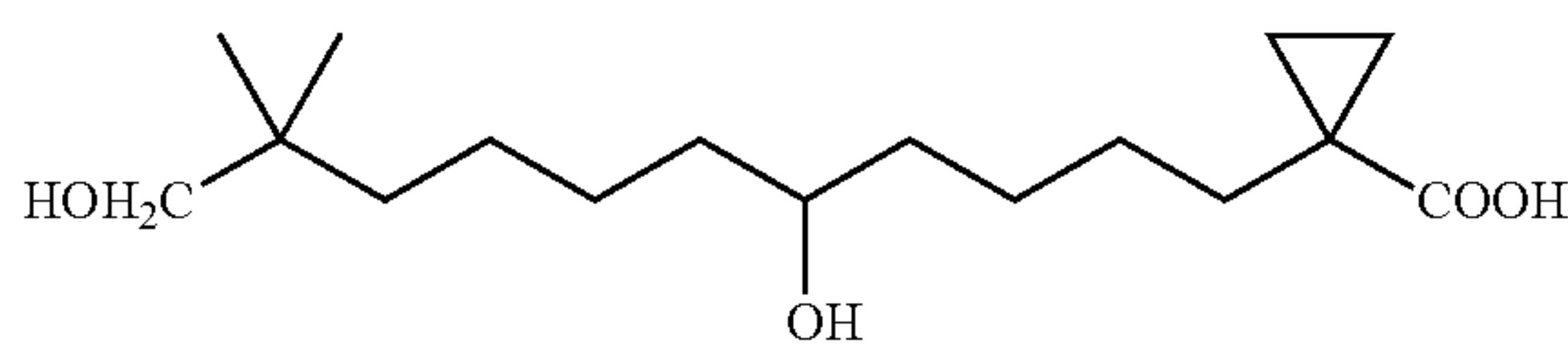
1-(5,11-Dihydroxy-10,10-dimethyl-undecyl)-cyclopropanecarboxylic acid
