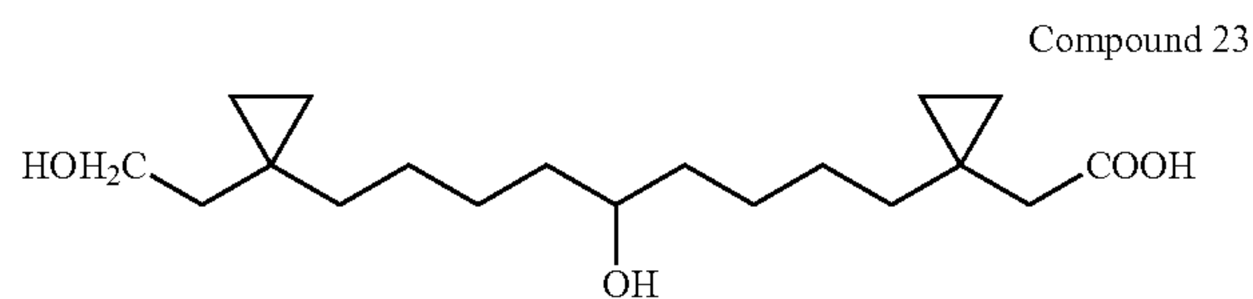
(1-{5-Hydroxy-9-[1-(2-hydroxy-ethyl)-cyclopropyl]-nonyl}-cyclopropyl)-acetic acid
