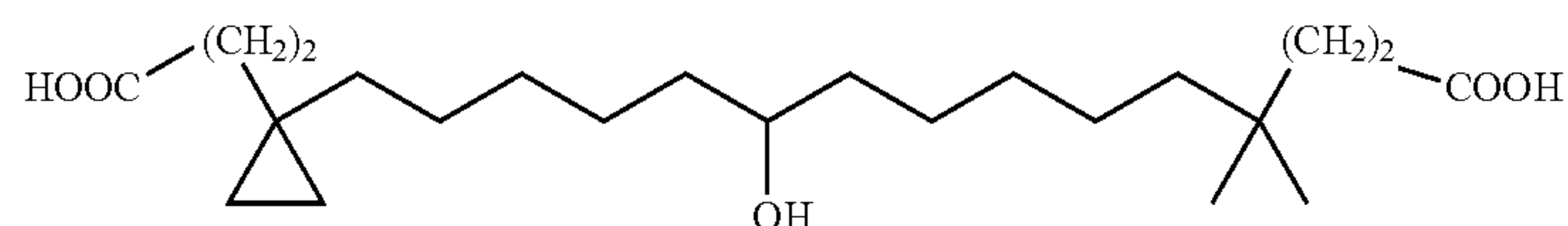
15-[1-(2-Carboxyethyl)-cyclopropyl]-10-hydroxy-4,4-dimethyl-tridecanoic acid
