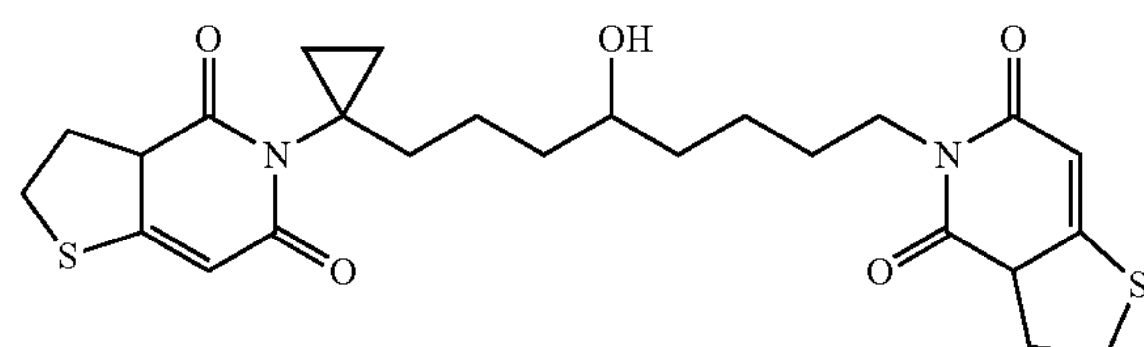
1,7-Bis-(4,6-dioxo-2,3,3a,6-tetrahydro-4H-thieno[3,2-c]pyridin-5-yl)-1-(cyclopropyl)-6-hydroxy-heptane
