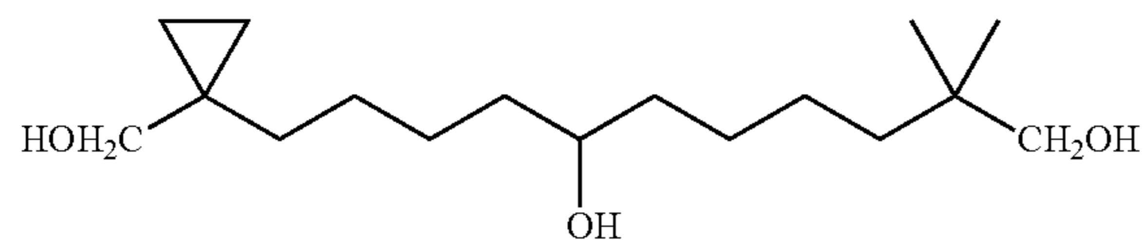
11-(1-Hydroxymethyl-cyclopropyl)-2,2-dimethyl-undecane-1,7-diol
