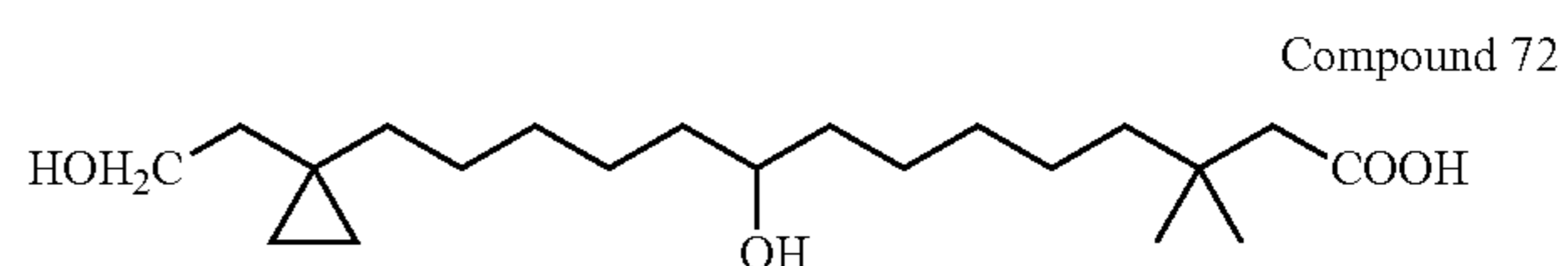
9-Hydroxy-14-[1-(2-hydroxy-ethyl)-cyclopropyl]-3,3-dimethyl-tetradecanoic acid
