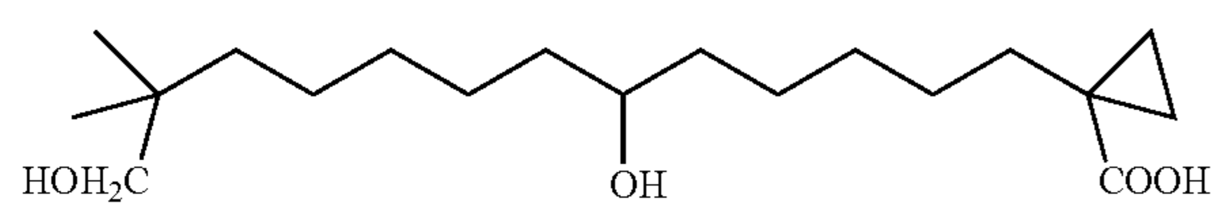
1-(6,13-Dihydroxy-12,12-dimethyl-tridecyl)-cyclopropanecarboxylic acid
