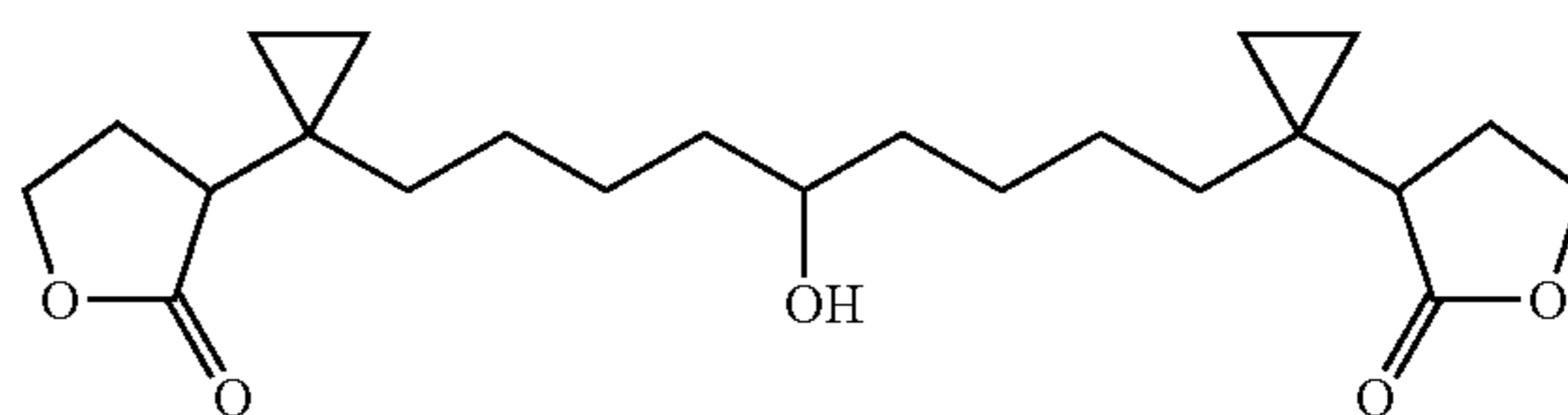
1,9-Bis-[1-(2-oxo-tetrahydrofuran-3-yl)-cyclopropyl]-nonan-5-ol
