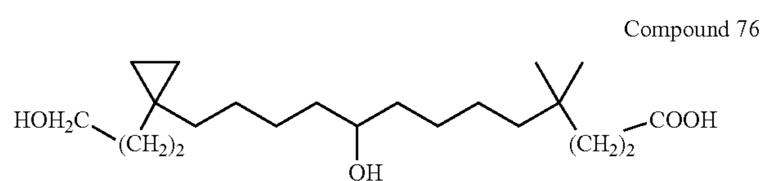
4,4-Dimethyl-9-hydroxy-13-[1-(3-hydroxypropyl)-cyclopropyl]-tridecanoic acid
