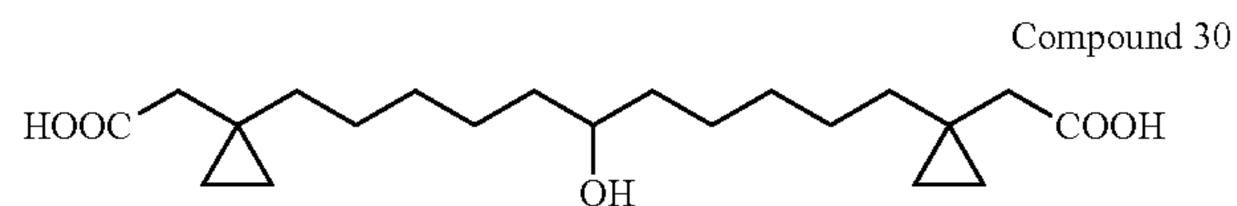
{1-11-(1-Carboxymethyl-cyclopropyl)-6-hydroxy-undecyl)-cyclopropyl}-acetic acid
