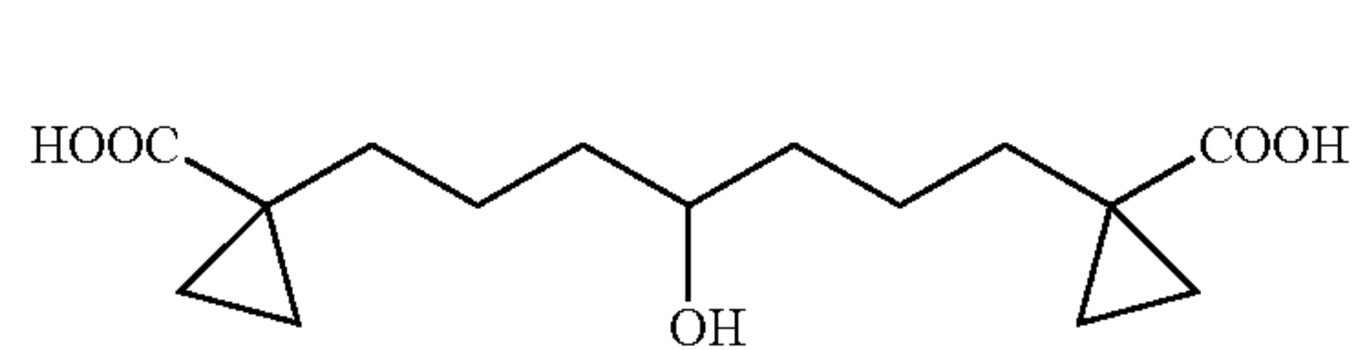
1,7-Bis-(1-carboxy-cyclopropyl)-heptan-4-ol
