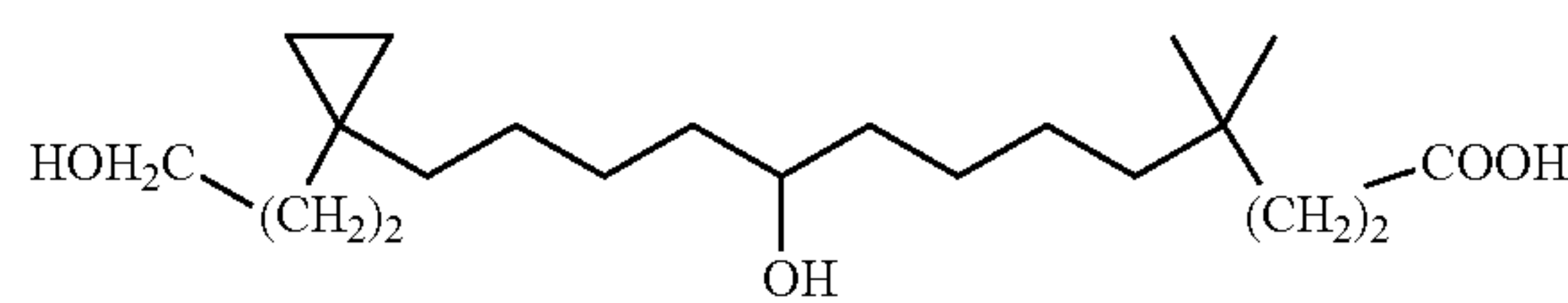
4,4-Dimethyl-9-hydroxy-13-[1-(3-hydroxypropyl)-cyclopropyl]-tridecanoic acid
