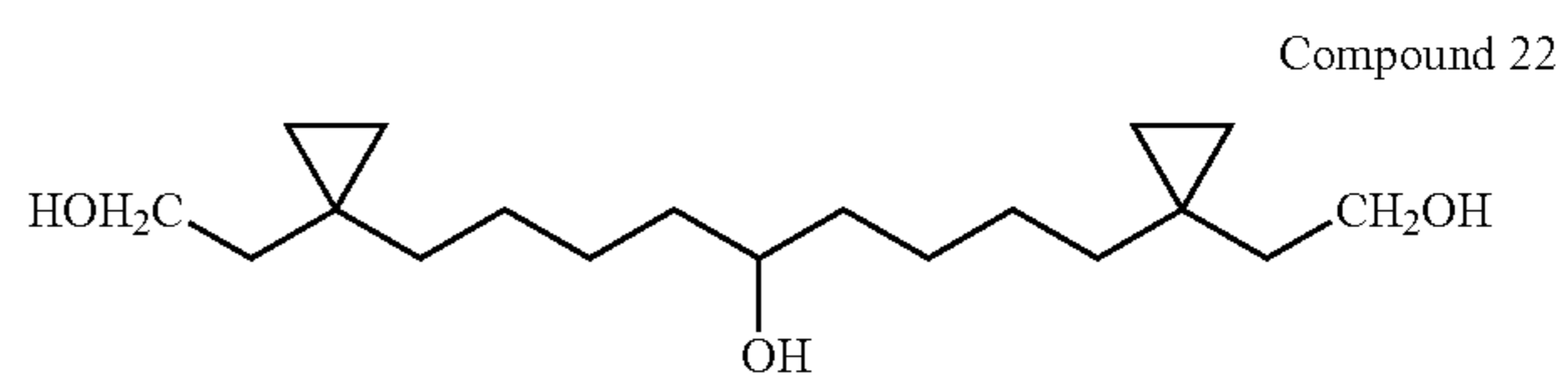
1,9-Bis-[1-(2-hydroxy-ethyl)-cyclopropyl]-nonan-5-ol
