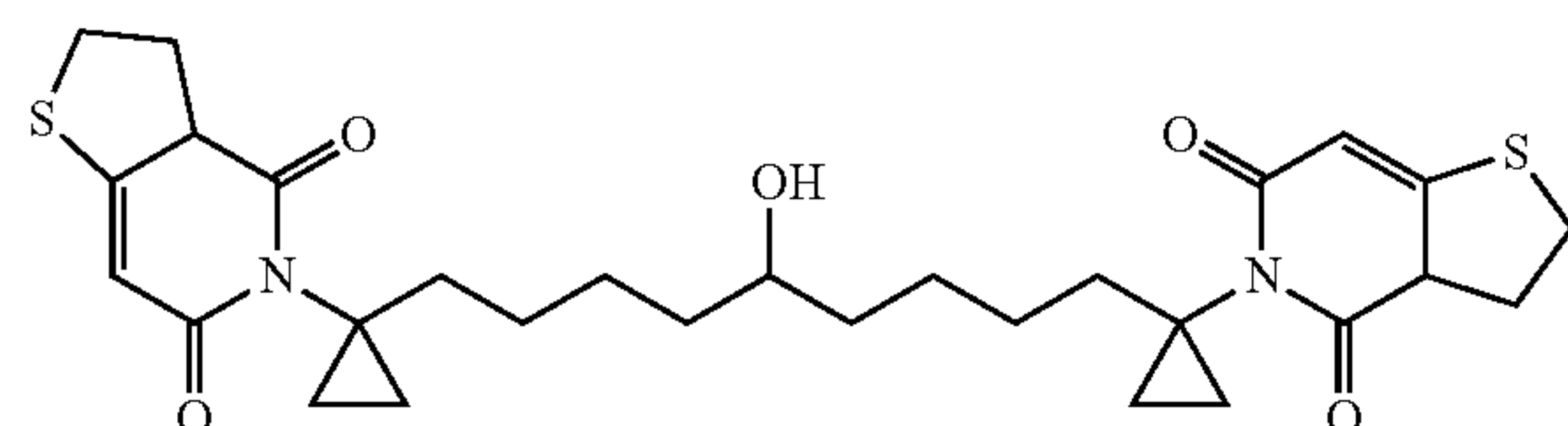
2,9-Bis-(4,6-dioxo-2,3,3a,6-tetrahydro-4H-thieno[3,2-c]pyridin-5-yl)-2,9-bis-(cyclopropyl)-5-hydroxy-nonane
