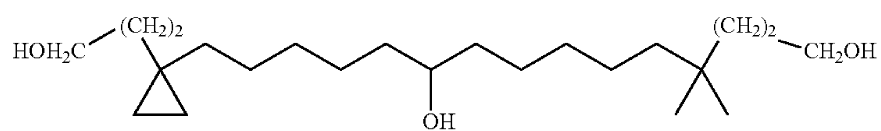
15-[1-(3-Hydroxy-propyl)-cyclopropyl]-4,4-dimethyl-pentadecane-1,10-diol
