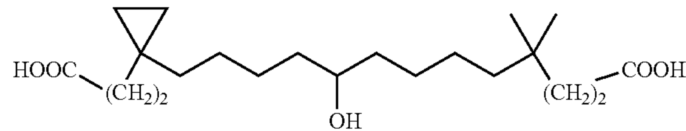
13-[1-(2-Carboxyethyl)-cyclopropyl]-9-hydroxy-4,4-dimethyl-tridecanoic acid
