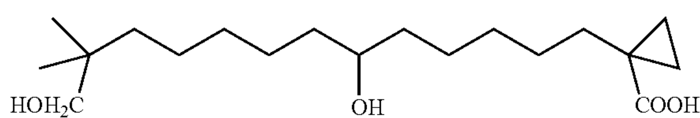
1-(6,13-Dihydroxy-12,12-dimethyl-tridecyl)-cyclopropanecarboxylic acid
