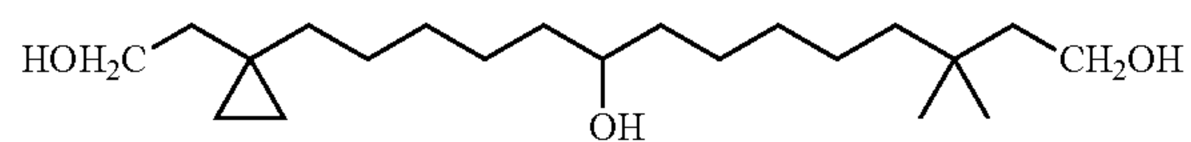
14-[1-(2-Hydroxy-ethyl)-cyclopropyl]-3,3-dimethyl-tetradecane-1,9-diol
