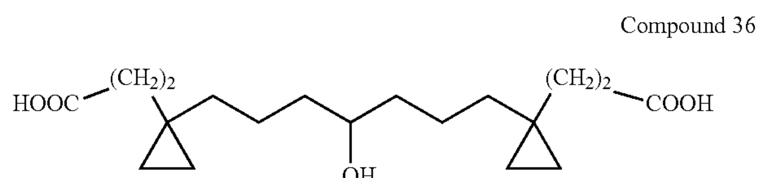
3-(1-{7-[1-(2-Carboxy-ethyl)-cyclopropyl]-4-hydroxy-heptyl}-cyclopropyl)-propionic acid
