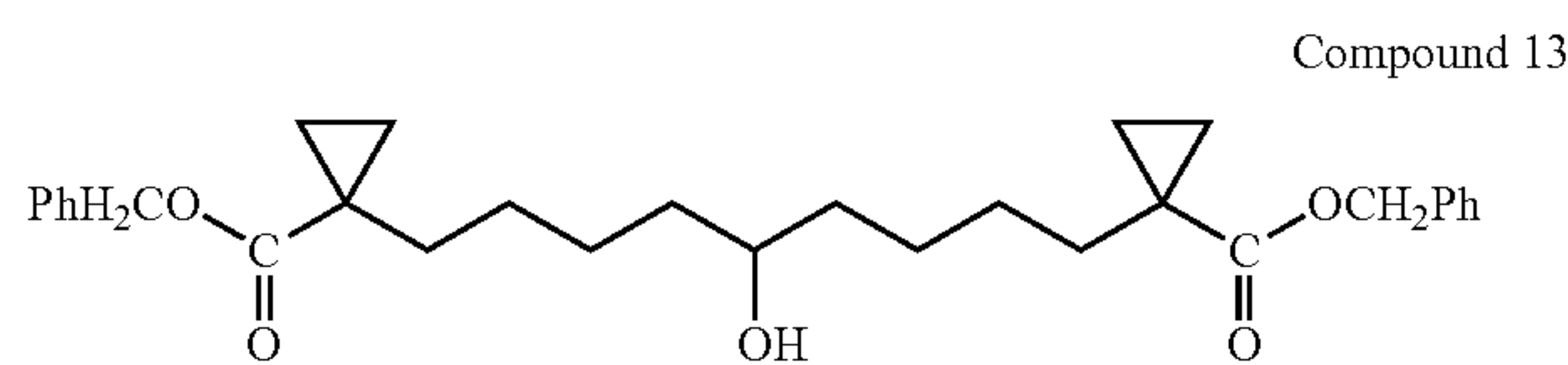
1,9-Bis-(1-benzyloxycarbonyl-cyclopropyl)-nonan-5-ol
