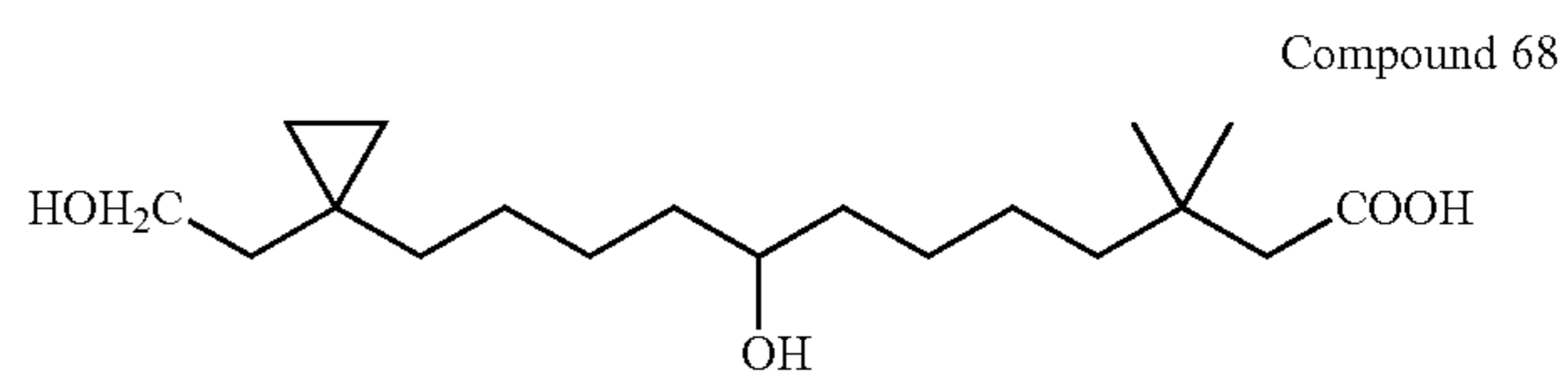
8-Hydroxy-12-[1-(2-hydroxy-ethyl)-cyclopropyl]-3,3-dimethyl-dodecanoic acid
