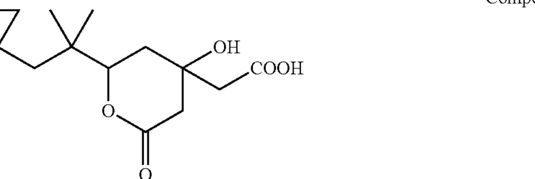
1,9-Bis {1-[9-(4-carboxymethyl-4-hydroxy-6-oxo-tetrahydro-pyran-2-yl)-(cyclopropyl)]}-5-hydroxy-nonane
