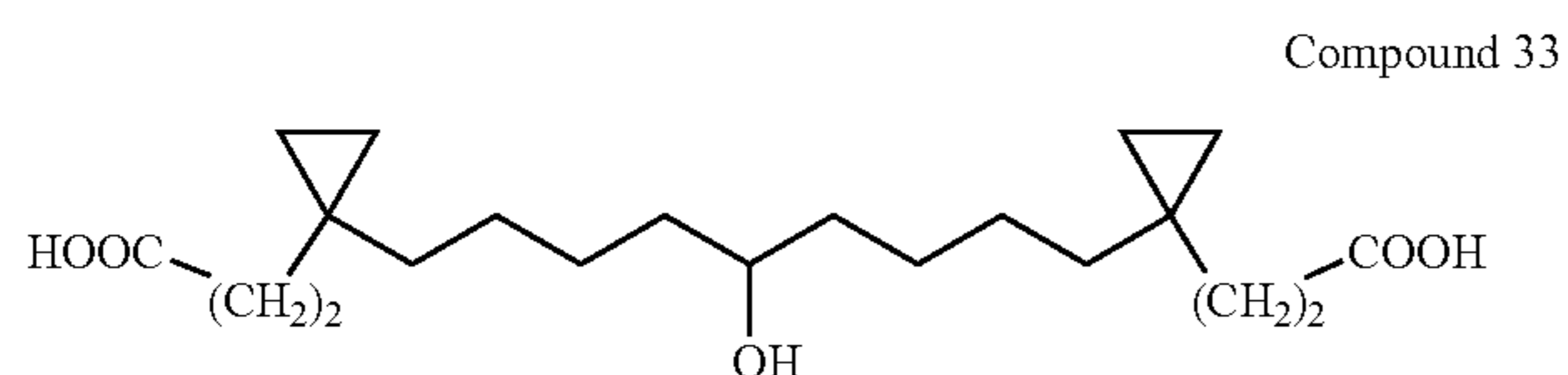
3-(1-{9-[1-(3-Carboxy-ethyl)-5-hydroxy-cyclopropyl]-nonyl}-cyclopropyl)-propionic acid
