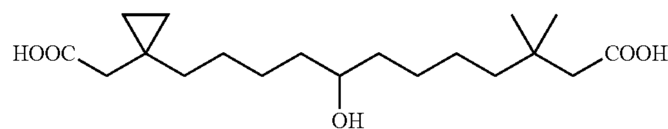
12-(1-Carboxymethyl-cyclopropyl)-8-hydroxy-3,3-dimethyl-dodecanoic acid
