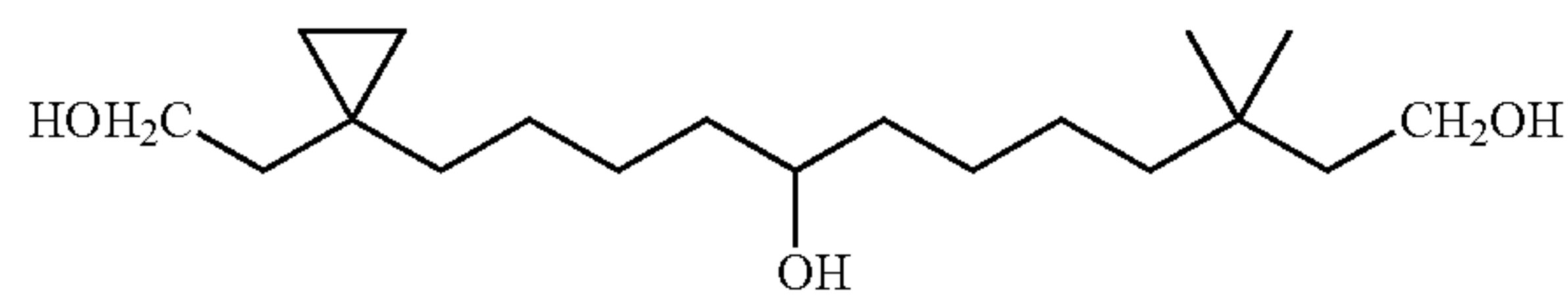
12-[1-(2-Hydroxy-ethyl)-cyclopropyl]-3,3-dimethyl-dodecane-1,8-diol
