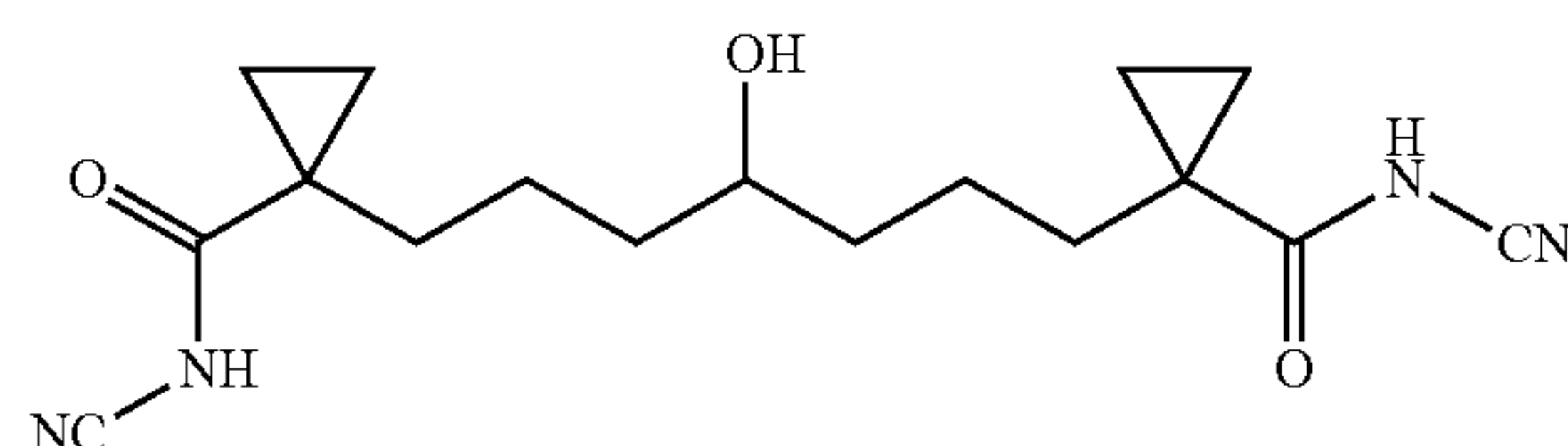
1,7-Bis-(1-dicyanimido-cyclopropyl)-4-hydroxy-heptane
