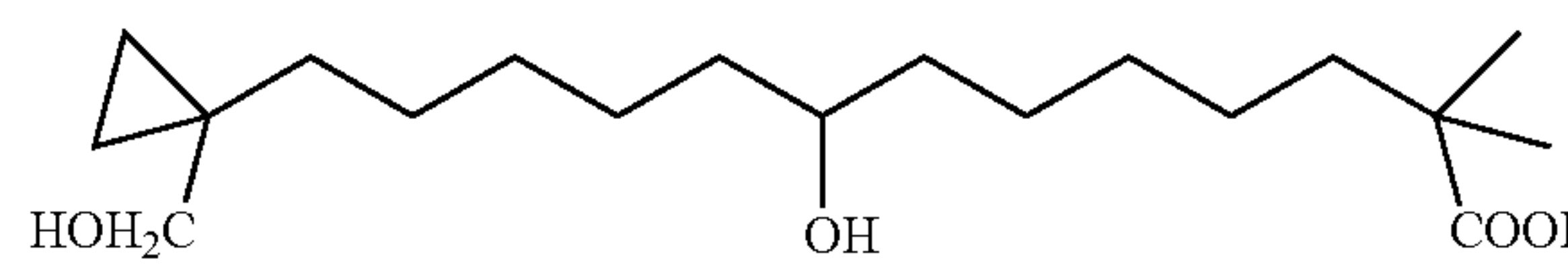
8-Hydroxy-13-(1-hydroxymethyl-cyclopropyl)-2,2-dimethyl-tridecanoic acid
