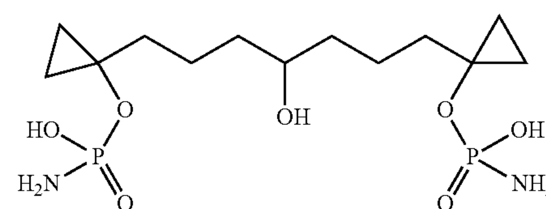
1,7-Bis-(1-phosponamid-cyclopropyl)-4-hydroxy-heptane
