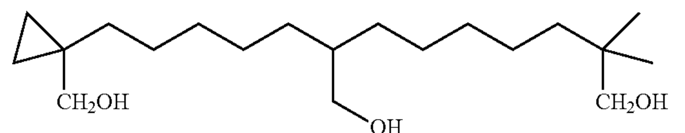
8-[5-(1-Hydroxymethyl-cyclopropyl)-pentyl]-2,2-dimethyl-nonane-1,9-diol
