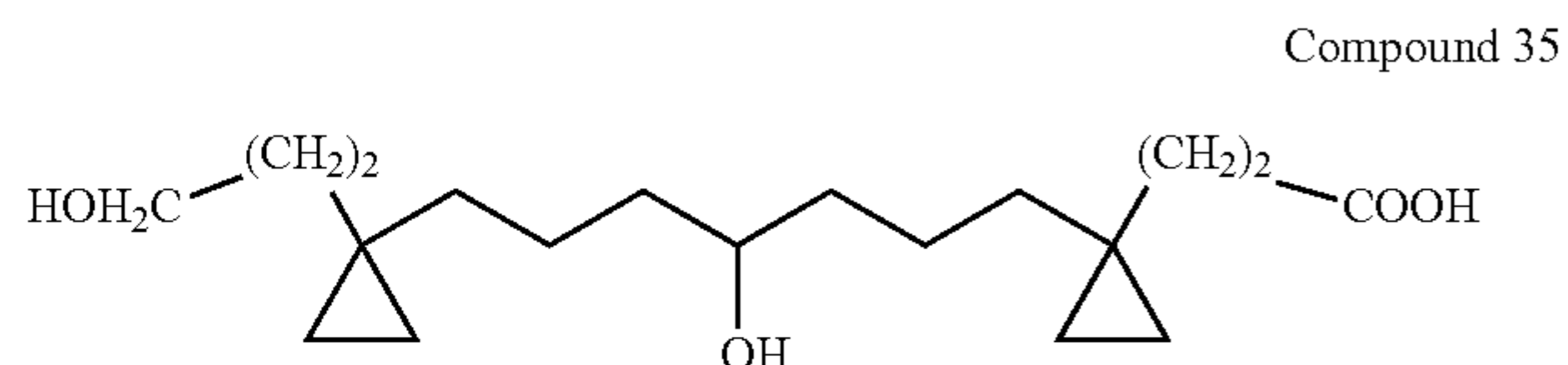
3-(1-{4-Hydroxy-7-[1-(3-hydroxy-propyl)-cyclopropyl]-heptyl}-cyclopropyl)-propionic acid
