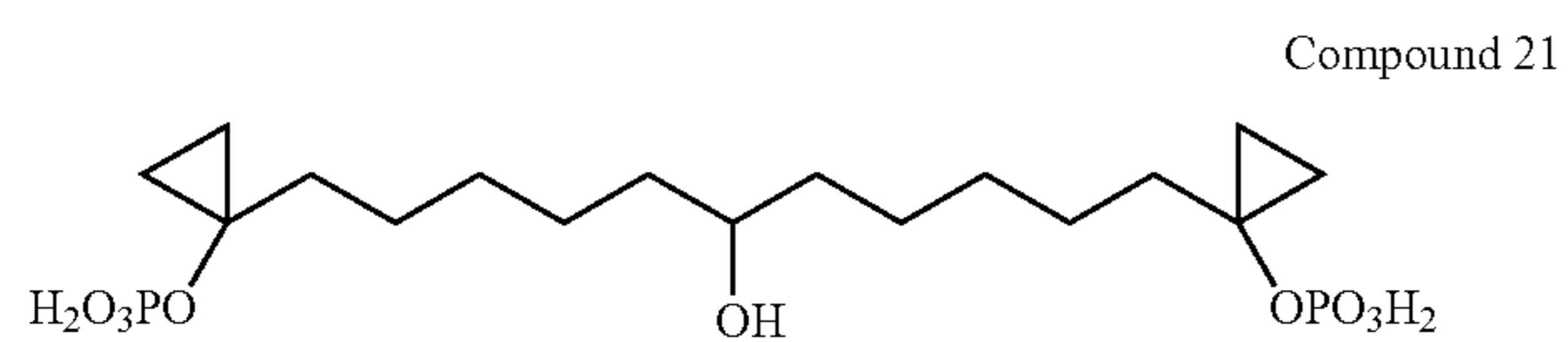
1,9-Bis-(1-phosphonoxy-cyclopropyl)-nonan-5-ol
