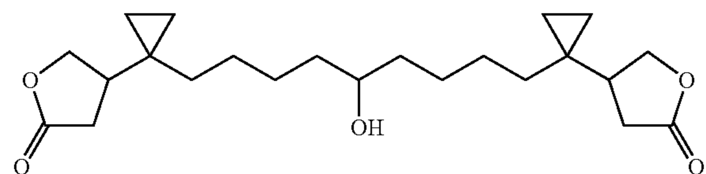
1,9-Bis-[1-(2-oxo-tetrahydrofuran-4-yl)-cyclopropyl]-nonan-5-ol
