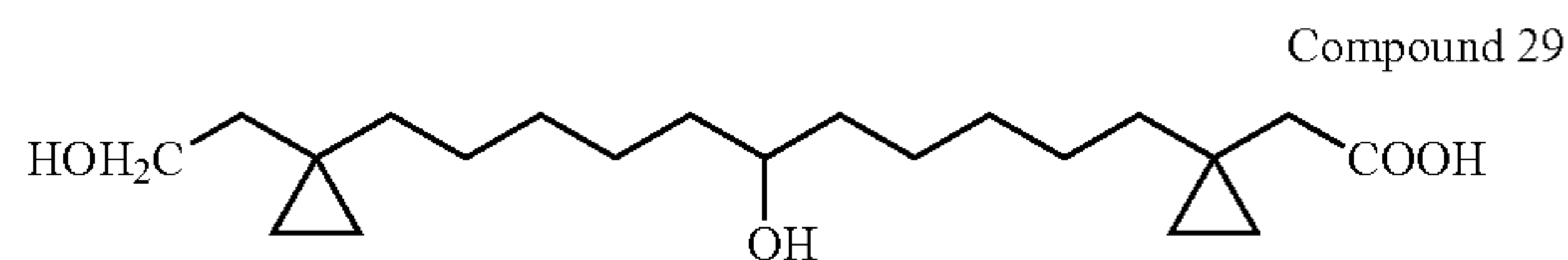
(1-{6-Hydroxy-11-[1-(2-hydroxy-ethyl)-cyclopropyl]-undecyl}-cyclopropyl)-acetic acid
