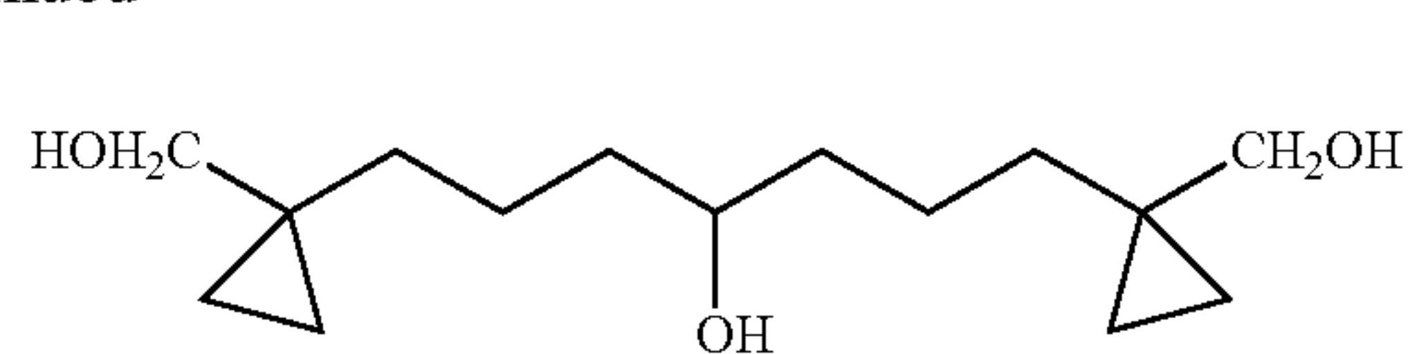
1,7-Bis-(1-hydroxymethyl-cyclopropyl)-heptan-4-ol
