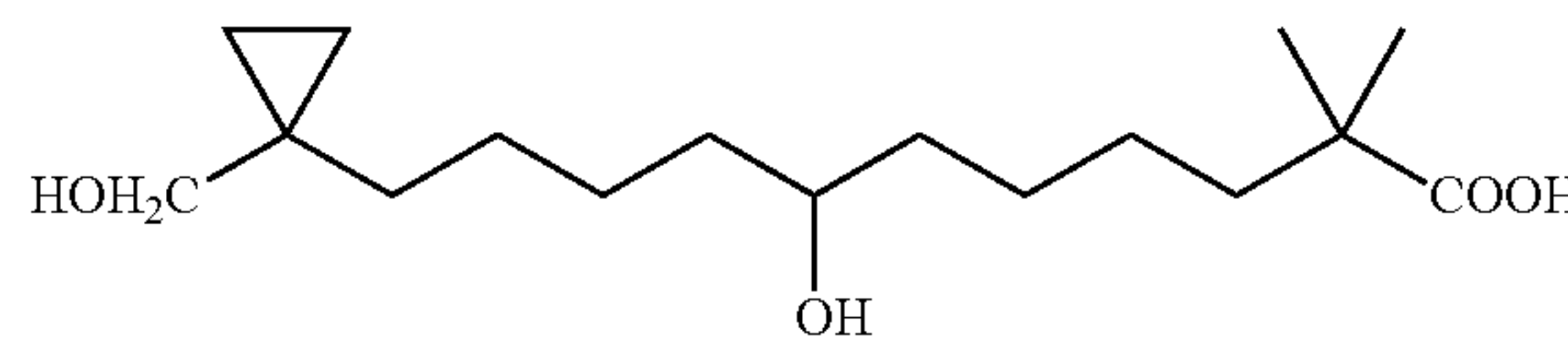
7-Hydroxy-11-(1-hydroxymethyl-cyclopropyl)-2,2-dimethyl-undecanoic acid
