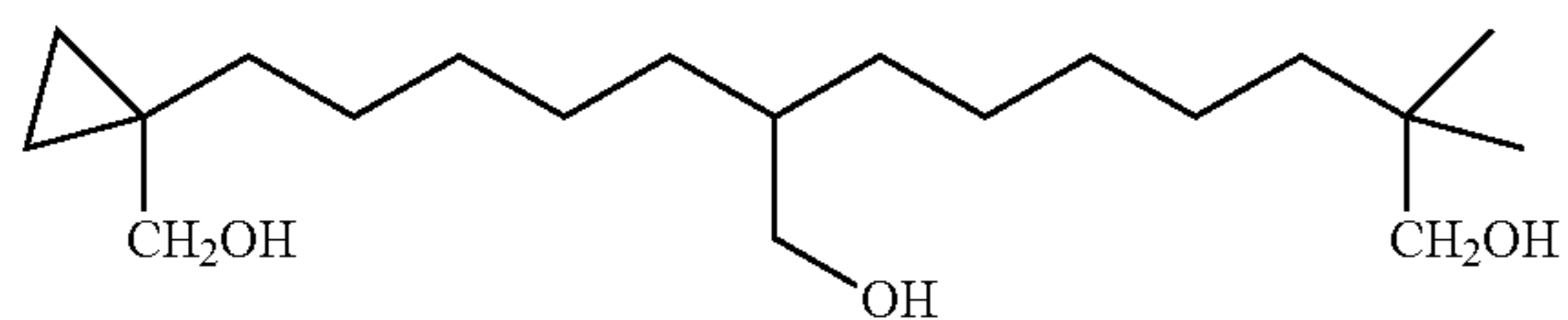
8-[5-(1-Hydroxymethyl-cyclopropyl)-pentyl]-2,2-dimethyl-nonane-1,9-diol
