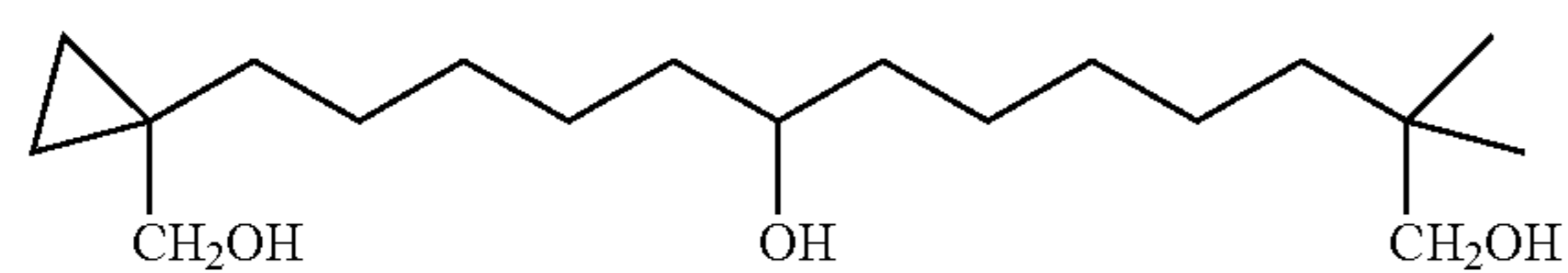
13-(1-Hydroxymethyl-cyclopropyl)-2,2-dimethyl-tridecane-1,8-diol
