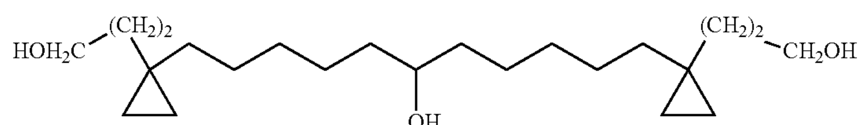
1,11-Bis-[1-(3-hydroxy-propyl)-cyclopropyl]-undecan-6-ol
