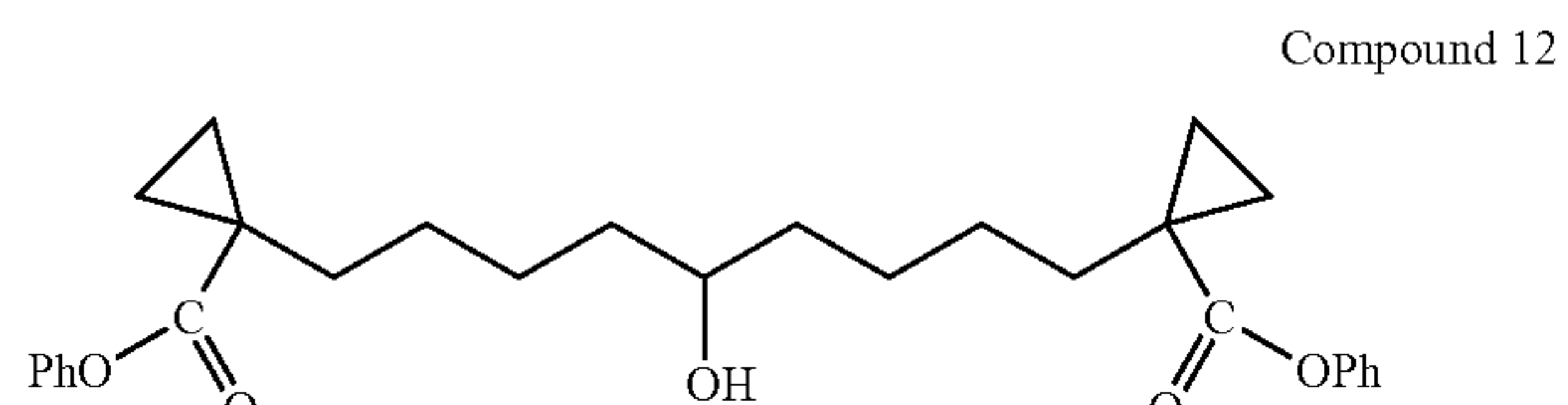
1,9-Bis-(1-phenoxy-carbonyl-cyclopropyl)-nonan-5-ol
