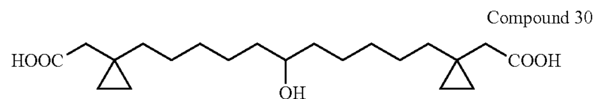
{1-11-(1-Carboxymethyl-cyclopropyl)-6-hydroxy-undecyl}-cyclopropyl}-acetic acid
