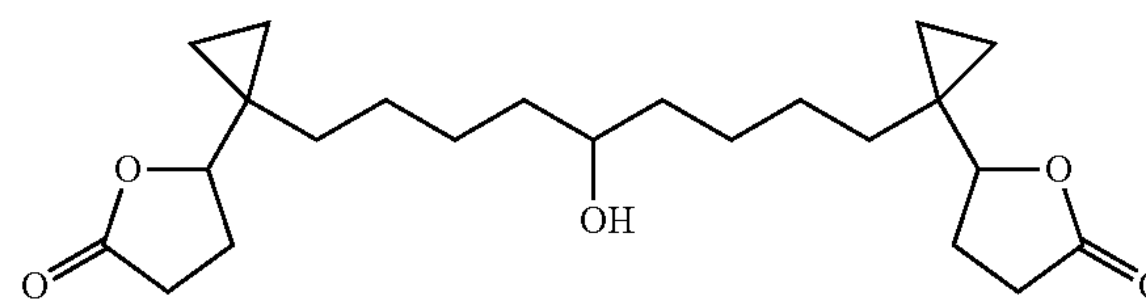
1,9-Bis-[1-(2-oxo-tetrahydrofuran-5-yl)-cyclopropyl]-nonan-5-ol
