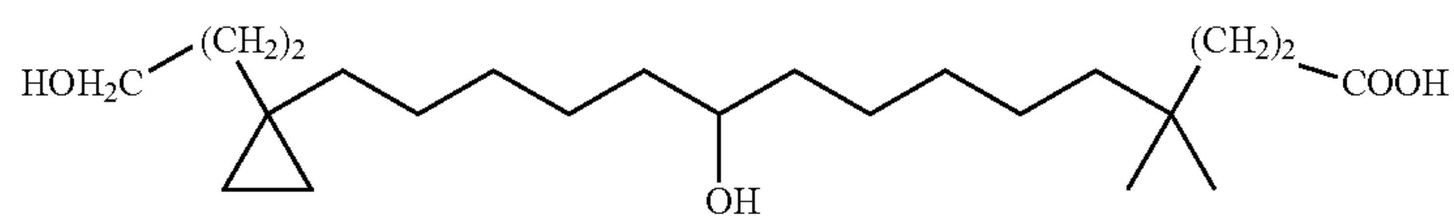
4,4-Dimethyl-10-hydroxy-15-[1-(3-hydroxy-propyl)-cyclopropyl]-pentadecanoic acid
