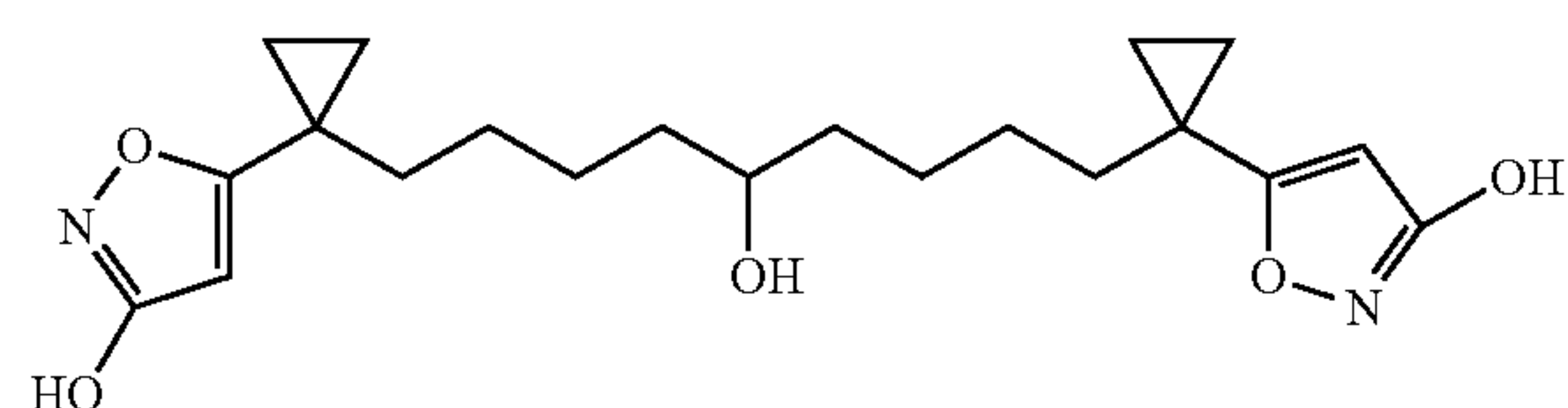
1,9-Bis-[1-(3-hydroxy-isoxazol-5-yl)-cyclopropyl]-nonan-5-ol
