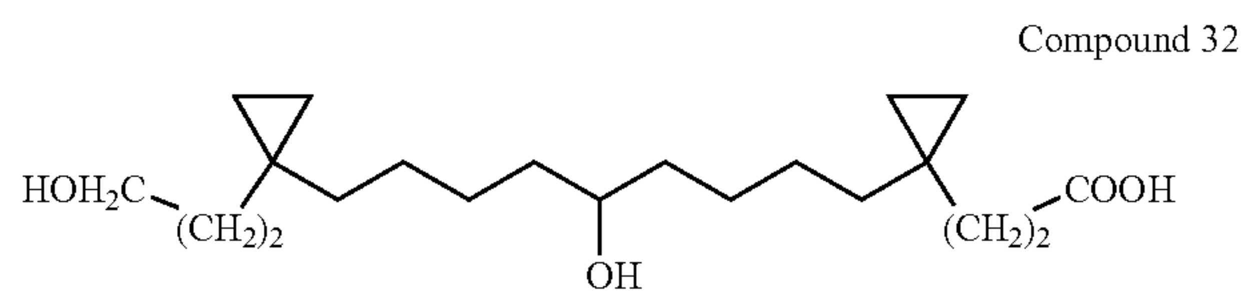
3-(1-{5-Hydroxy-9-[1-(3-hydroxy-propyl)-cyclopropyl]-nonyl}-cyclopropyl)-propionic acid
