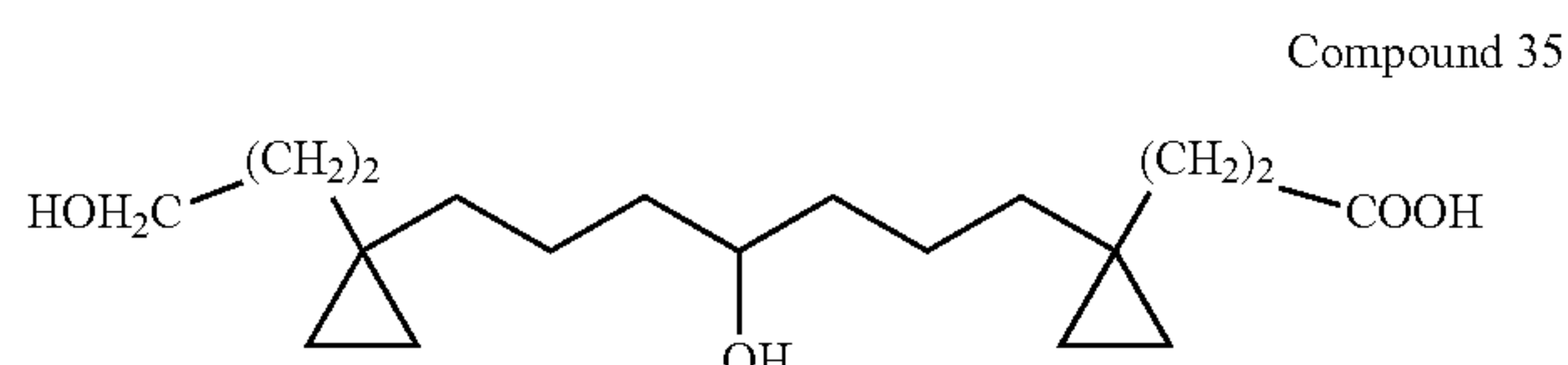
3-(1-{4-Hydroxy-7-[1-(3-hydroxy-propyl)-cyclopropyl]-heptyl}-cyclopropyl)-propionic acid
