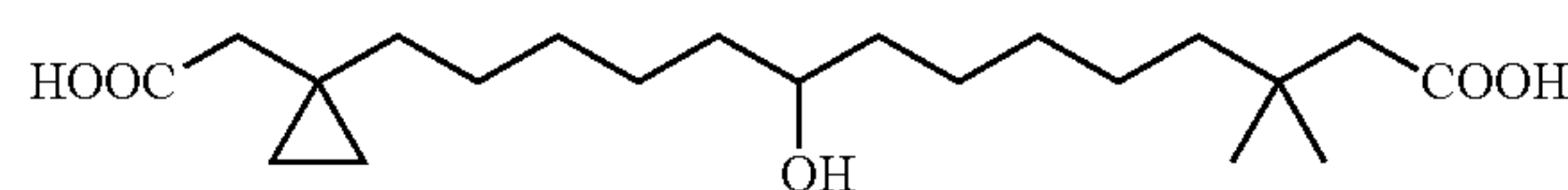
14-(1-Carboxymethyl-cyclopropyl)-9-hydroxy-3,3-dimethyl-tetradecanoic acid
