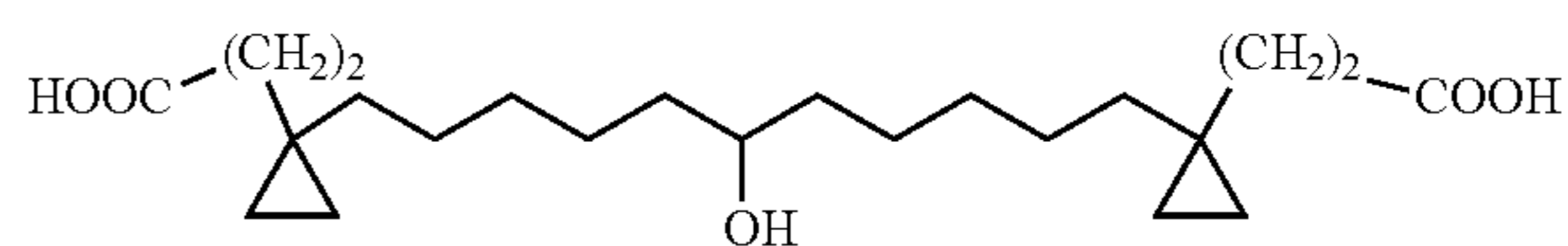
3-(1-(11-[1-(2-Carboxy-ethyl)-cyclopropyl]-6-hydroxy-undecyl)-cyclopropyl)-propionic acid
