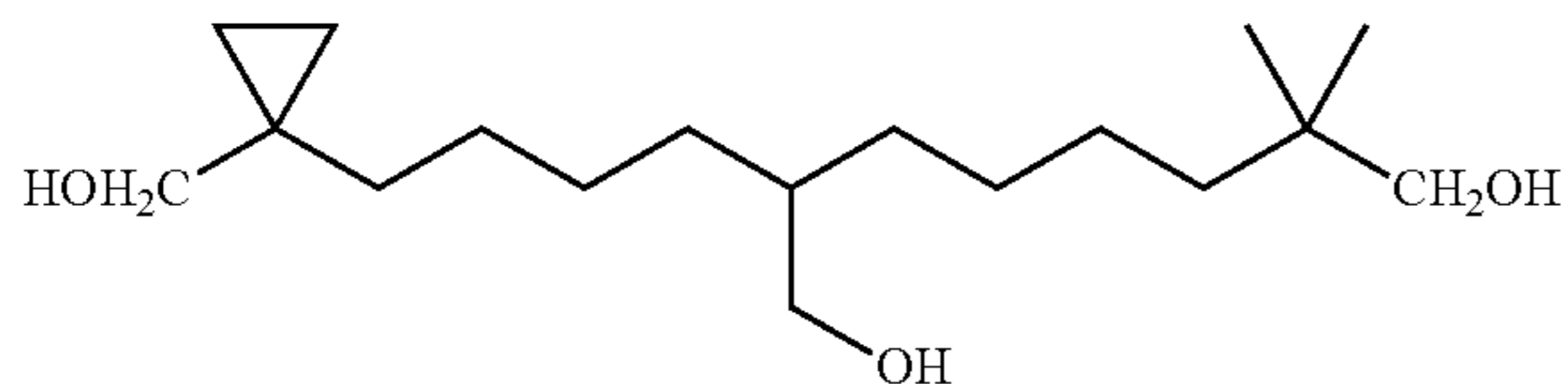
7-[4-(1-Hydroxymethyl-cyclopropyl)-butyl] 2,2-dimethyl-octane-1,8-diol
