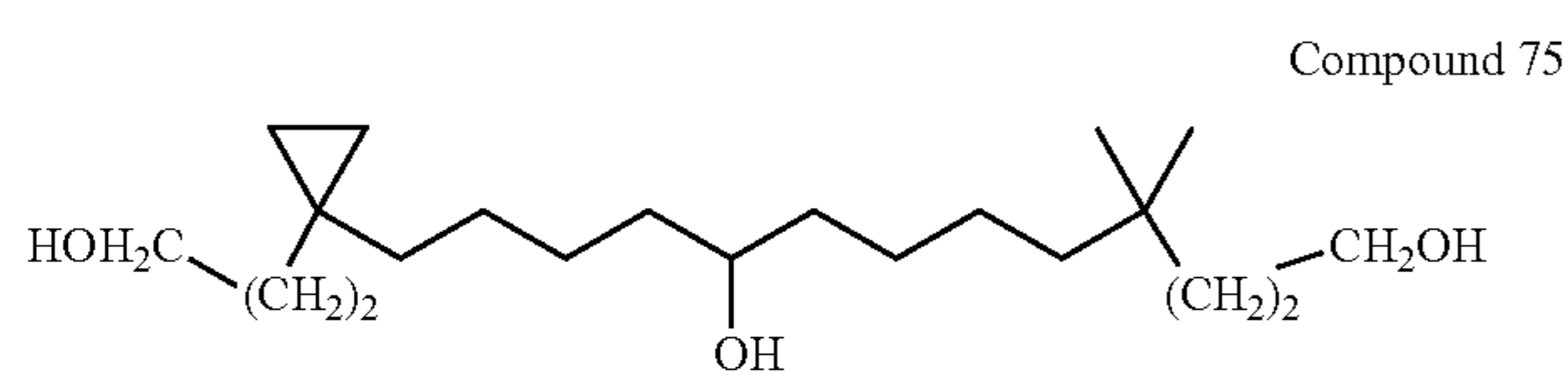
13-[1-(3-Hydroxy-propyl)-cyclopropyl]-4,4-dimethyl-tridecane-1,9-diol
