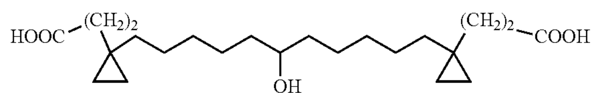
3-(1-(11-[1-(2-Carboxy-ethyl)-cyclopropyl]-6-hydroxy-undecyl)-cyclopropyl)-propionic acid
