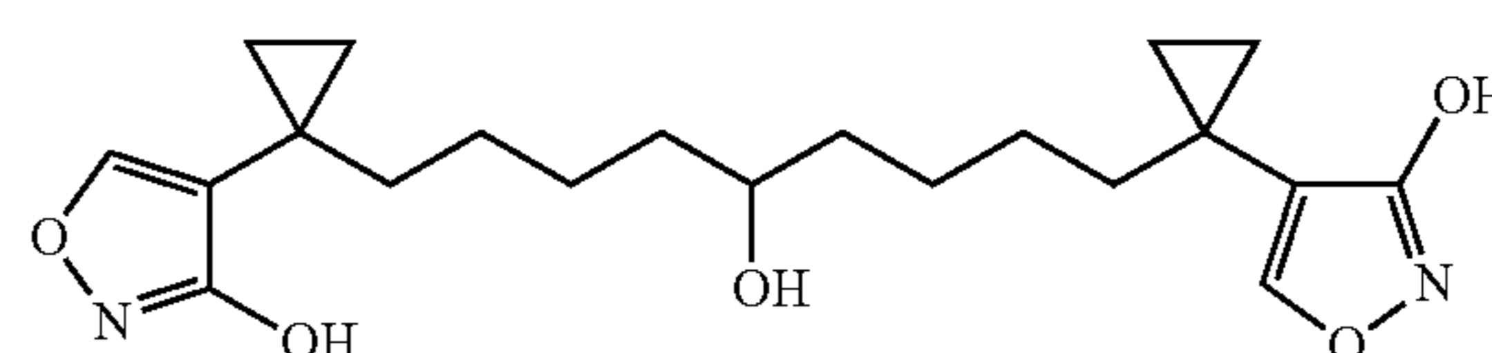
1,9-Bis-[1-(3-hydroxy-isoxazol-4-yl)-cyclopropyl]-nonan-5-ol
