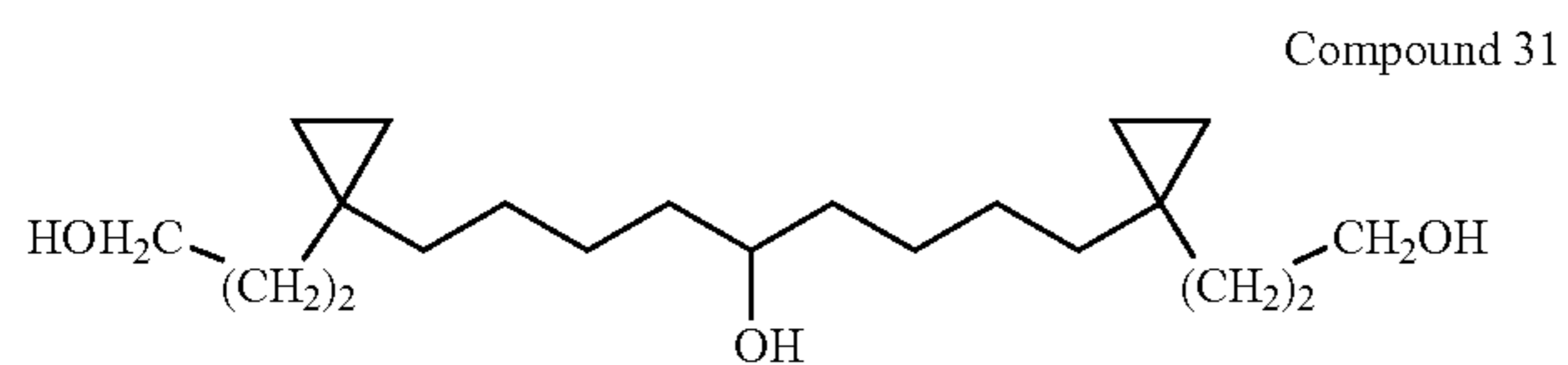
1,9-Bis-[1-(3-hydroxy-propyl)-cyclopropyl]-nonan-5-ol
