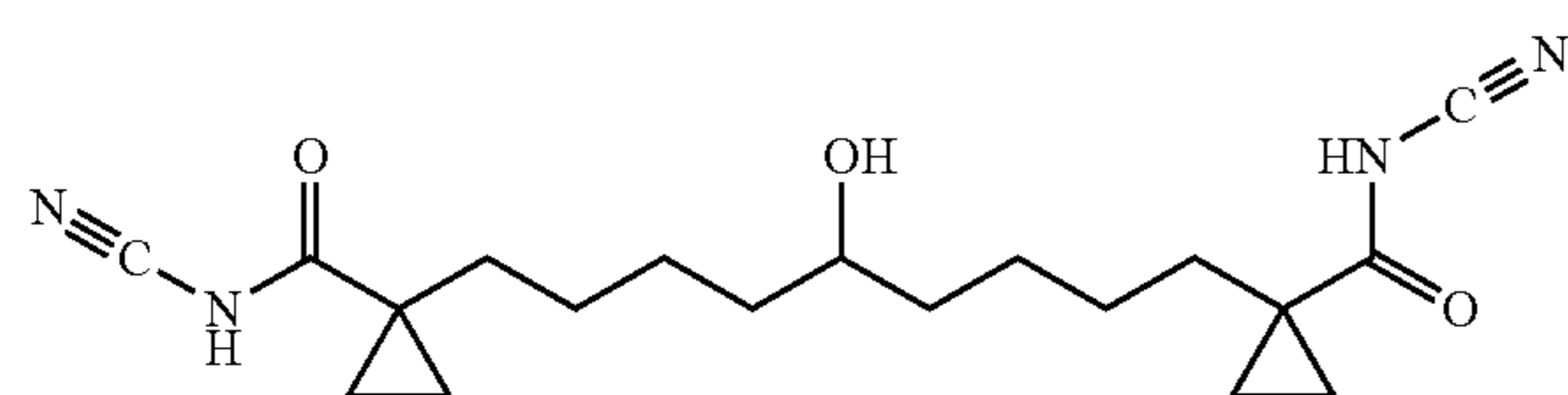
1,7-Bis-(1-dicyanimido-cyclopropyl)-5-hydroxy-nonane
