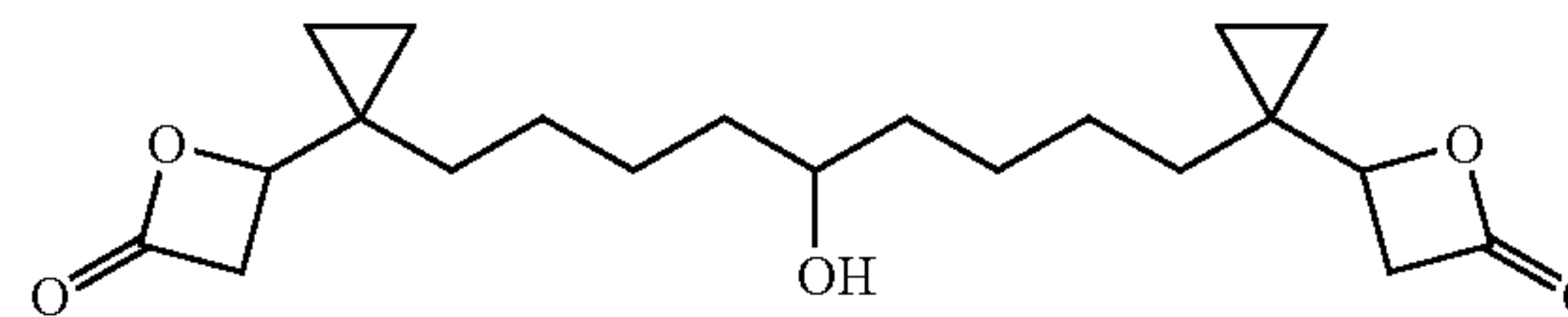
1,9-Bis-[1-(2-oxo-oxoethan-3-yl)-cyclopropyl]-nonan-5-ol
