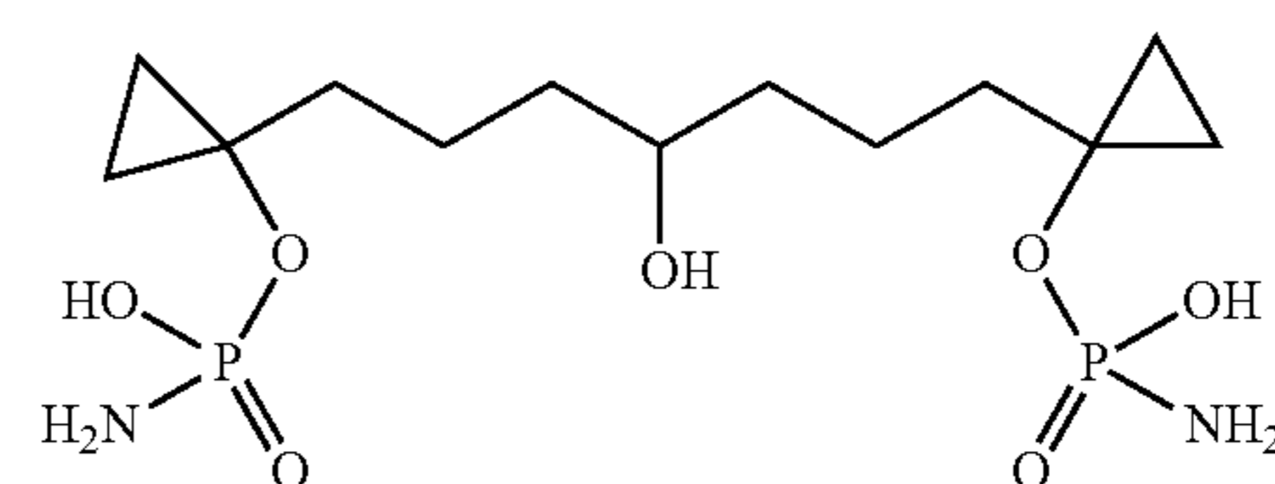
1,7-Bis-(1-phosponamid-cyclopropyl)-4-hydroxy-heptane
