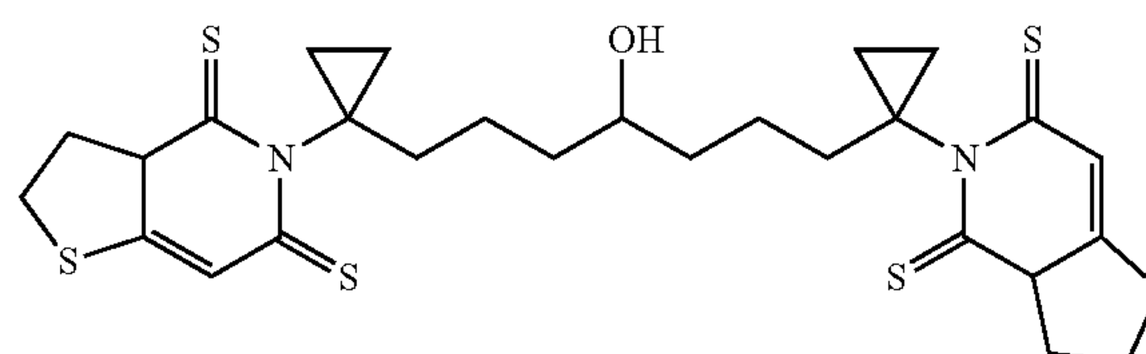
1,7-Bis-(4,6-dithio-2,3,3a,6-tetrahydro-4H-thieno[3,2-c]pyridin-5-yl)-1,7-bis-(cyclopropyl)-6-hydroxy-undecane
