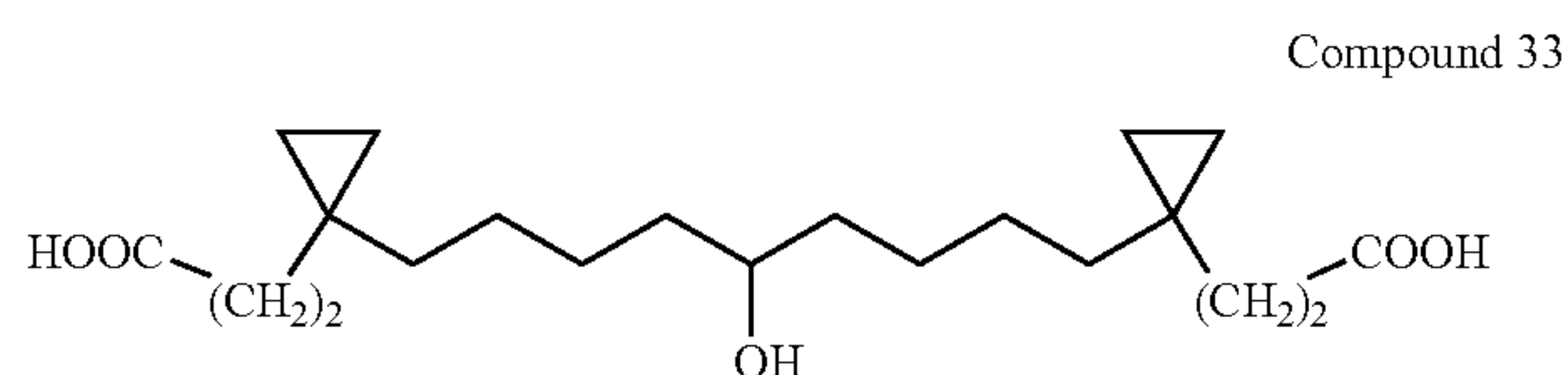
3-(1-{9-[1-(3-Carboxy-ethyl)-5-hydroxy-cyclopropyl]-nonyl}-cyclopropyl)-propionic acid
