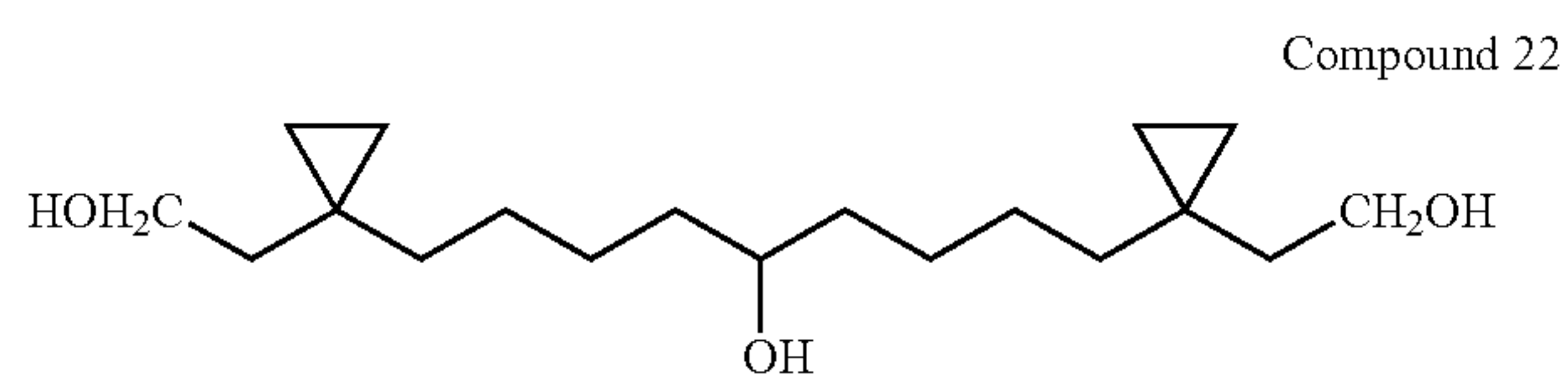
1,9-Bis-[1-(2-hydroxy-ethyl)-cyclopropyl]-nonan-5-ol
