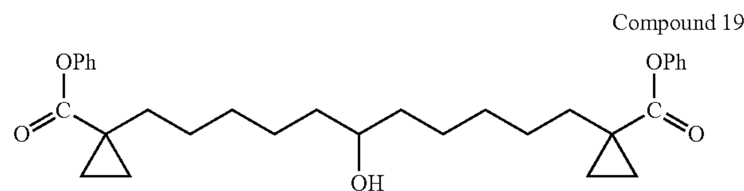
1,11-Bis-(1-phenoxy-carbonyl-cyclopropyl)-undecan-6-ol
