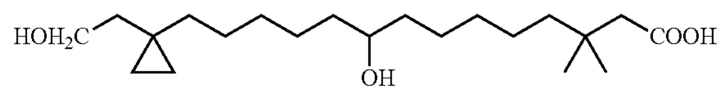
9-Hydroxy-14-[1-(2-hydroxy-ethyl)-cyclopropyl]-3,3-dimethyl-tetradecanoic acid
