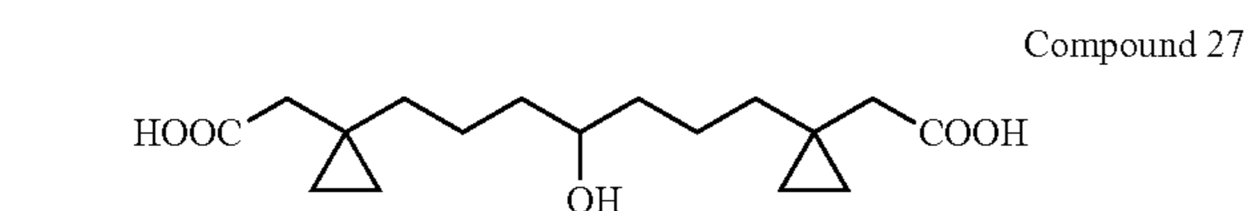
{1-[7-(1-Carboxymethyl-cyclopropyl)-4-hydroxy-heptyl]-cyclopropyl}-acetic acid
