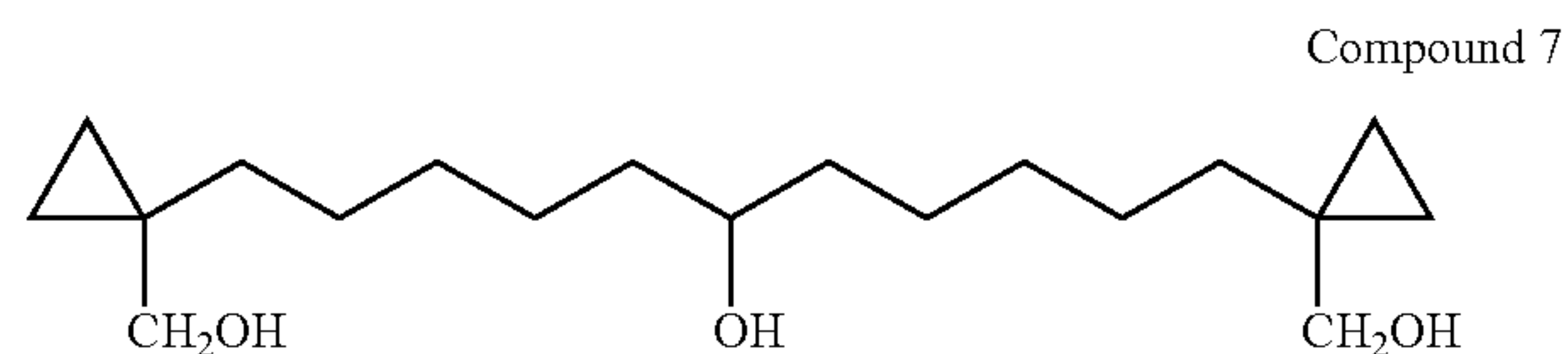
1,11-Bis-(1-hydroxymethyl-cyclopropyl)-undecan-6-ol
