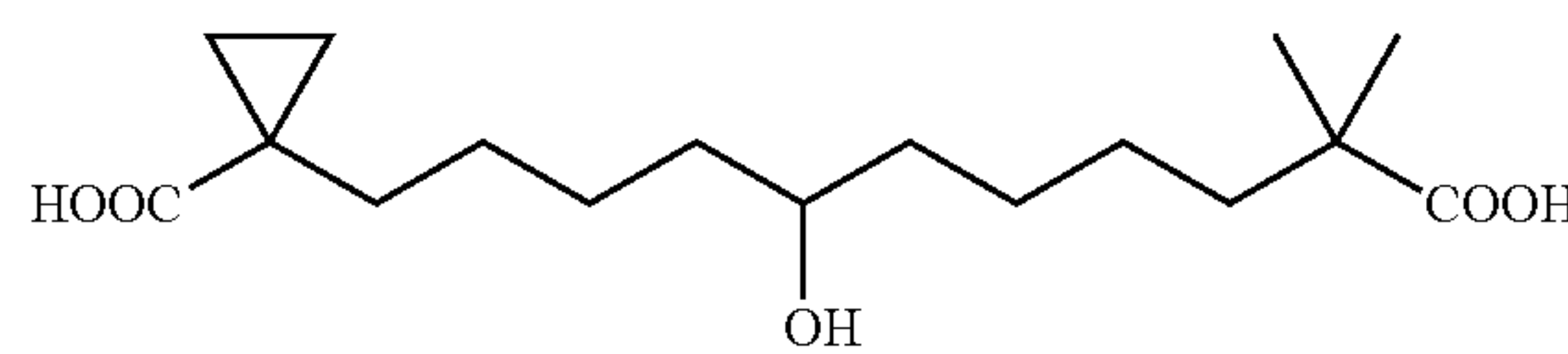
1-(10-Carboxy-5-hydroxy-10-methyl-undecyl)-cyclopropanecarboxylic acid
