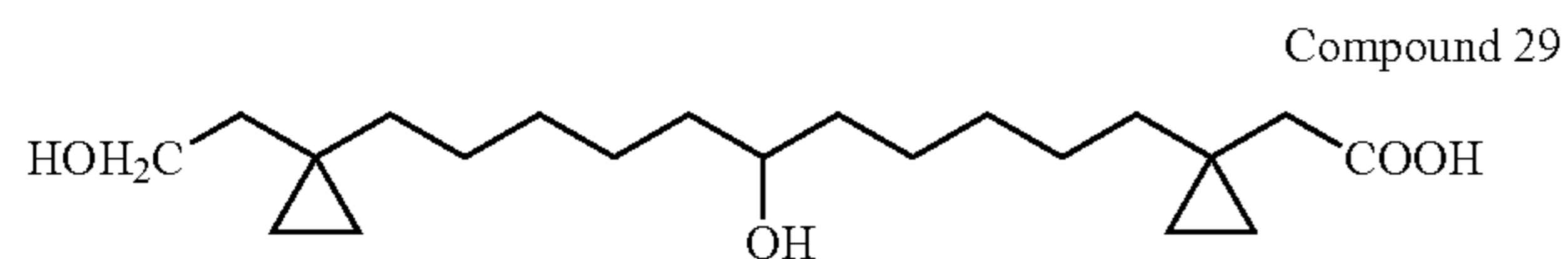
(1-{6-Hydroxy-11-[1-(2-hydroxy-ethyl)-cyclopropyl]-undecyl}-cyclopropyl)-acetic acid
