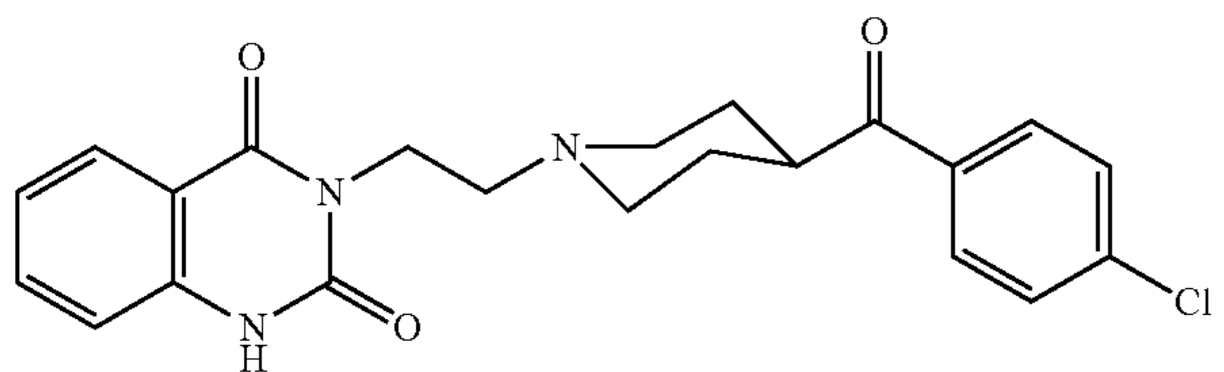
compound 12
