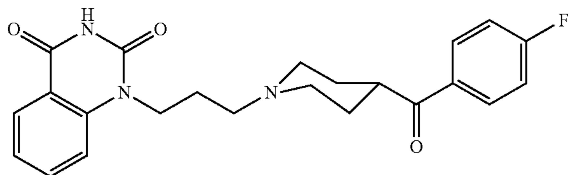
compound 12
