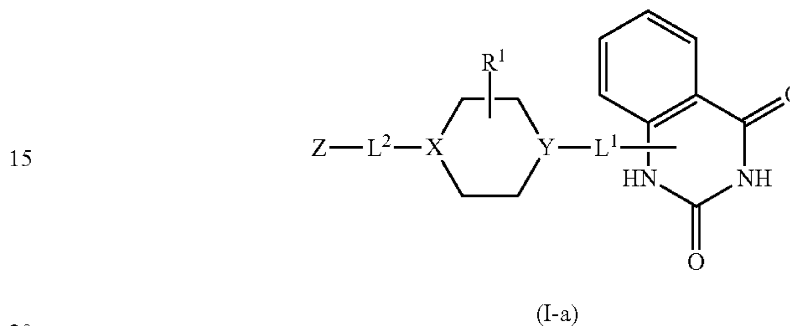
compound 1
