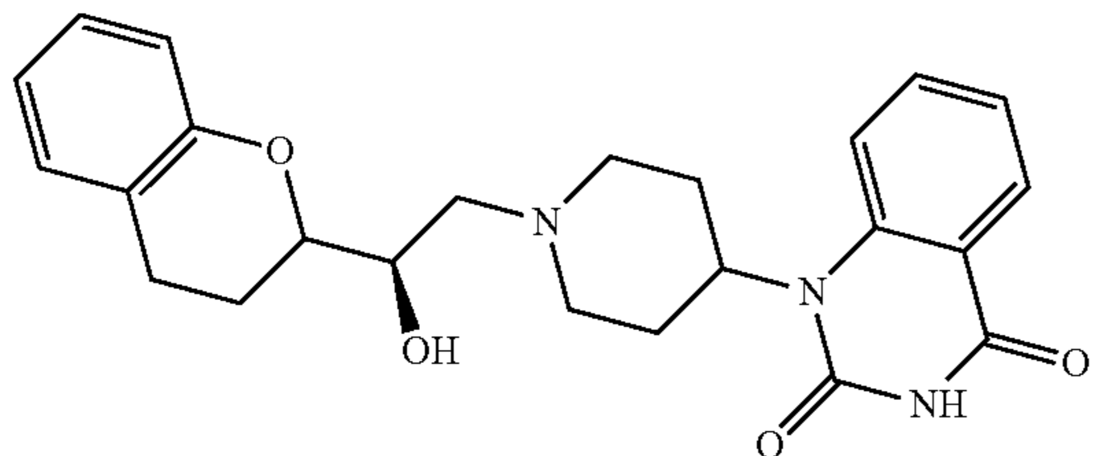
compound 9
