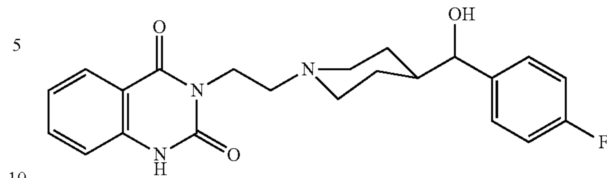
compound 9
