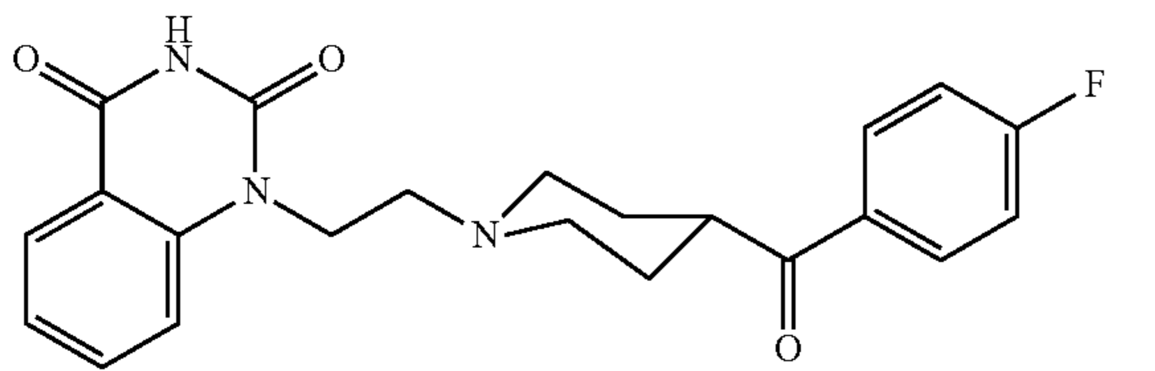
compound 11
