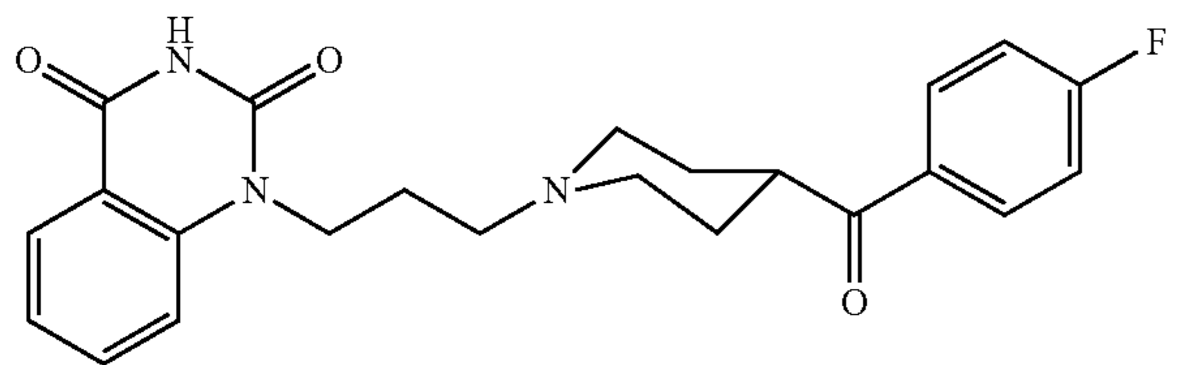
compound 12
