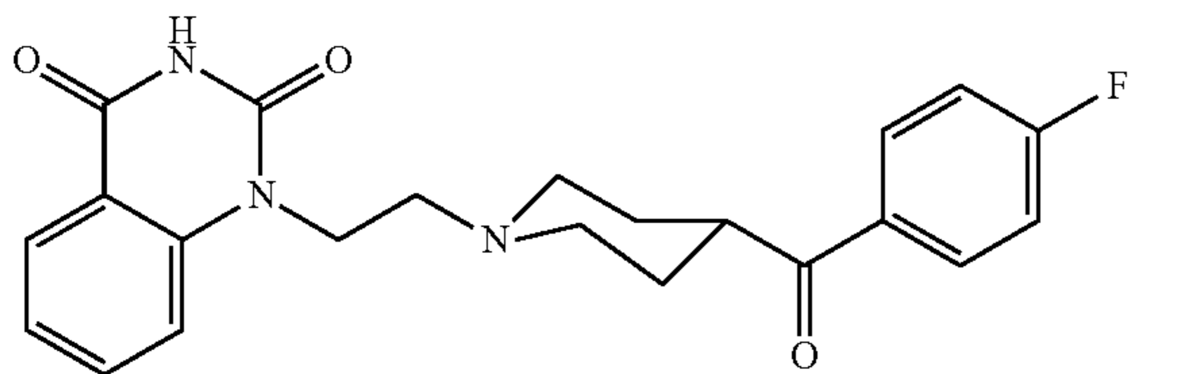
compound 11
