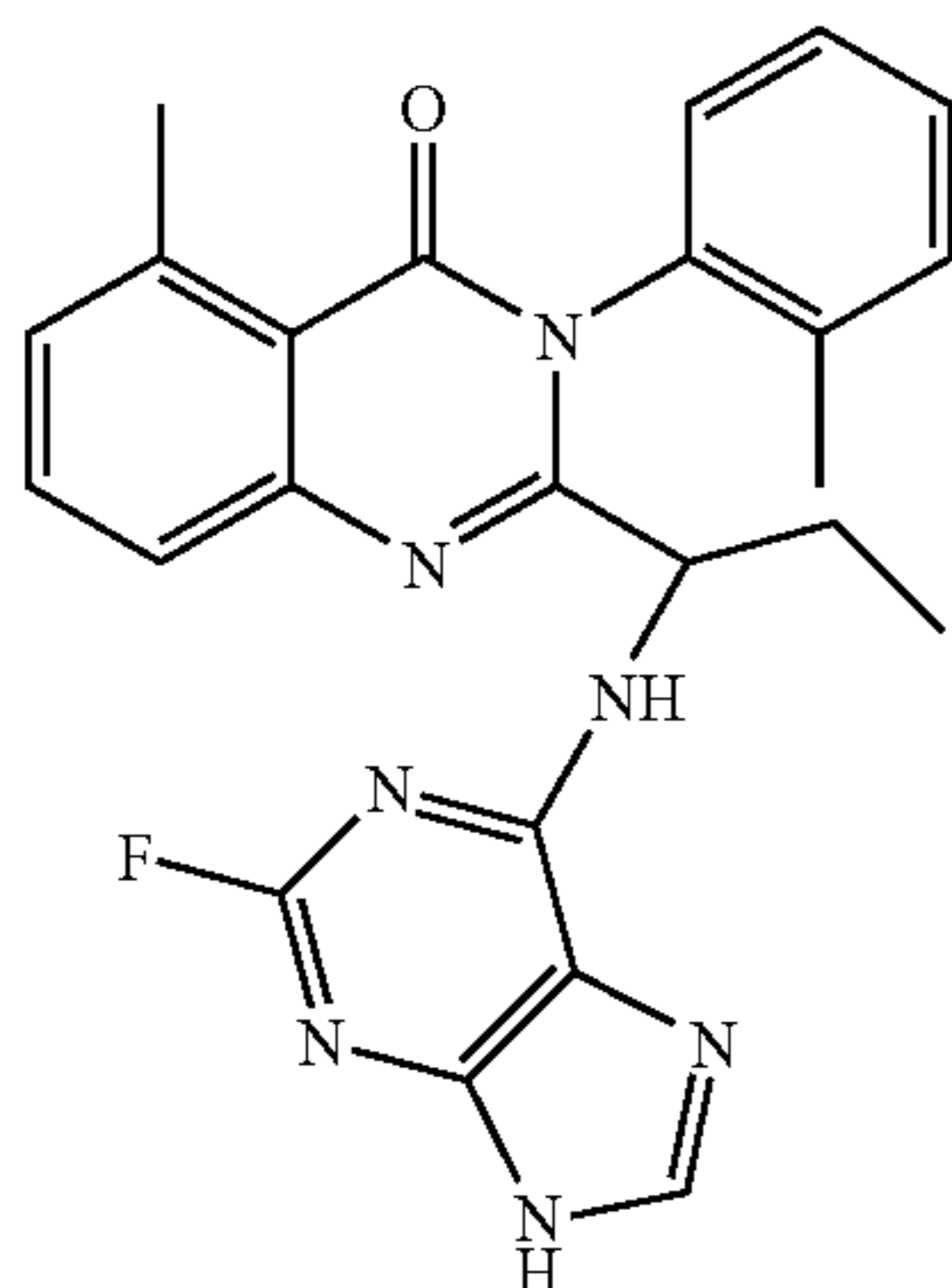
2-(1-(2-Fluoro-9H-purin-6-ylamino)propyl)-5-methyl-3-o-tolyl-3H-quinazolin-4-one (D-081c)
