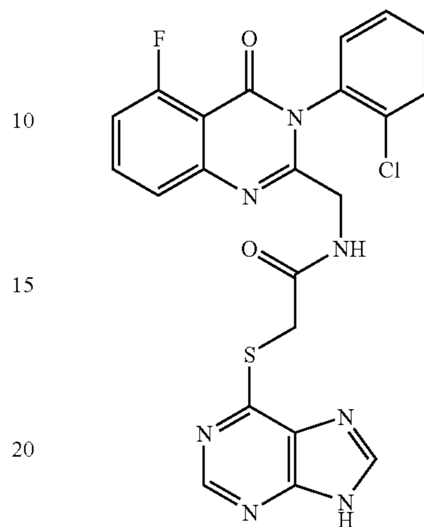
N-[3-(2-Chlorophenyl)-5-fluoro-4-oxo-3,4-dihydro-quinazolin-2-ylmethyl]-2-(9H-purin-6-ylsulfanyl)-acetamide (D-077)
