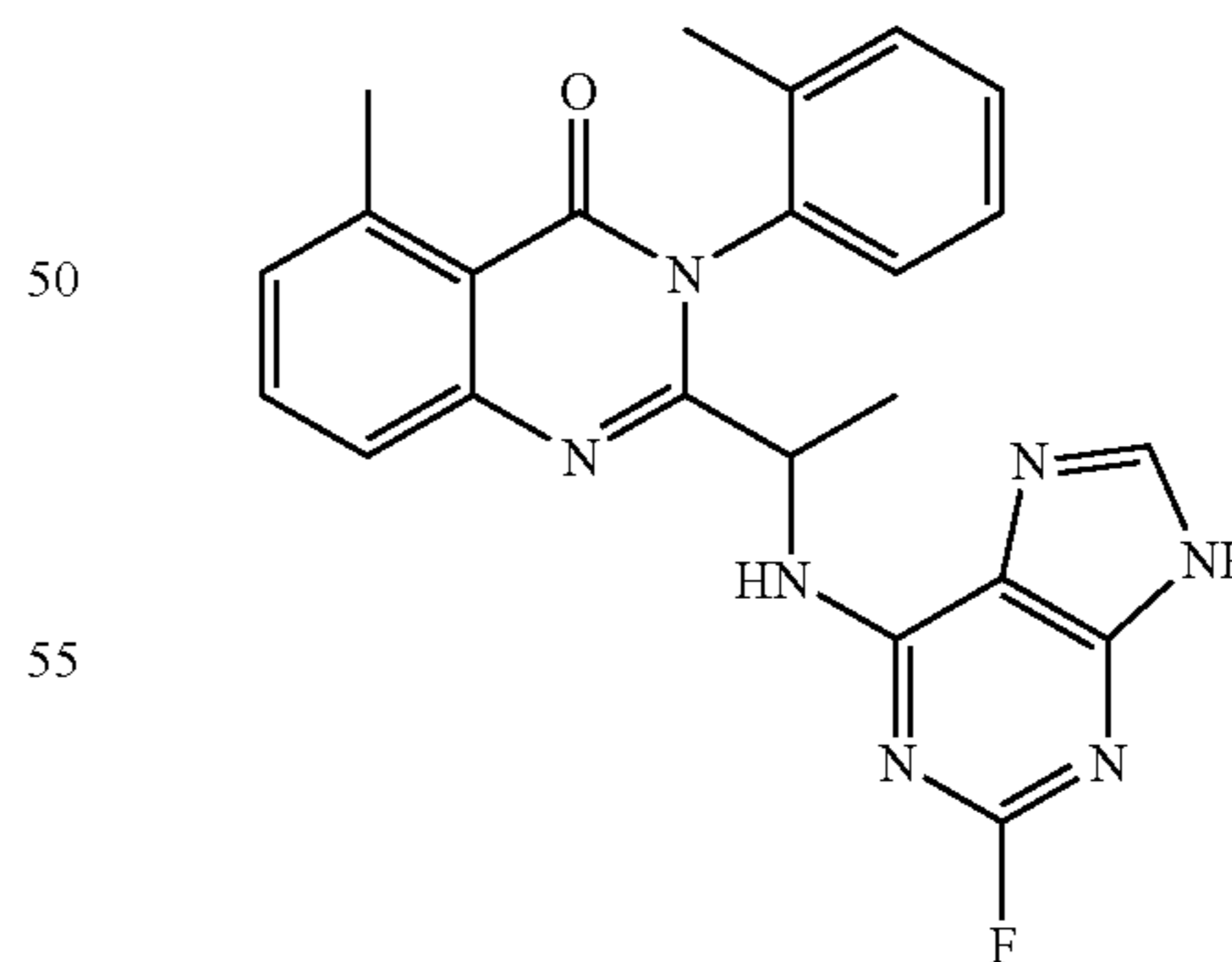
2-[1-(2-Fluoro-9H-purin-6-ylamino)ethyl]-5-methyl-3-o-tolyl-3H-quinazolin-4-one (D-080)
