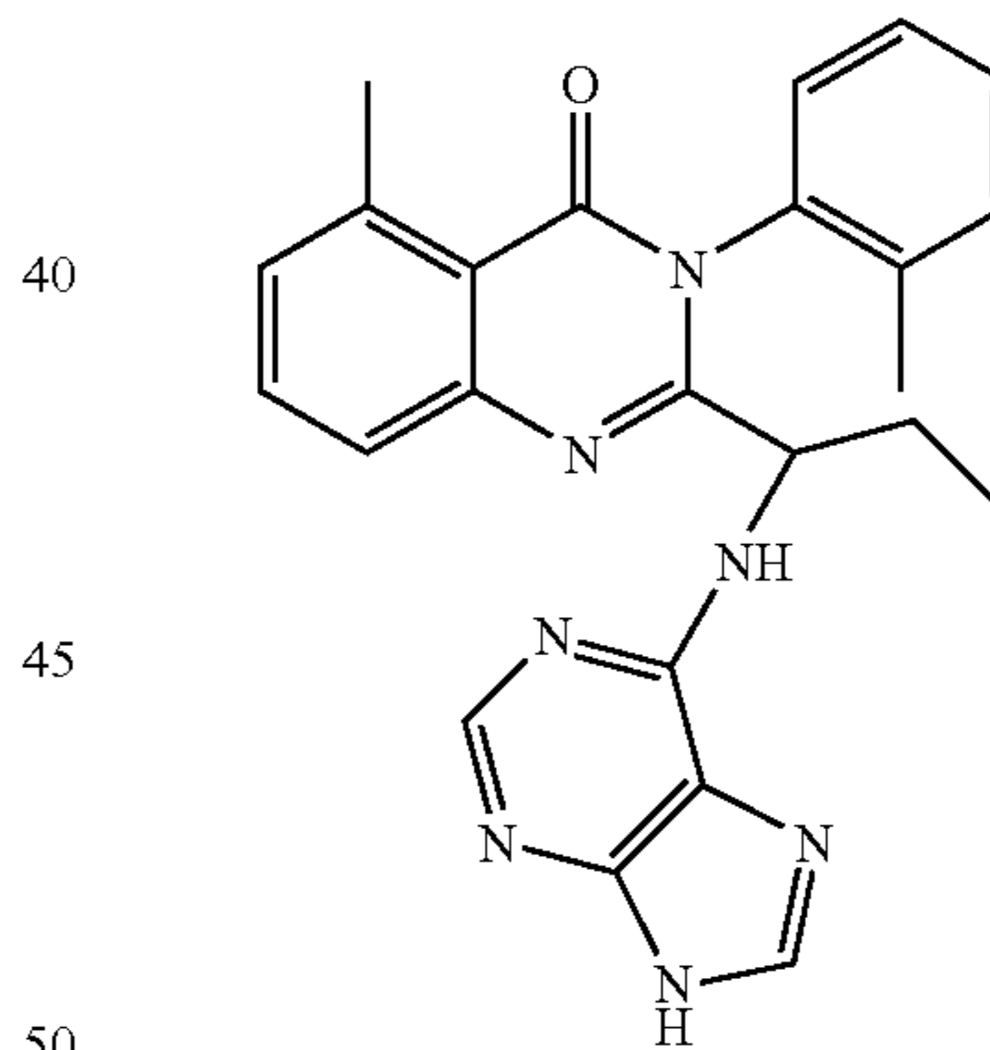
5-Methyl-2-(1-(9H-purin-6-ylamino)propyl)-3-o-tolyl-3H-quinazolin-4-one (D-081b)
