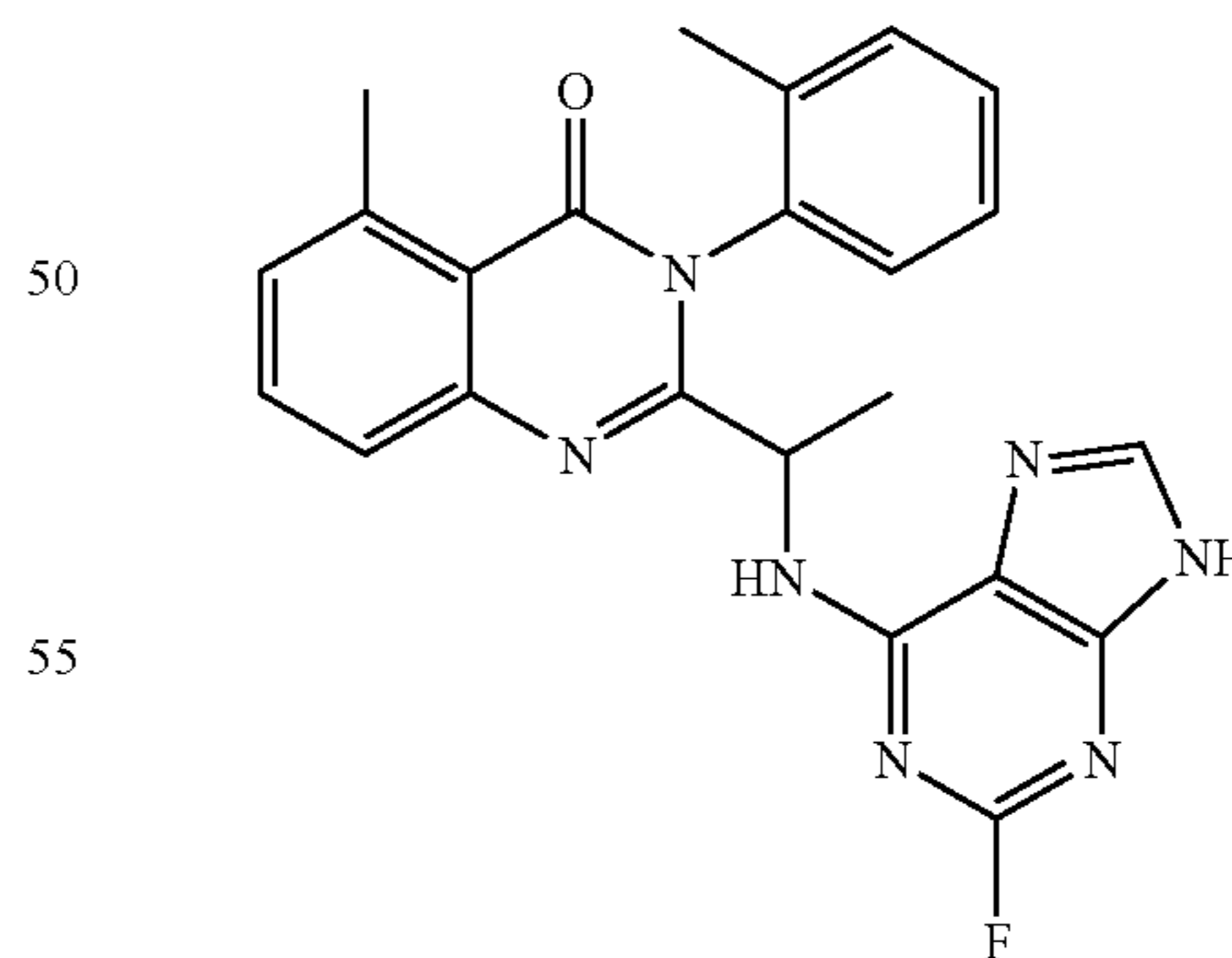
2-[1-(2-Fluoro-9H-purin-6-ylamino)ethyl]-5-methyl-3-o-tolyl-3H-quinazolin-4-one (D-080)
