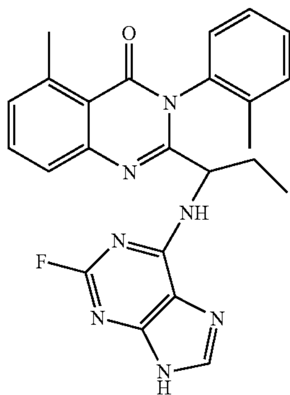
2-(1-(2-Fluoro-9H-purin-6-ylamino)propyl)-5-methyl-3-o-tolyl-3H-quinazolin-4-one (D-081c)
