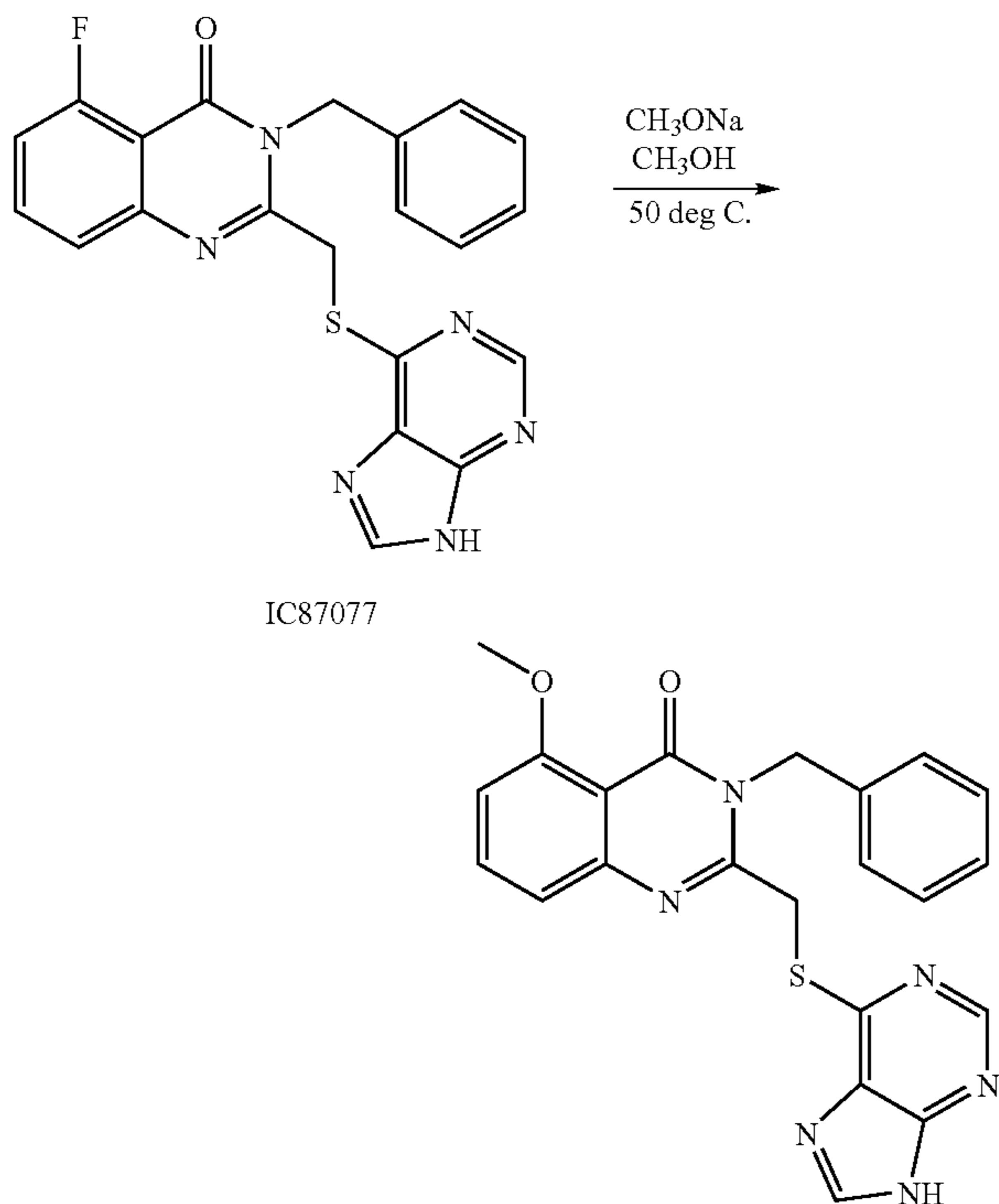
Scheme H
