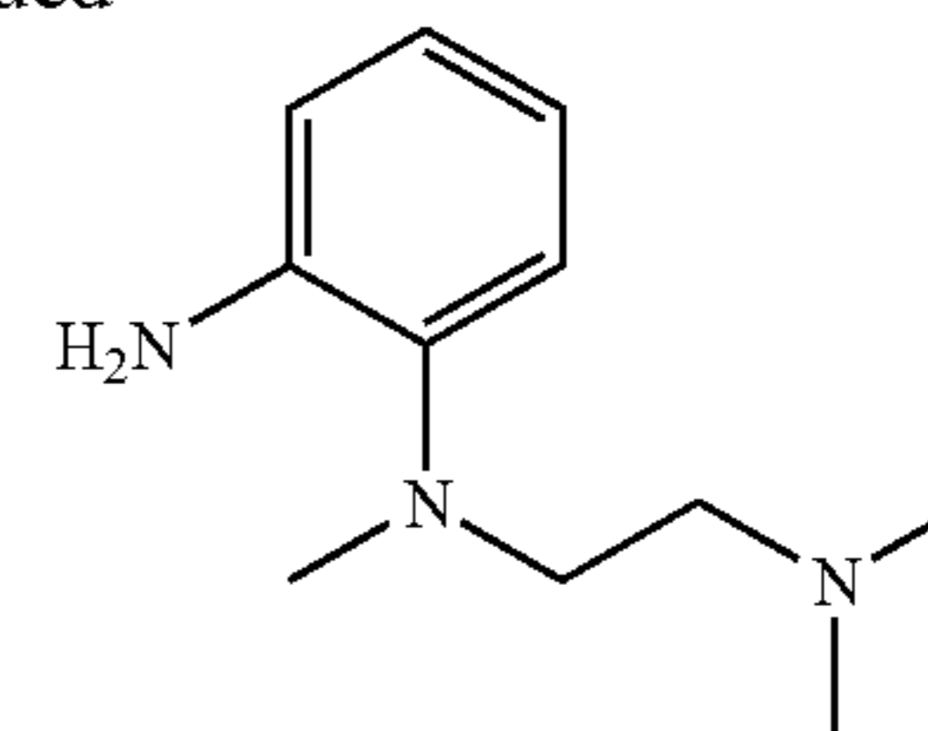
Intermediate E-3
