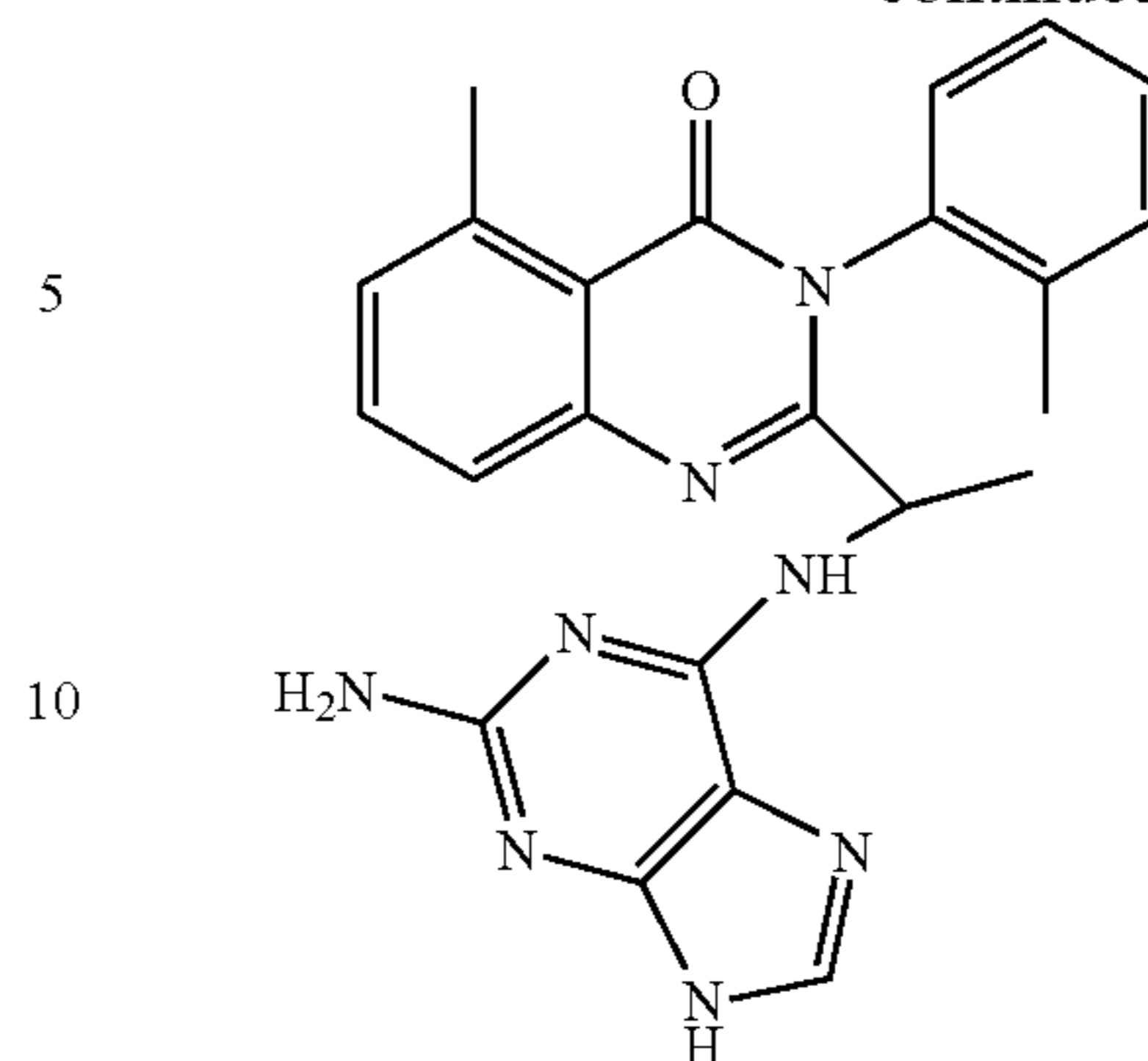
2-(1-(2-Amino-9H-purin-6-ylamino)ethyl)-5-methyl-3-o-tolyl-3H-quinazolin-4-one (D-081a)
