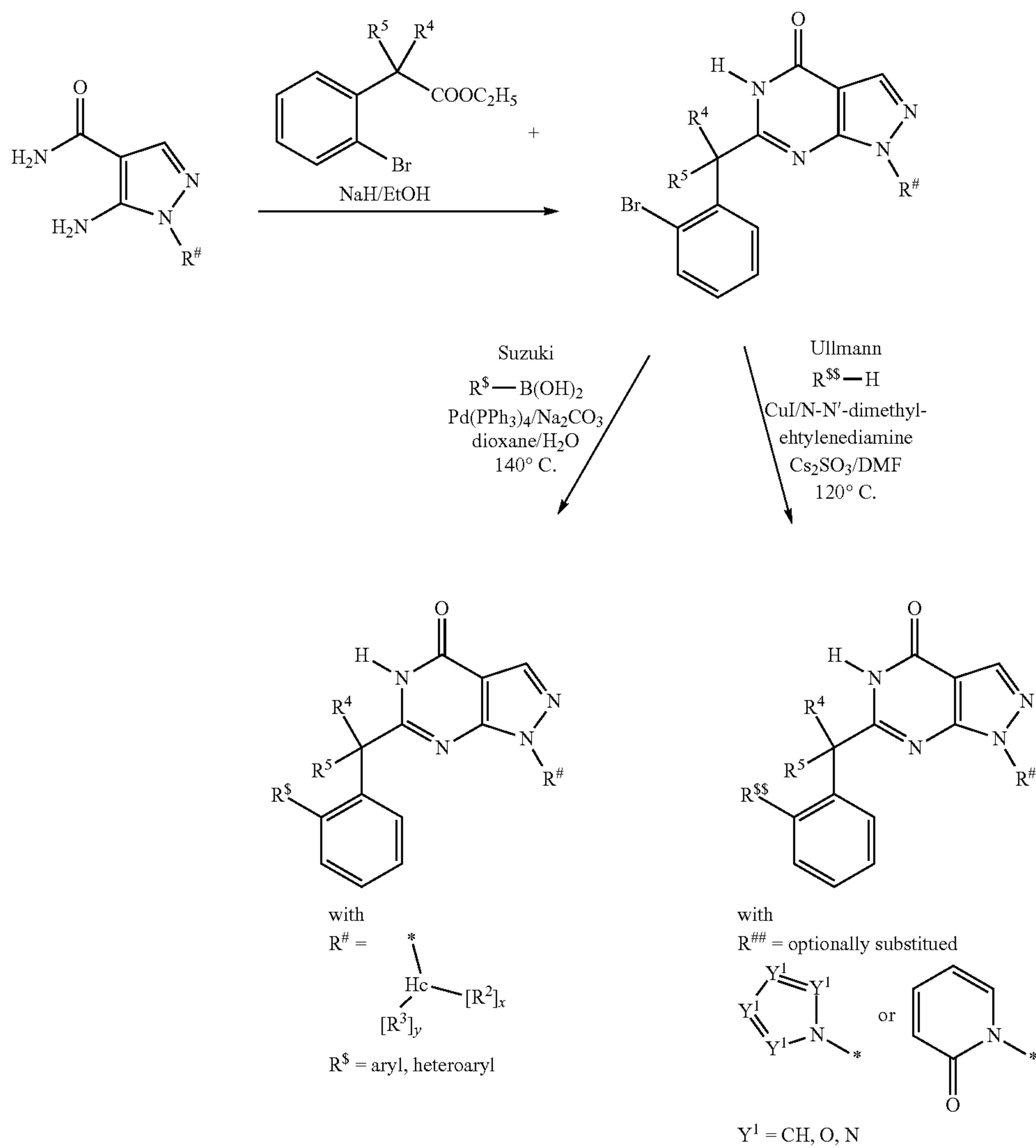
Scheme 4
