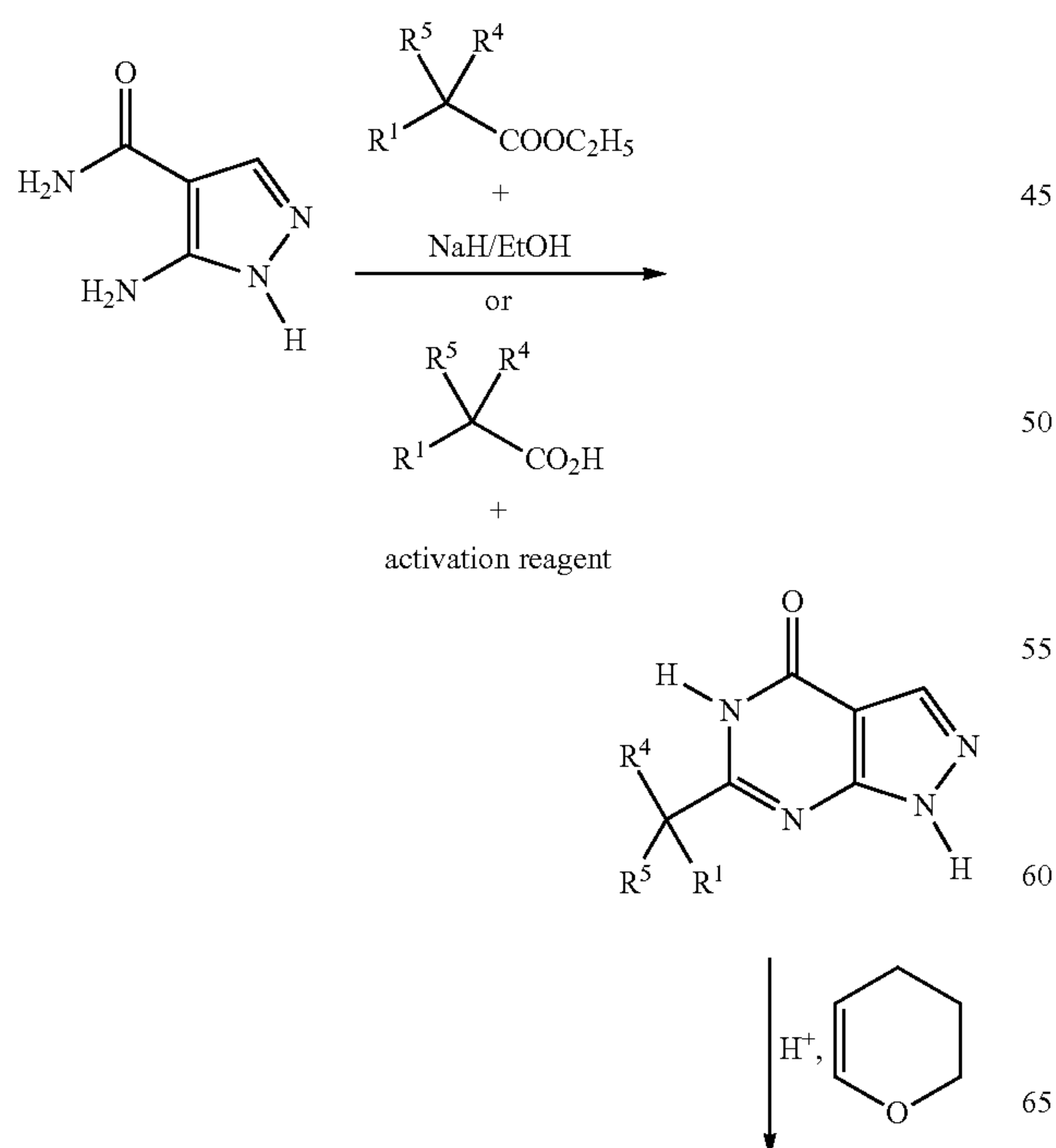
Scheme 2
