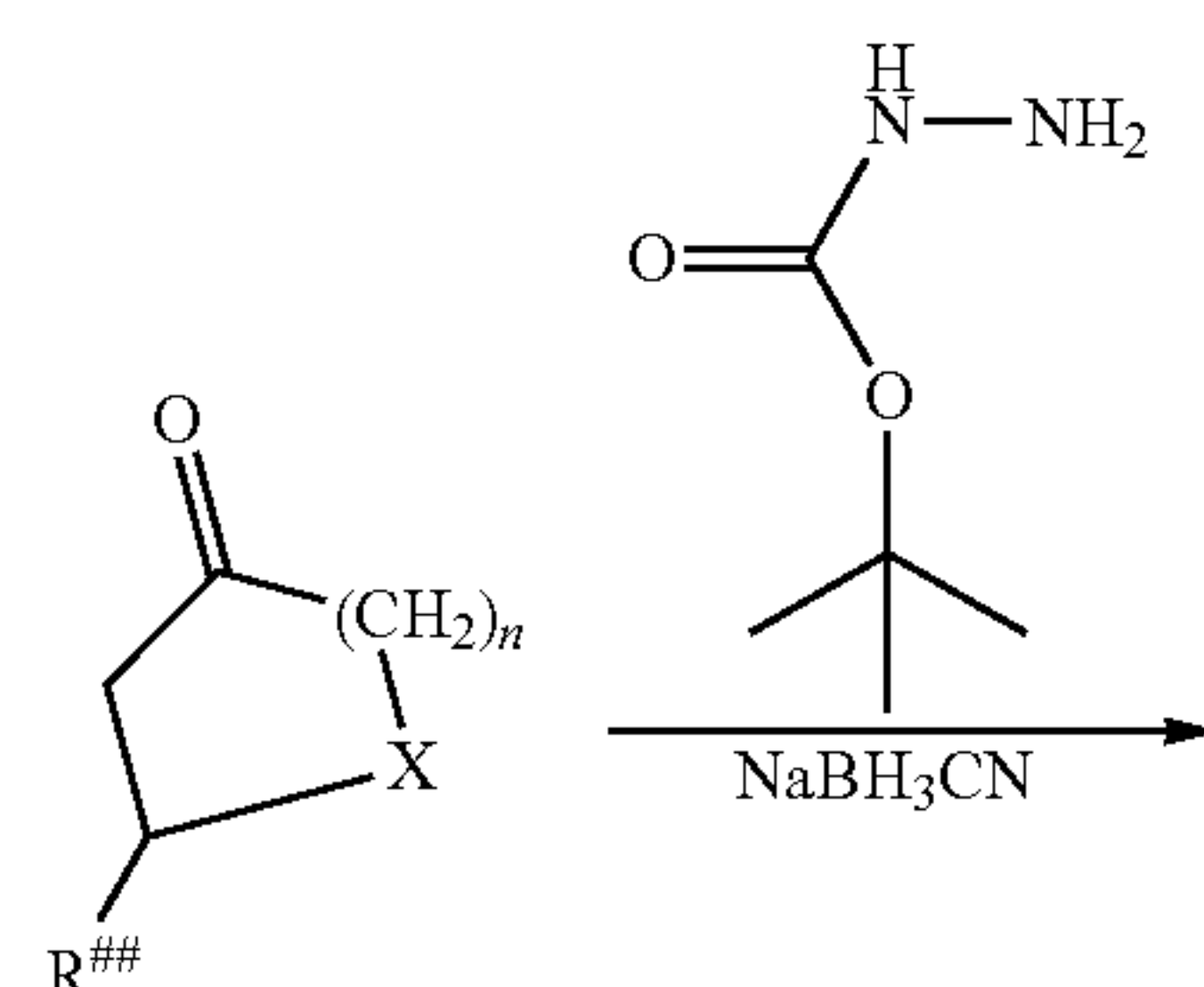
Scheme 7
