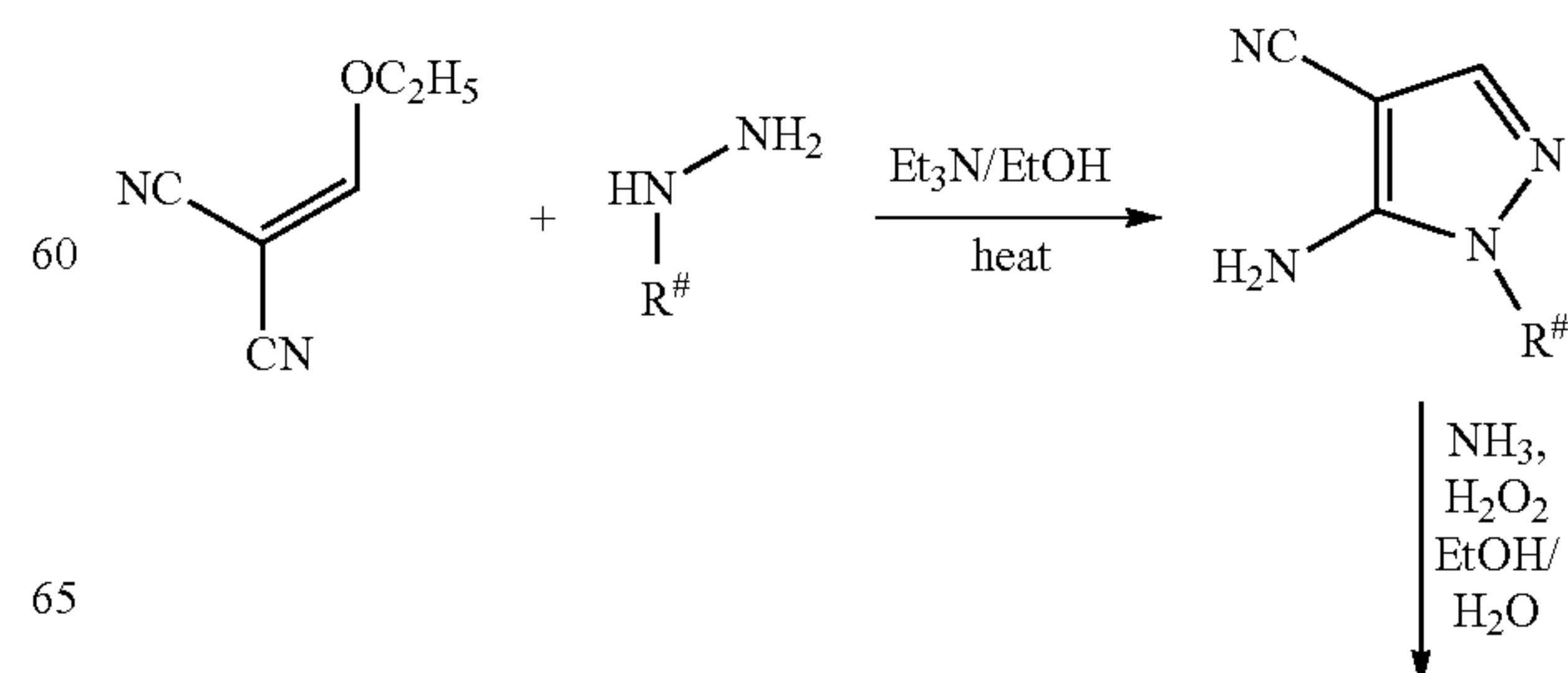
Scheme 1
