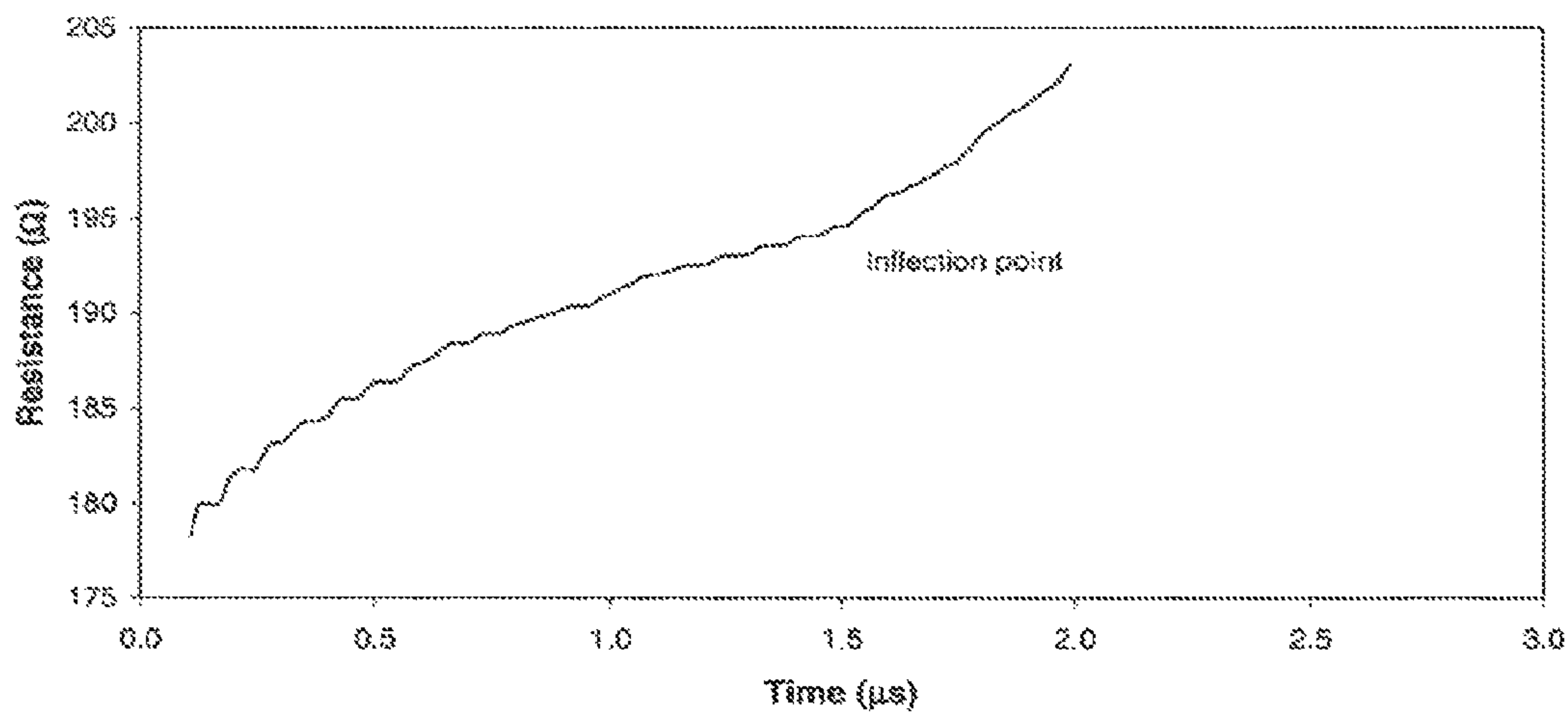
Resistance of a suspended TiN heater vs time during a 2 \mu\text{s} fire pulse in an overdriven condition
