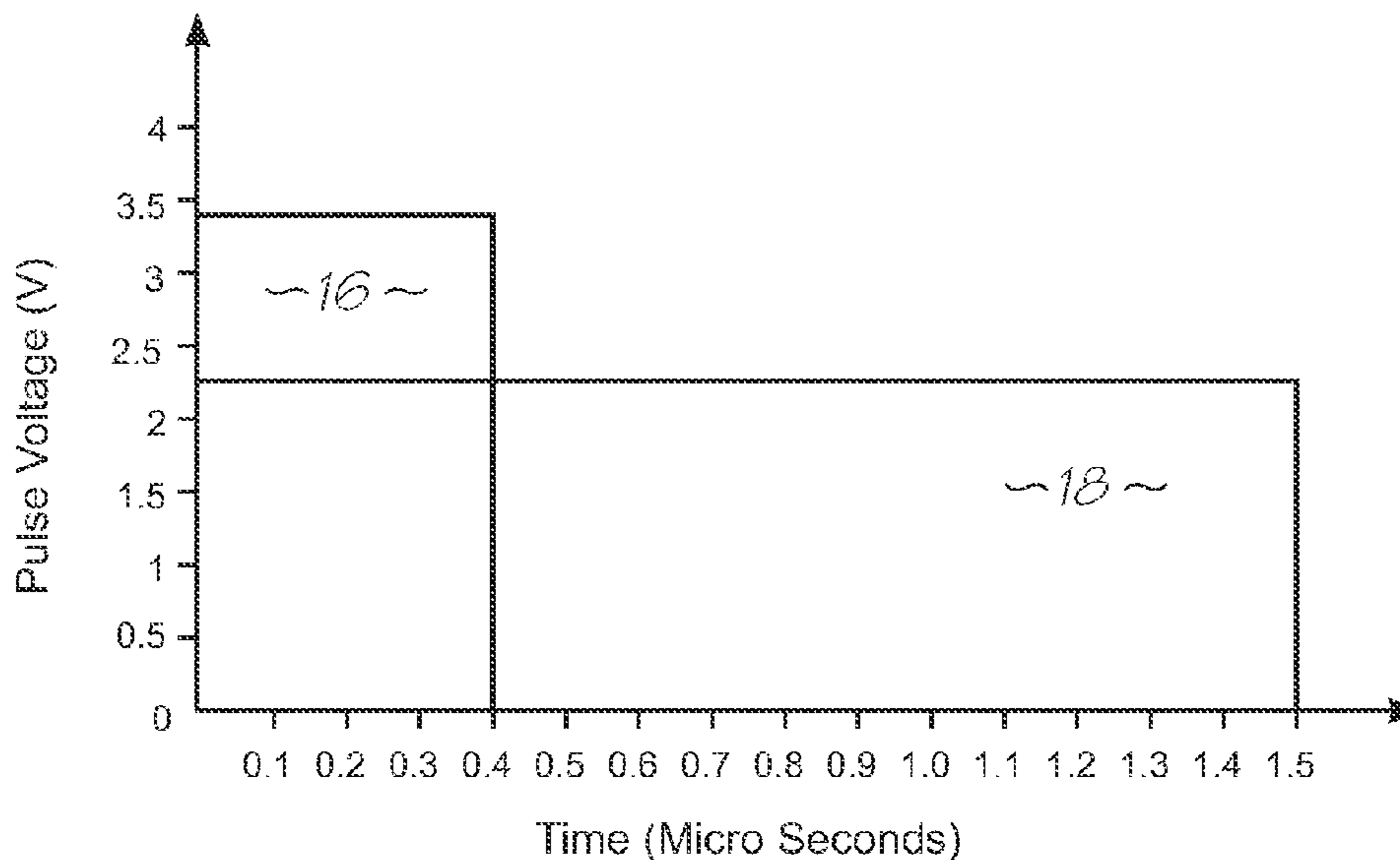
Pulse Power Variation (Amplitude Modulation)
