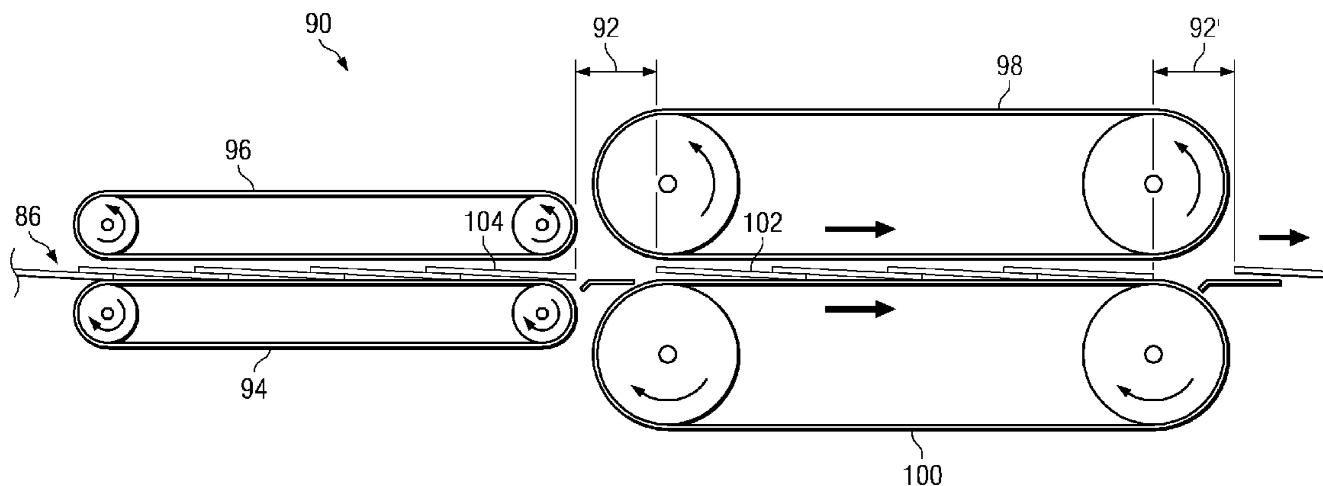
GAP GENERATION IN A STREAM OF UNDER-SHINGLED PIECES
