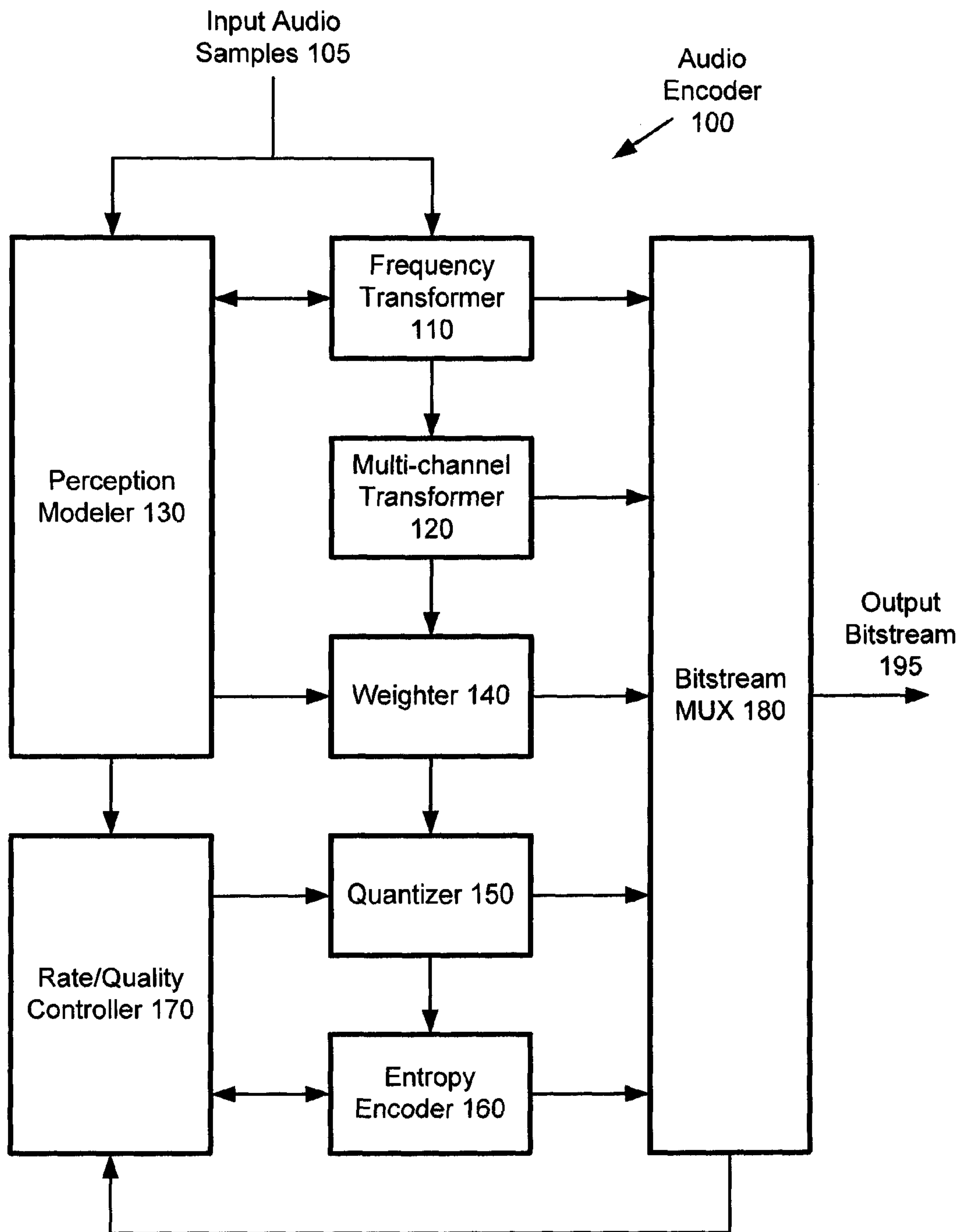
Figure 1, Prior Art
