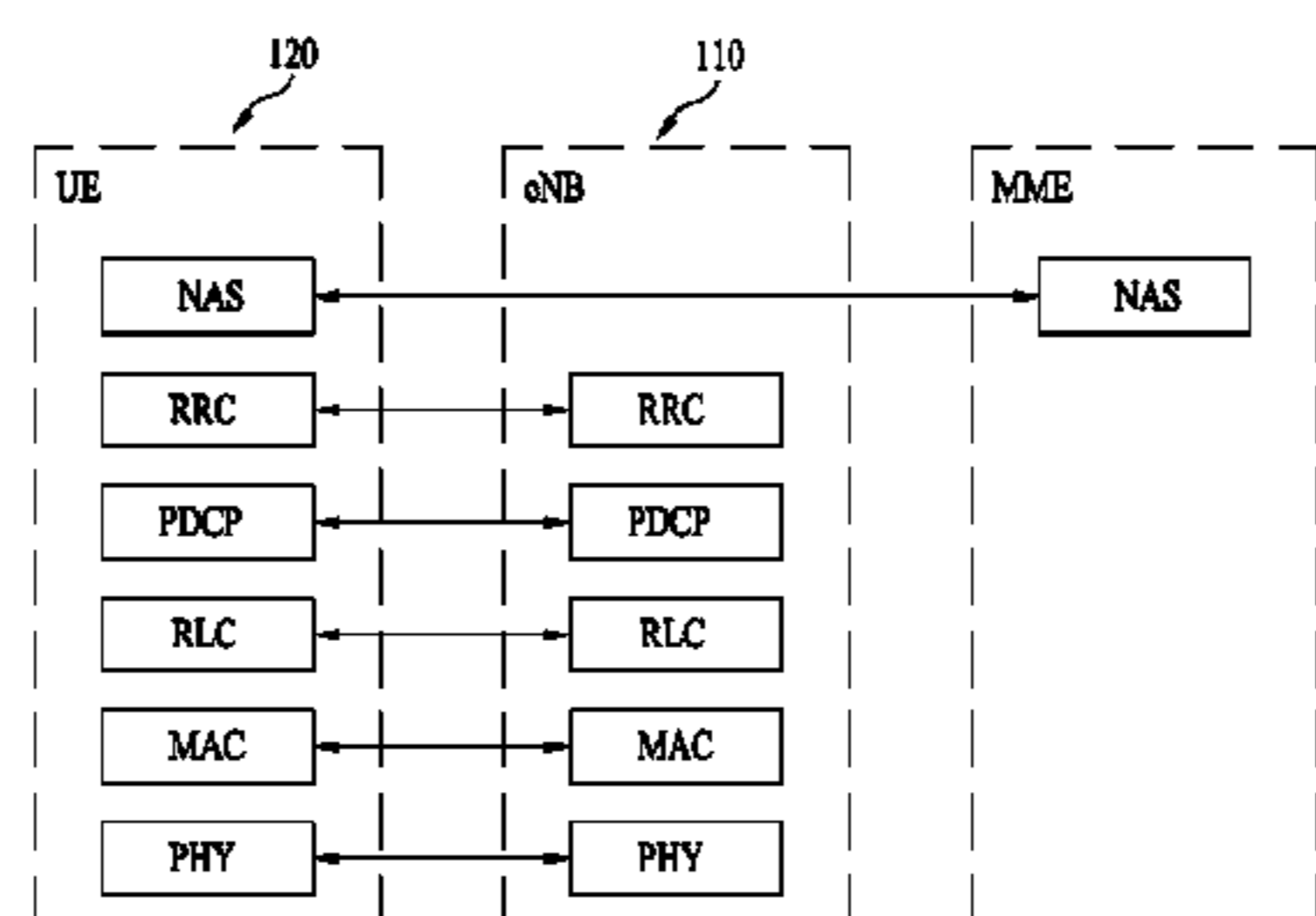
(a) control-plane protocol stack
