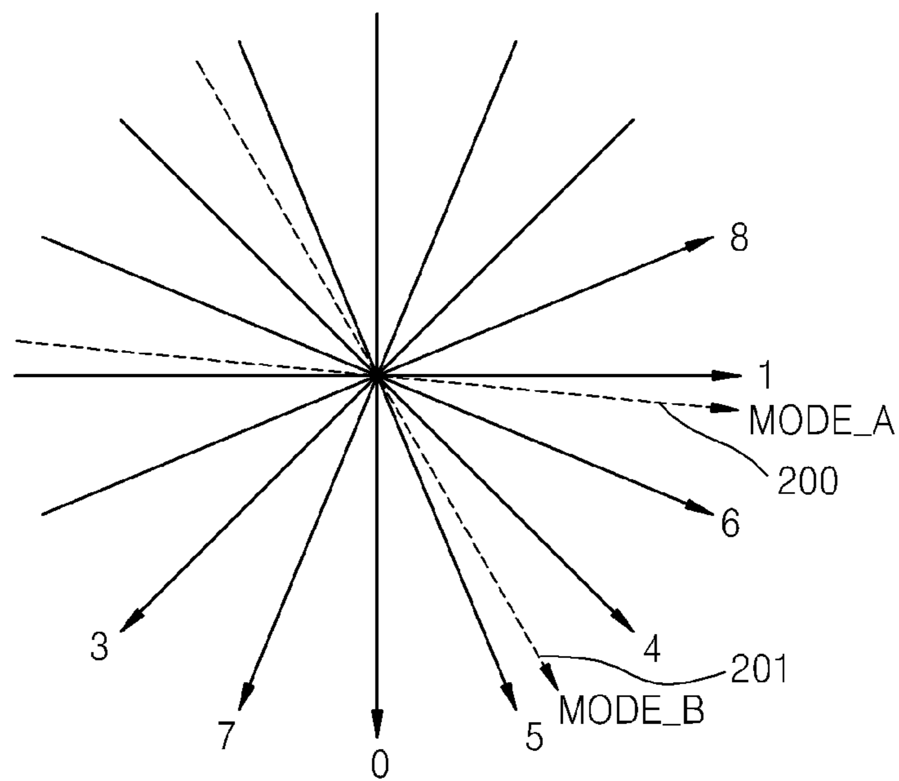
REPRESENTATIVE INTRA PREDICTION MODES
