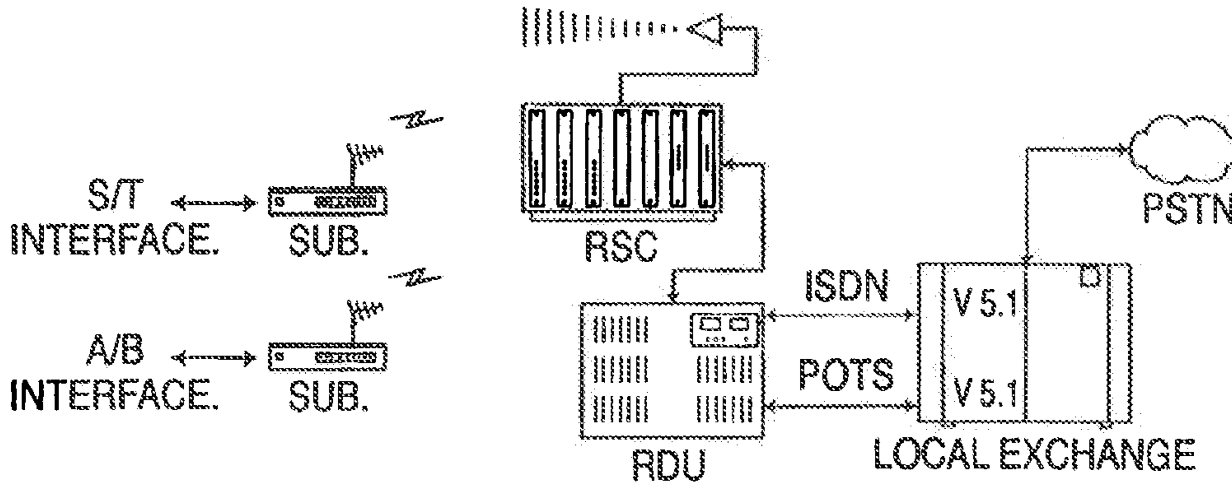
ISDN AND POTS NETWORK INTERFACE
