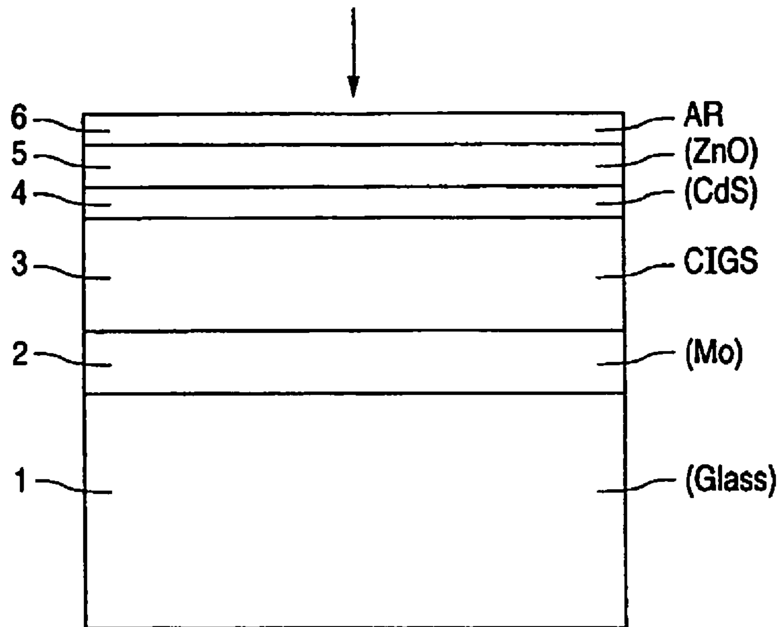
FIG. 1 (PRIOR ART)
