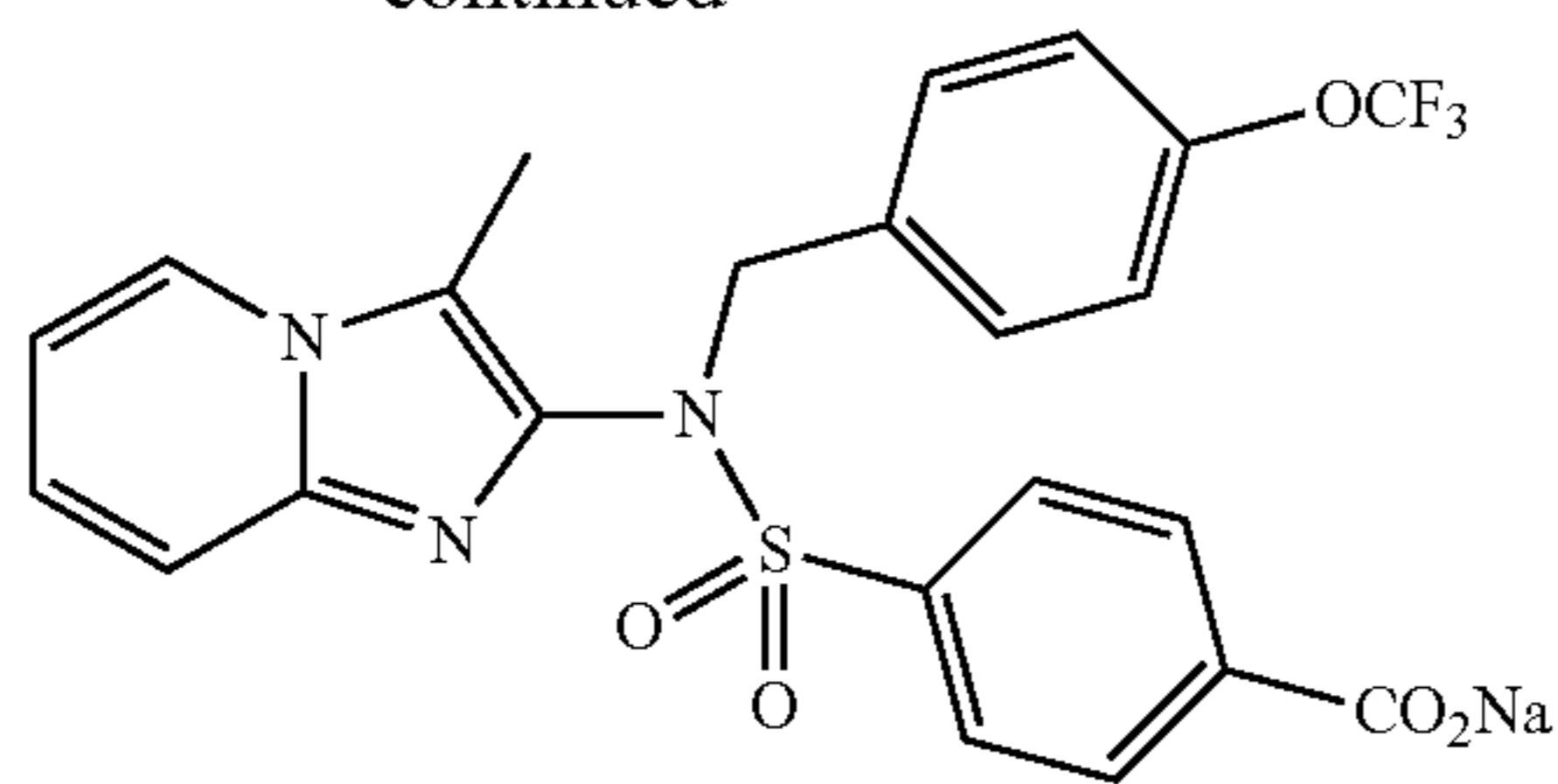
Compound 107
