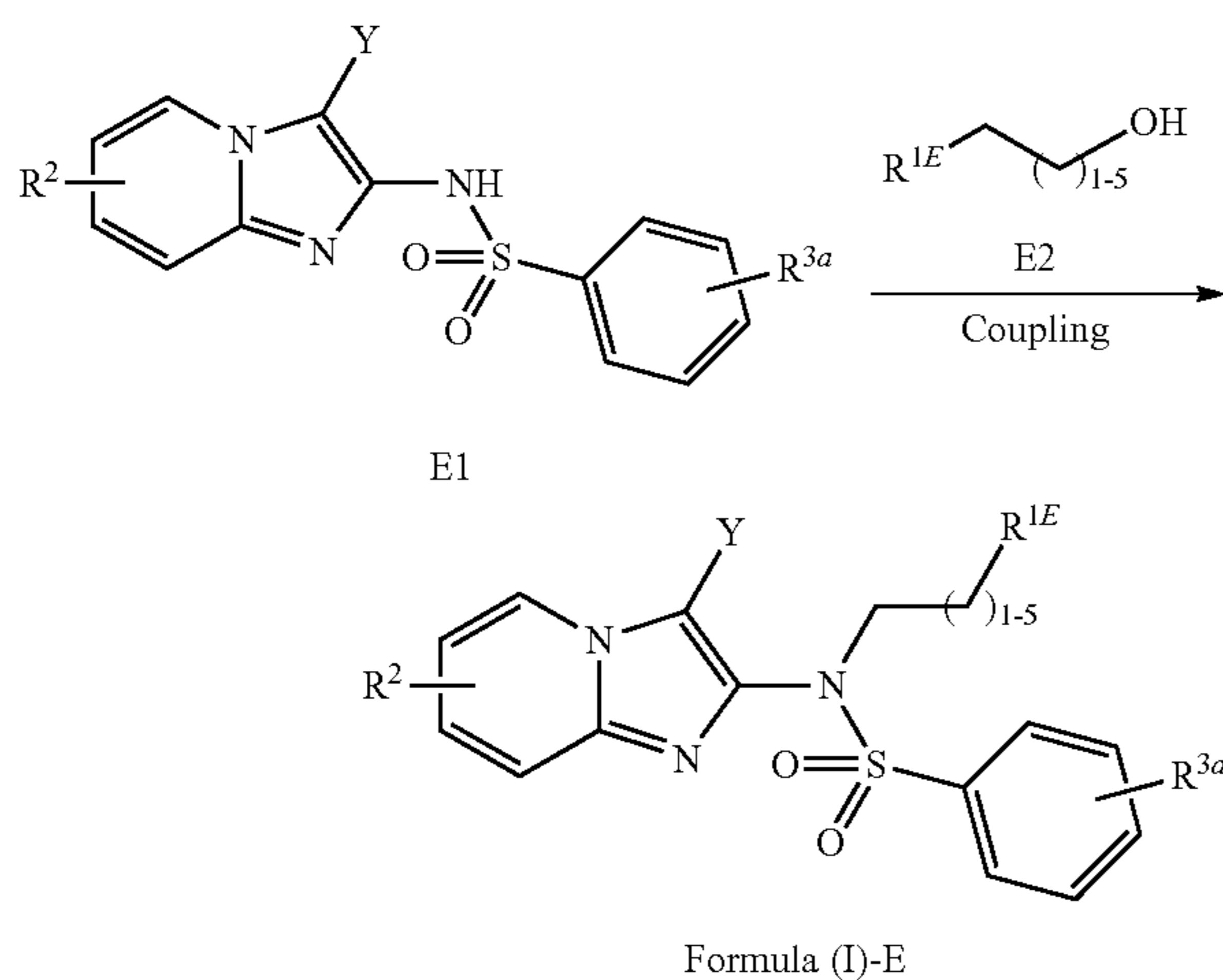
Scheme E
