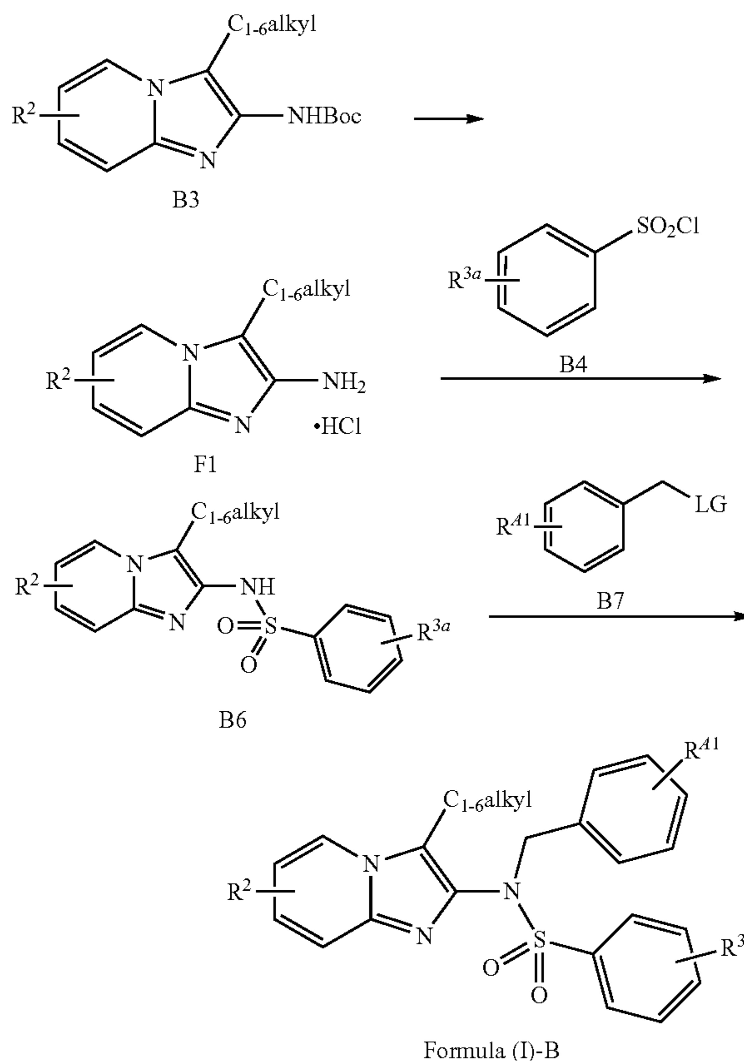
Scheme F
