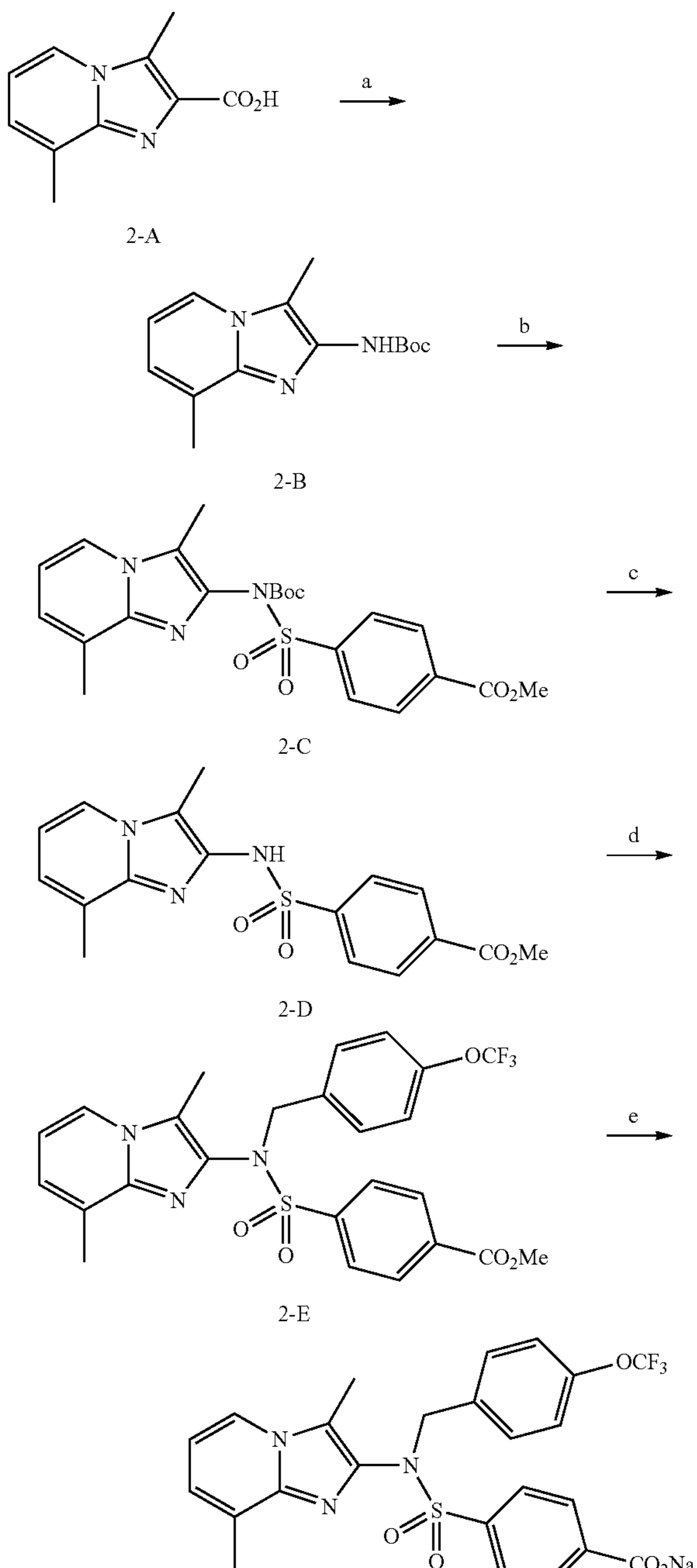
Compound 117
