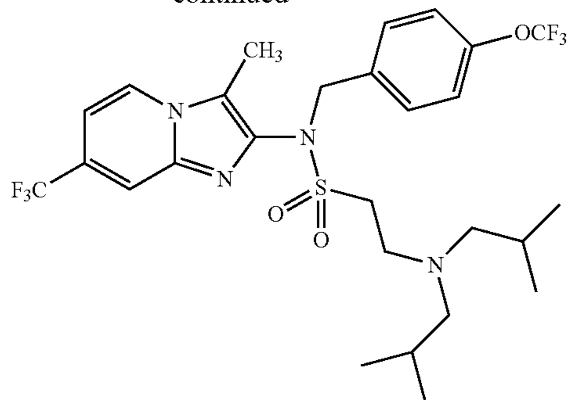
Compound 106
