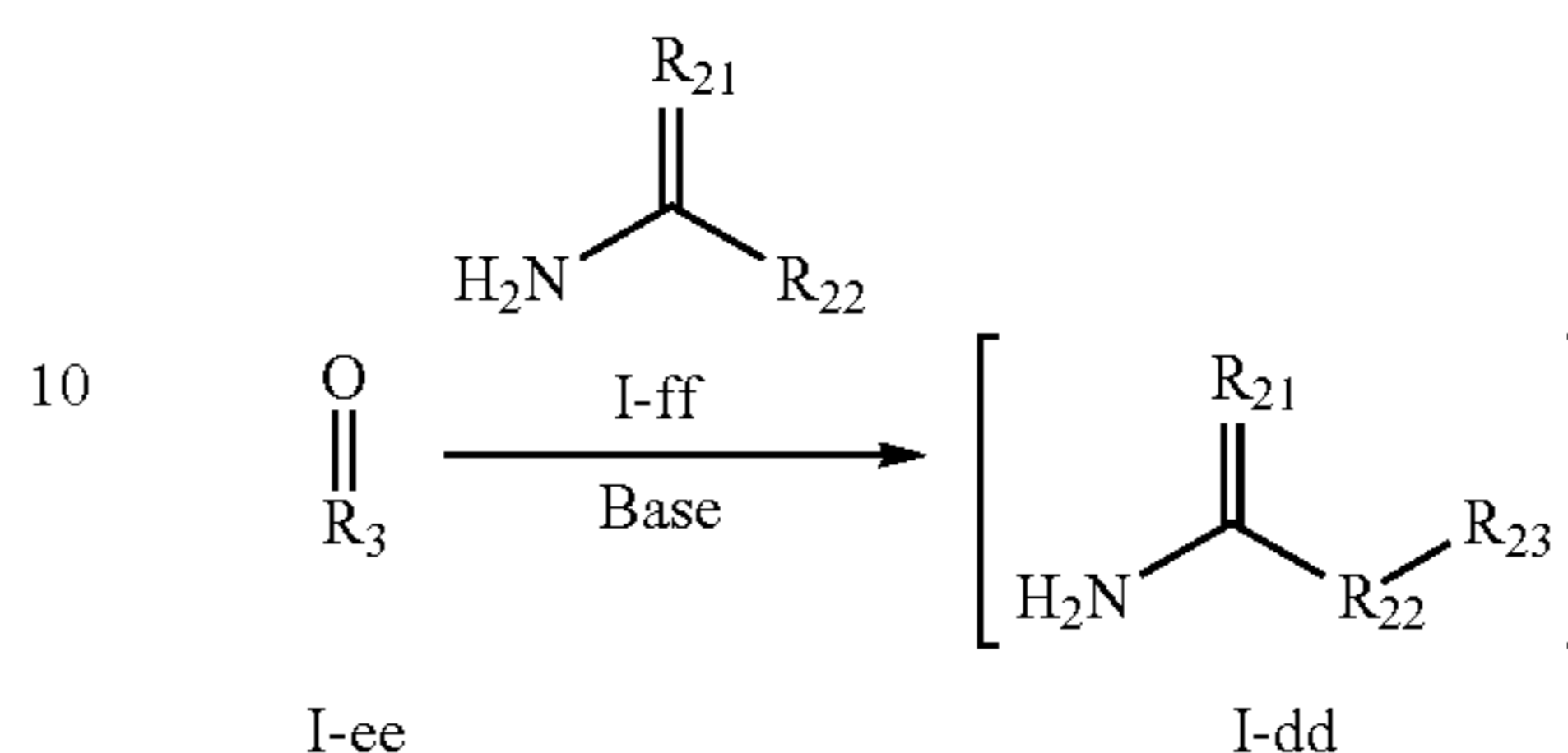
Scheme 1: Preparation of hydrazone I-dd
