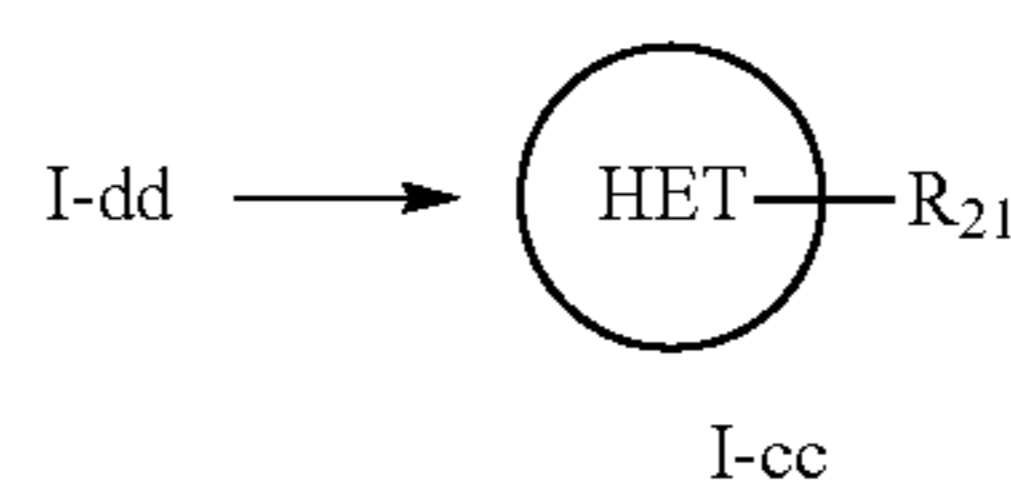
Scheme 2: Preparation of hydrazone of Formula I-cc
