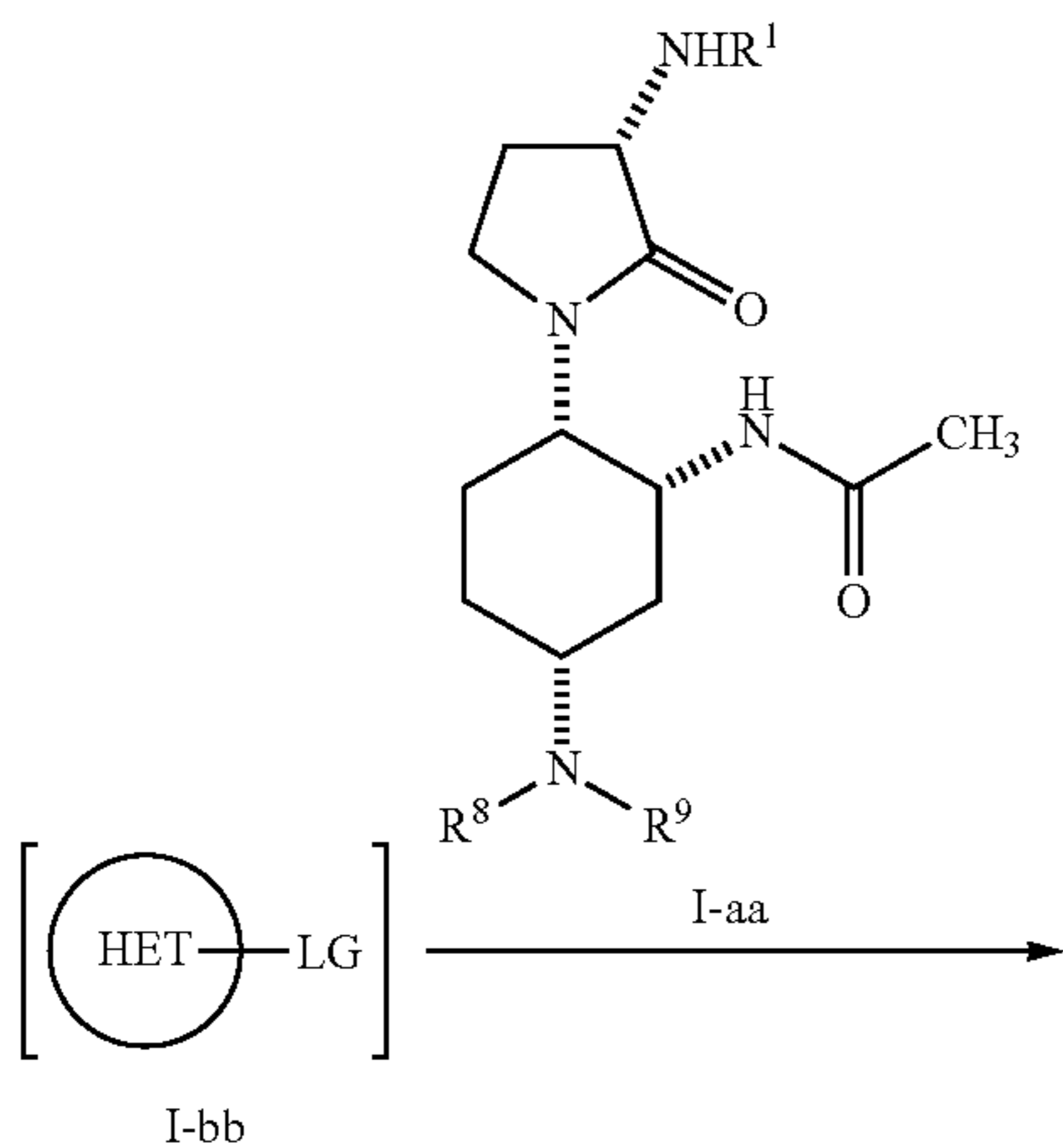
Scheme 4: Preparation of a compound of formula I, or a salt thereof
