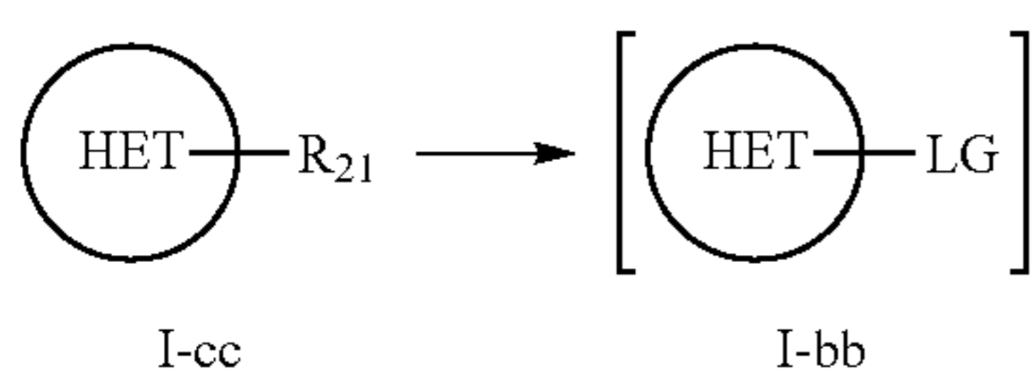
Scheme 3: Conversion of Compound I-cc
