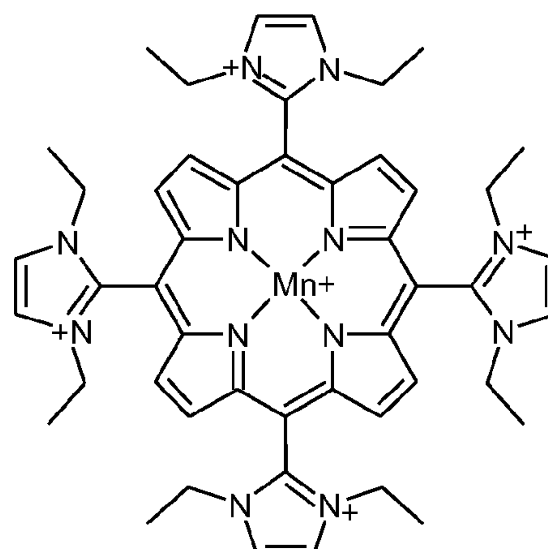
Mn III TDE-2-ImP 5+
