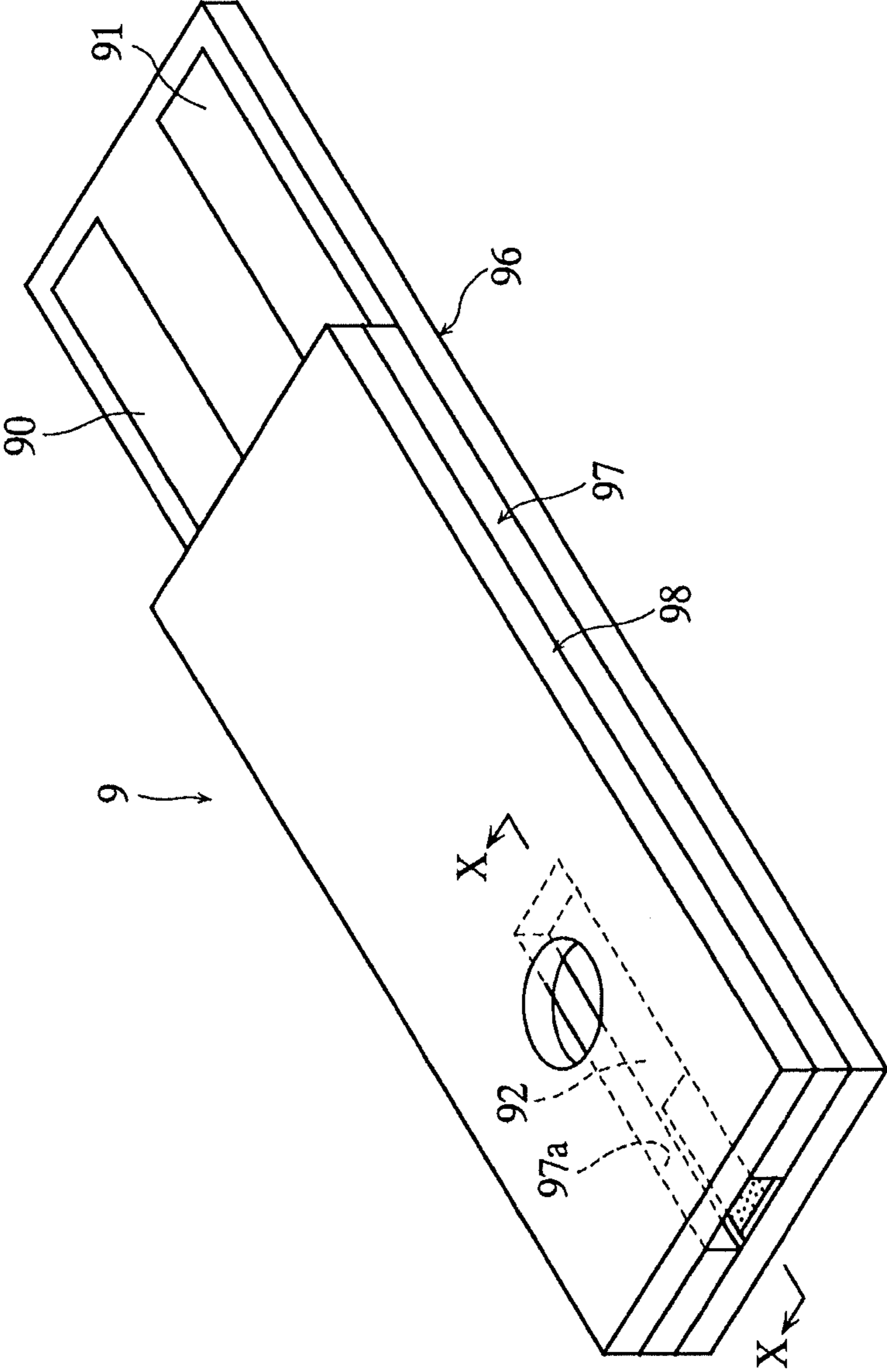
FIG.9 Prior Art
