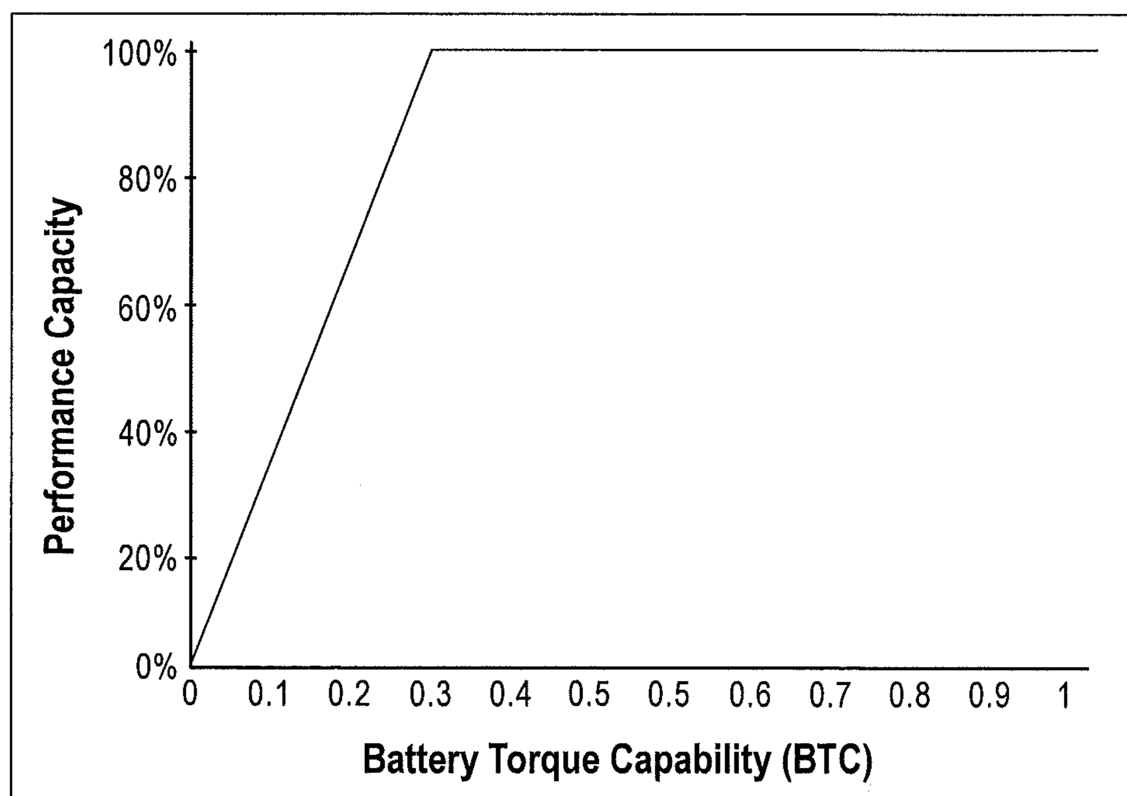
Regen Braking
