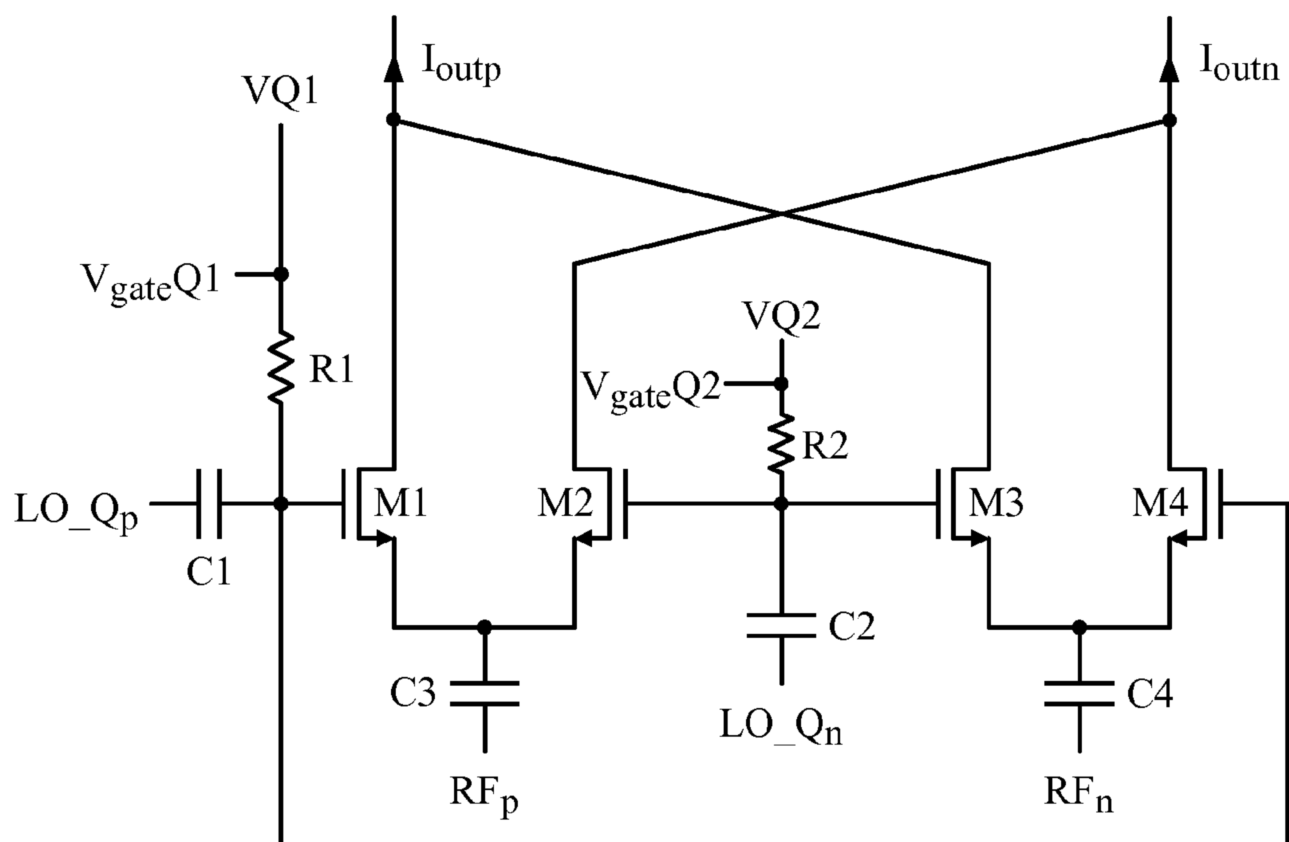
Q MIXER
