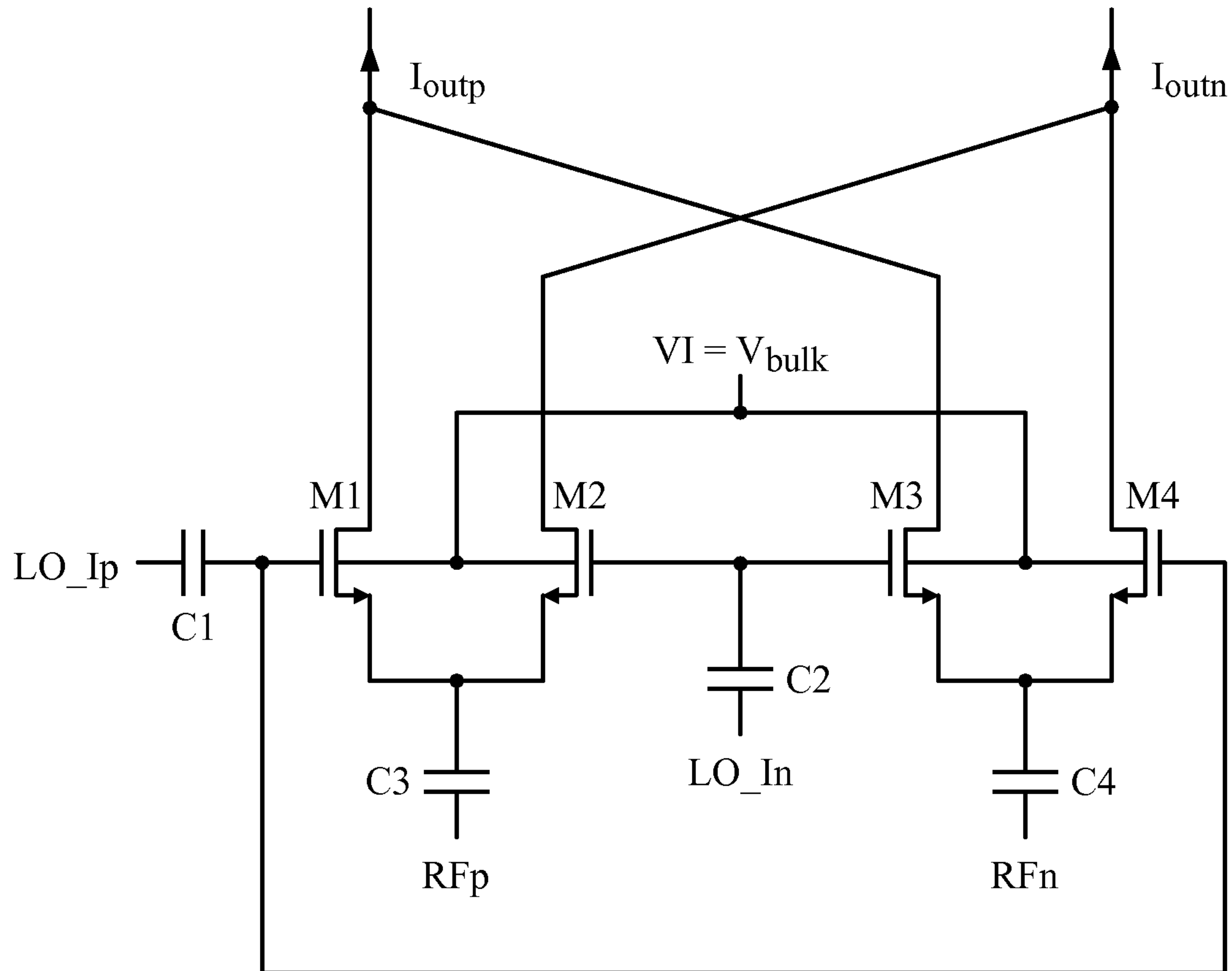
I MIXER
