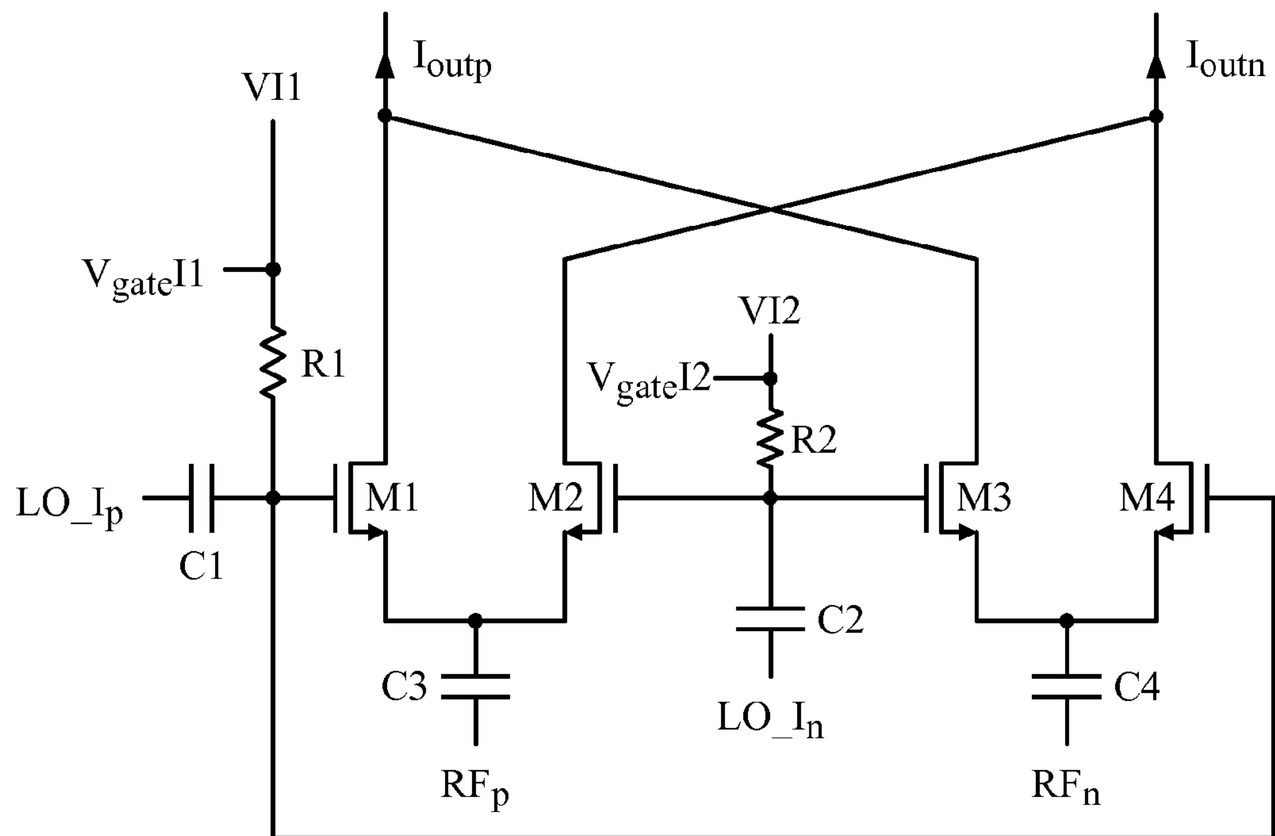
I MIXER
