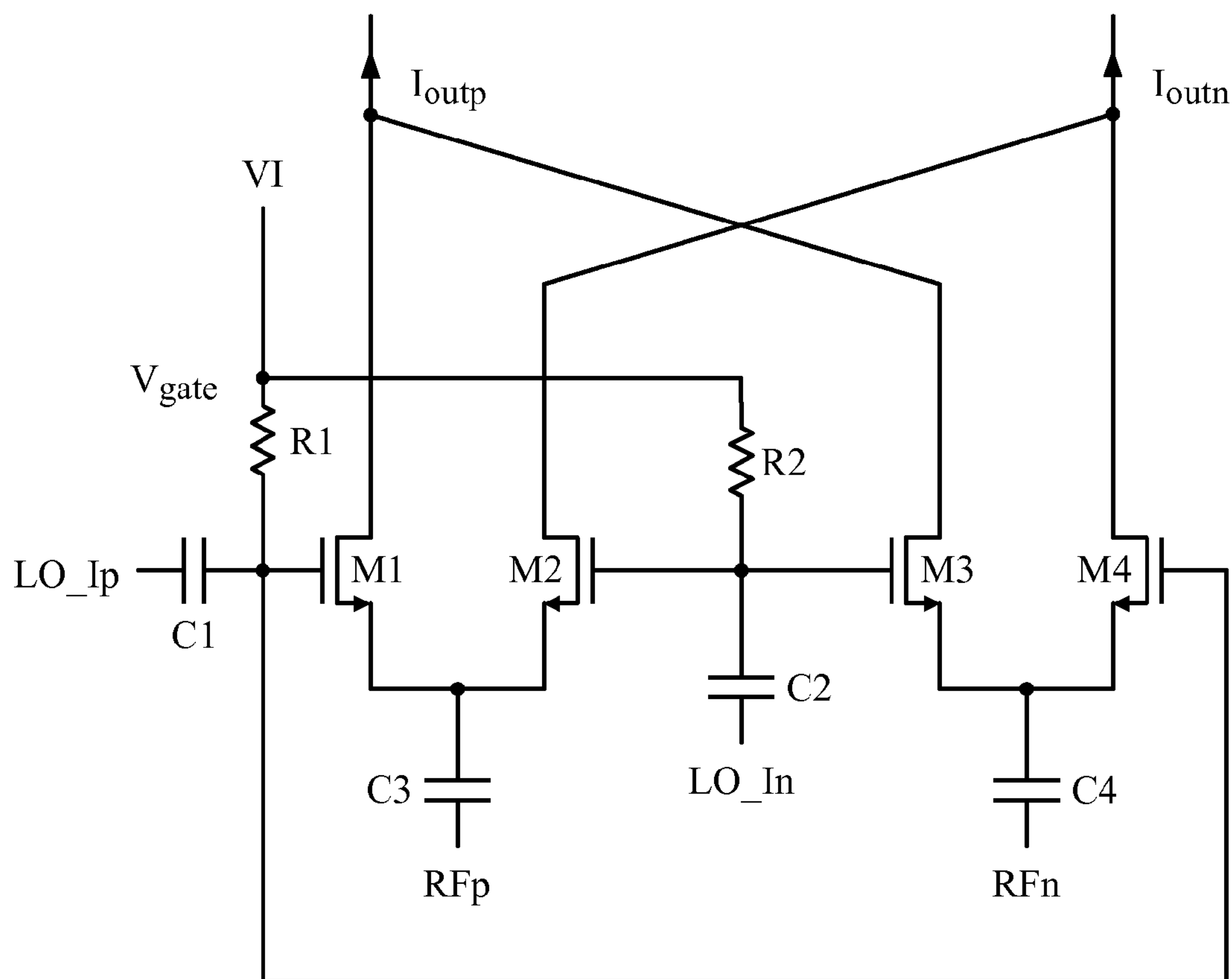
I MIXER
