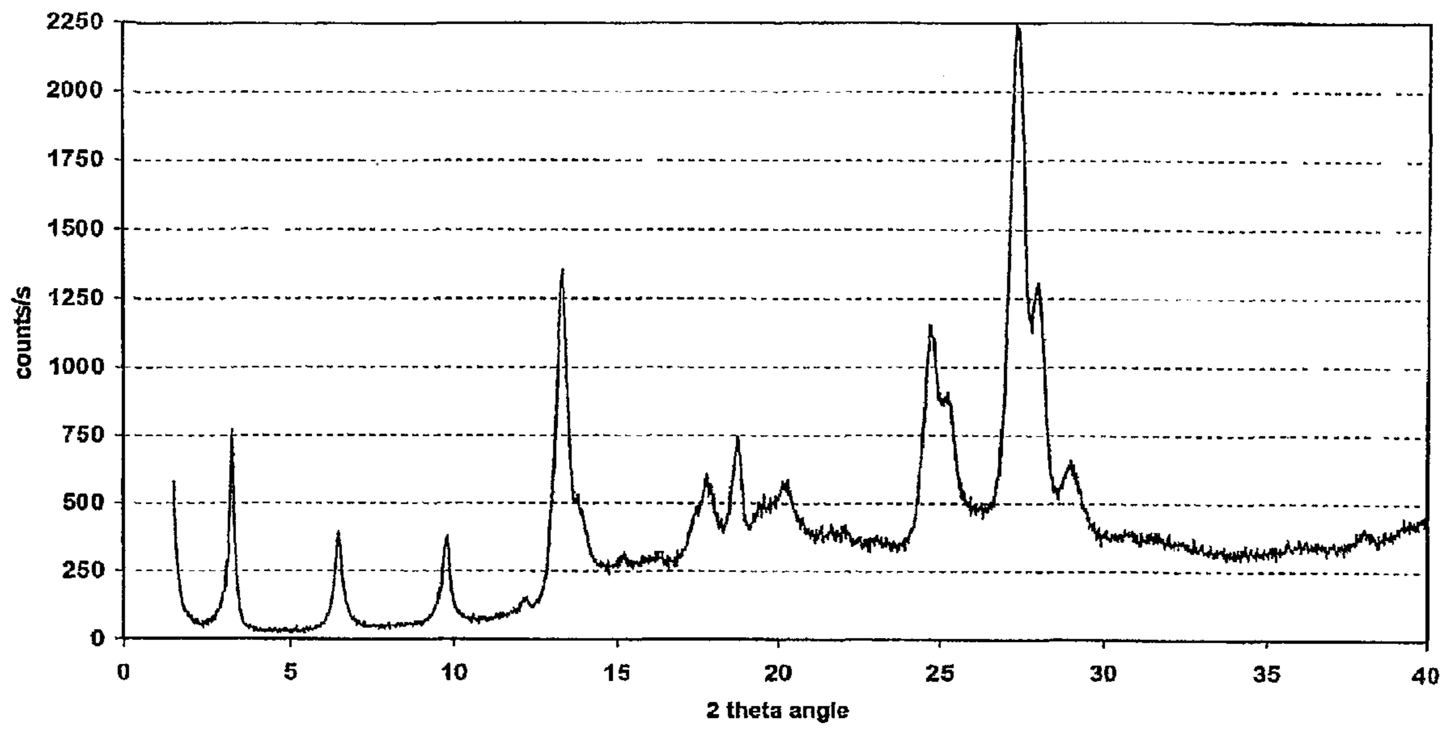
Powder X-ray Diffraction Pattern of Form C
