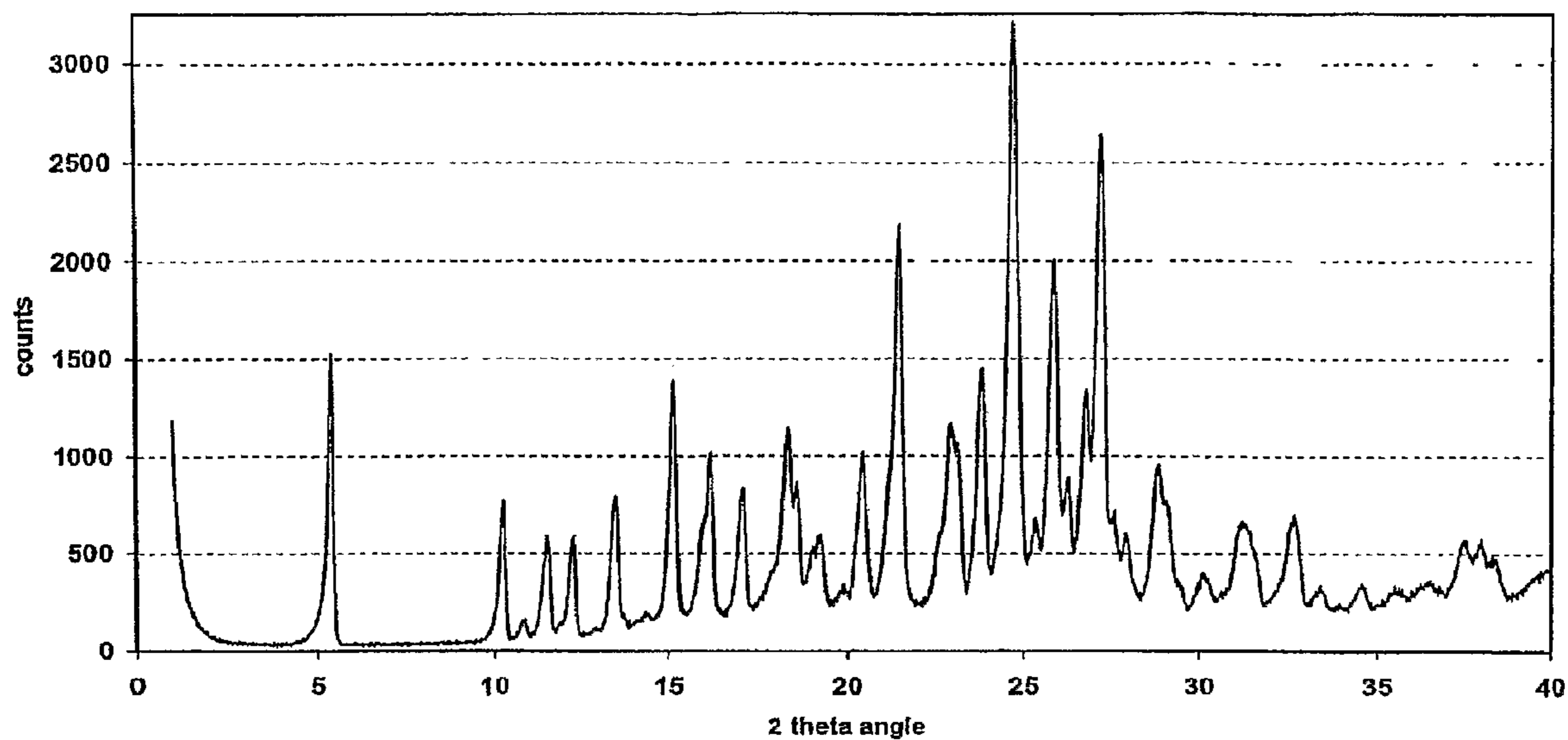
Powder X-ray Diffraction Pattern of Benzene Hemisolvate
