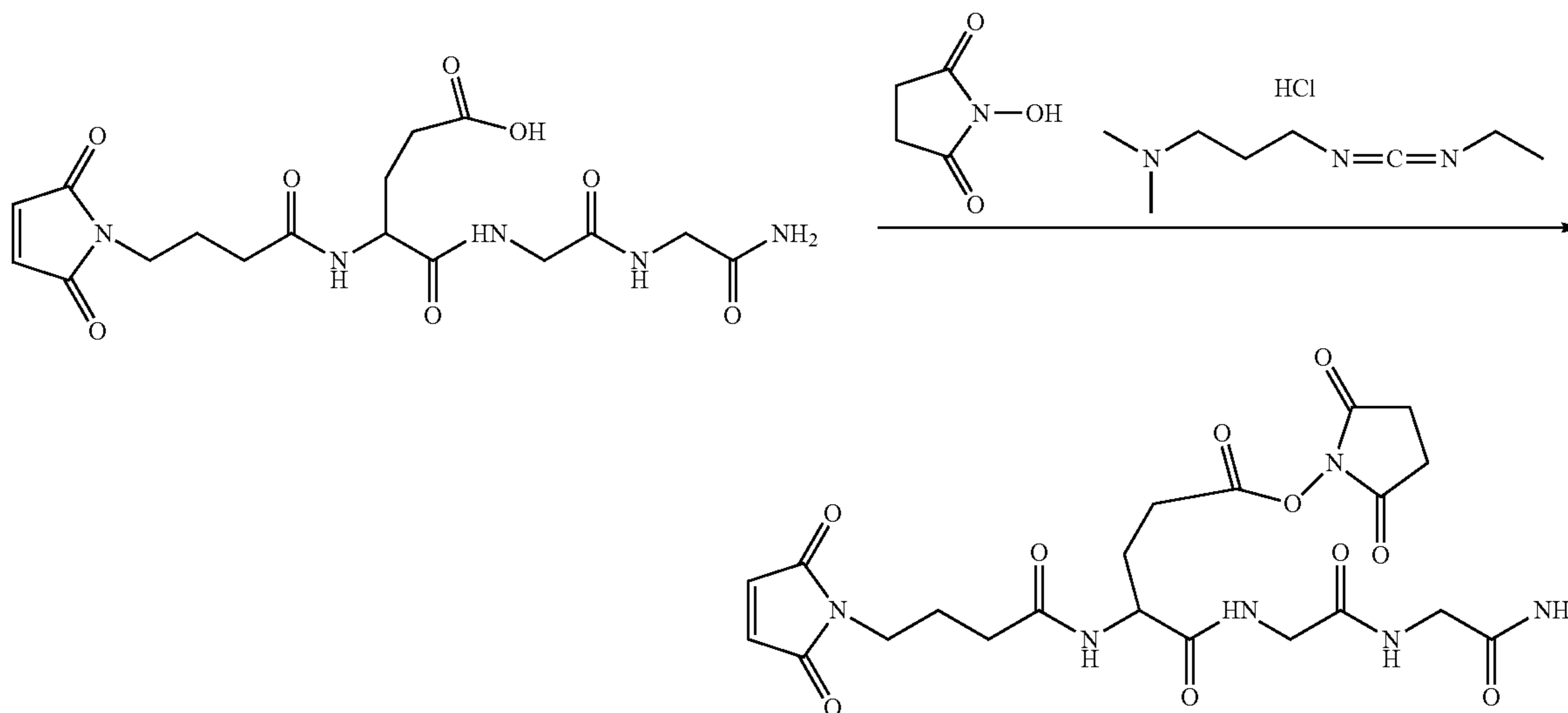
Mal-Gaba-Glu(OHNS)-Gly-Gly-NH 2
