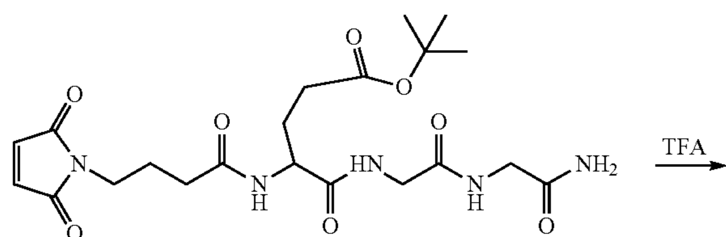
Mal-Gaba-Glu(OH)-Gly-Gly-NH 2
