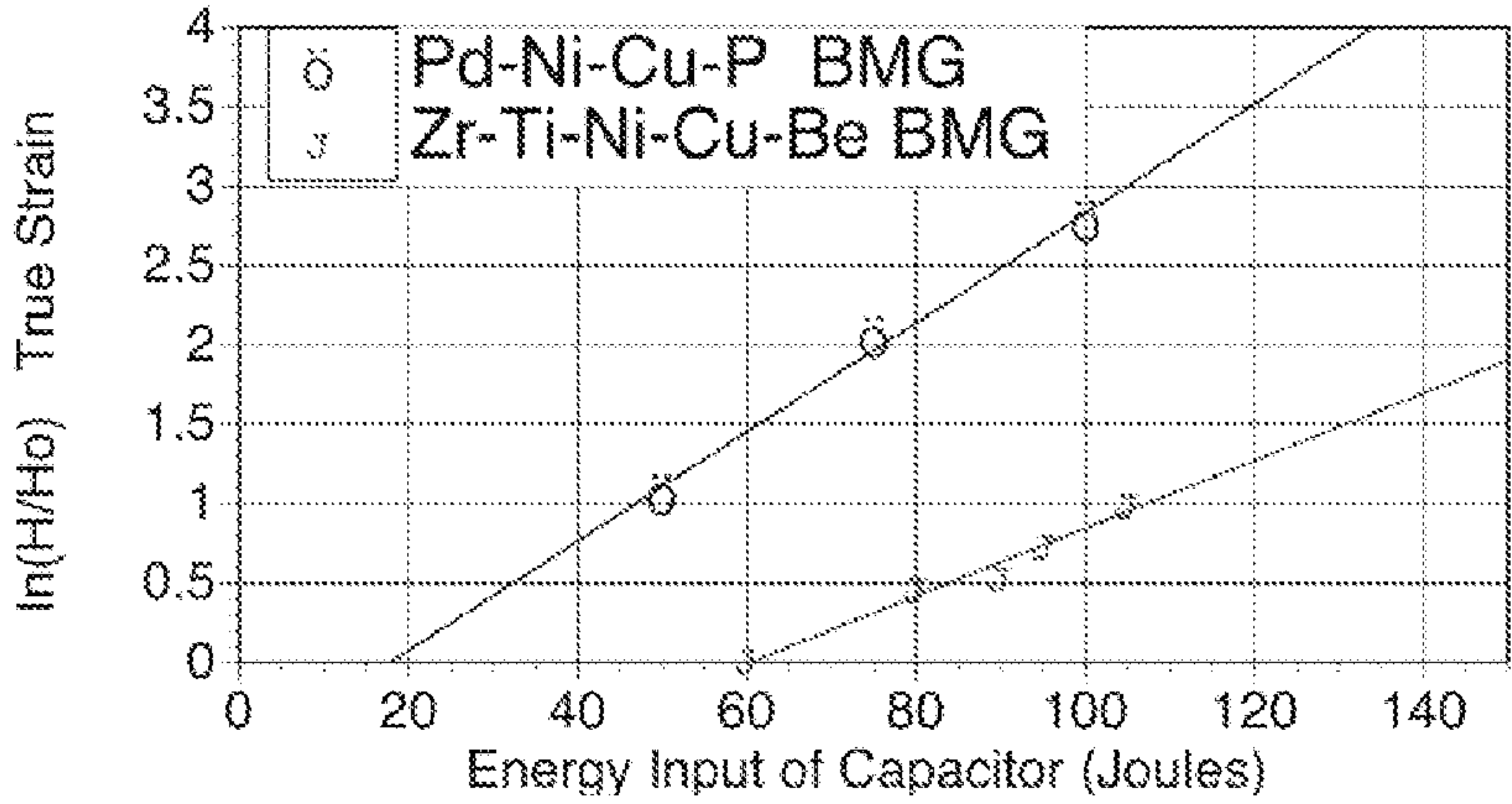
Rapid Discharge Forming of PdNiCuP & Vitreloy 1 BMG rods
