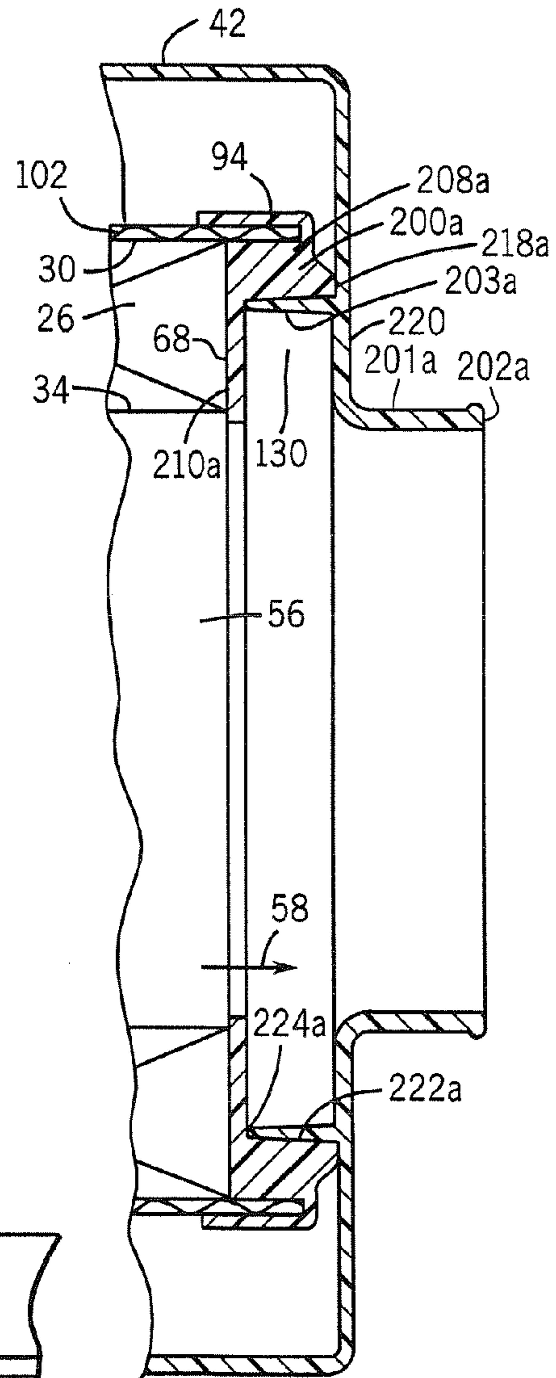
FIG. 11 PRIOR ART
