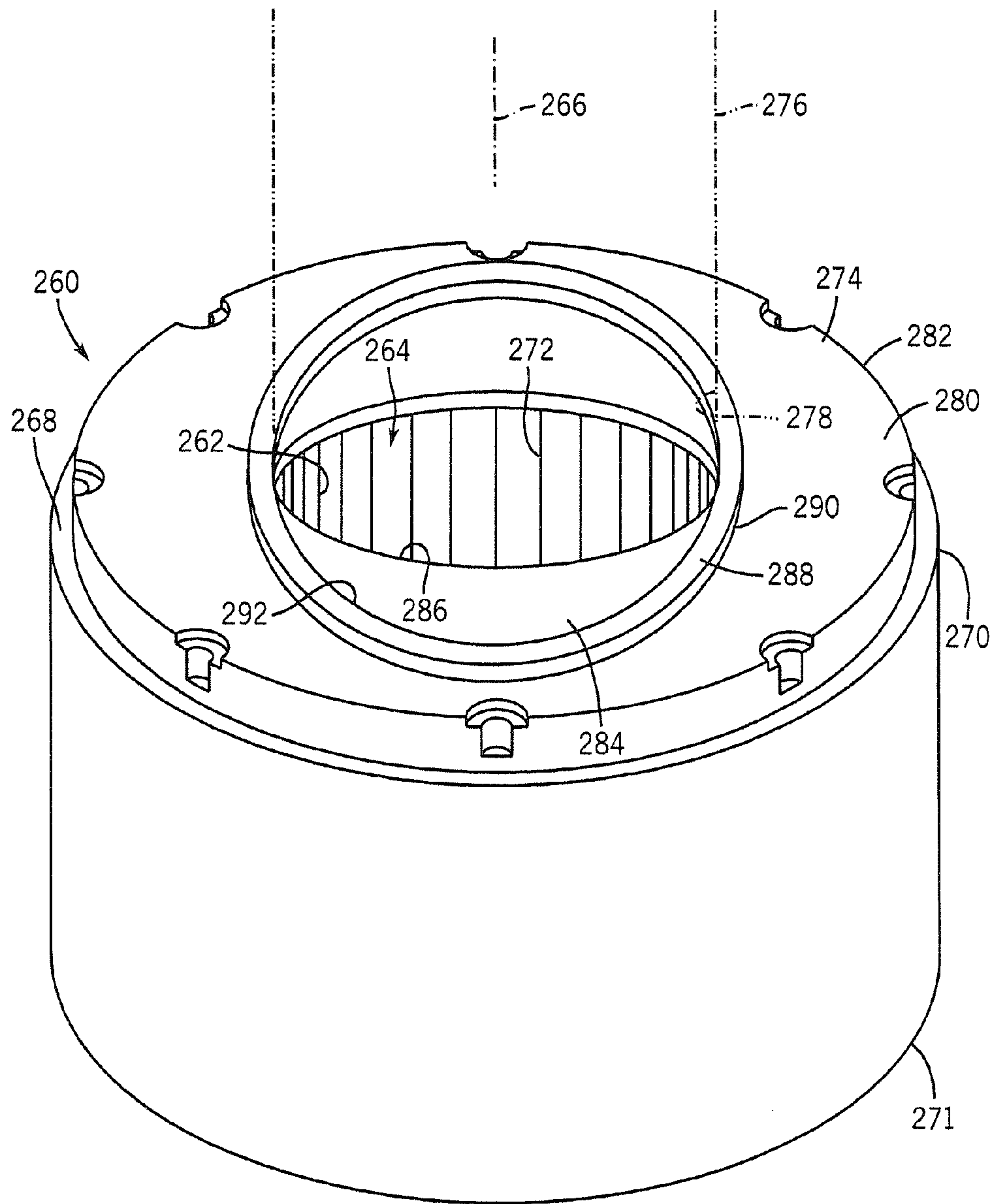
FIG. 14 PRIOR ART
