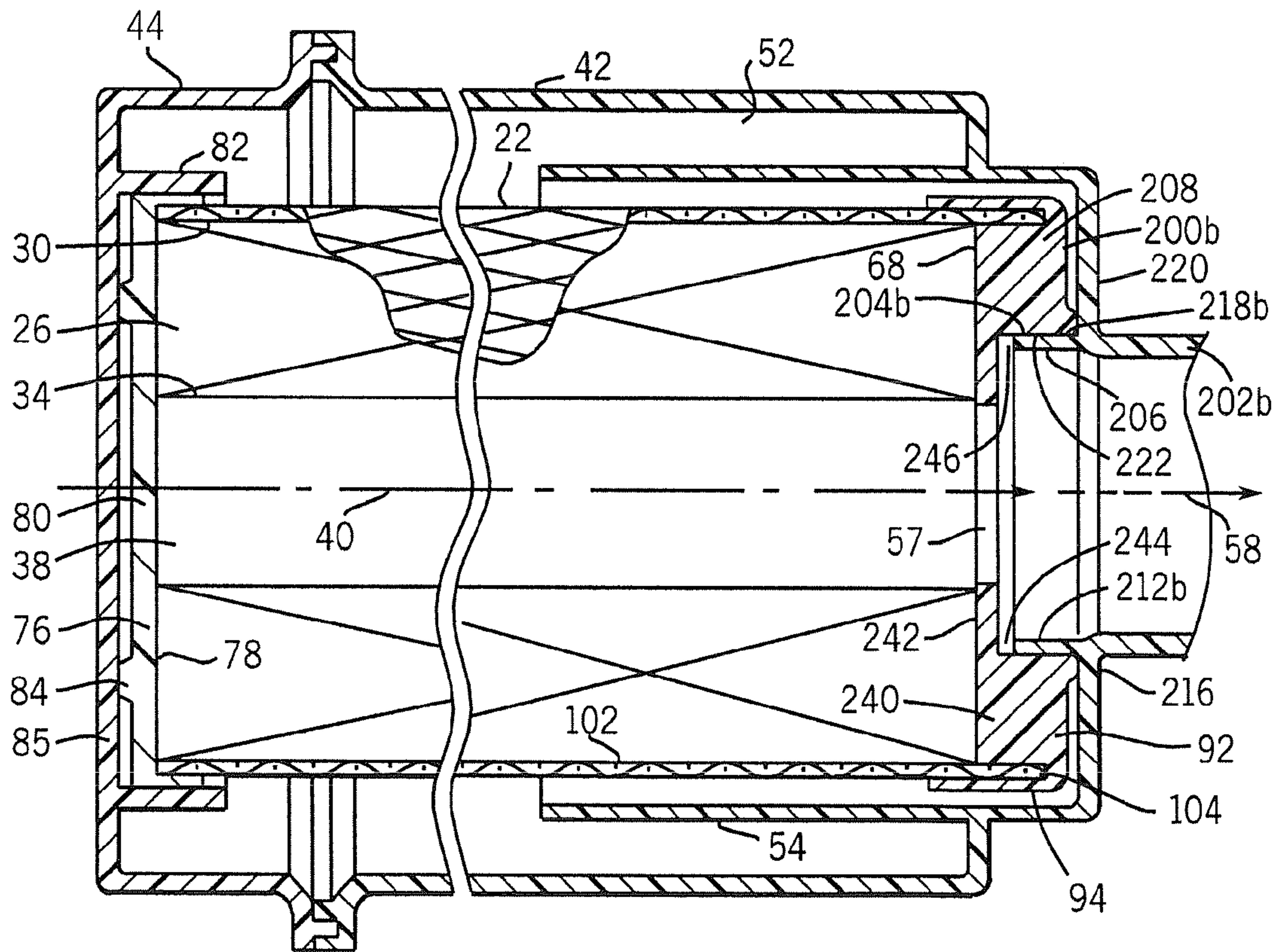
FIG. 12 PRIOR ART
