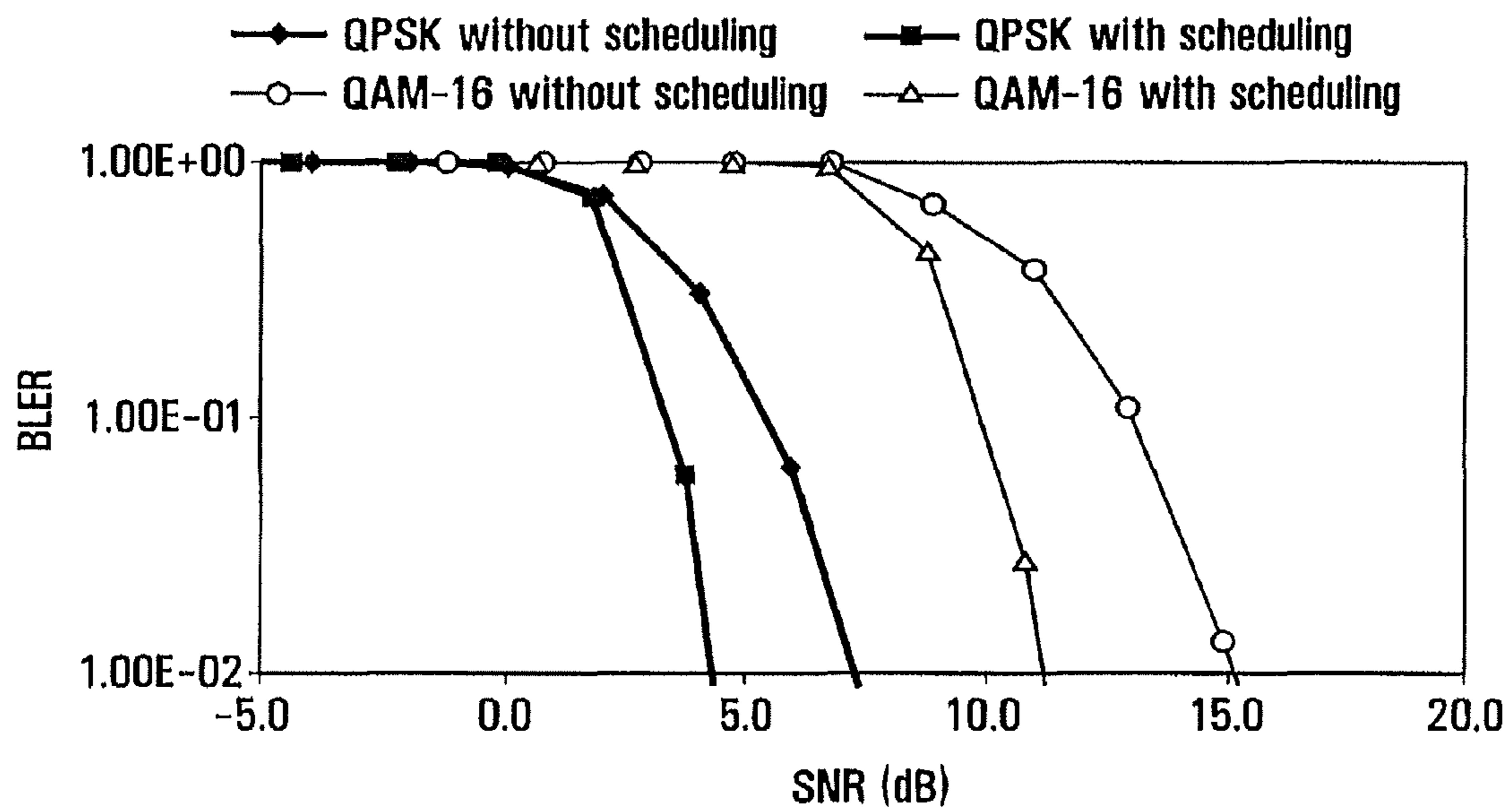
Impact on Max Capacity Scheduling (SM 2x2 MLD, 16 UEs, ITU-VA, Turbo R=1/2, 10MHz 1024-FFT, 6-Band)
