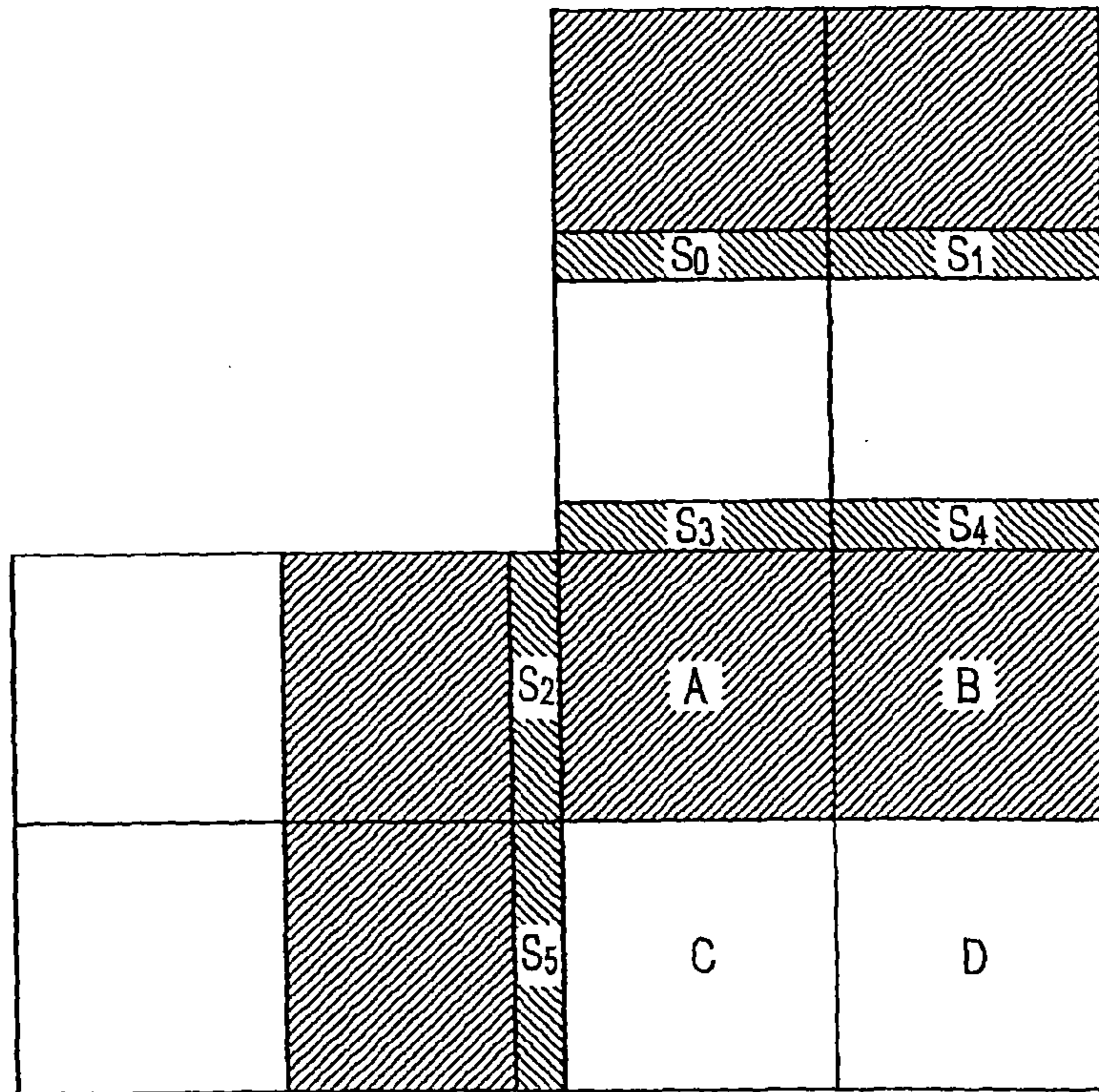
FIG. 21 BACKGROUND ART
