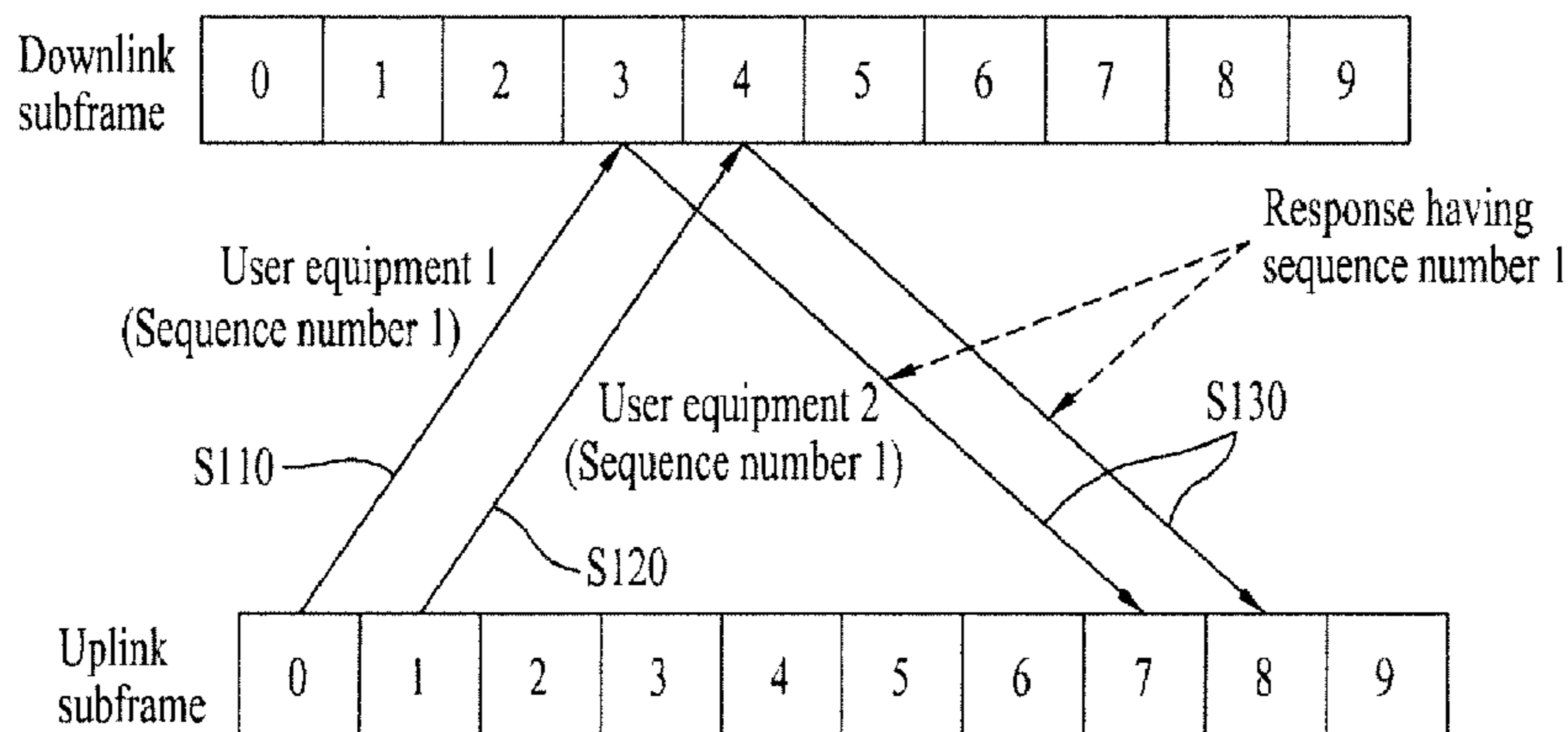
< Example of random access response >
