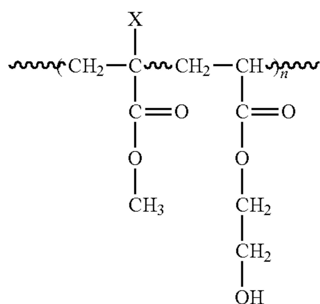
PMMA-POLYOL X is H or methyl
