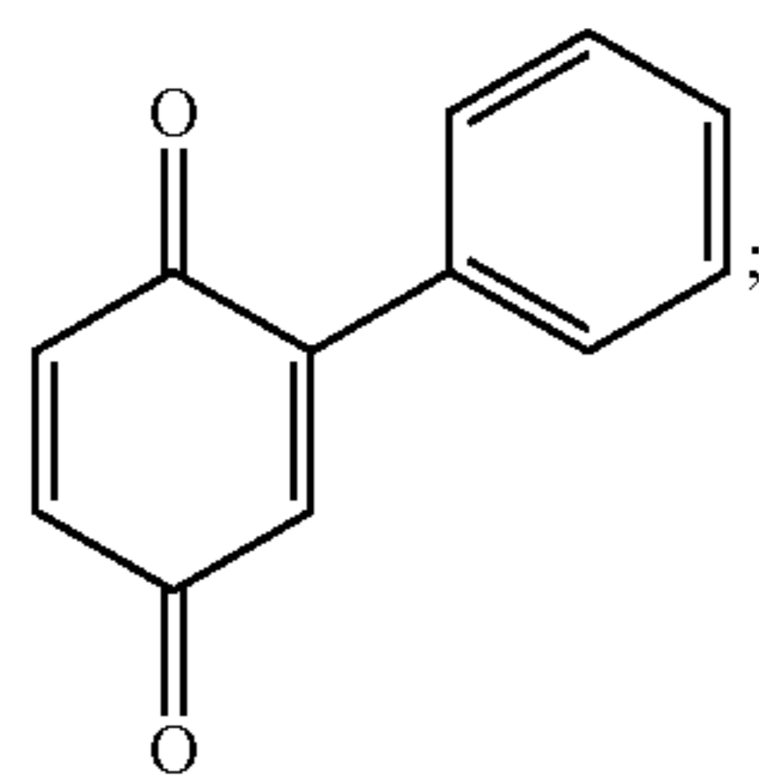
Phenyl-1,4-benzoquinone
