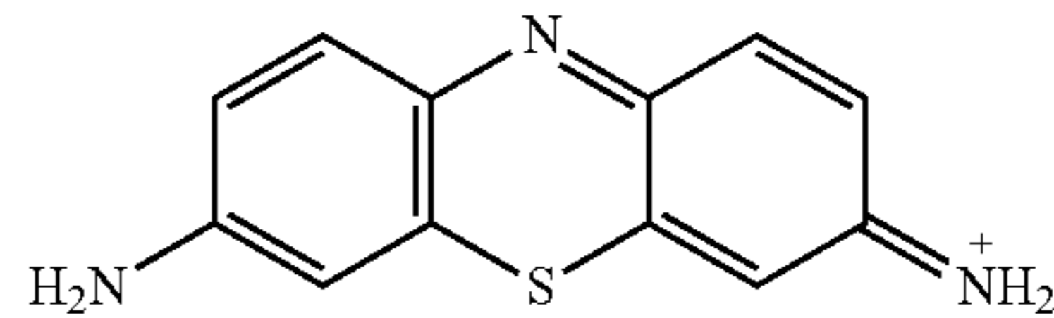
Thionin ("TH")
