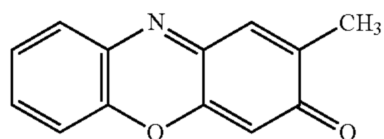
2-methylphenoxazin-3-one ("MPOZ")
