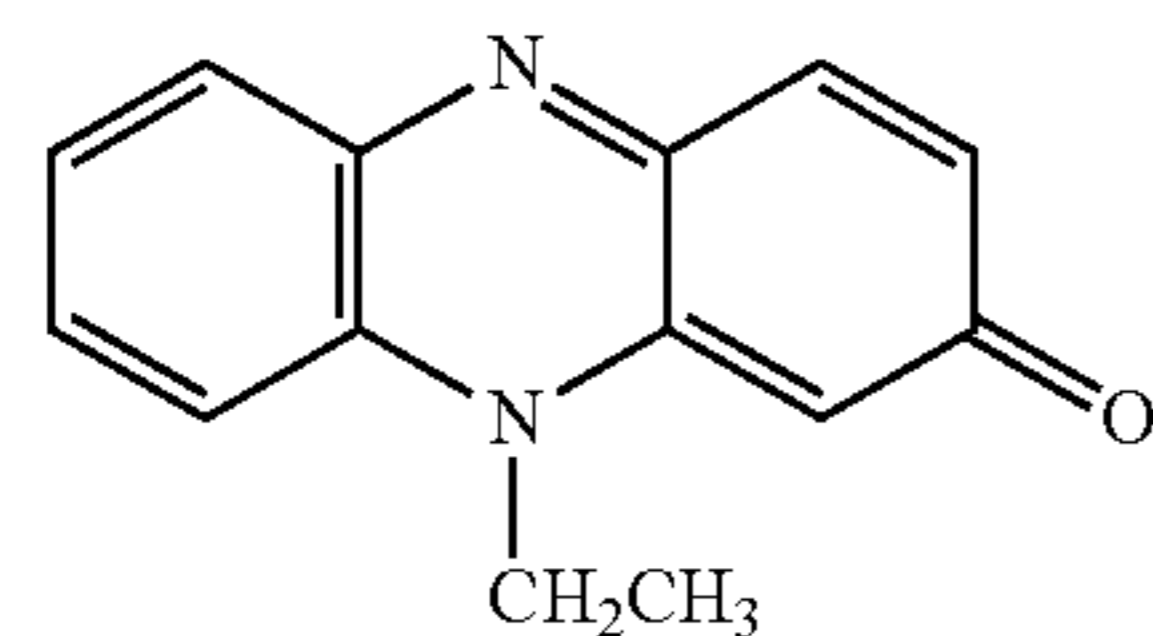
2-keto-N-ethylphenazine ("KEPA")
