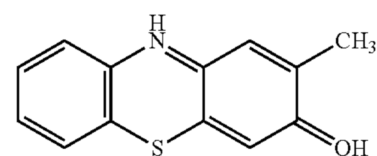
("RMPT")
