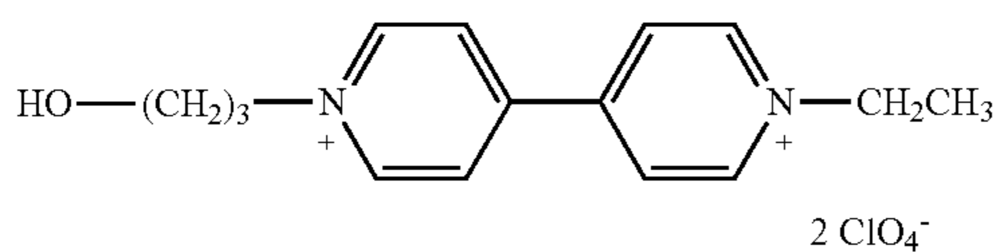
Ethylhydroxypropylviologen Perchlorate ("EHPVCIO 4 ")
