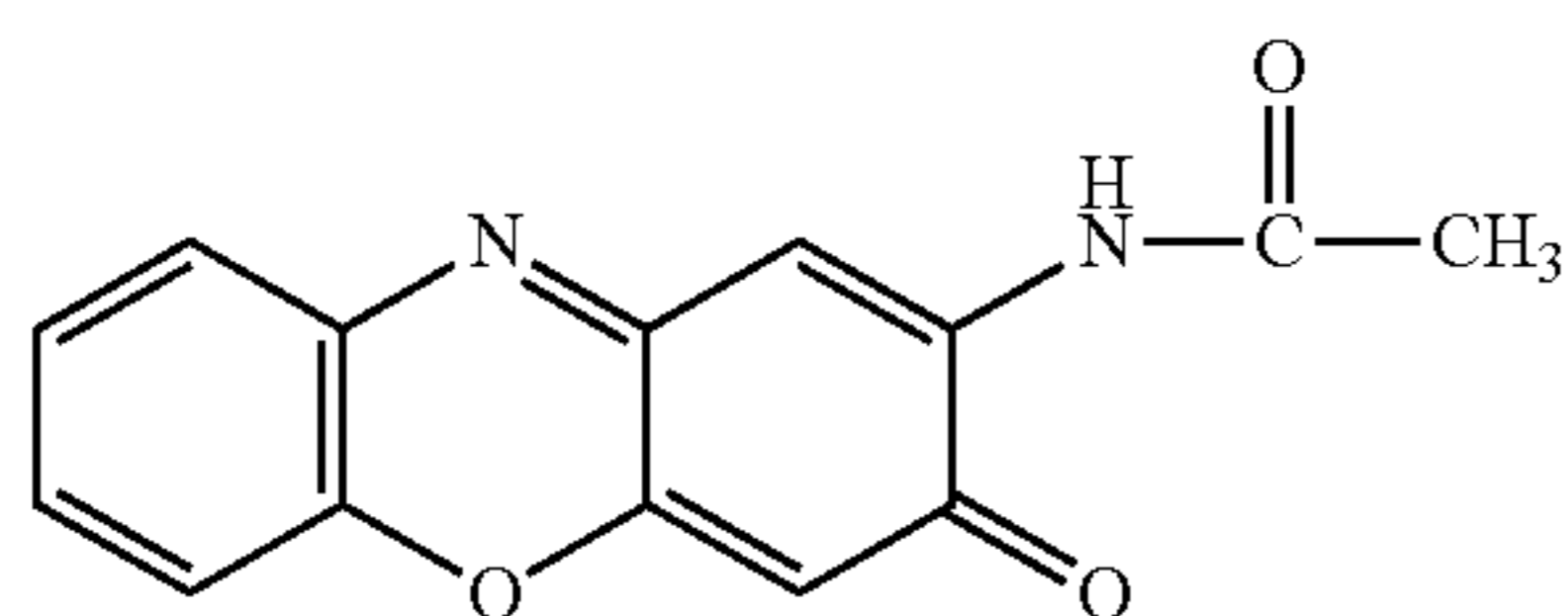
2-acetylaminophenoxazin-3-one ("AAPOZ")
