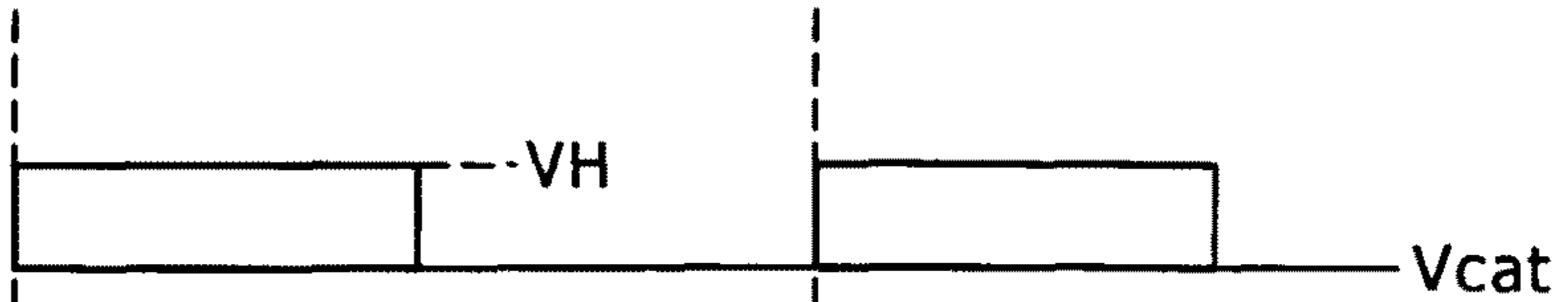
FIG. 39A DUTY 50%
