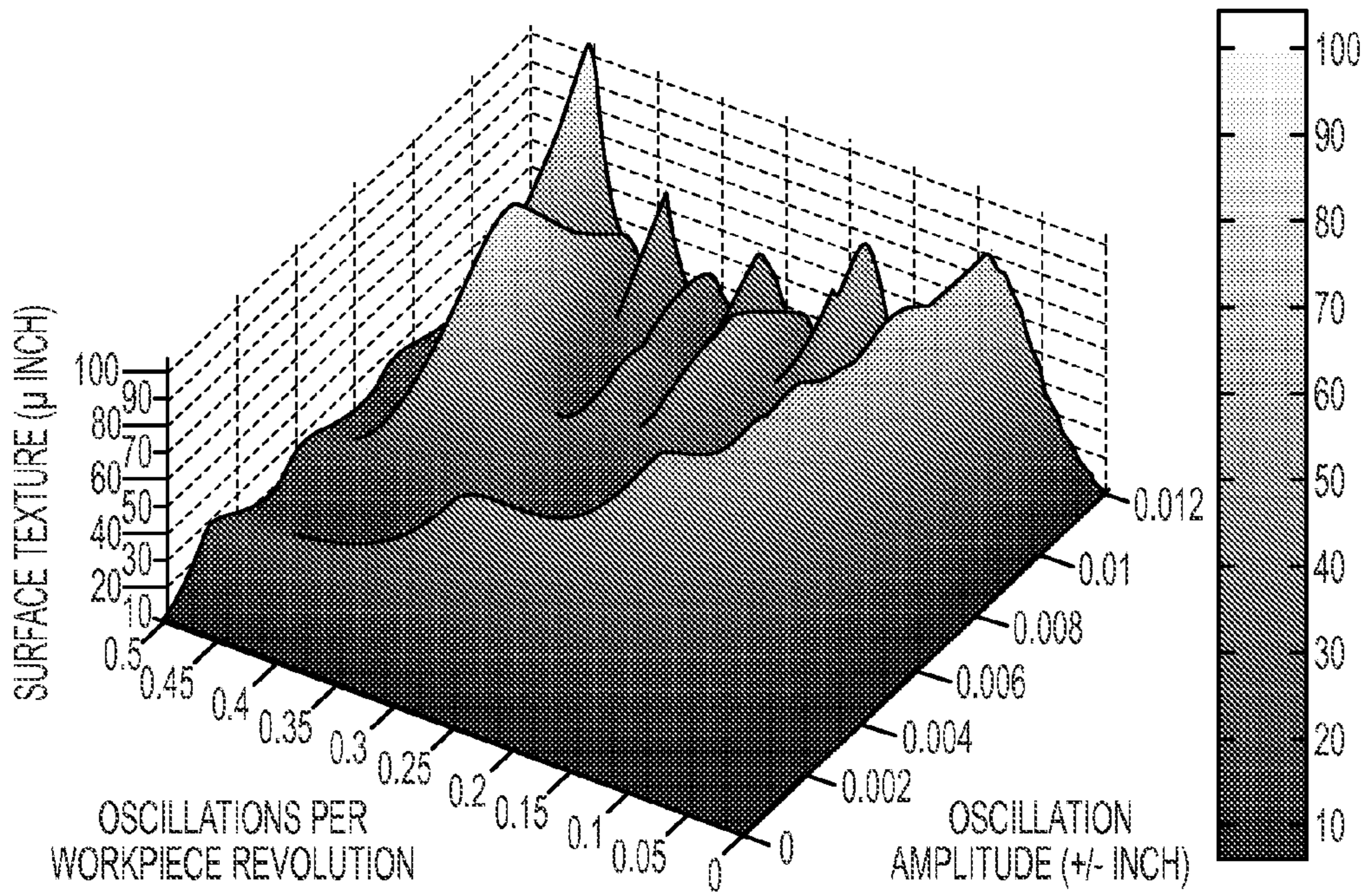
3D PLOT OF SURFACE TEXTURE VALUES CORRESPONDING TO A RANGE OF OPR AND OSCILLATION AMPLITUDES. 0.031 INCH TOOL NOSE RADIUS AND 0.003 INCH FEED PER REVOLUTION.
