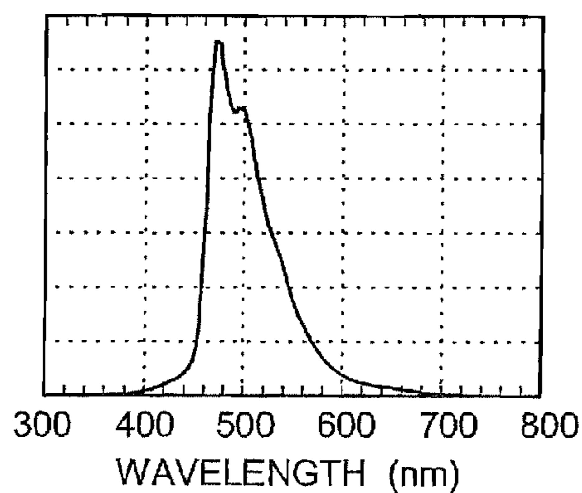
FIG. 8D LIGHT EMISSION SPECTRUM
