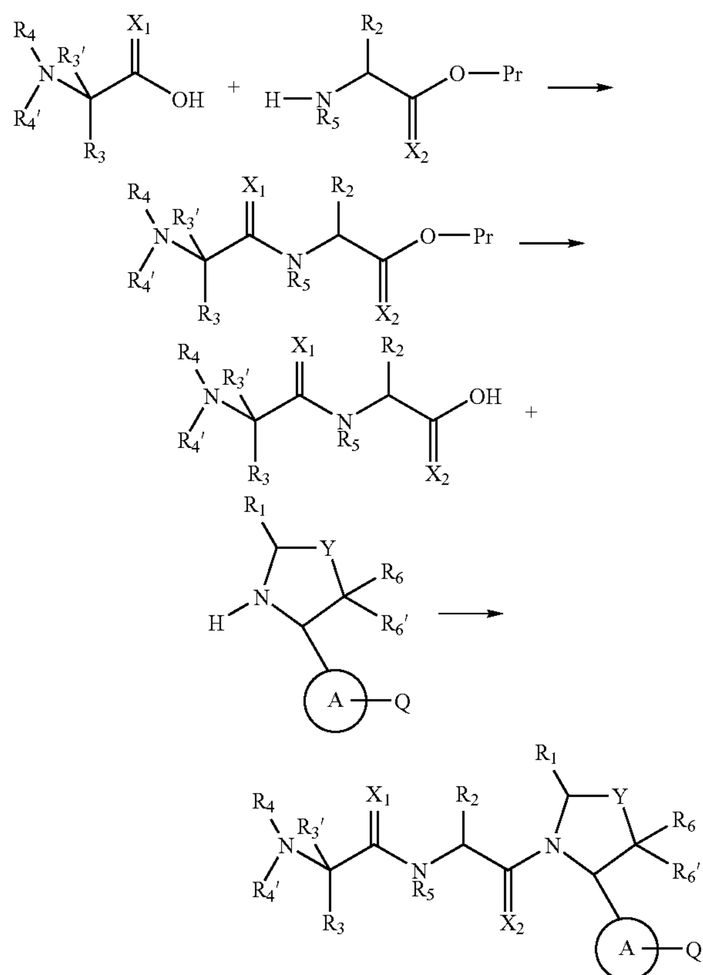
Scheme 2
