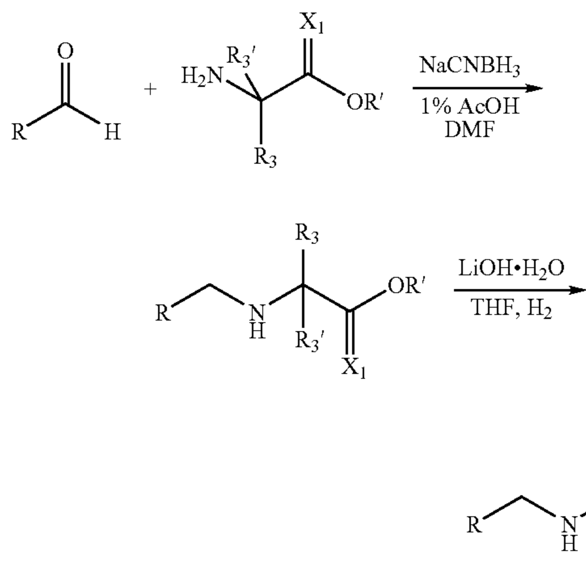
Scheme 5
