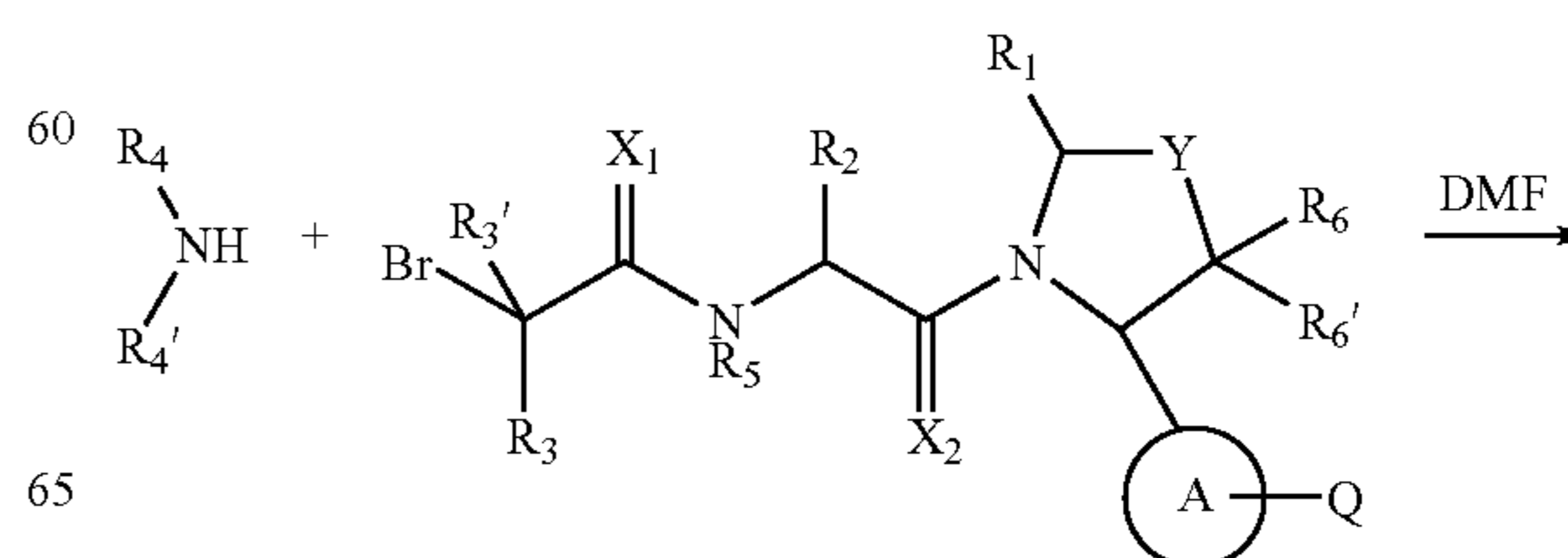
Scheme 8
