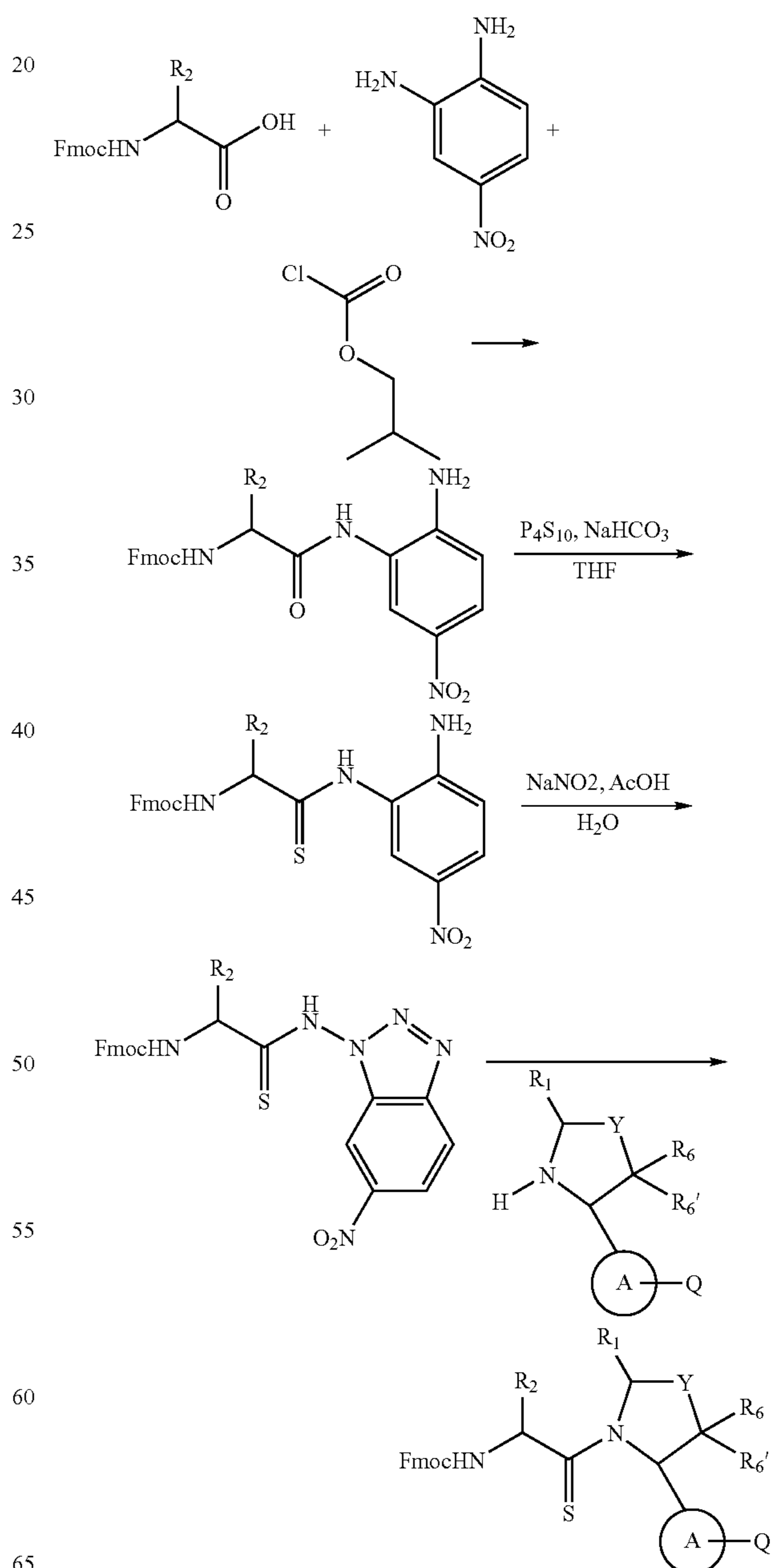
Scheme 9
