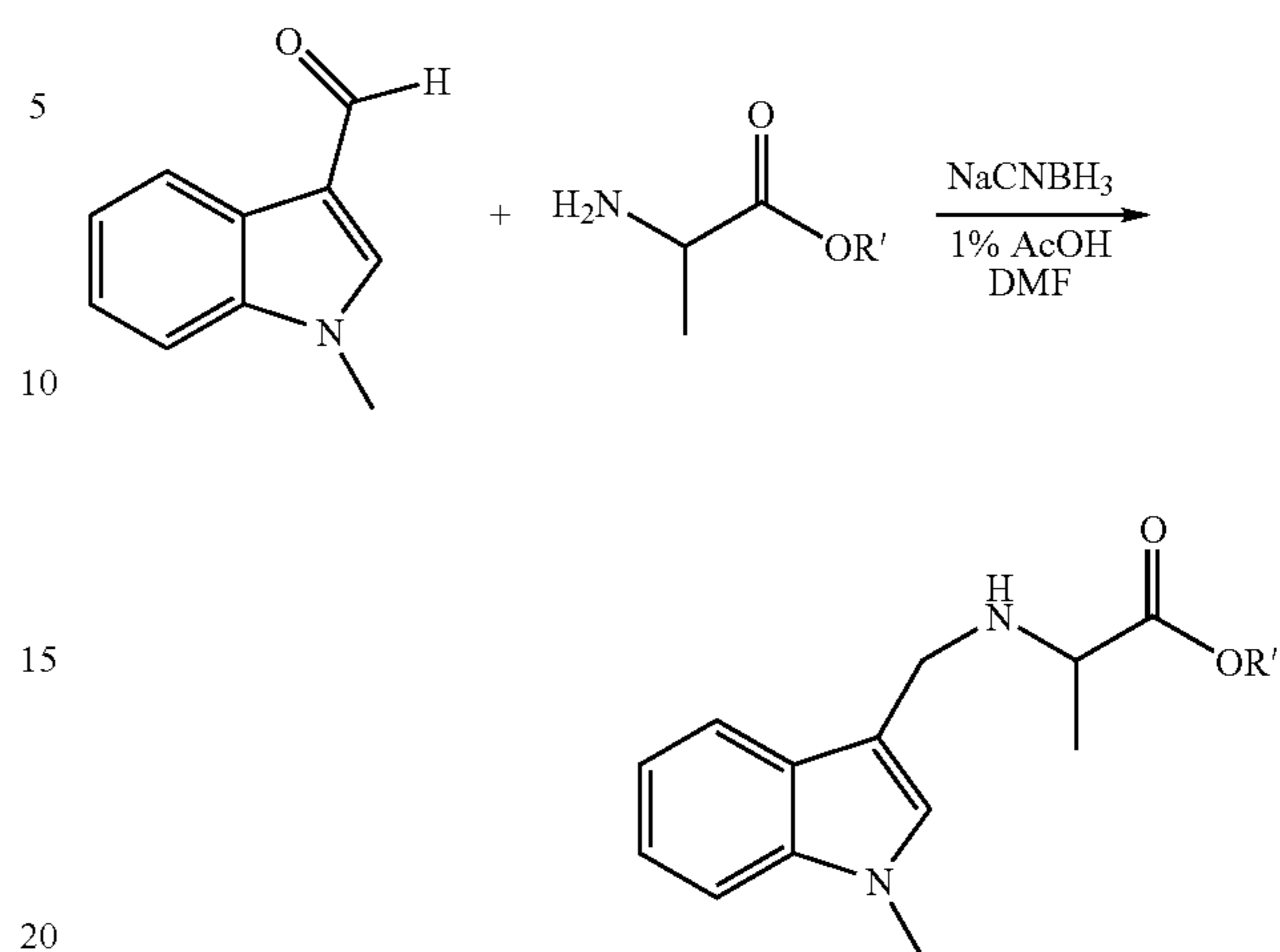
Scheme 6
