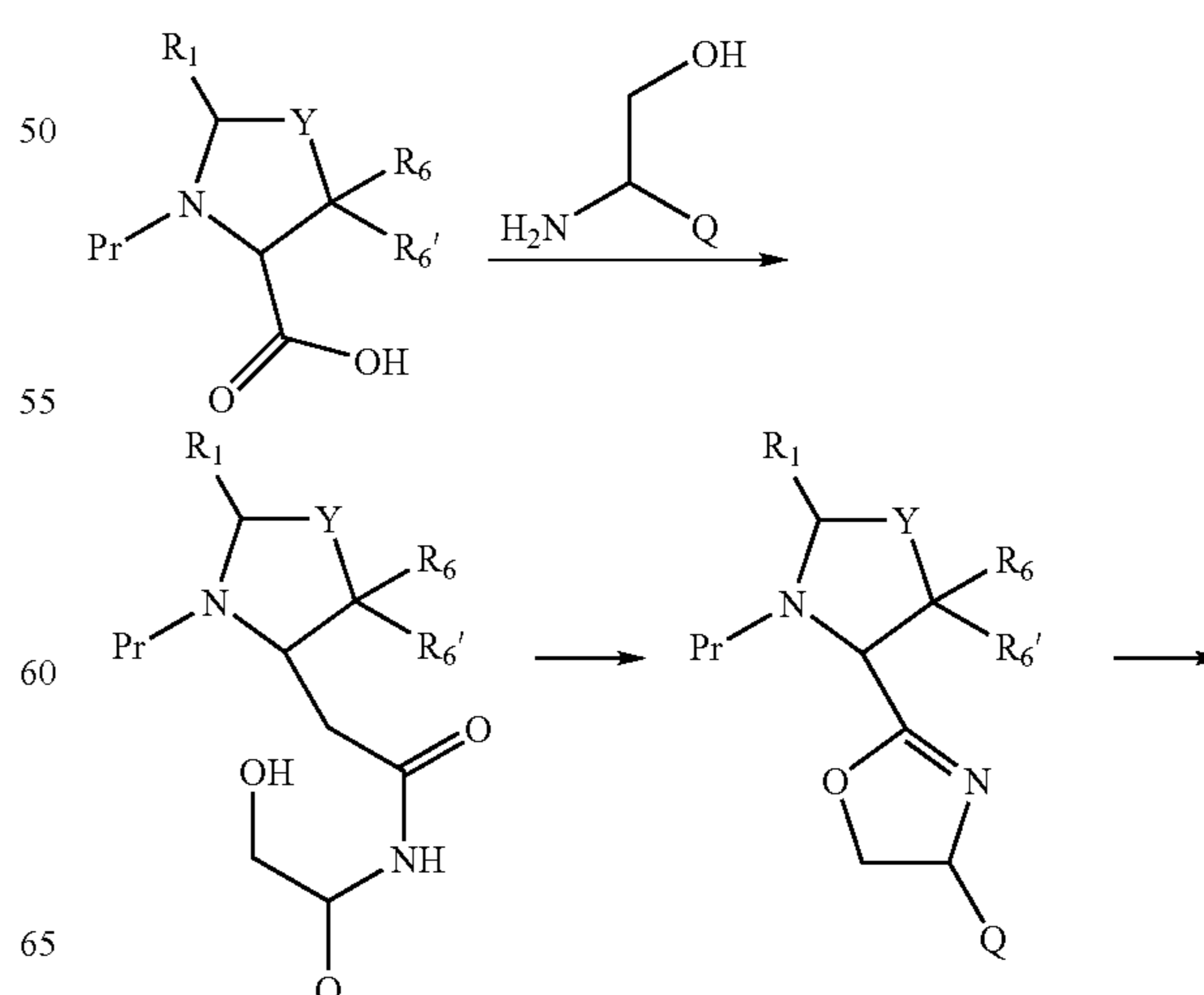
Scheme 4
