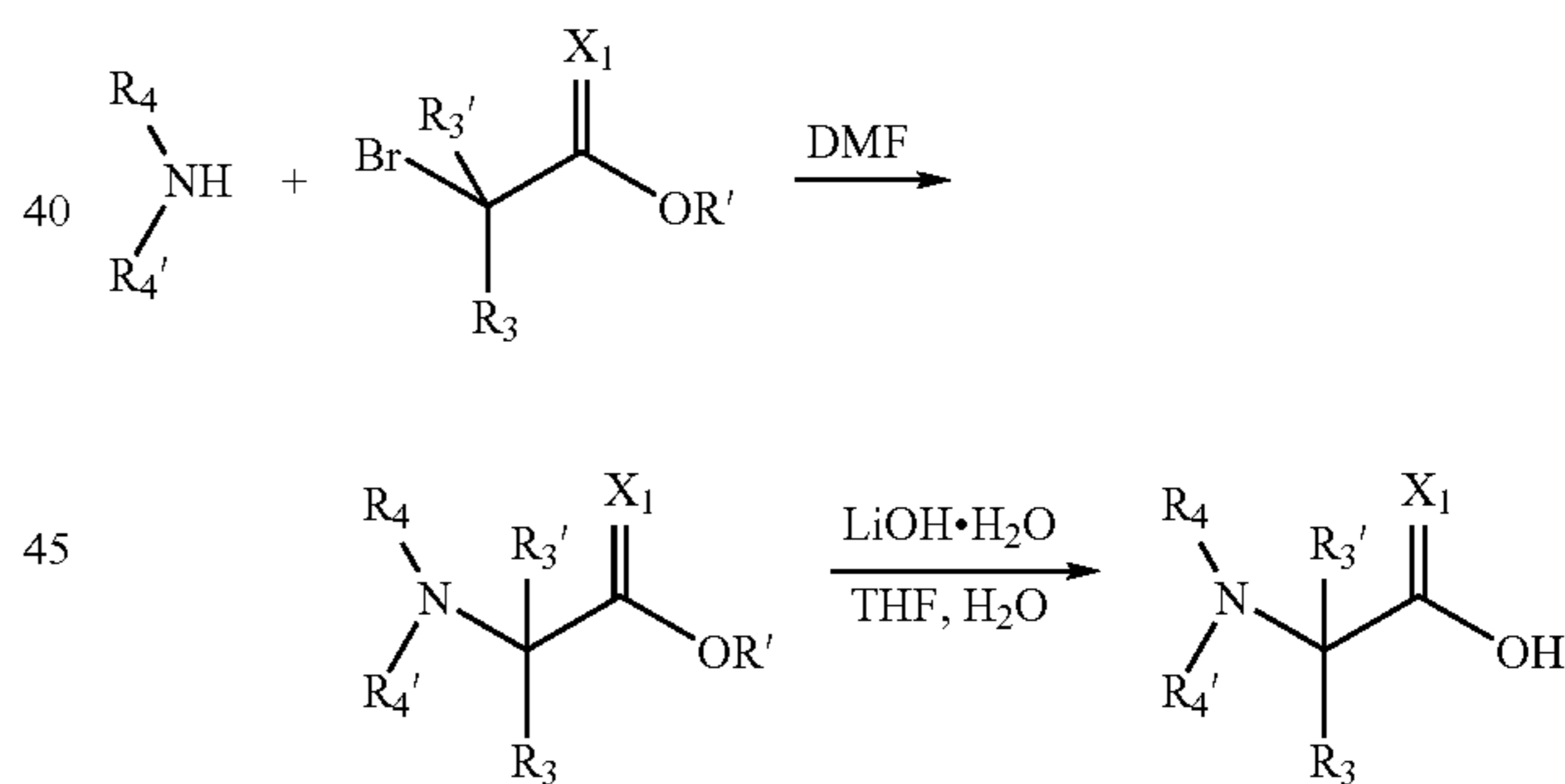
Scheme 7
