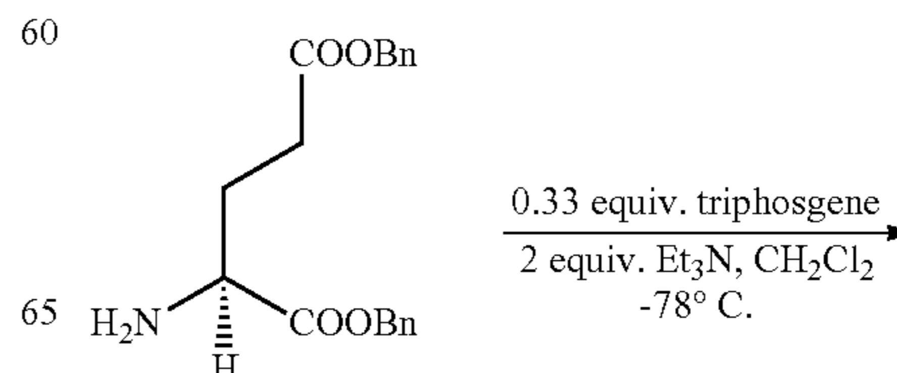
Scheme 2. Synthesis of unsymmetrical ureas, AA-C(O)-AA'.
