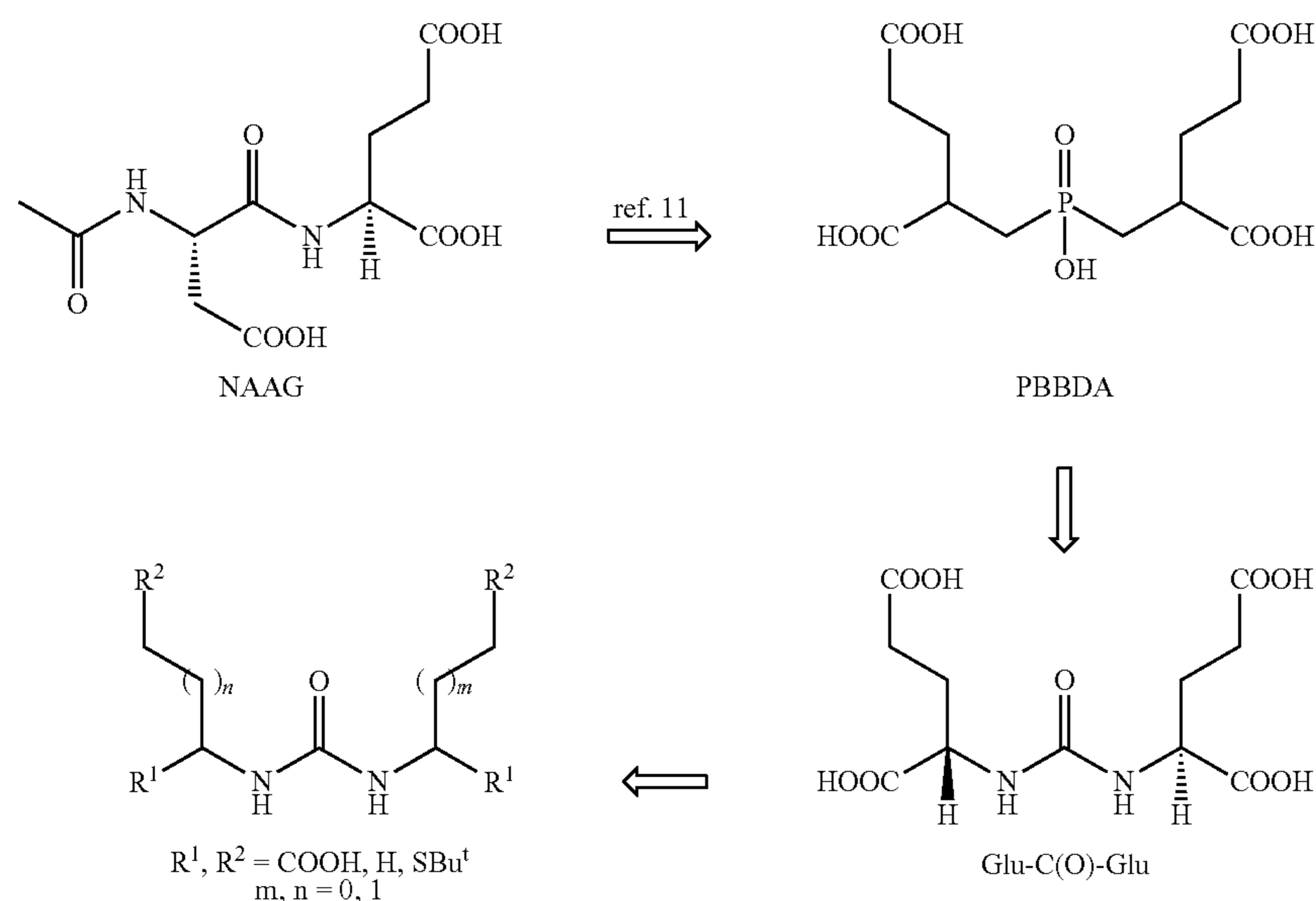
Scheme 1. Rational design of urea based GCPII inhibitors.
