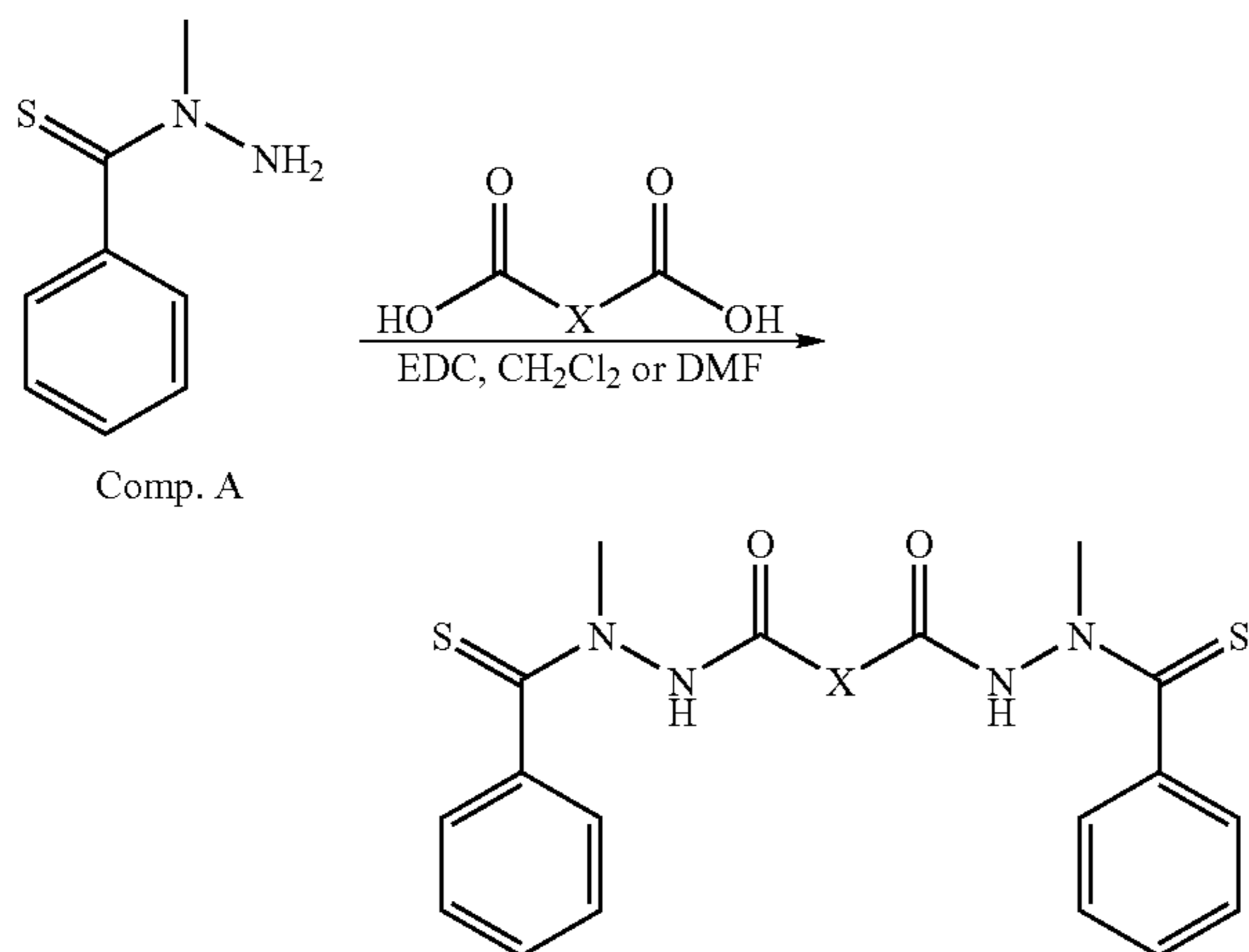
Scheme A
