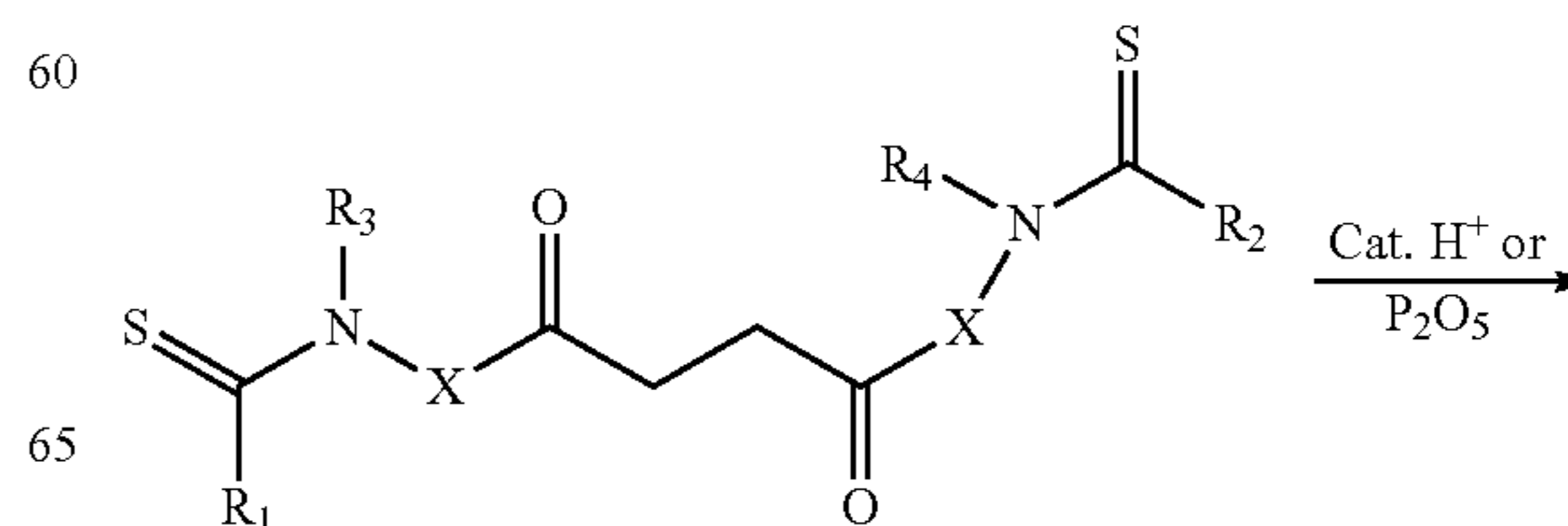
Scheme X:
