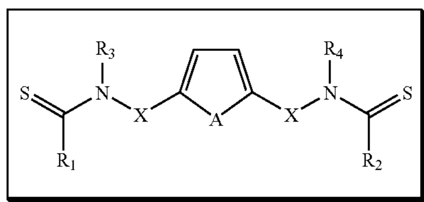
Scheme X:
