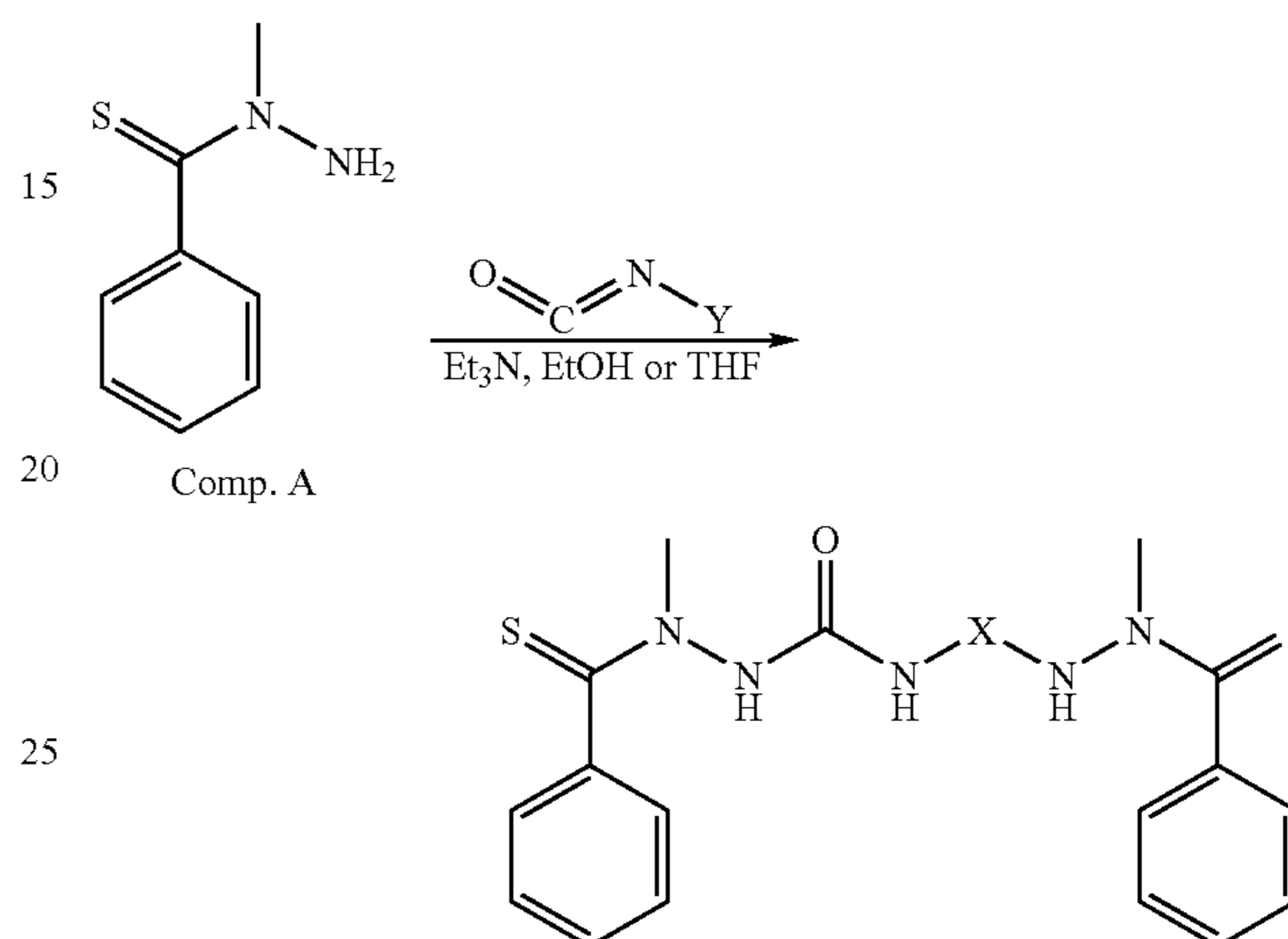
Scheme B
