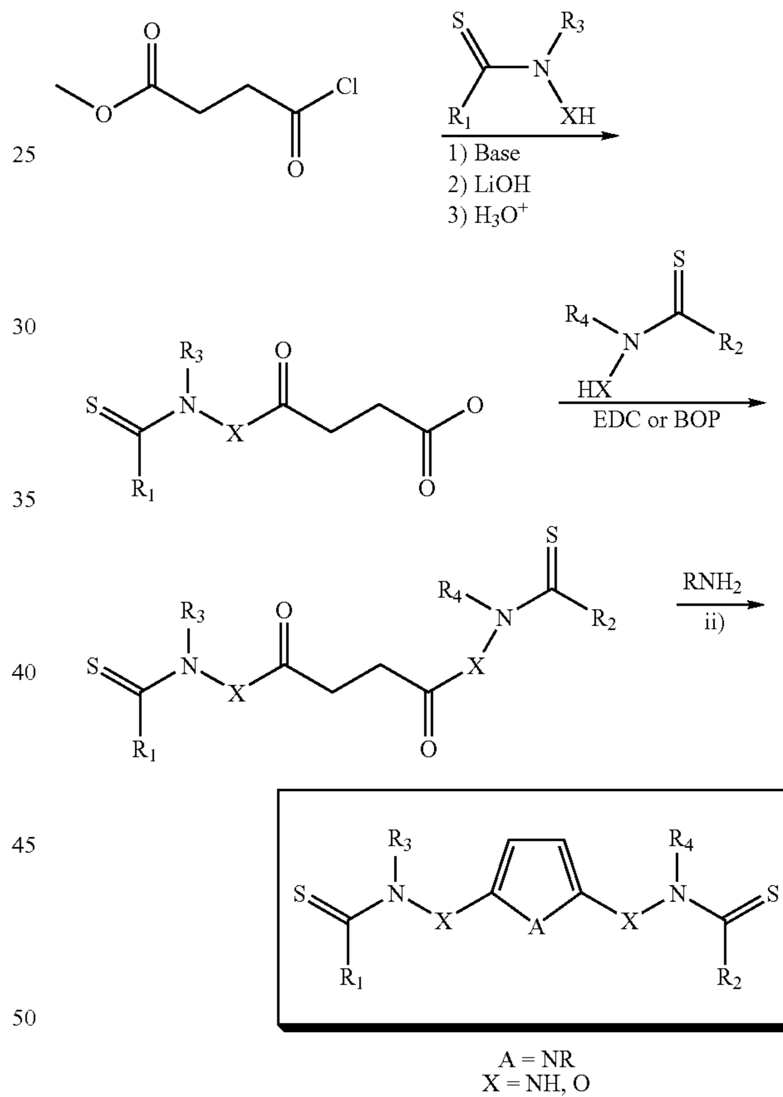
Scheme IX:
