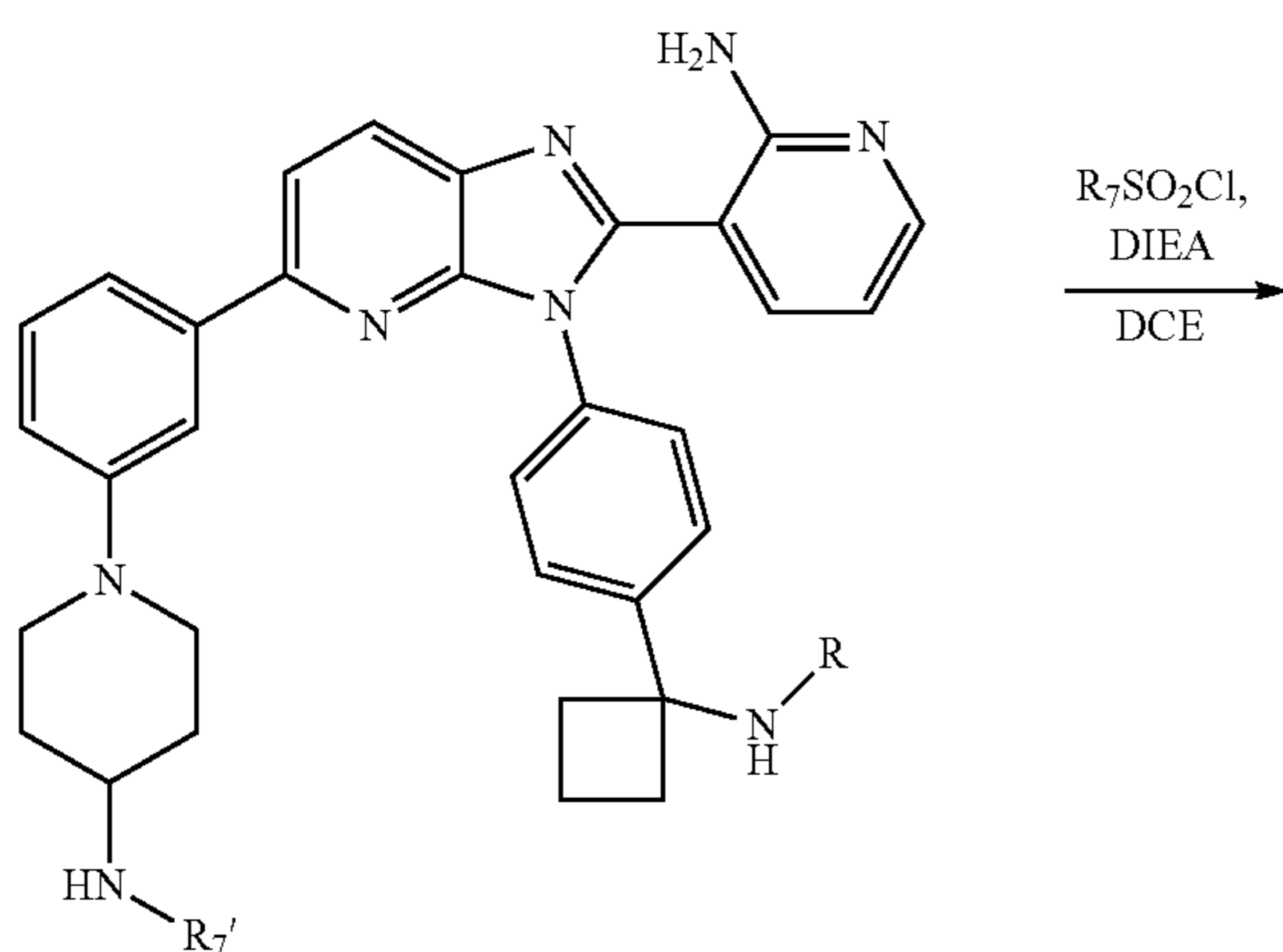
Scheme 4: Sulfonamide formation
