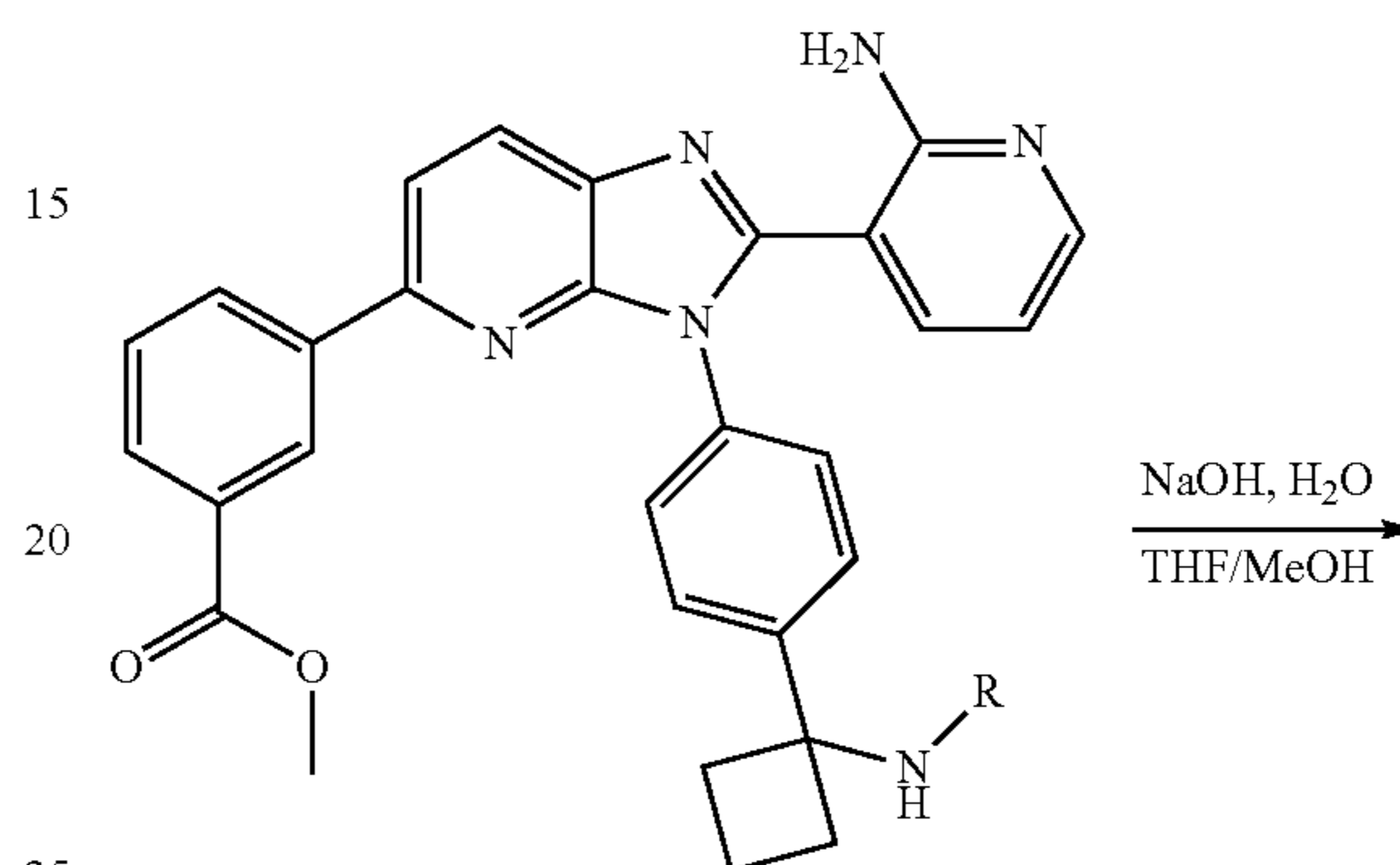
Scheme 5: Saponification
