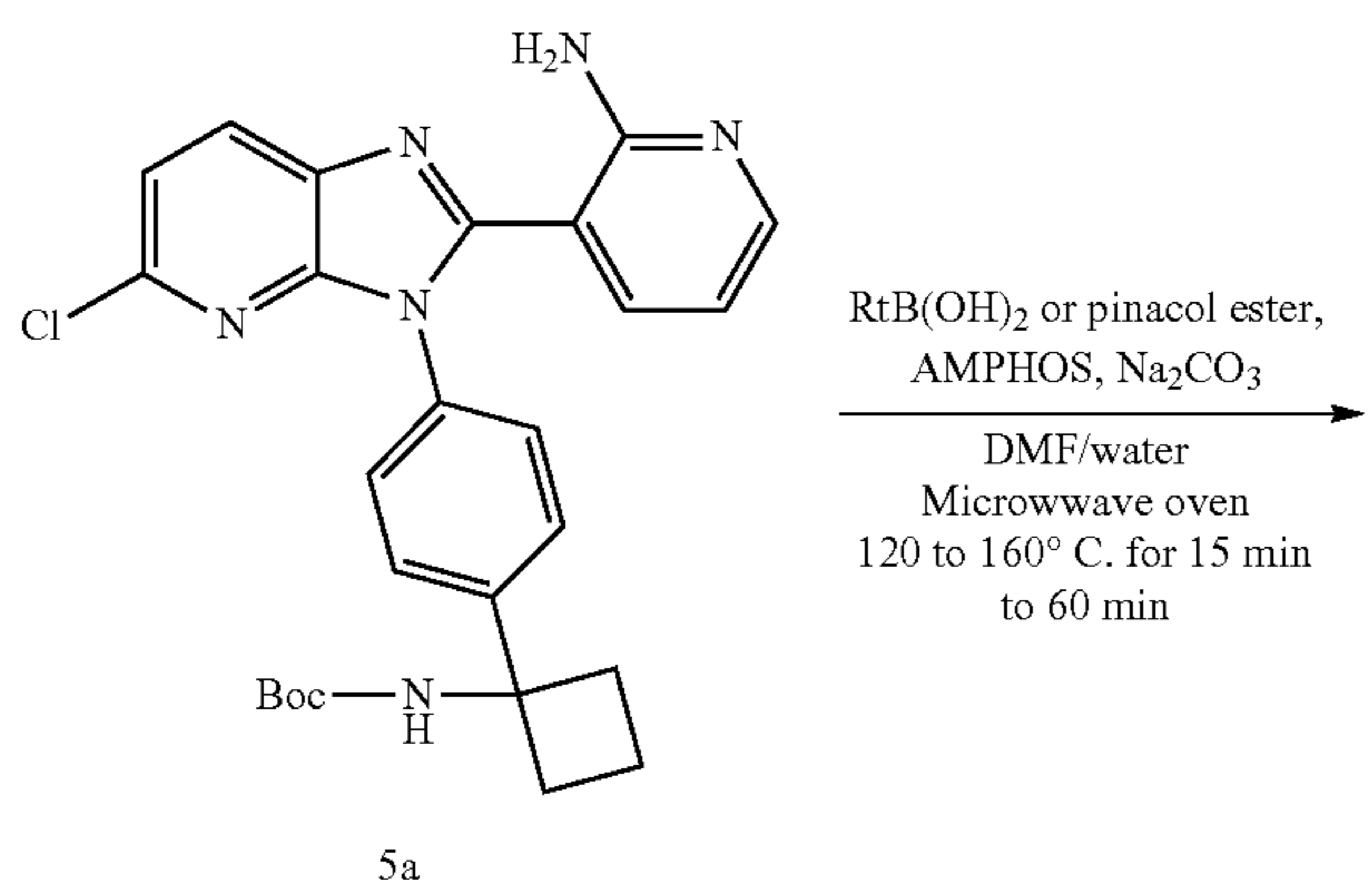
Scheme 7: Suzuki coupling 2
