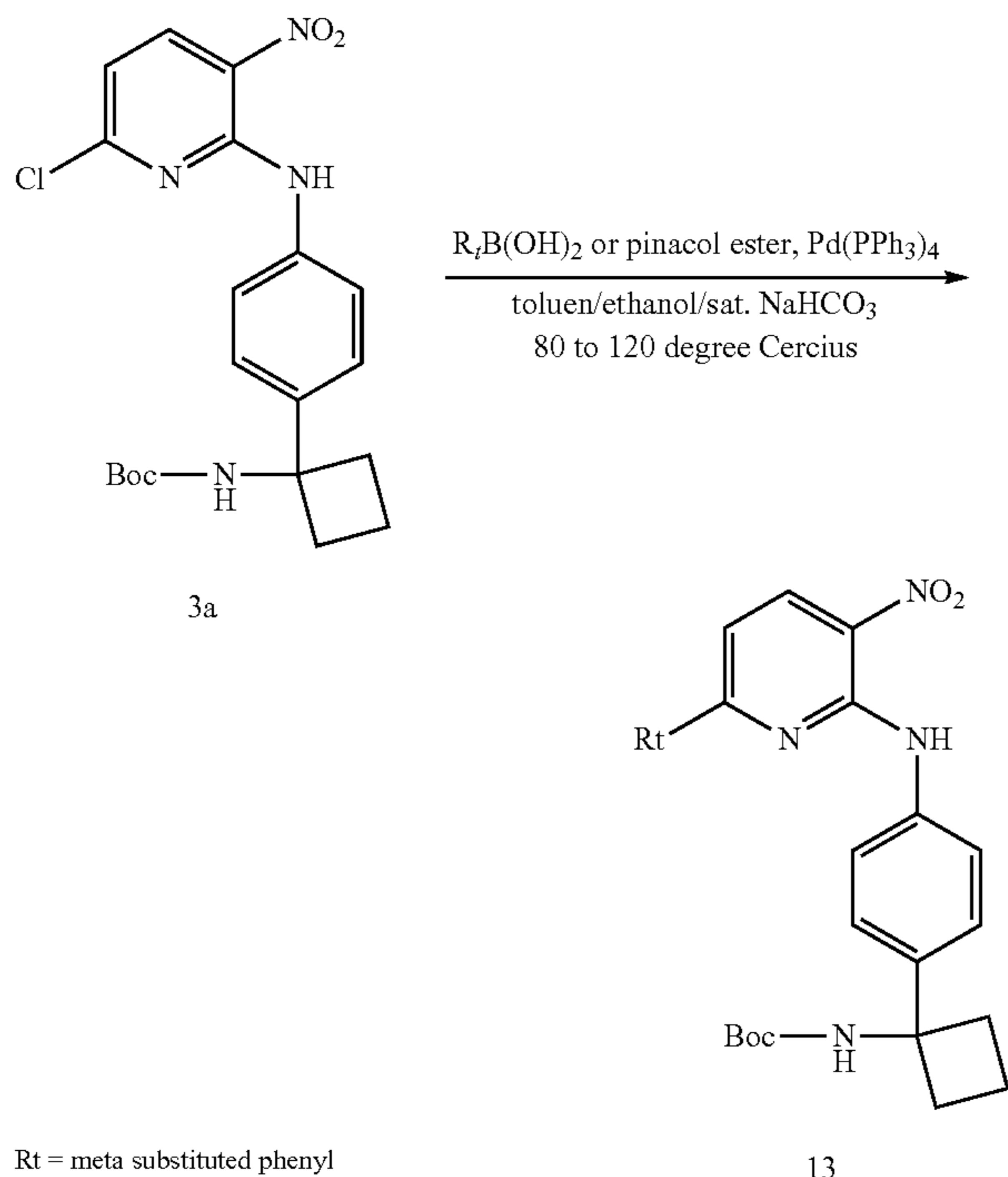
Scheme 6: Suzuki coupling 1
