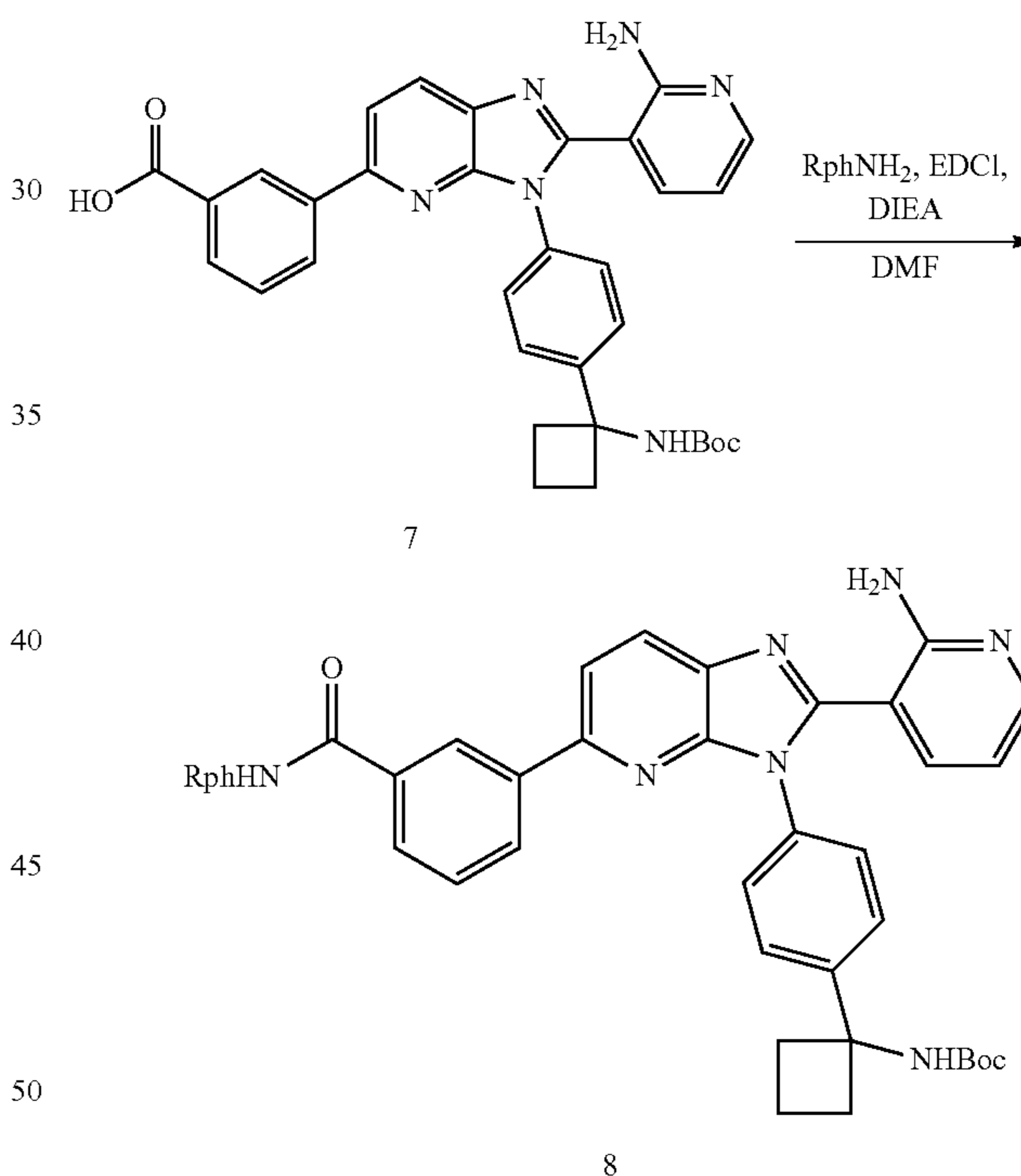
Scheme 3: Amido formation
