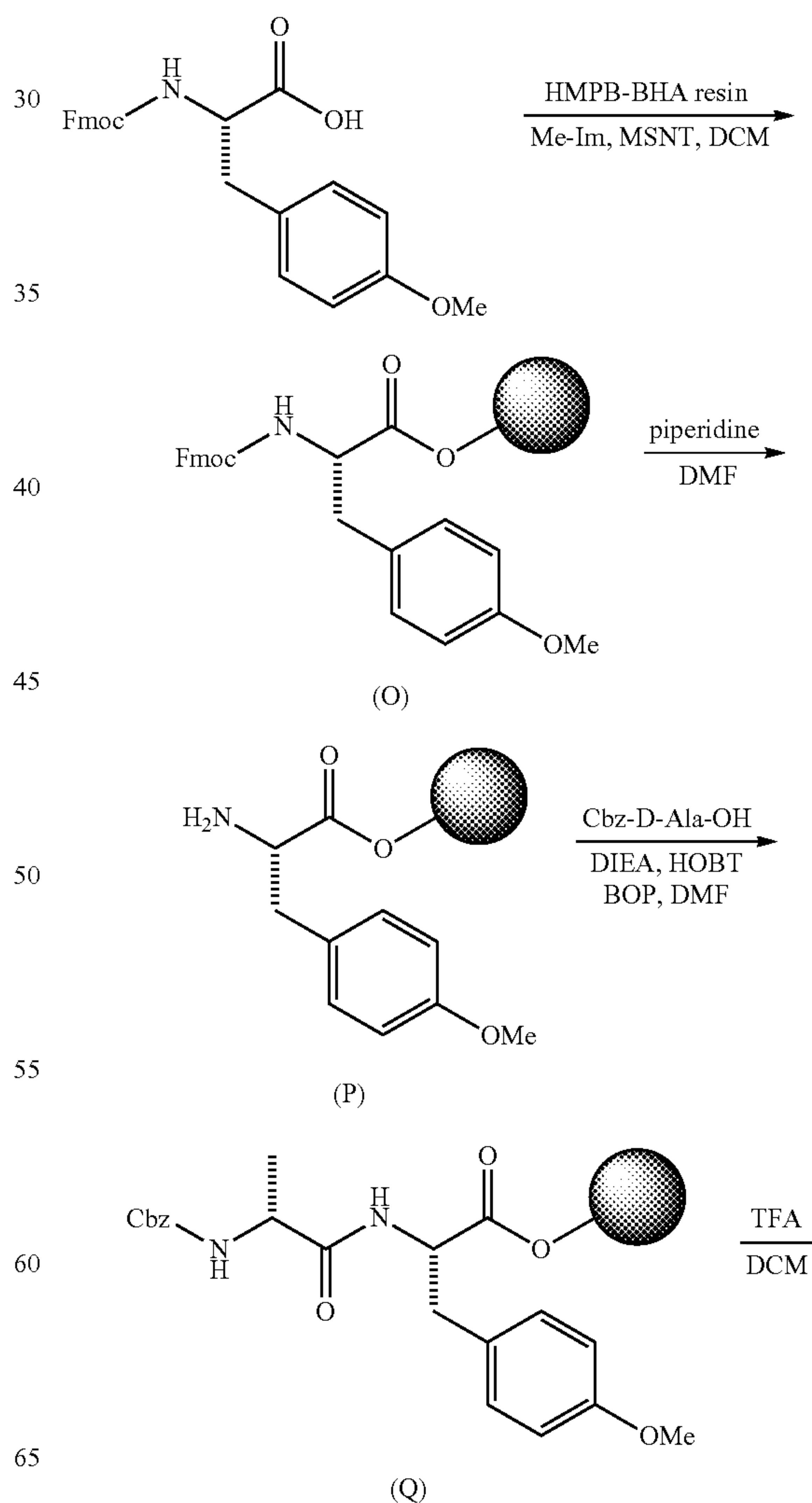
Scheme 3: Synthesis of Example 3
