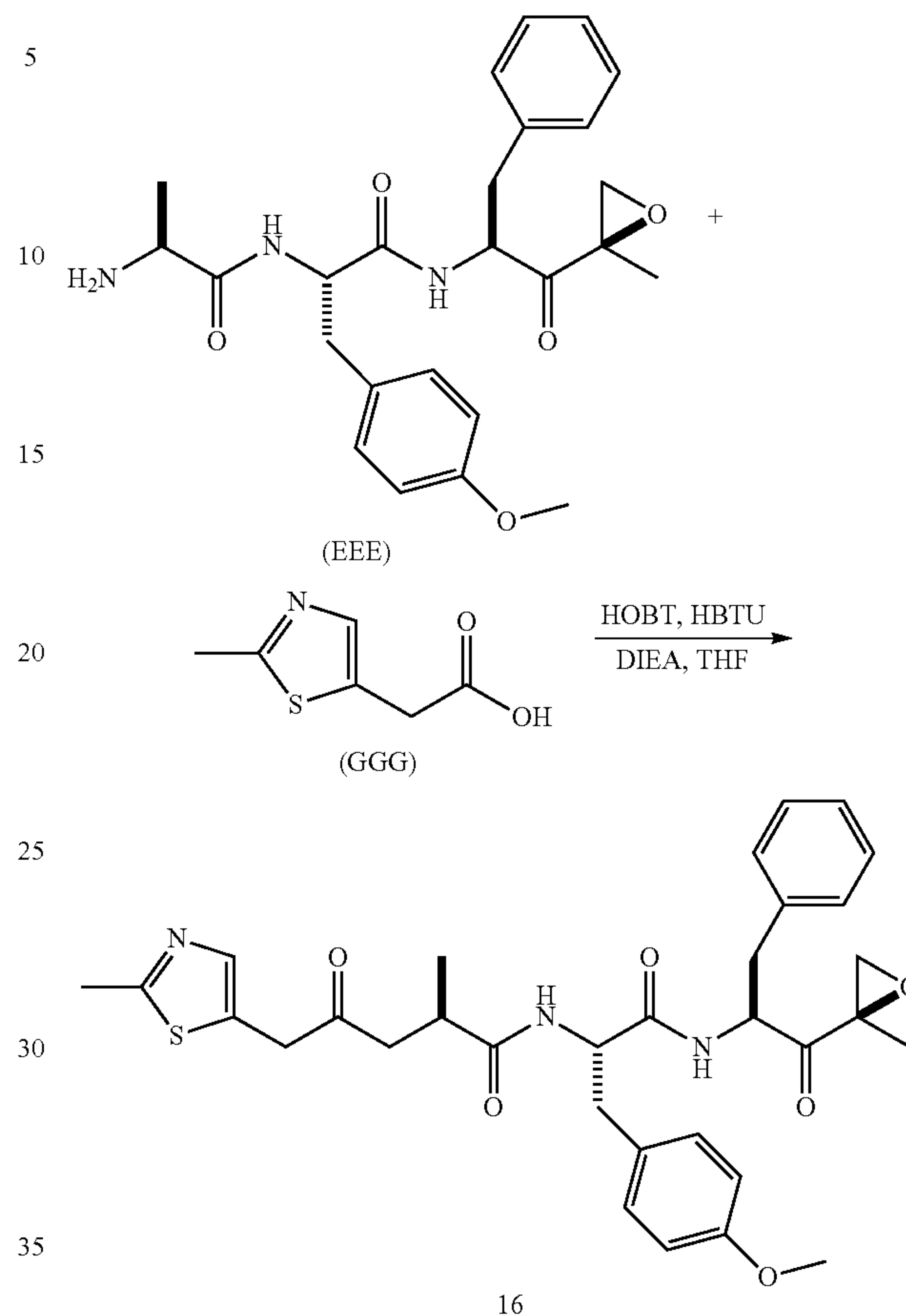
Scheme 16: Synthesis of Example 16
