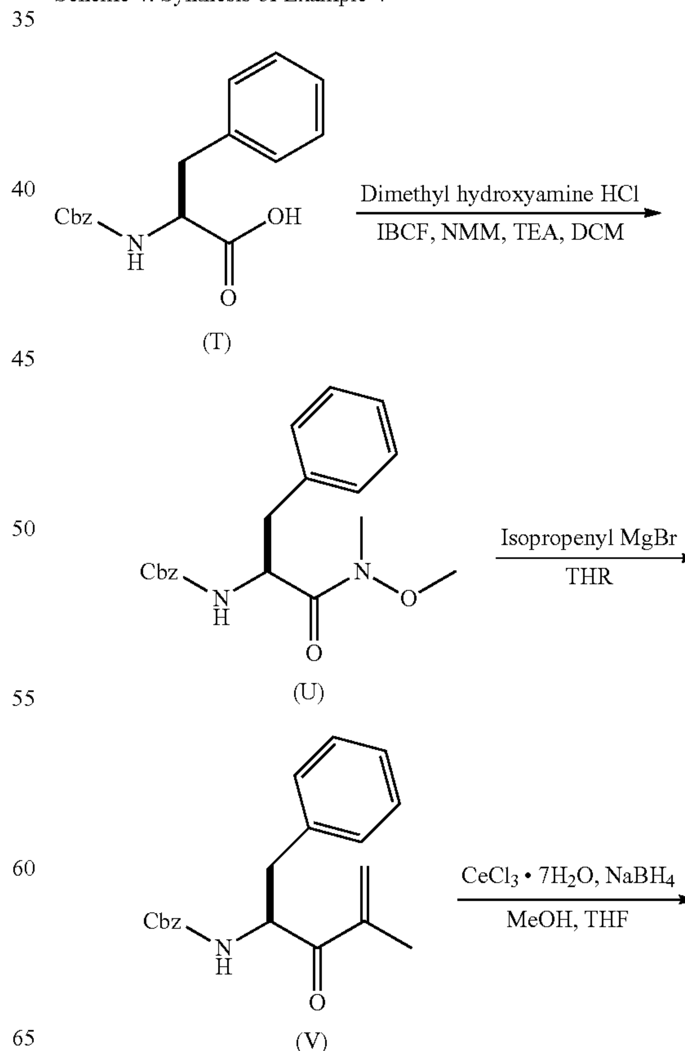
Scheme 4: Synthesis of Example 4
