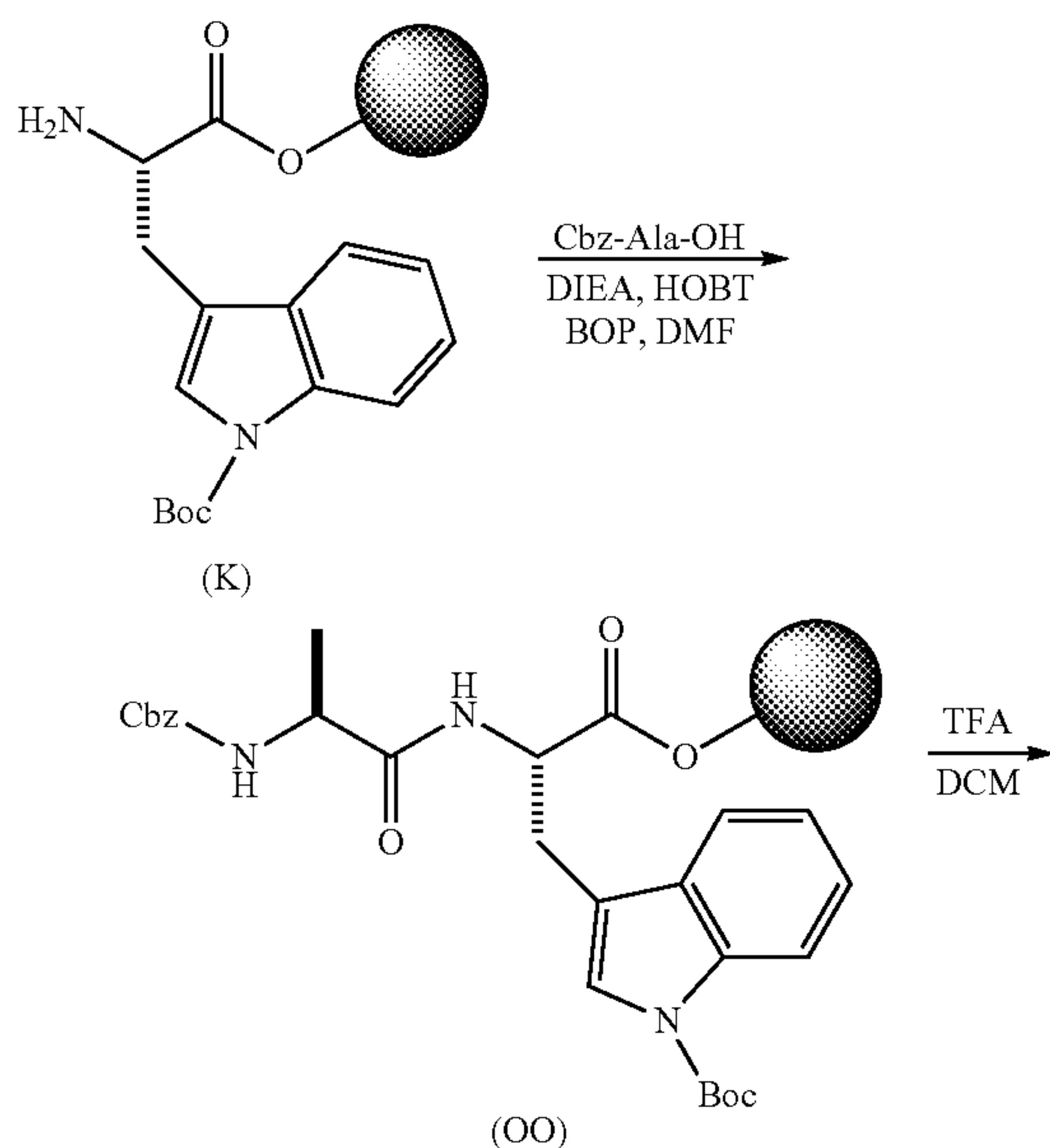
Scheme 9: Synthesis of Example 9
