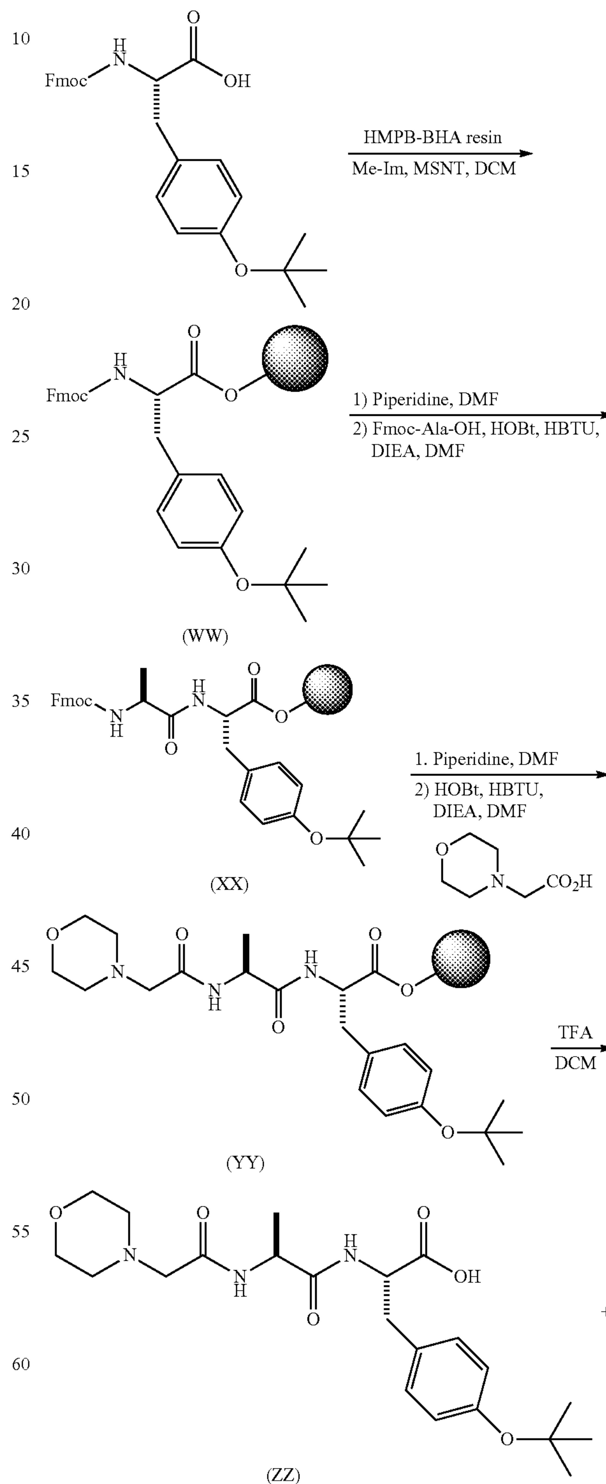
Scheme 13: Synthesis of Example 13
