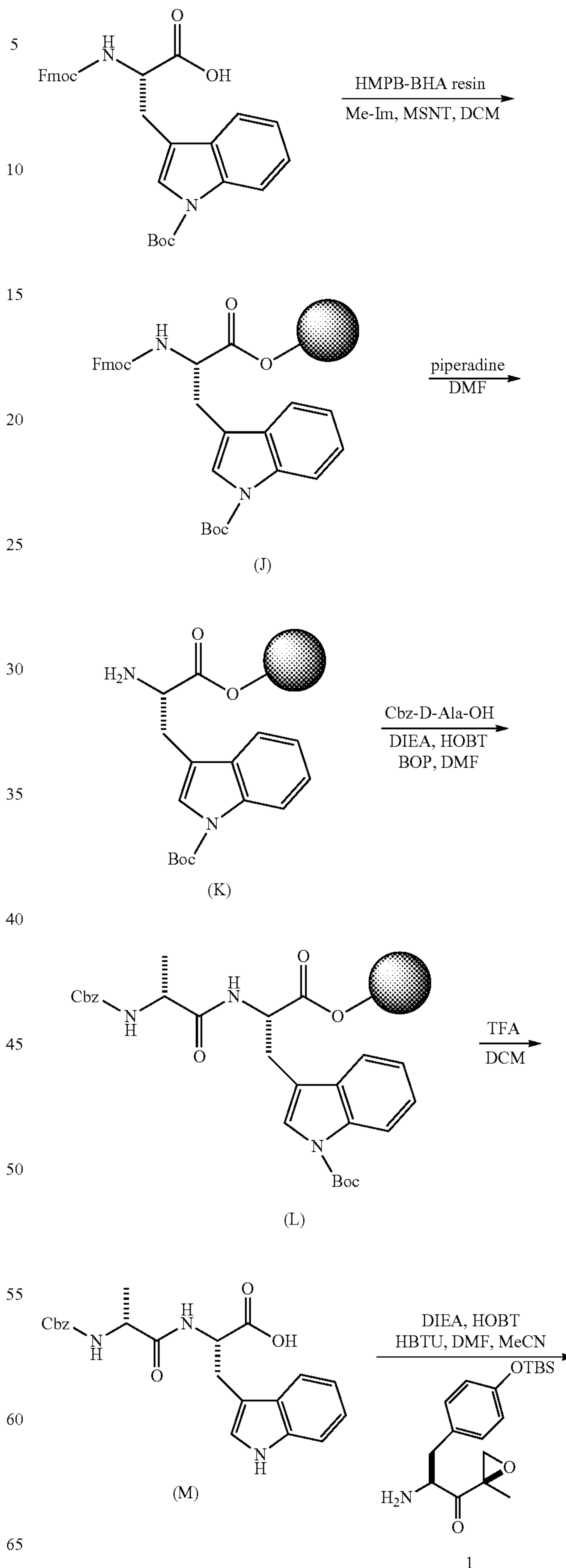
Scheme 2: Synthesis of Example 2
