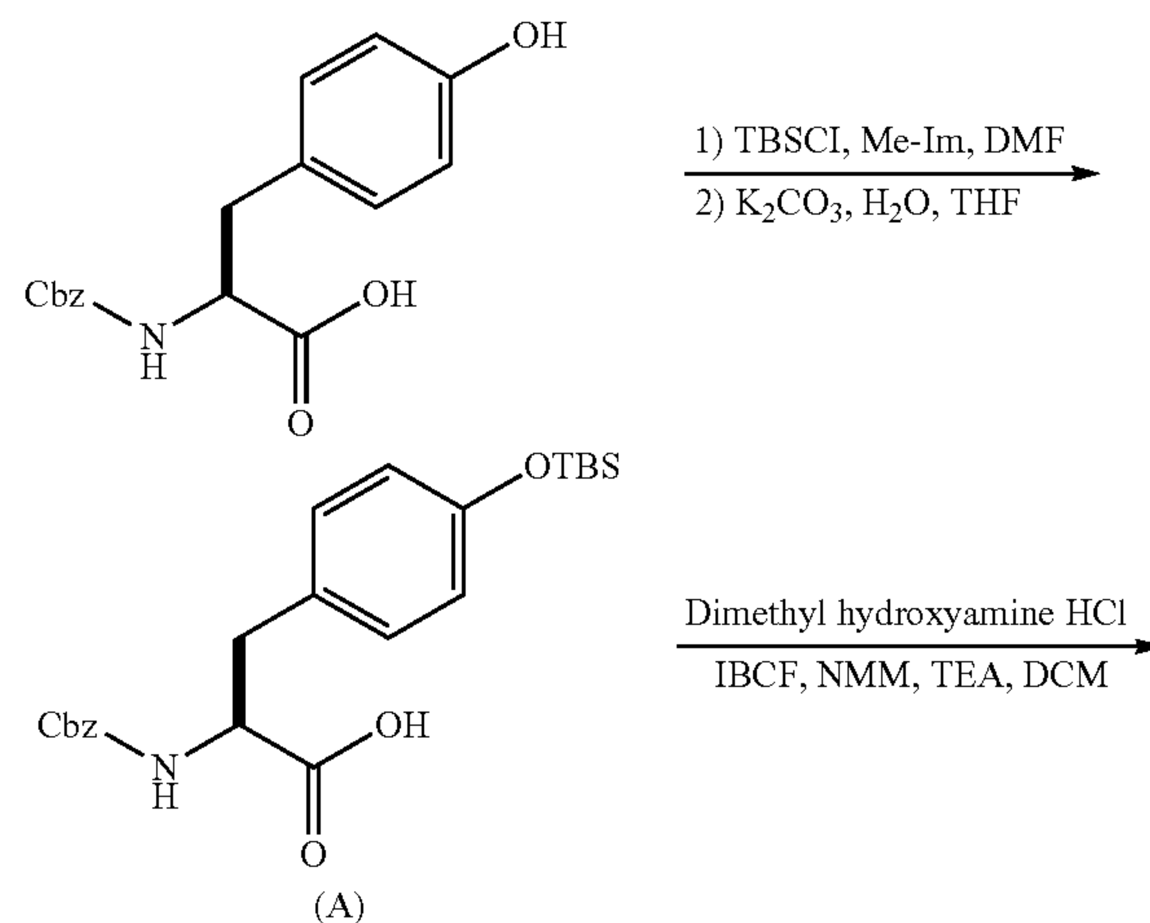
Scheme 1: Synthesis of Example 1
