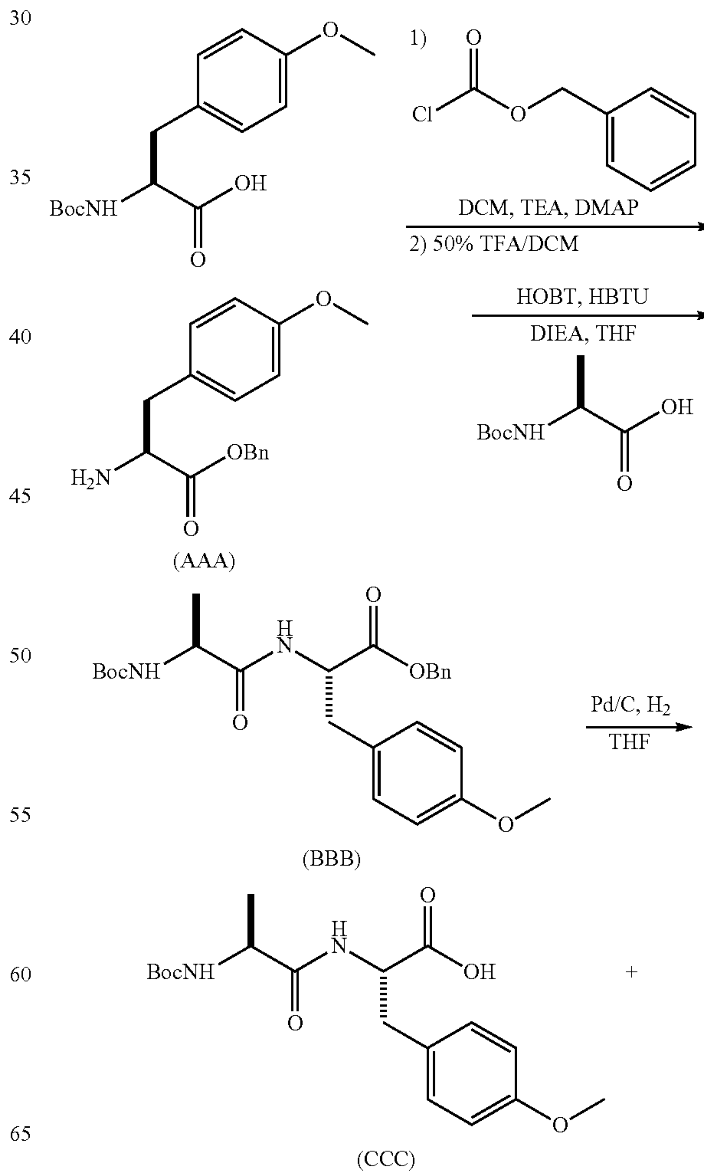
Scheme 14: Synthesis of Example 14
