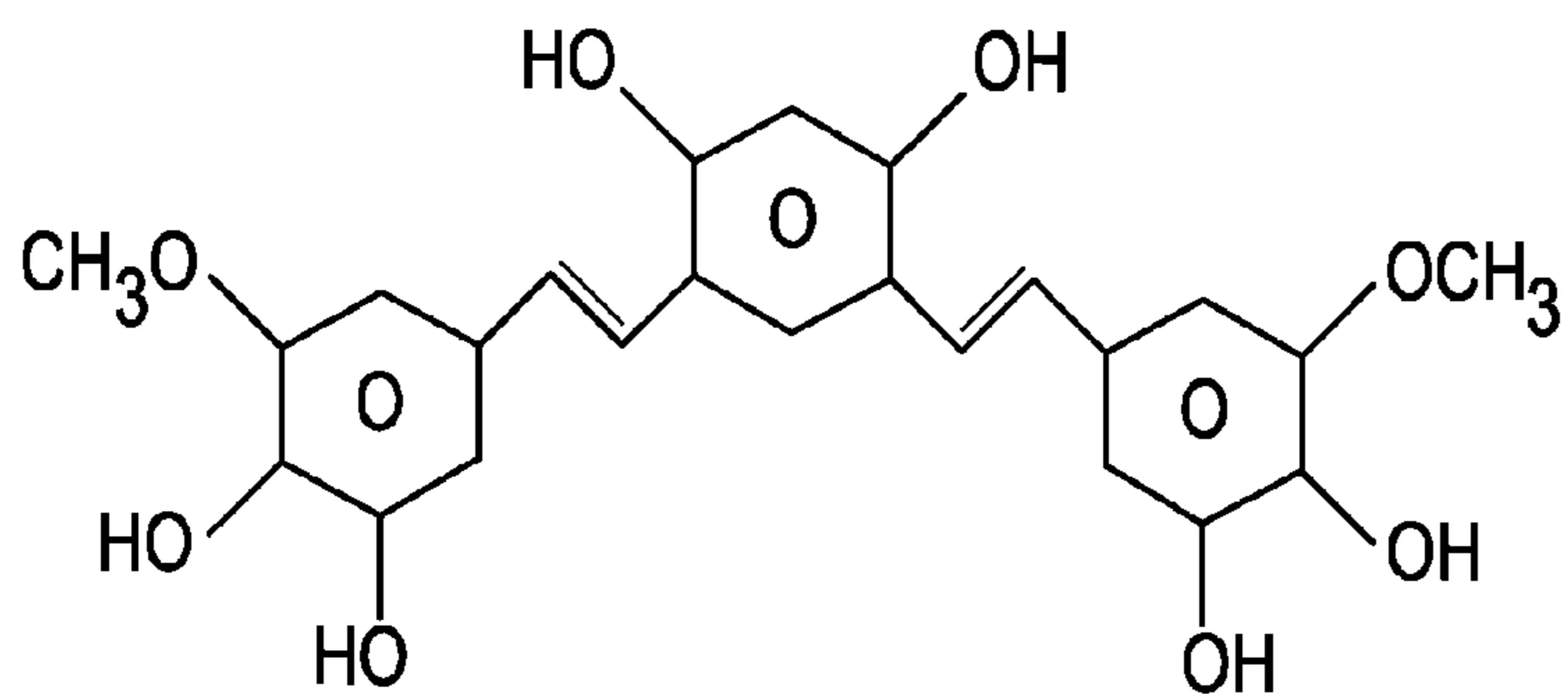
Curcumin-resveratrol III
