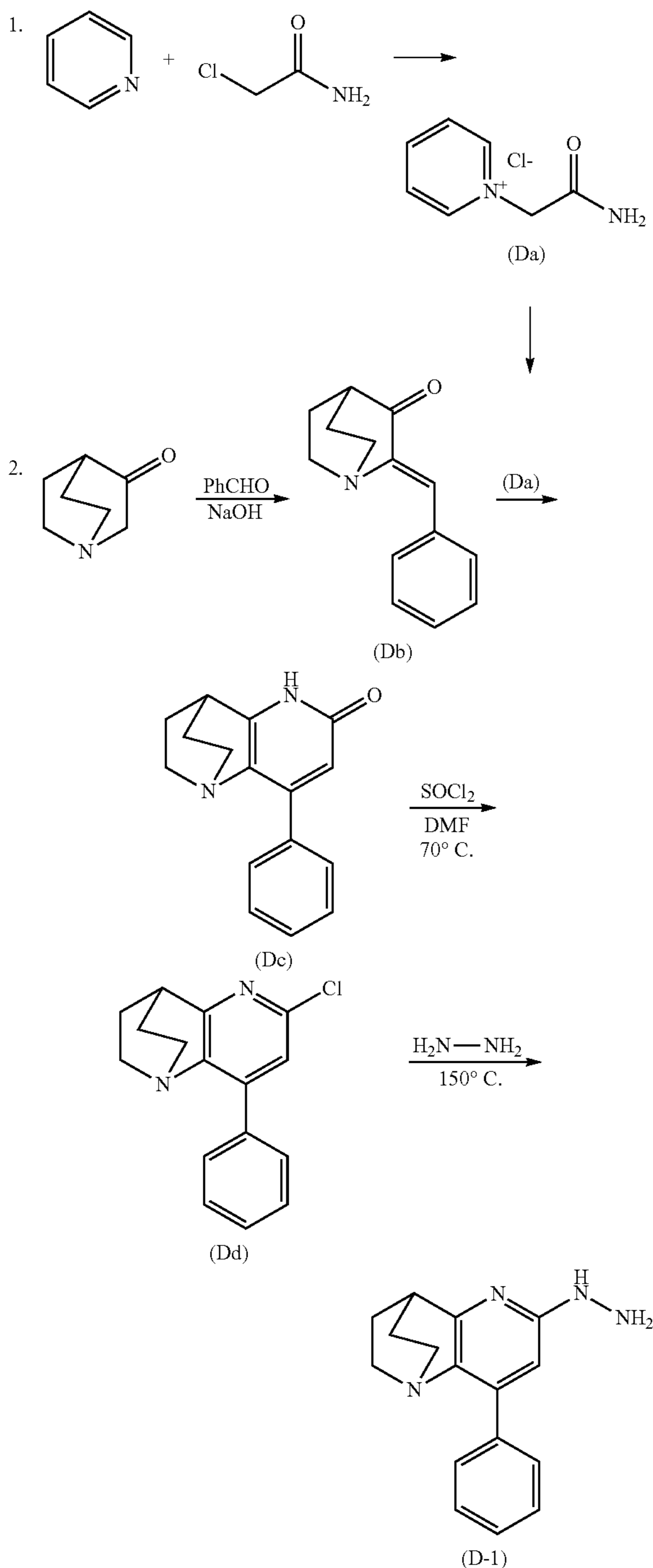
REACTION SCHEME 2
