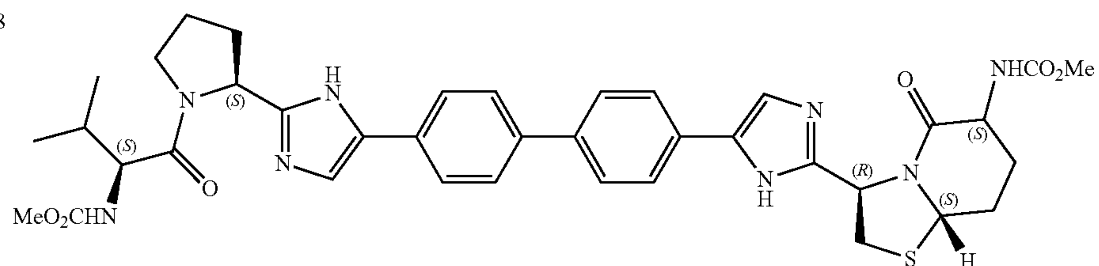
Compounds 368-376
