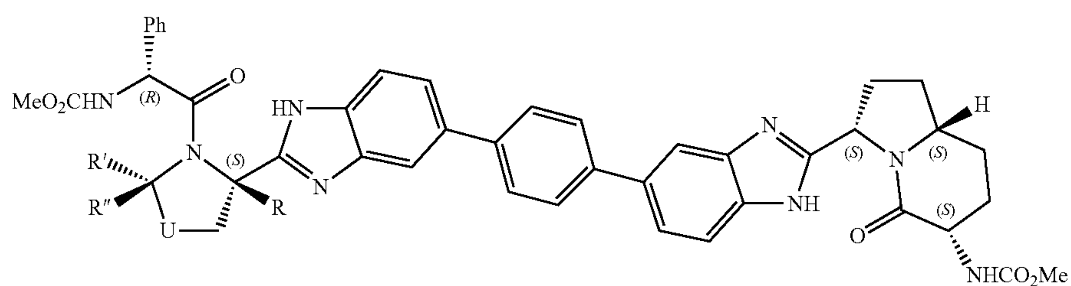
Compounds 248-251
