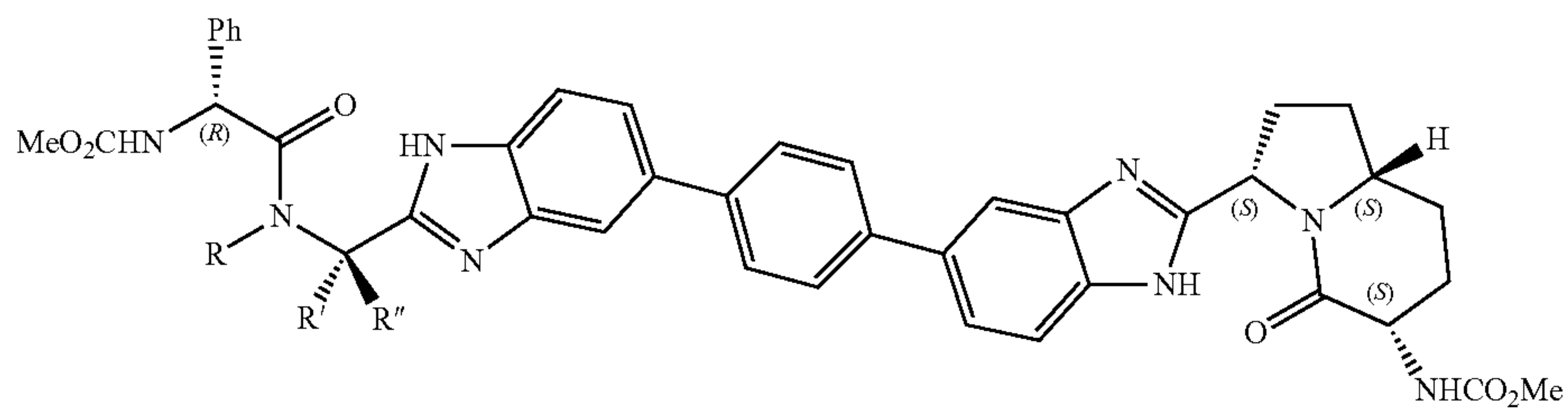
Compounds 252-261.
