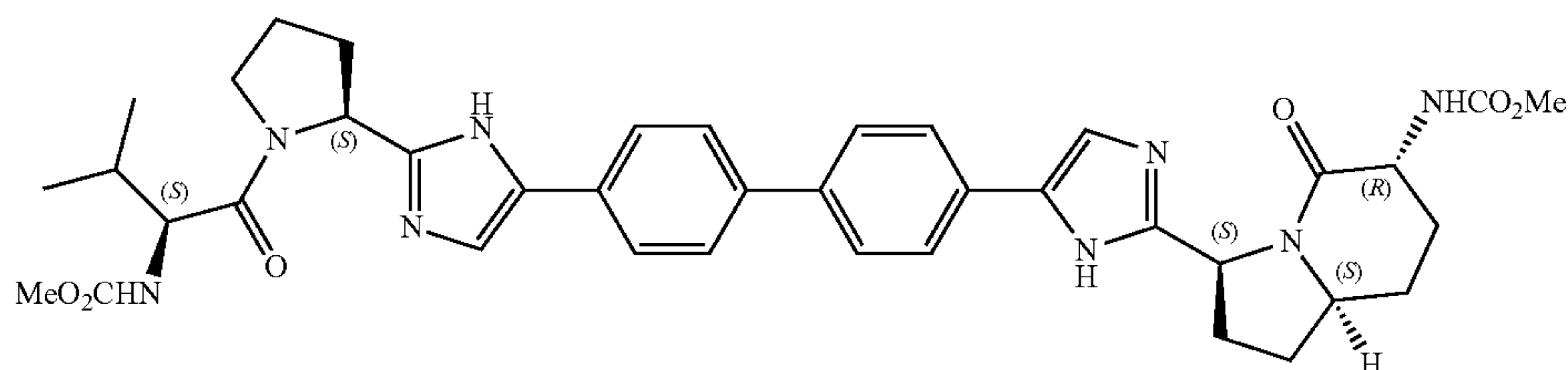
Example 370
