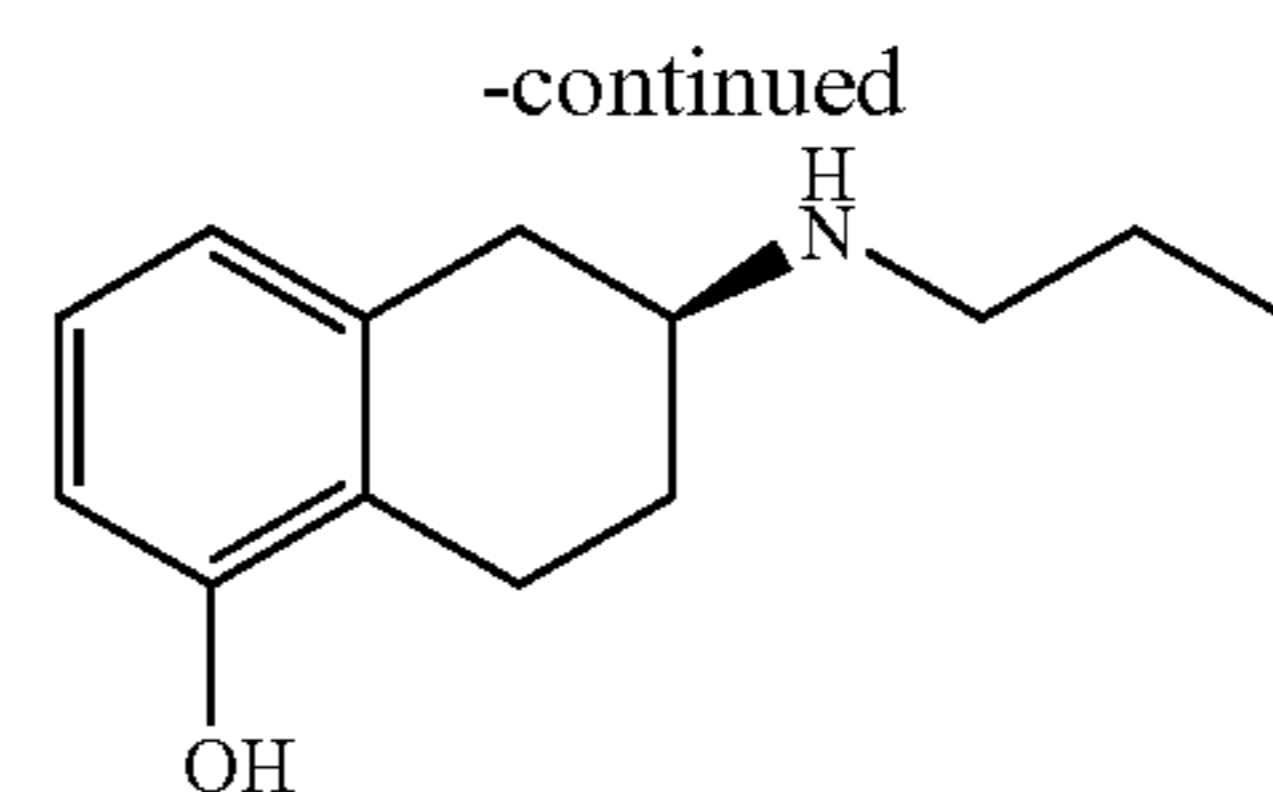
(S)-2-N-propylamino-5-hydroxytetralin
