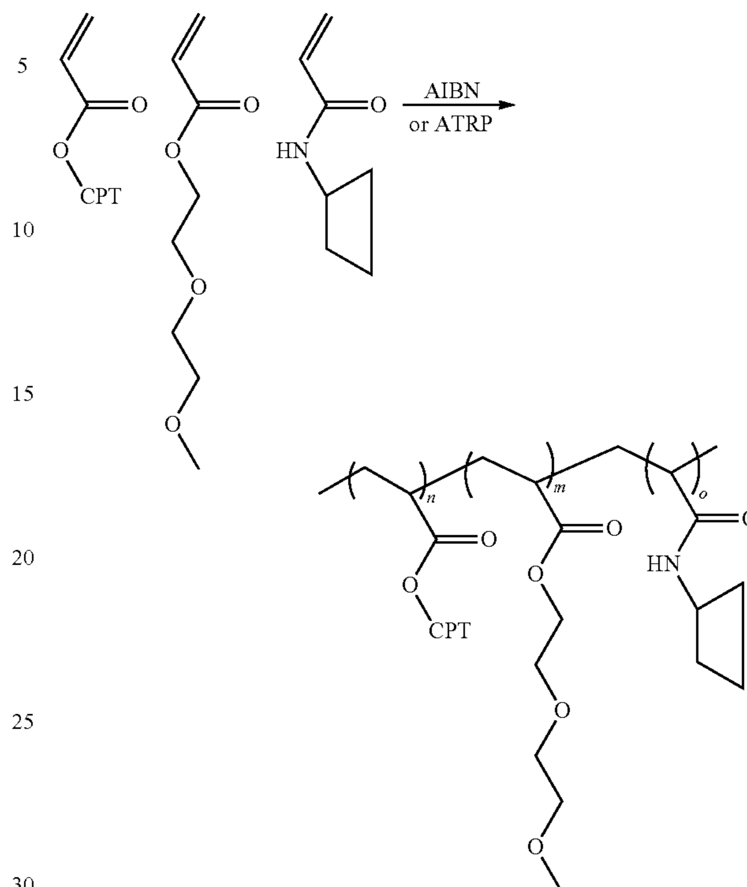
Scheme X
