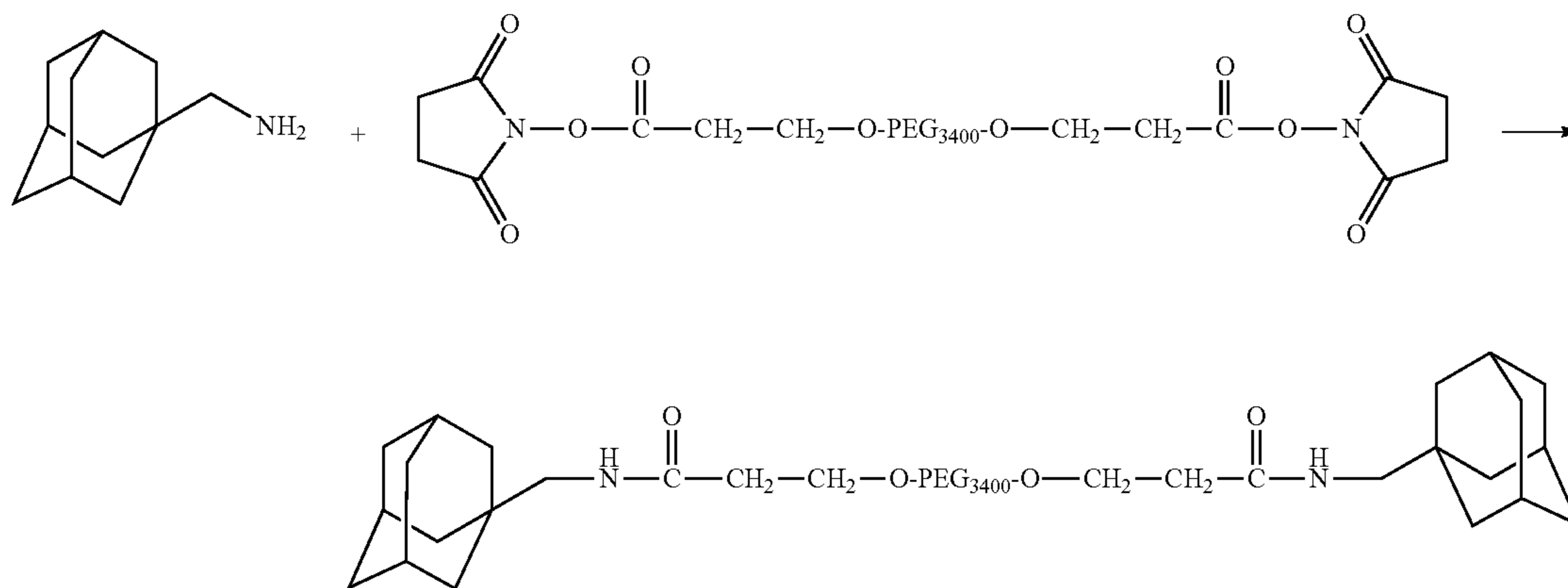
Scheme XXXXVI
