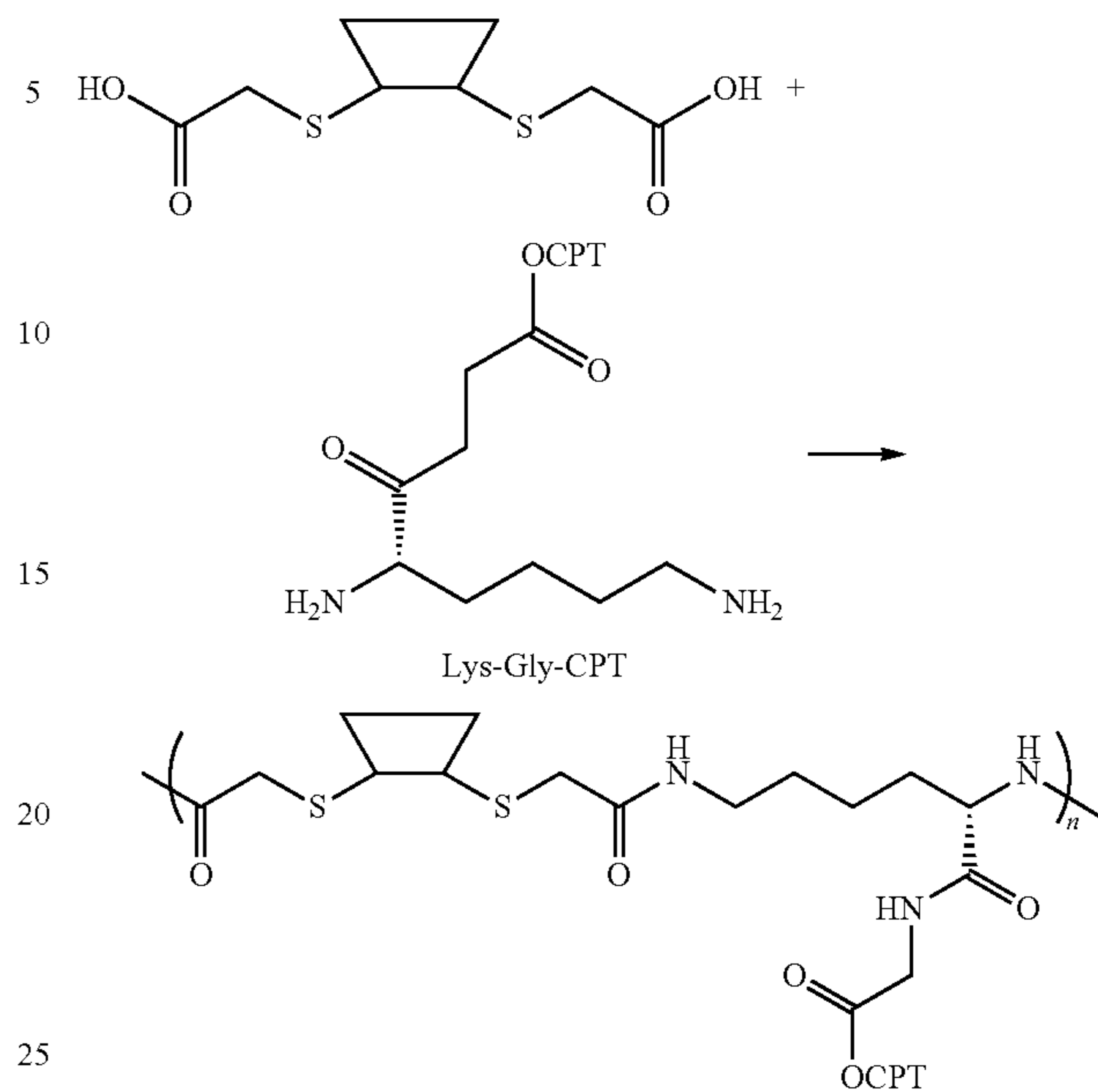
Scheme VIII
