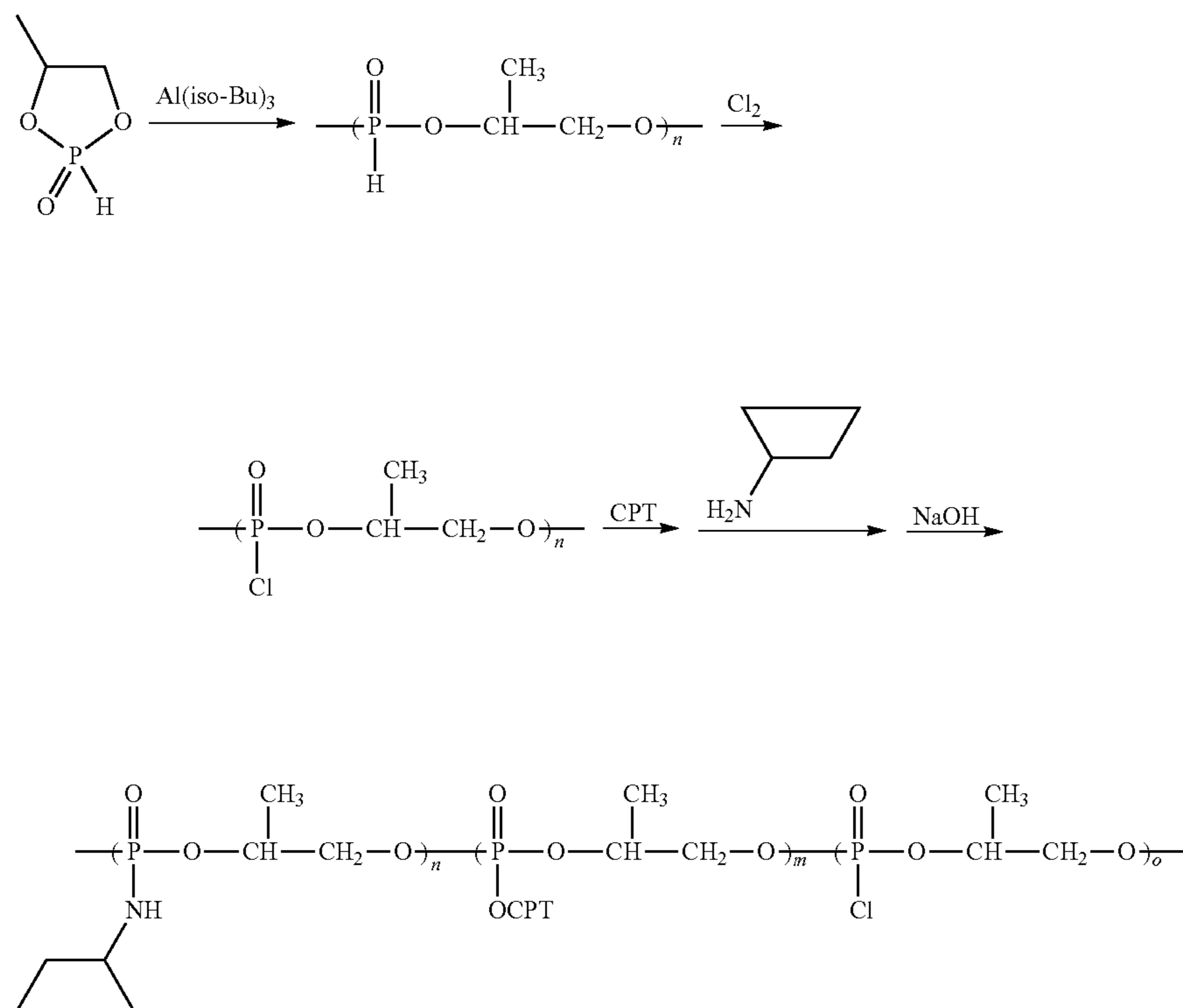
Scheme IX
