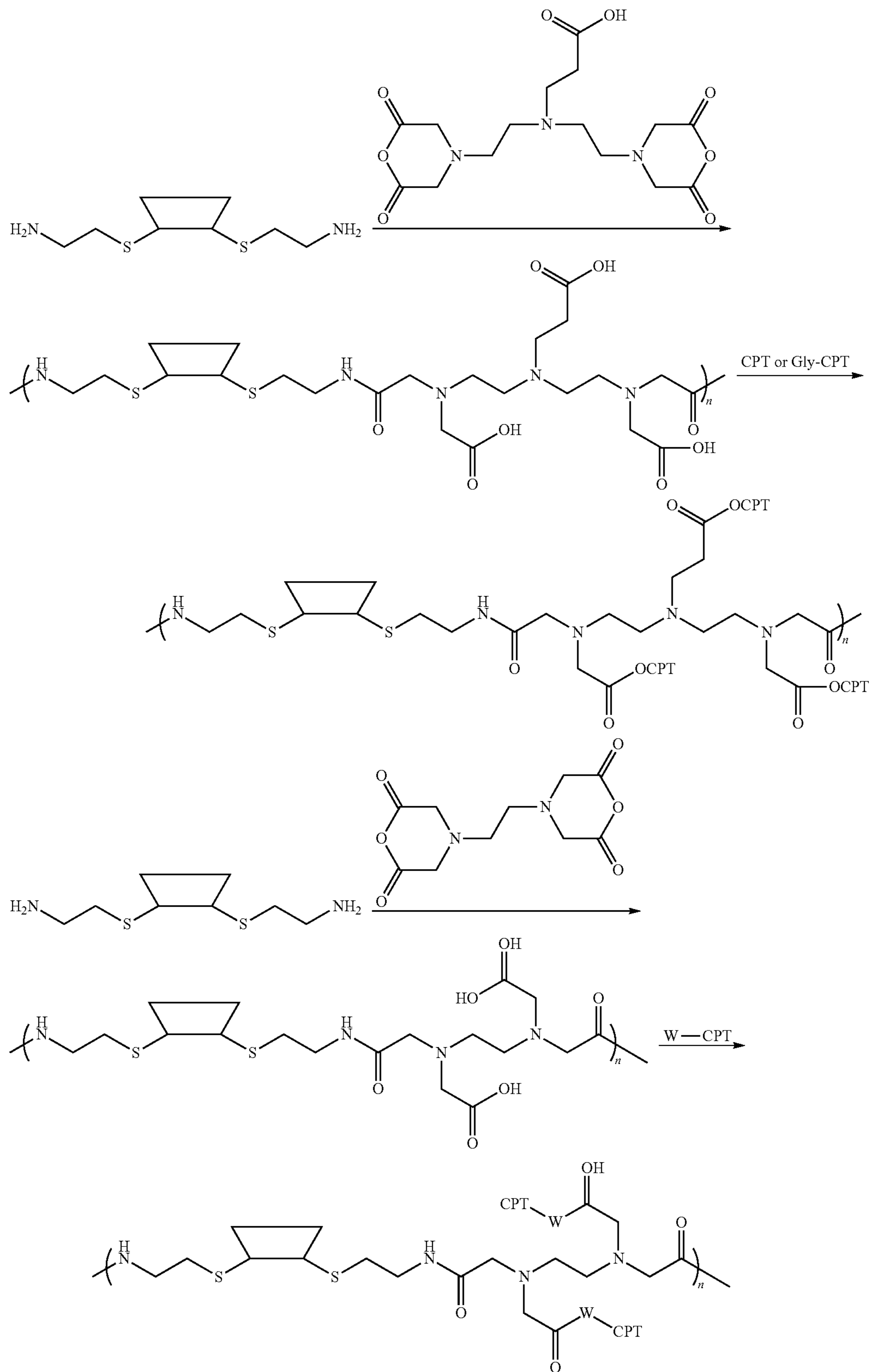
Scheme V
