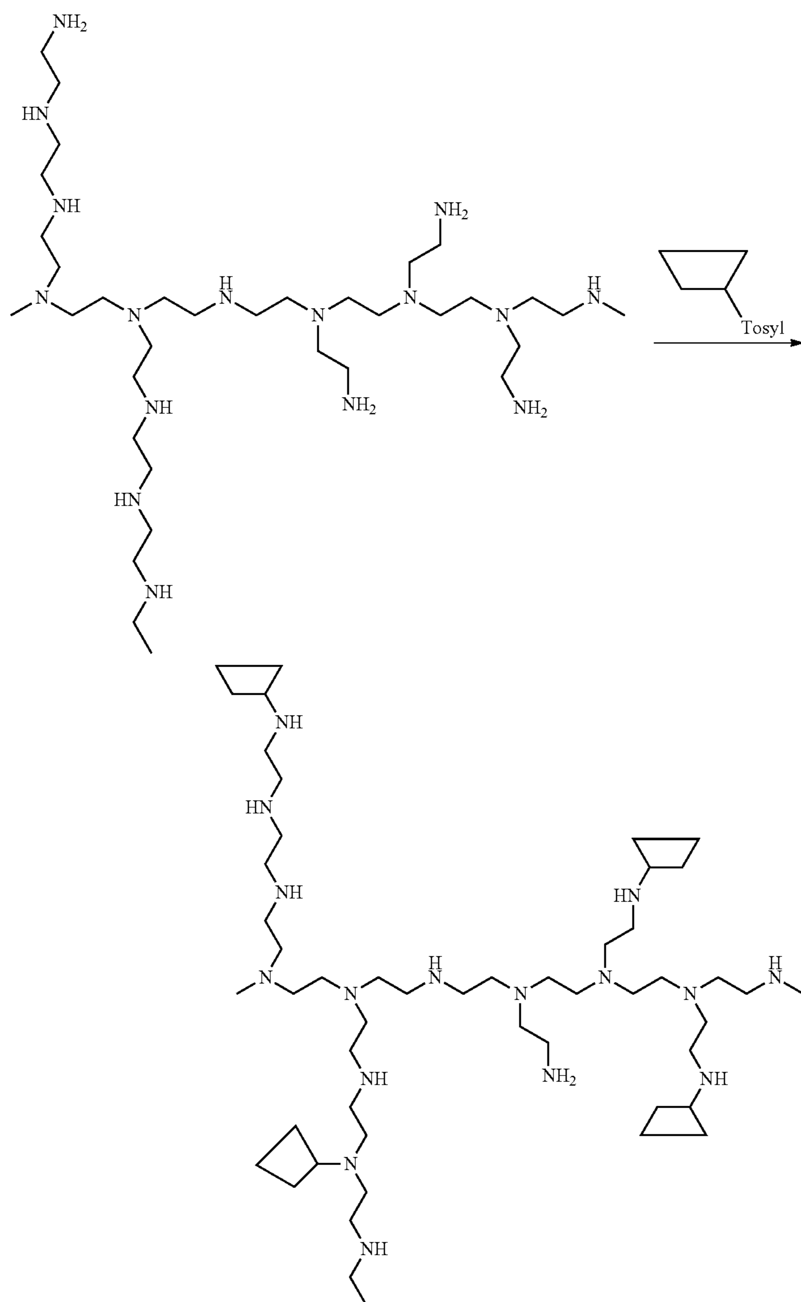
Scheme XXXXIV
