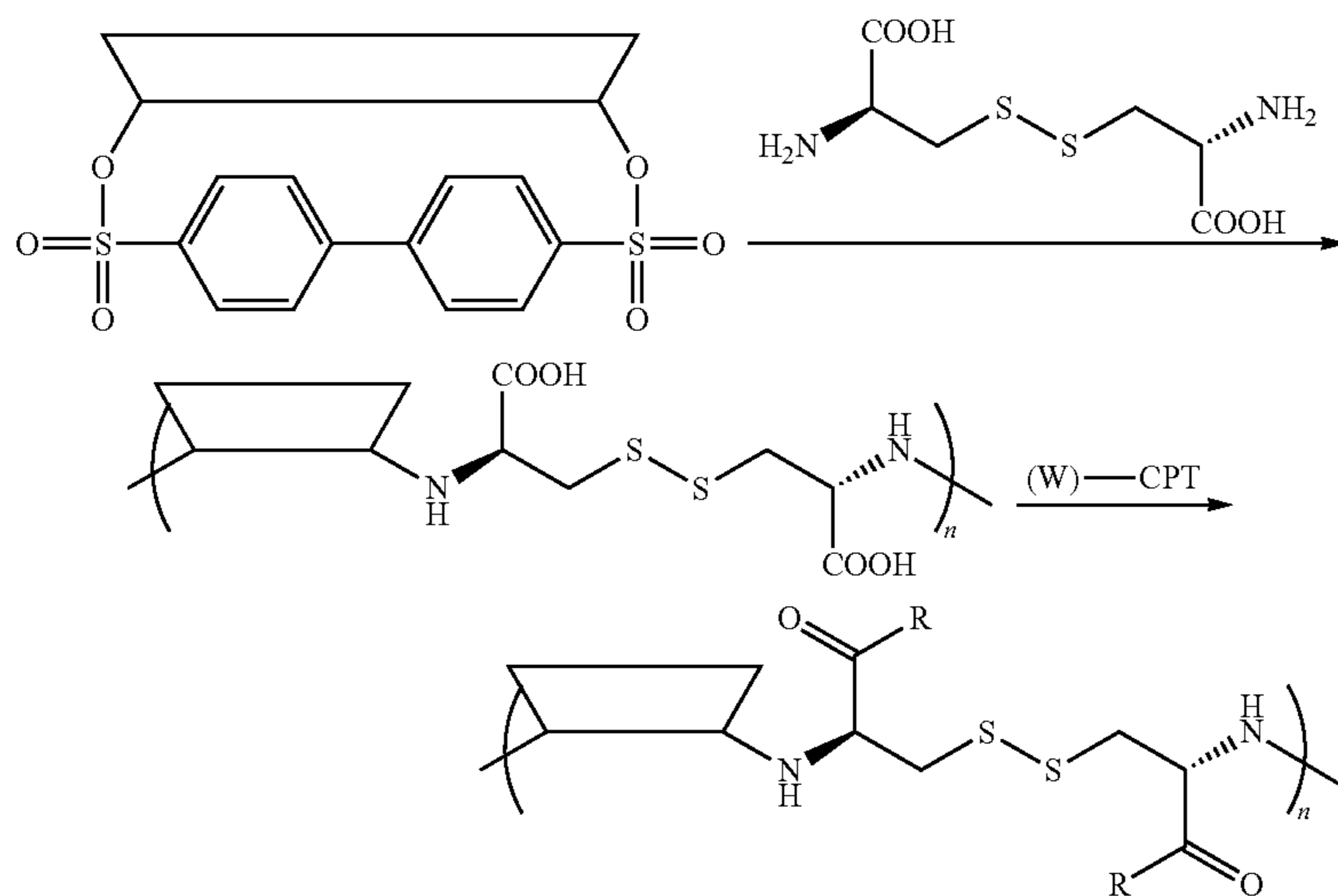
Scheme III
