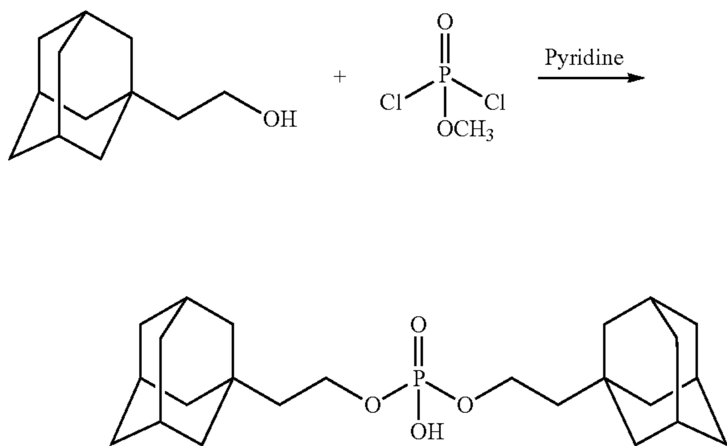
Scheme XXXXVII
