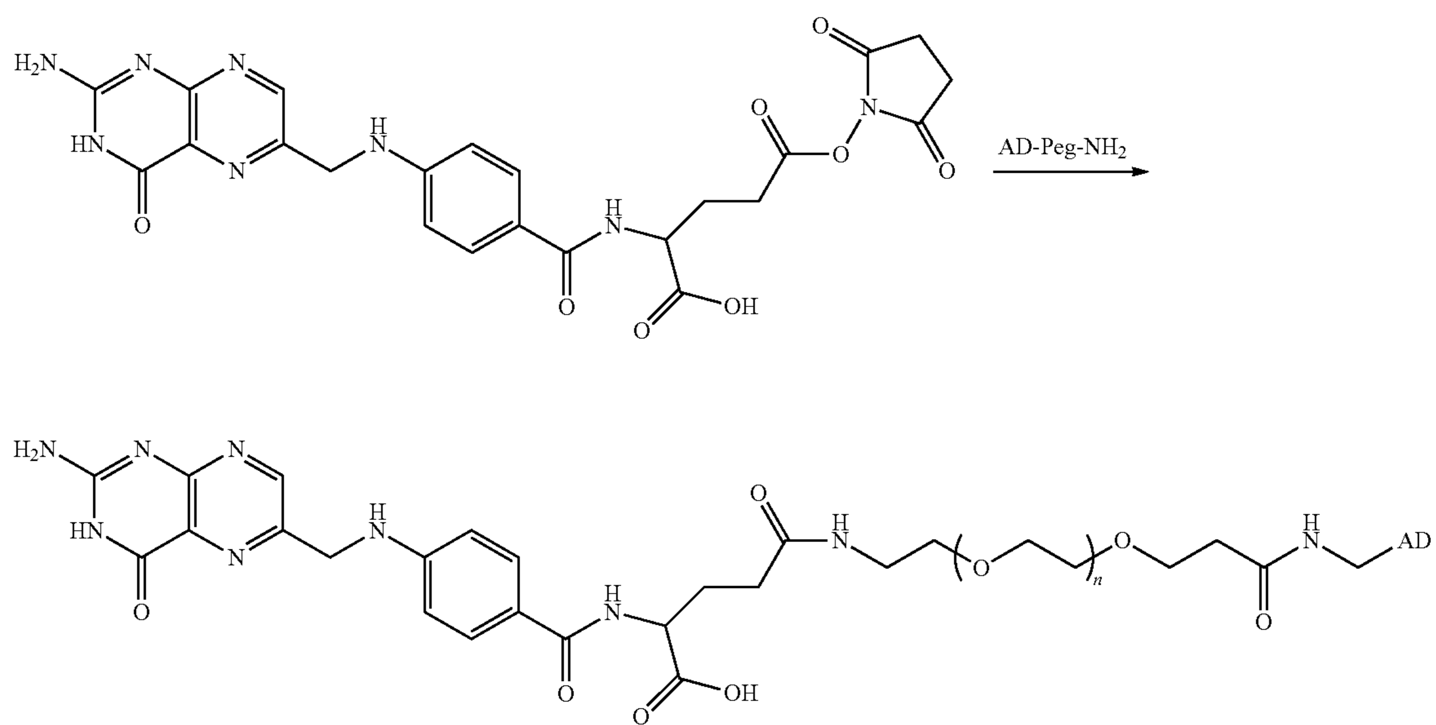
Scheme L
