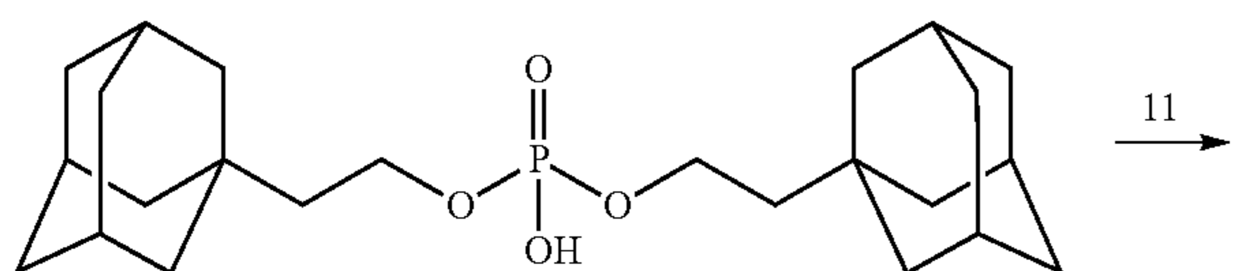
Scheme XXXXVIII
