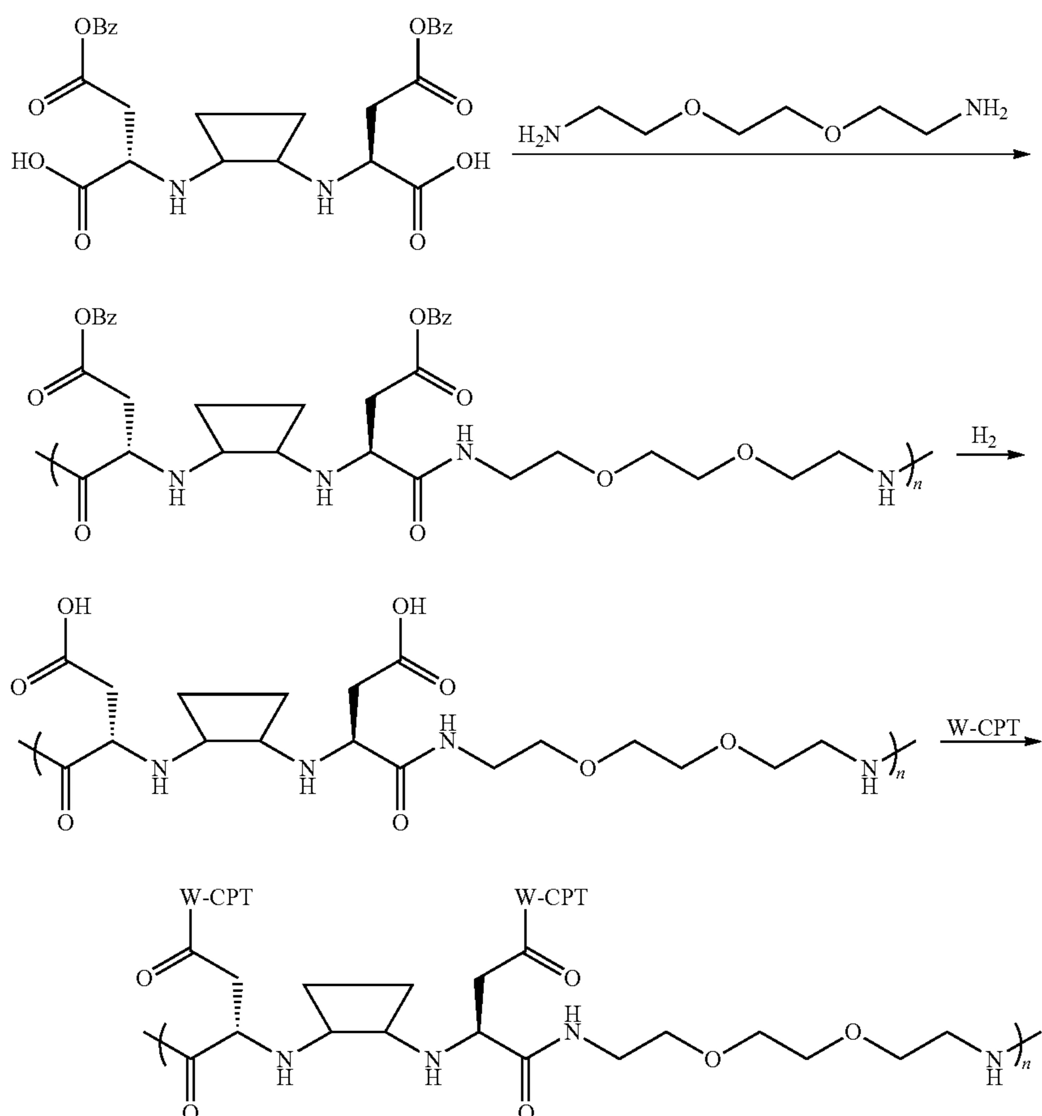
Scheme IV
