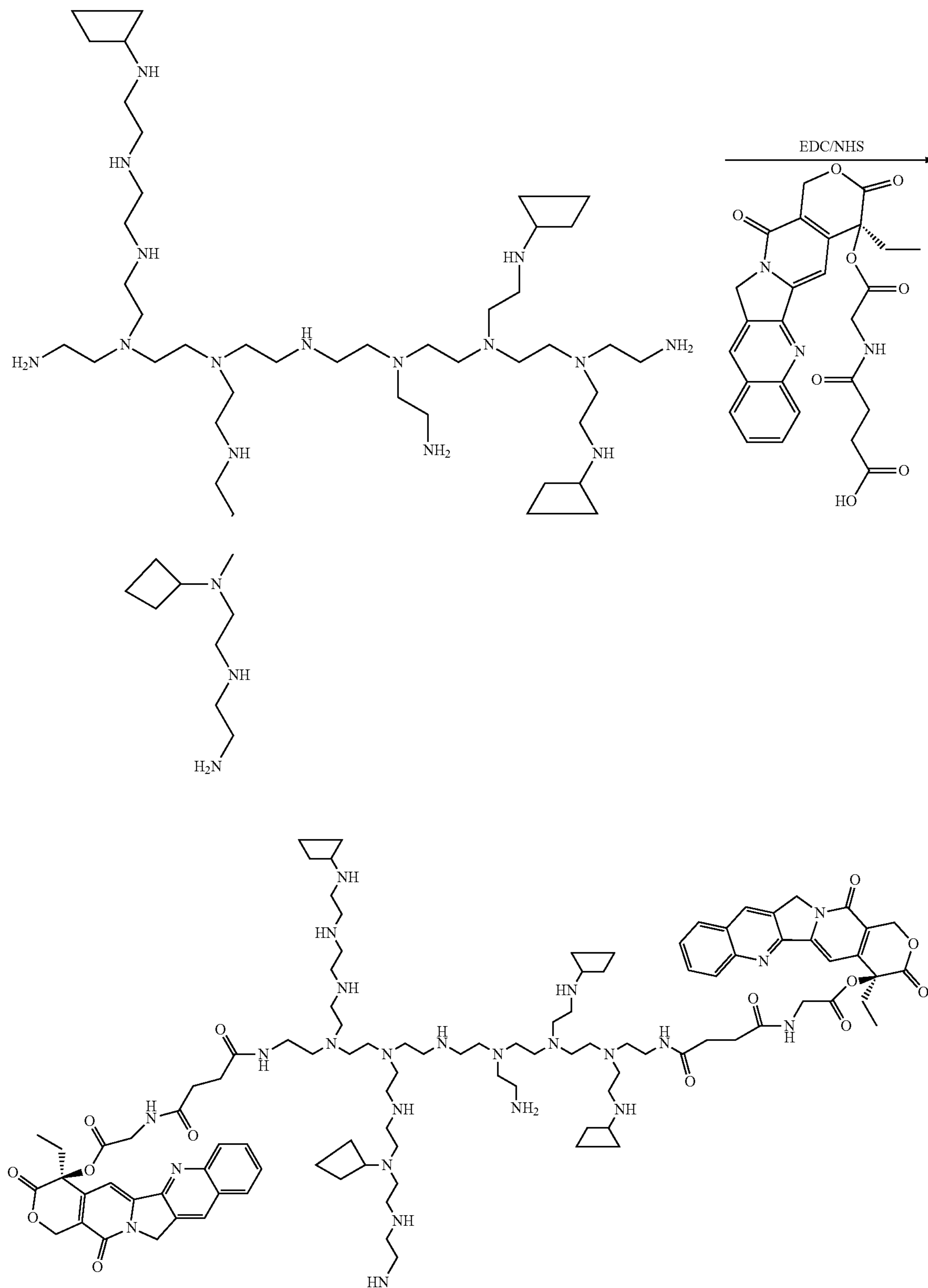
Scheme XXXV
