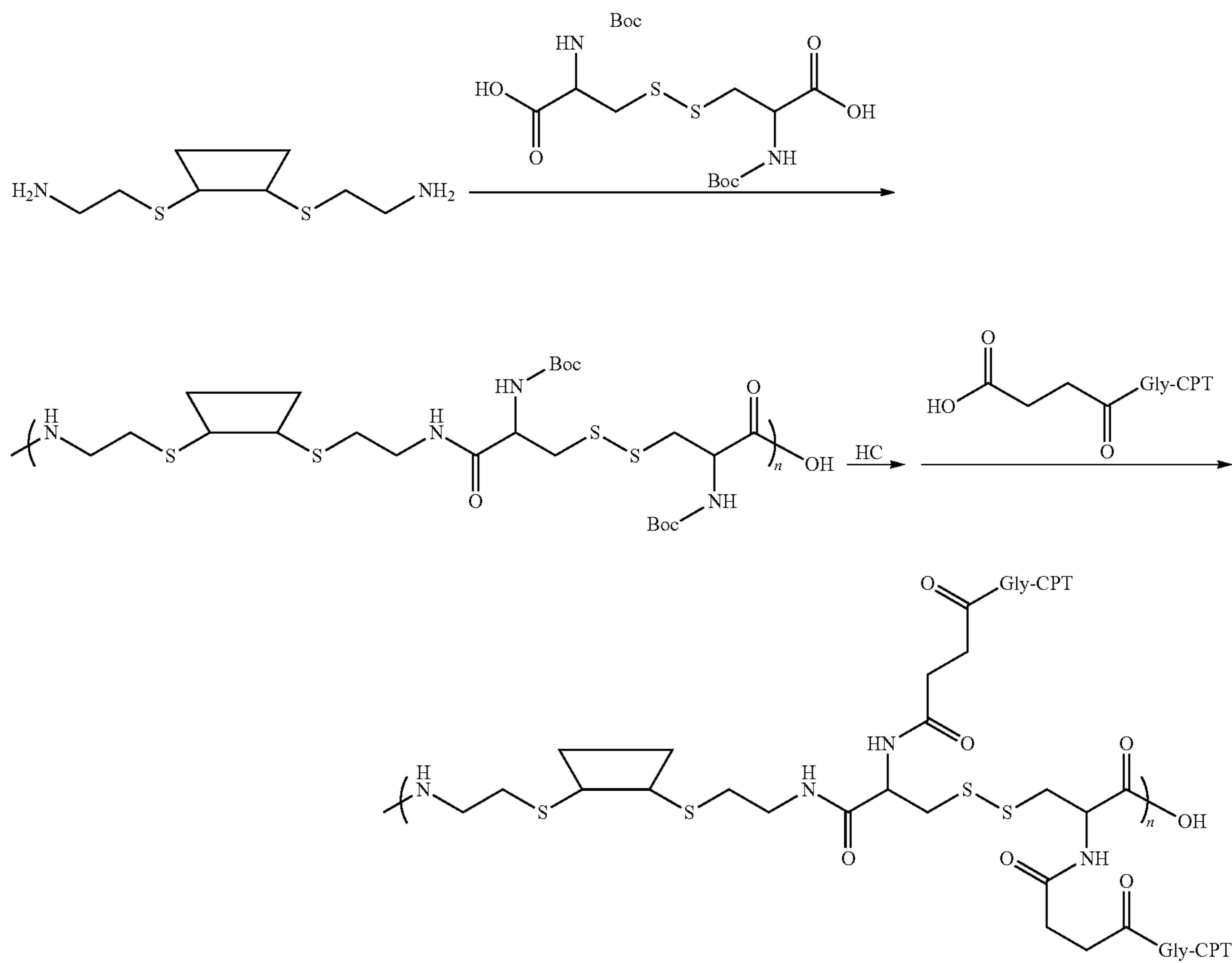
Scheme VII
