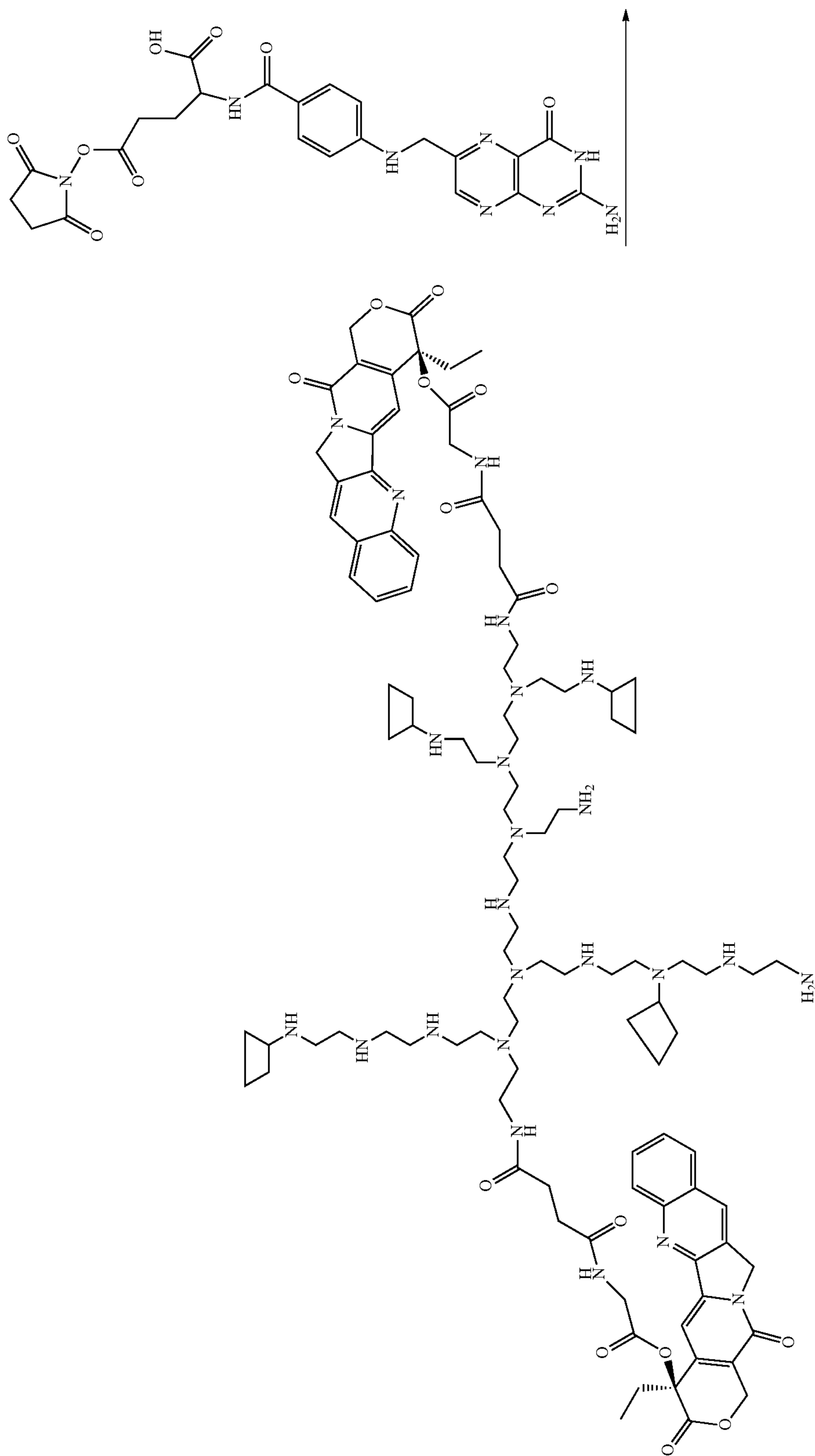
Scheme L1
