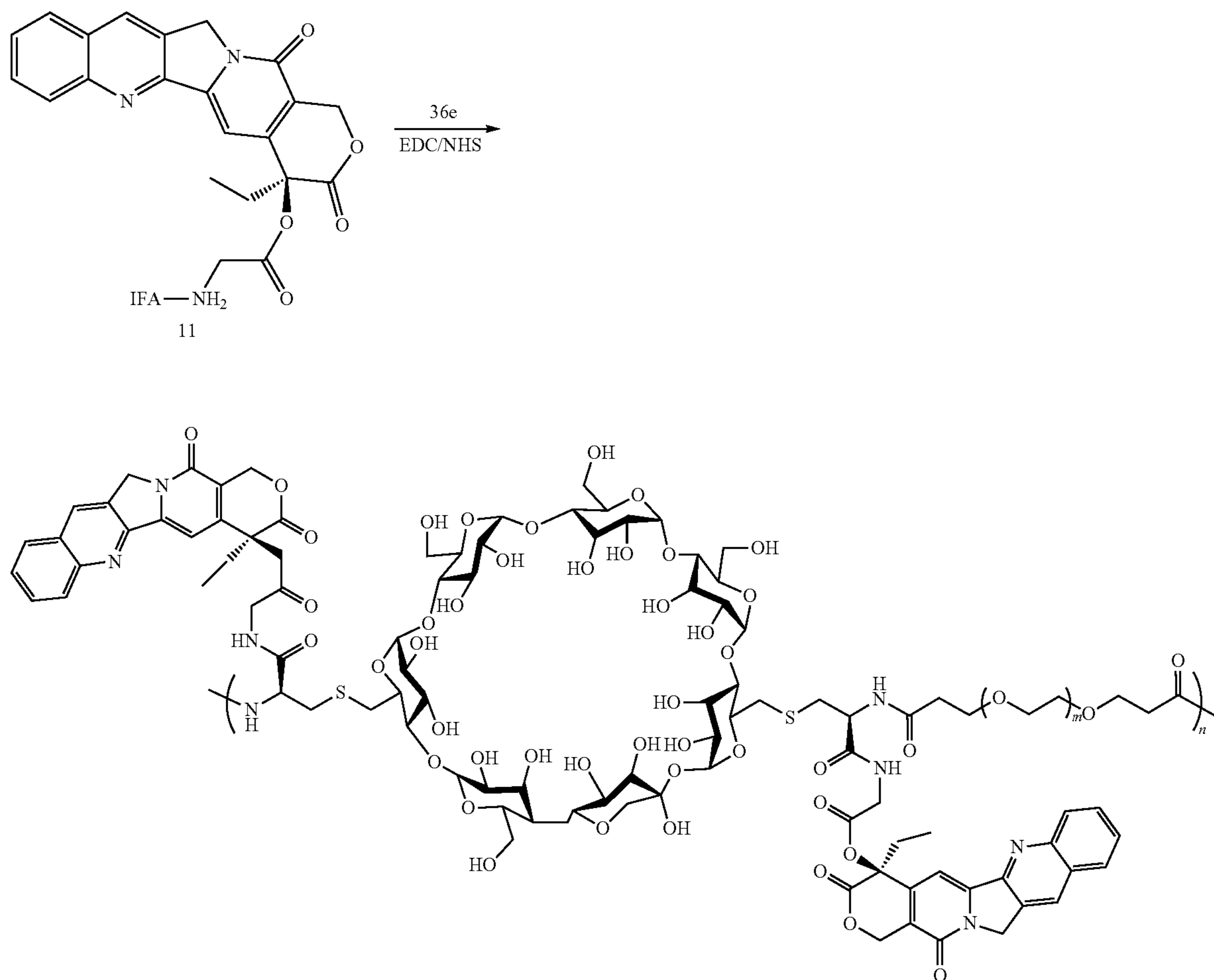
Scheme XXXIX
