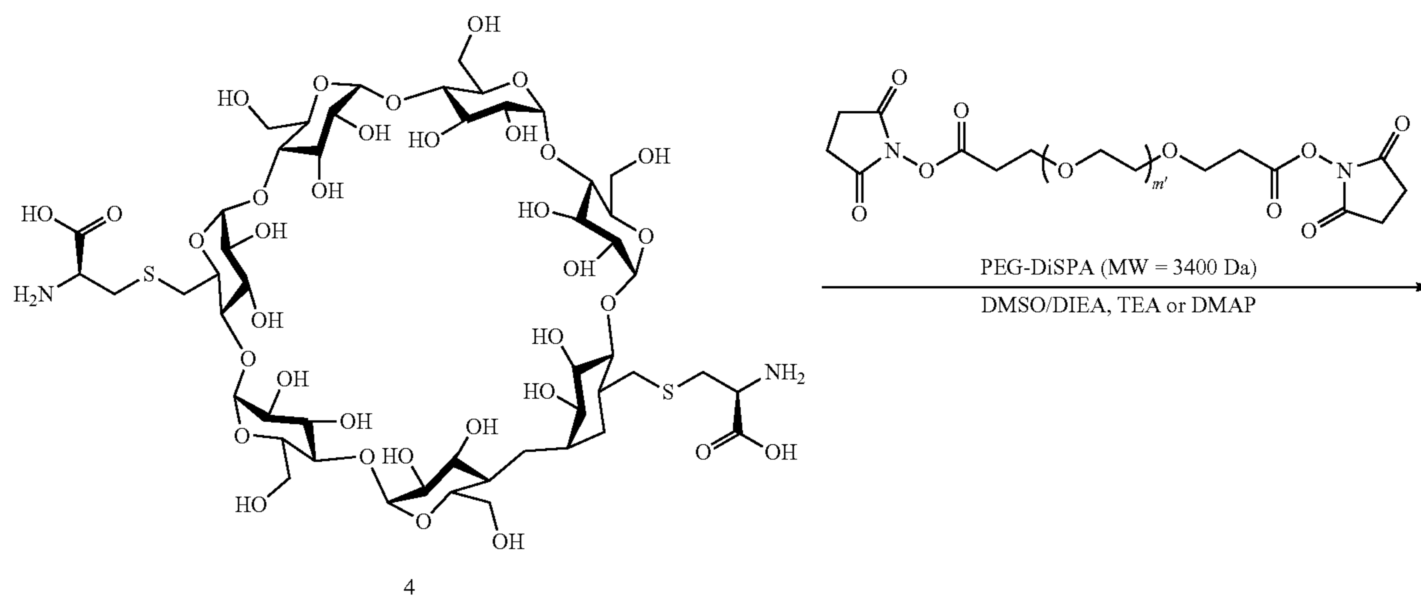
Scheme XXXVIIIa
