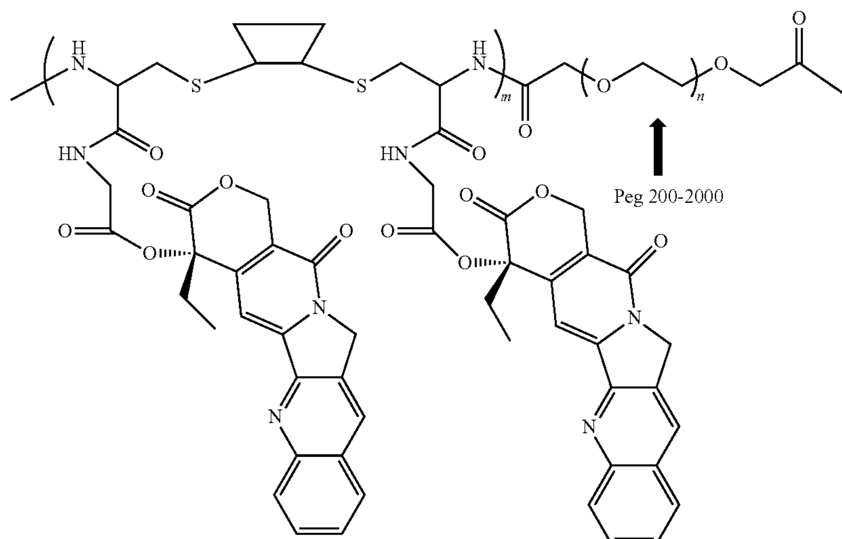
Scheme XXXXII
