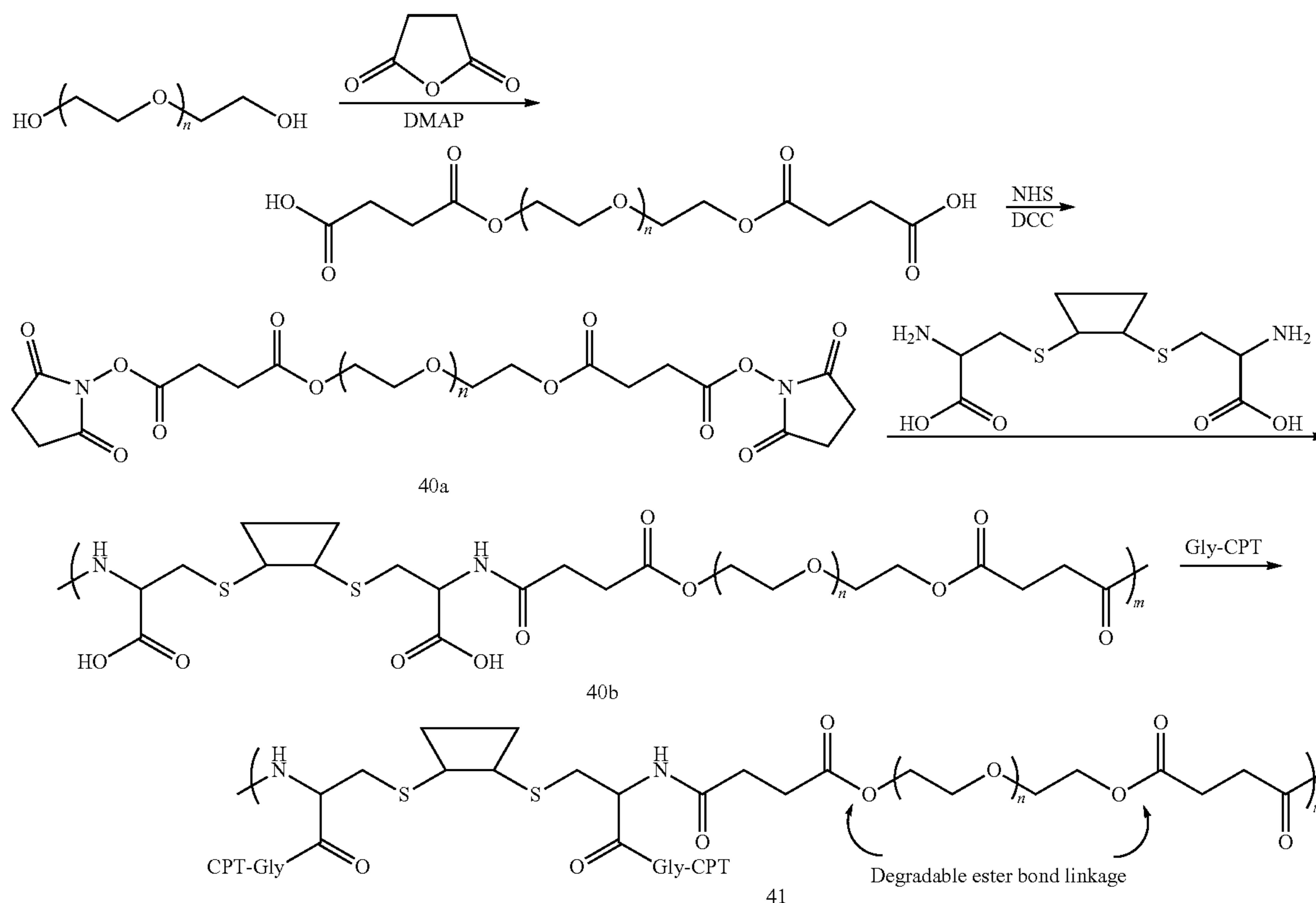
Scheme XXXXI
