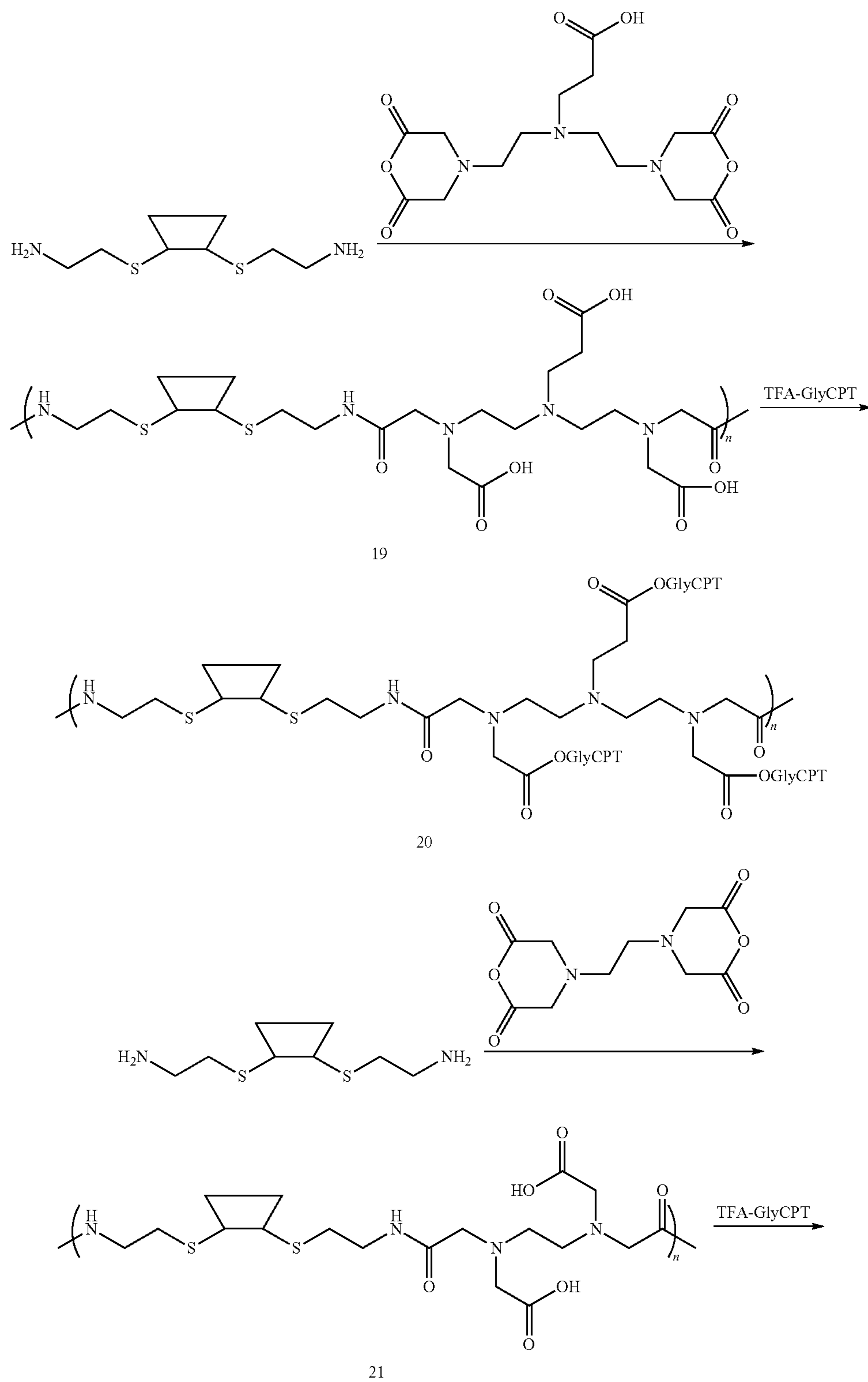
Scheme XXIX
