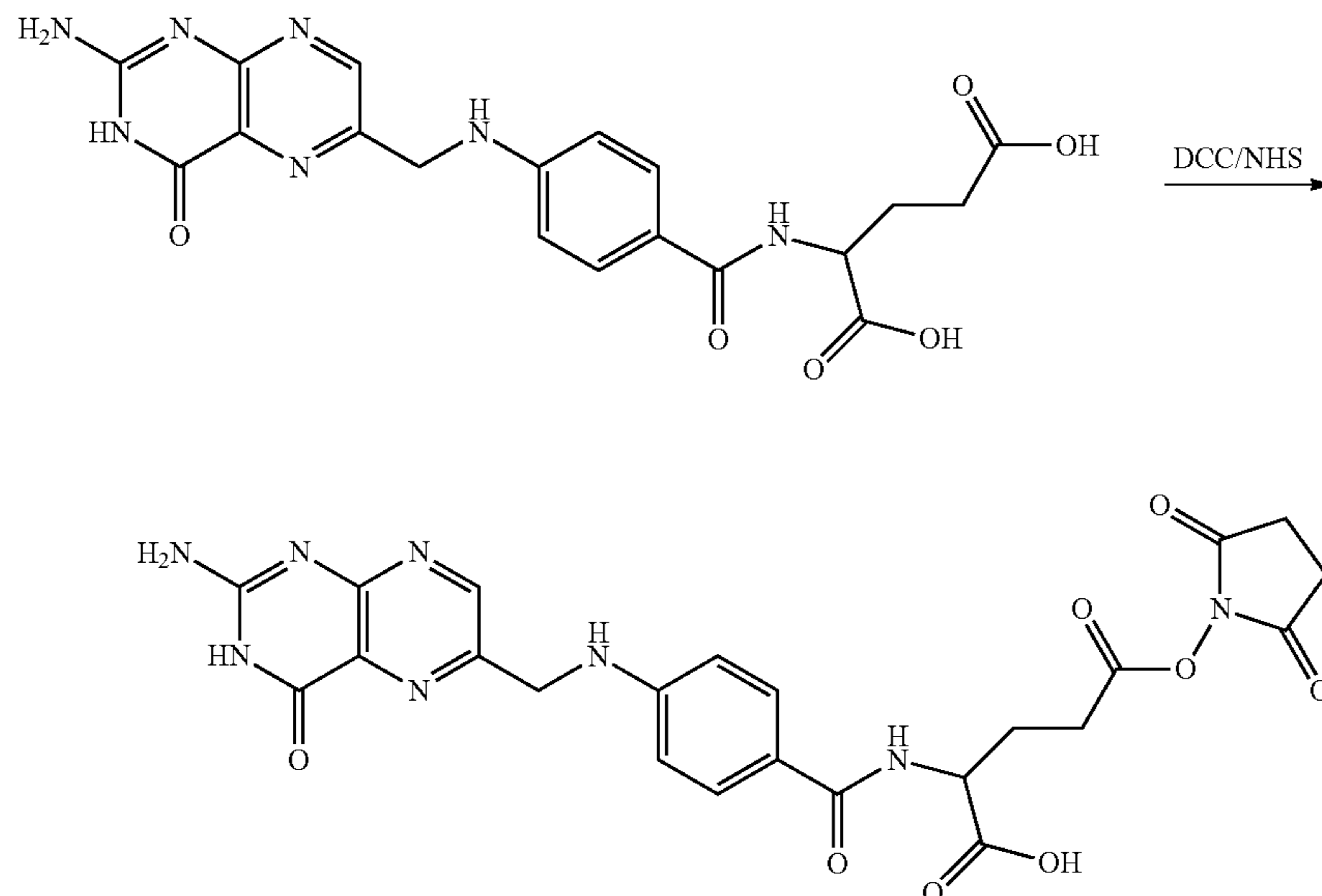
Scheme XXXXIX
