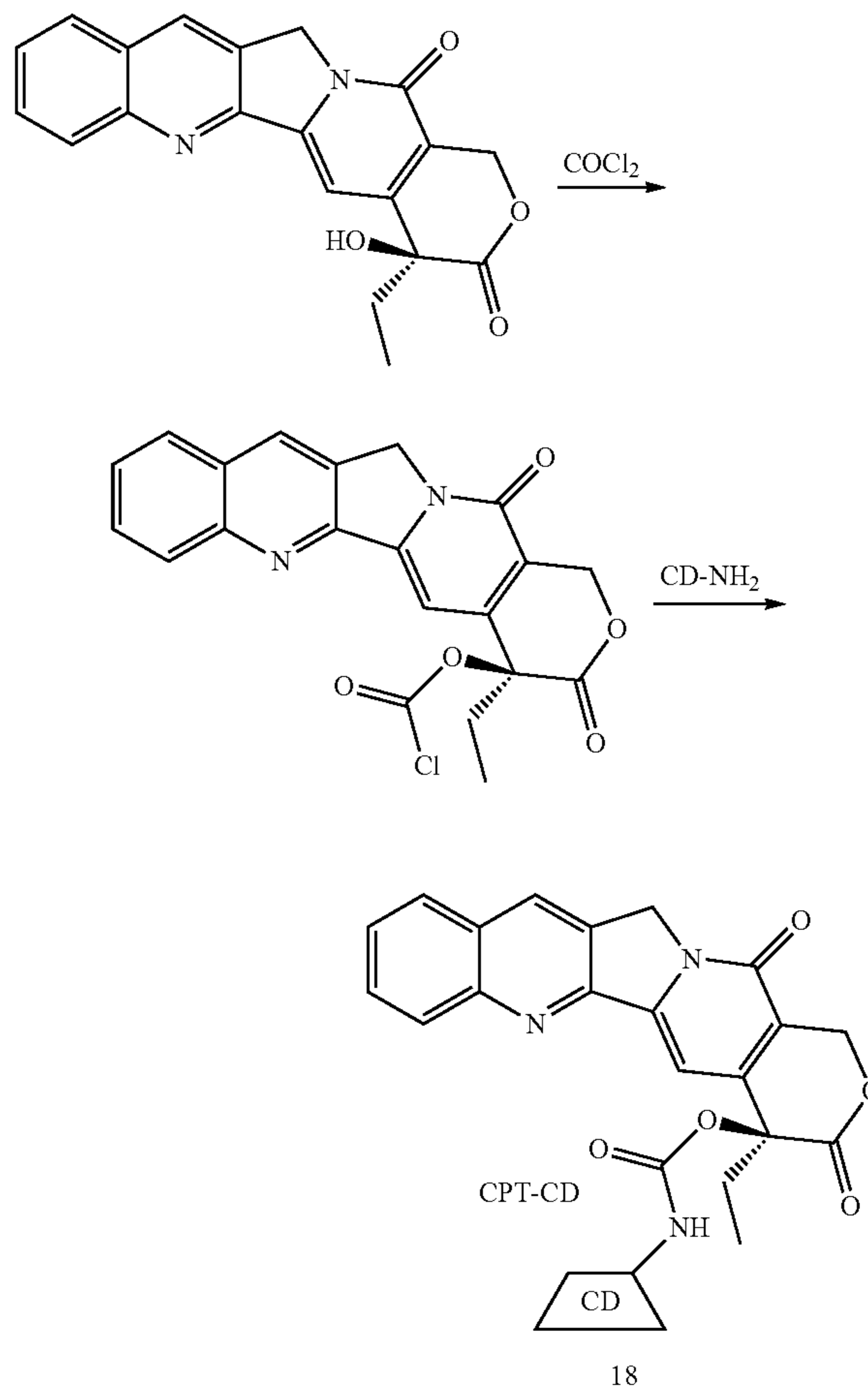
Scheme XXVIII
