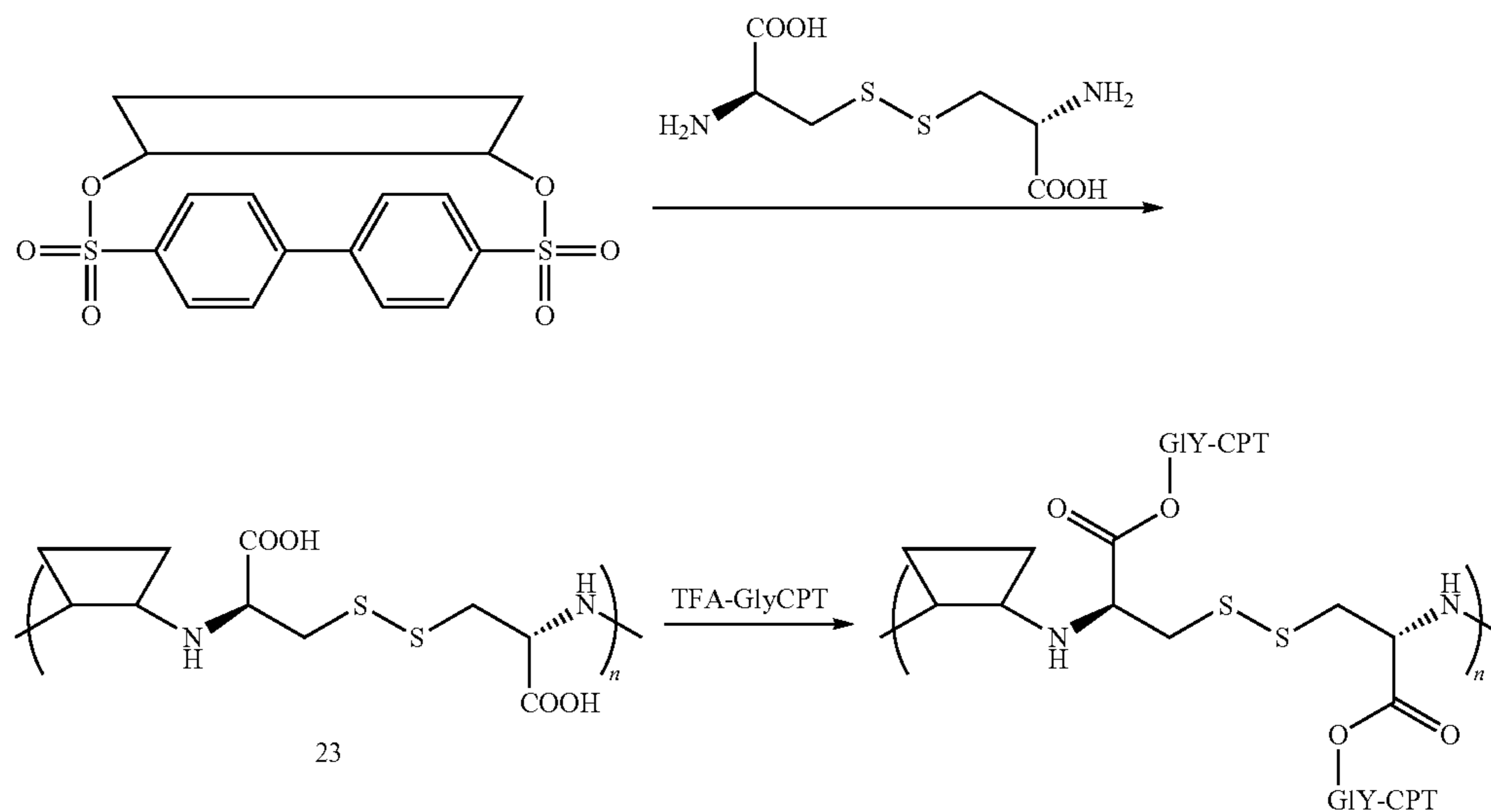
Scheme XXX
