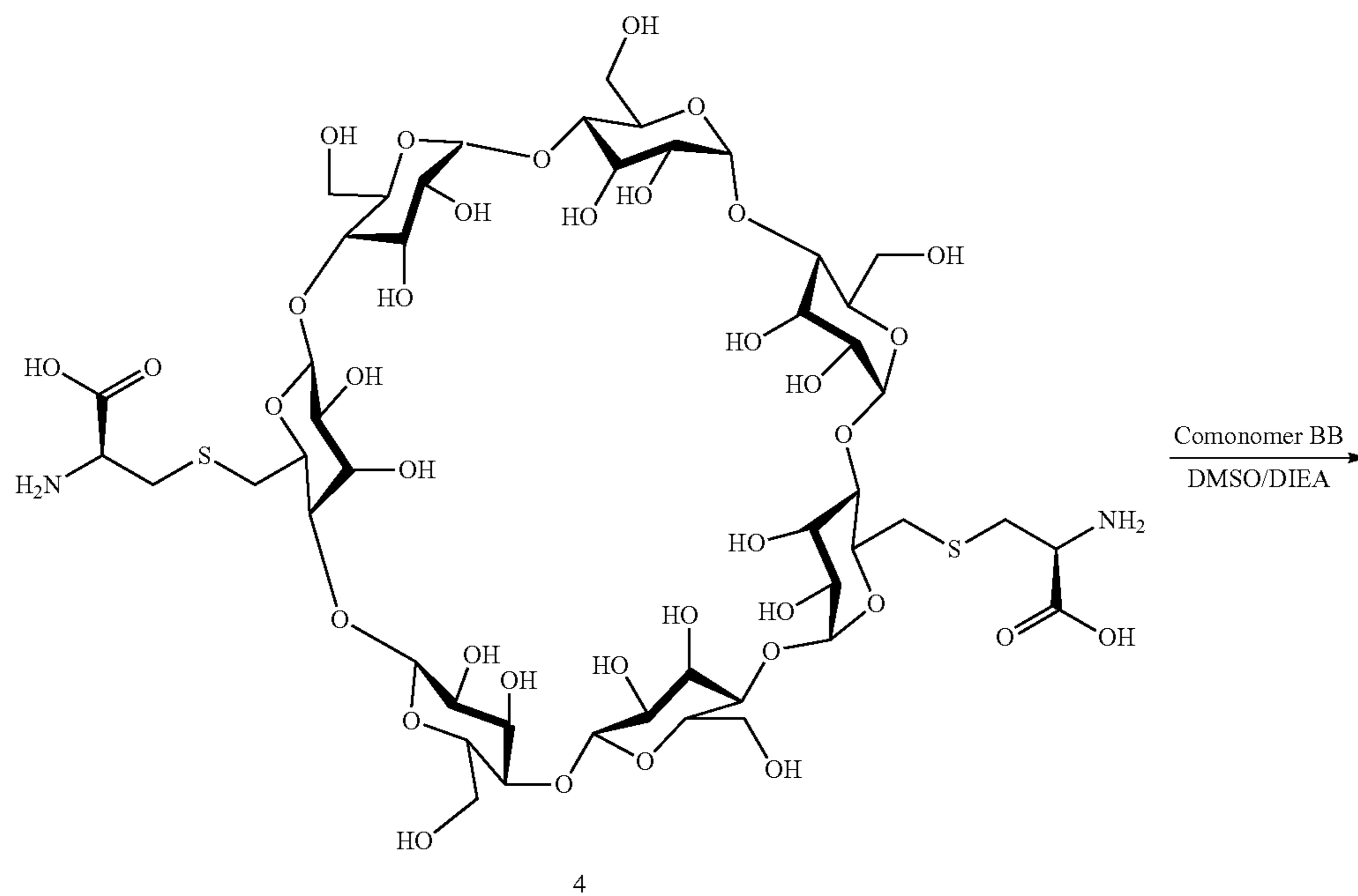
Scheme XXXVIIIb
