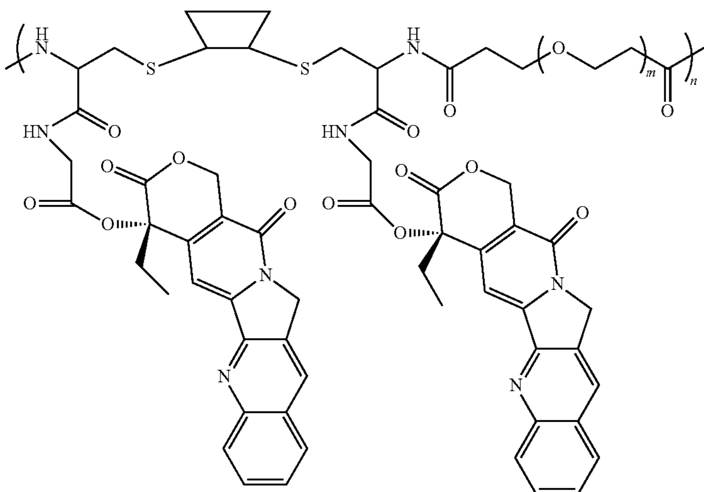
Scheme XXXVIII
