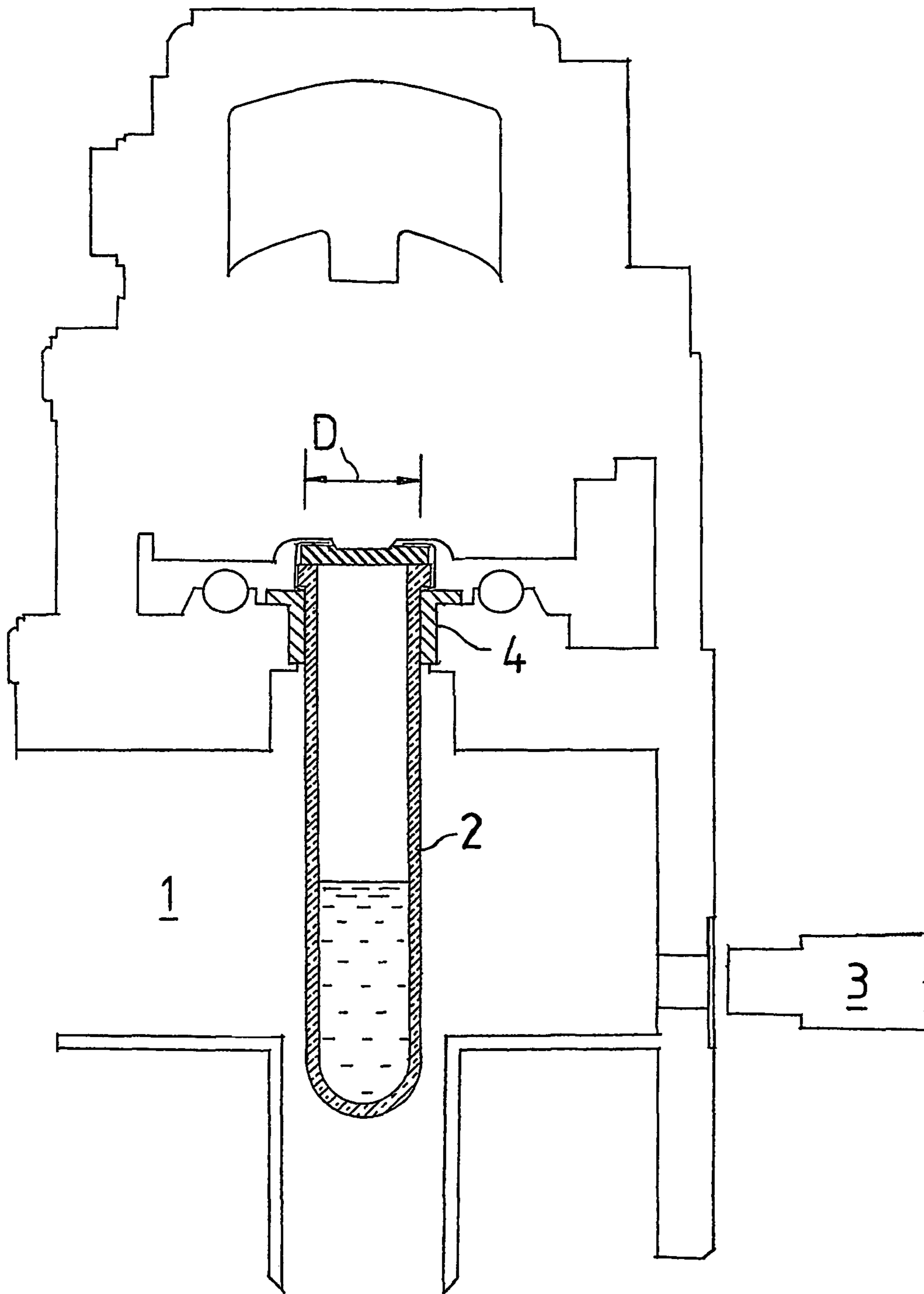
Fig.1 (Prior art vessel)
