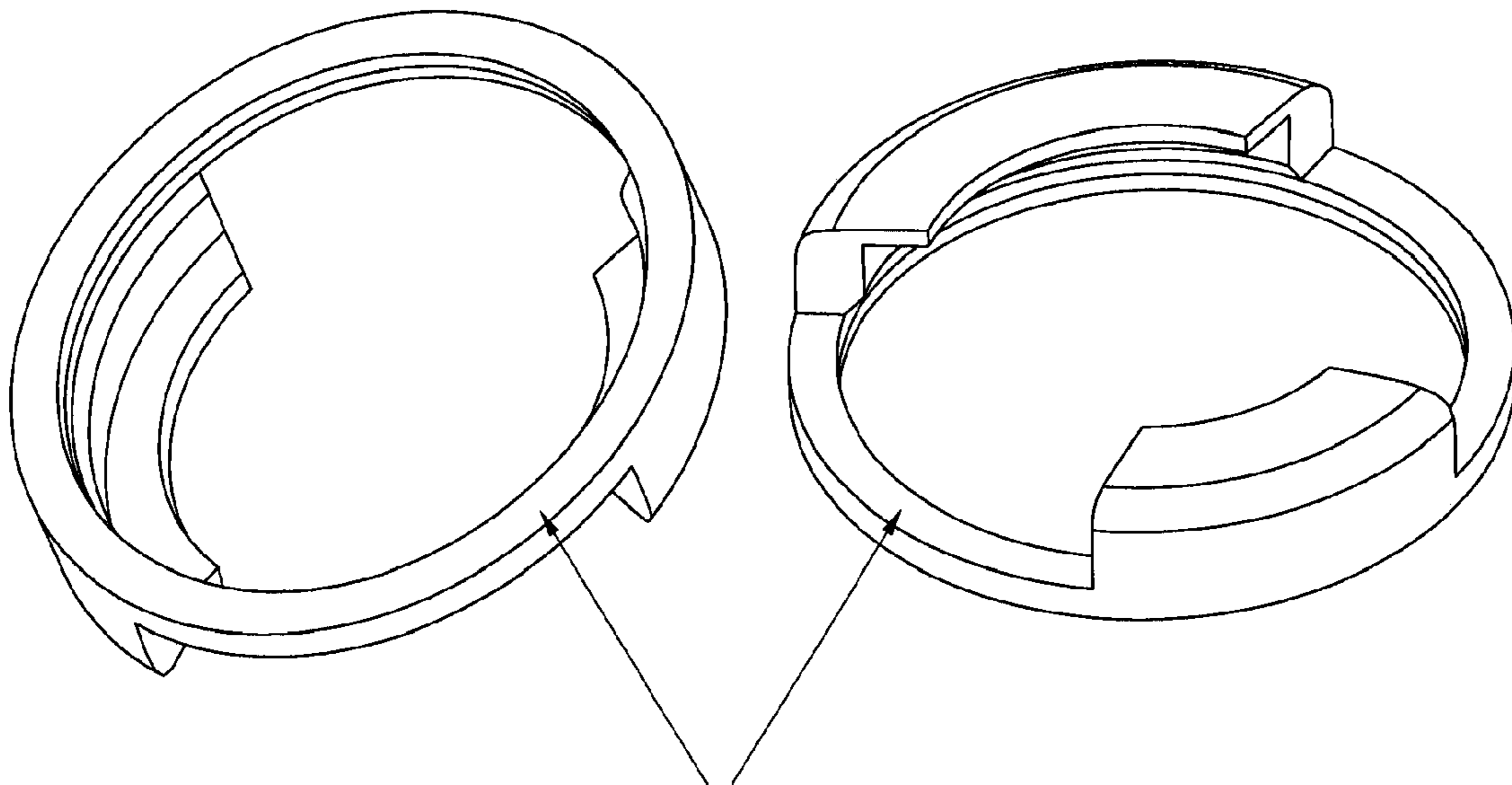
Constraining Ring (56) in Different Orientations.
