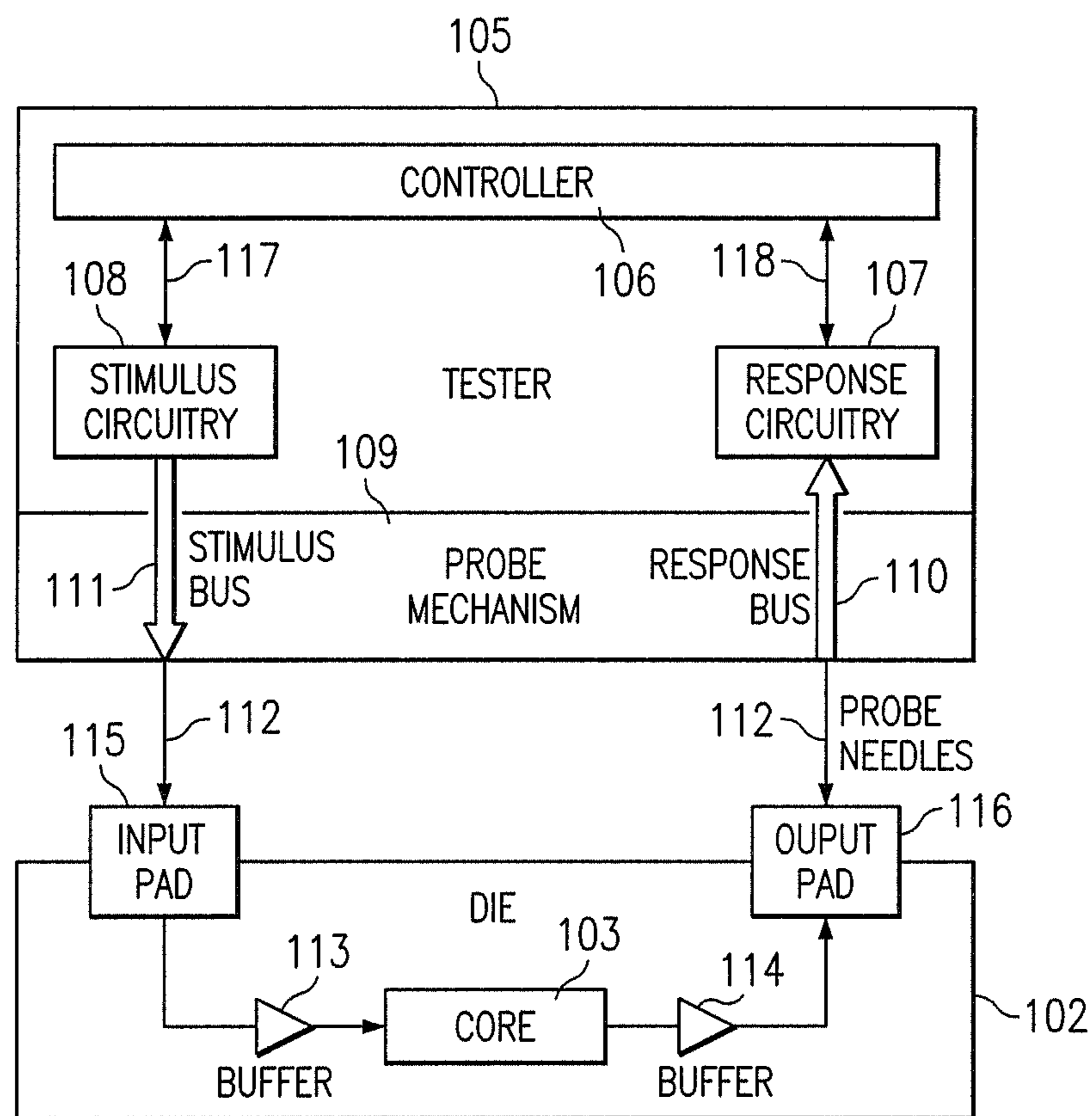
FIG. 1C (PRIOR ART)
